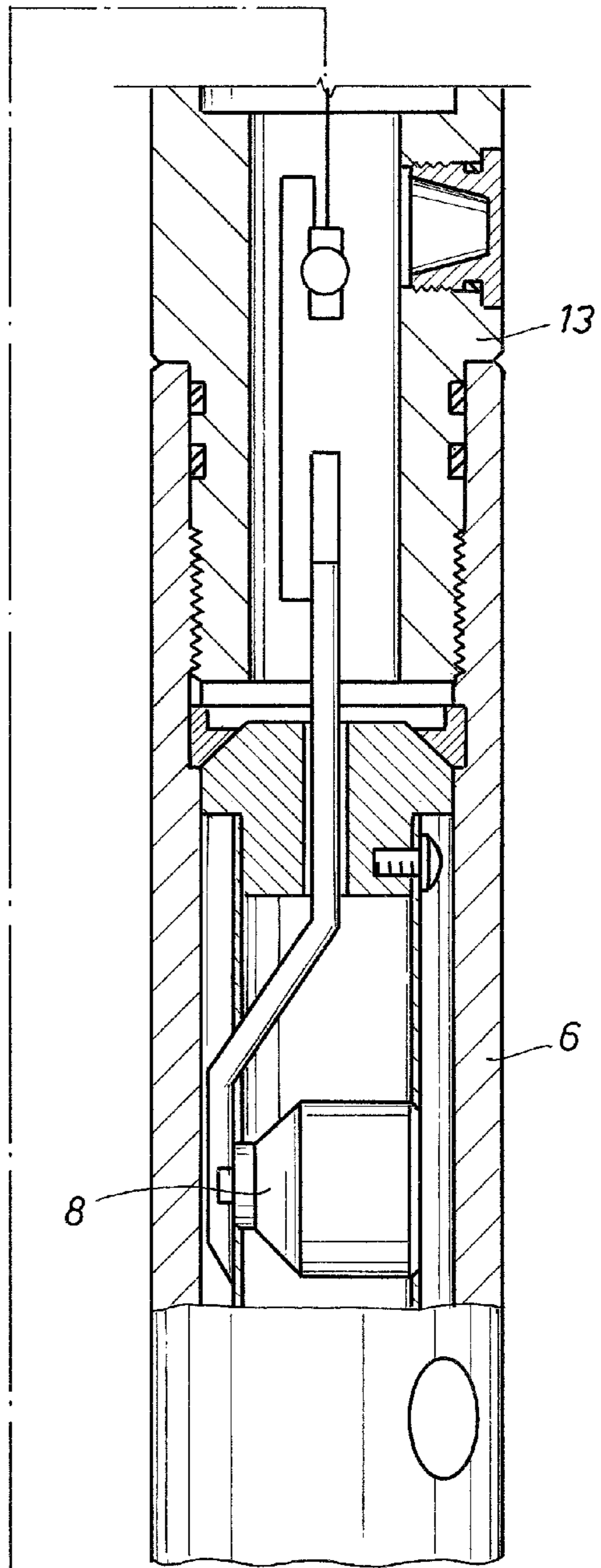
FIG. 2 (PRIOR ART)
