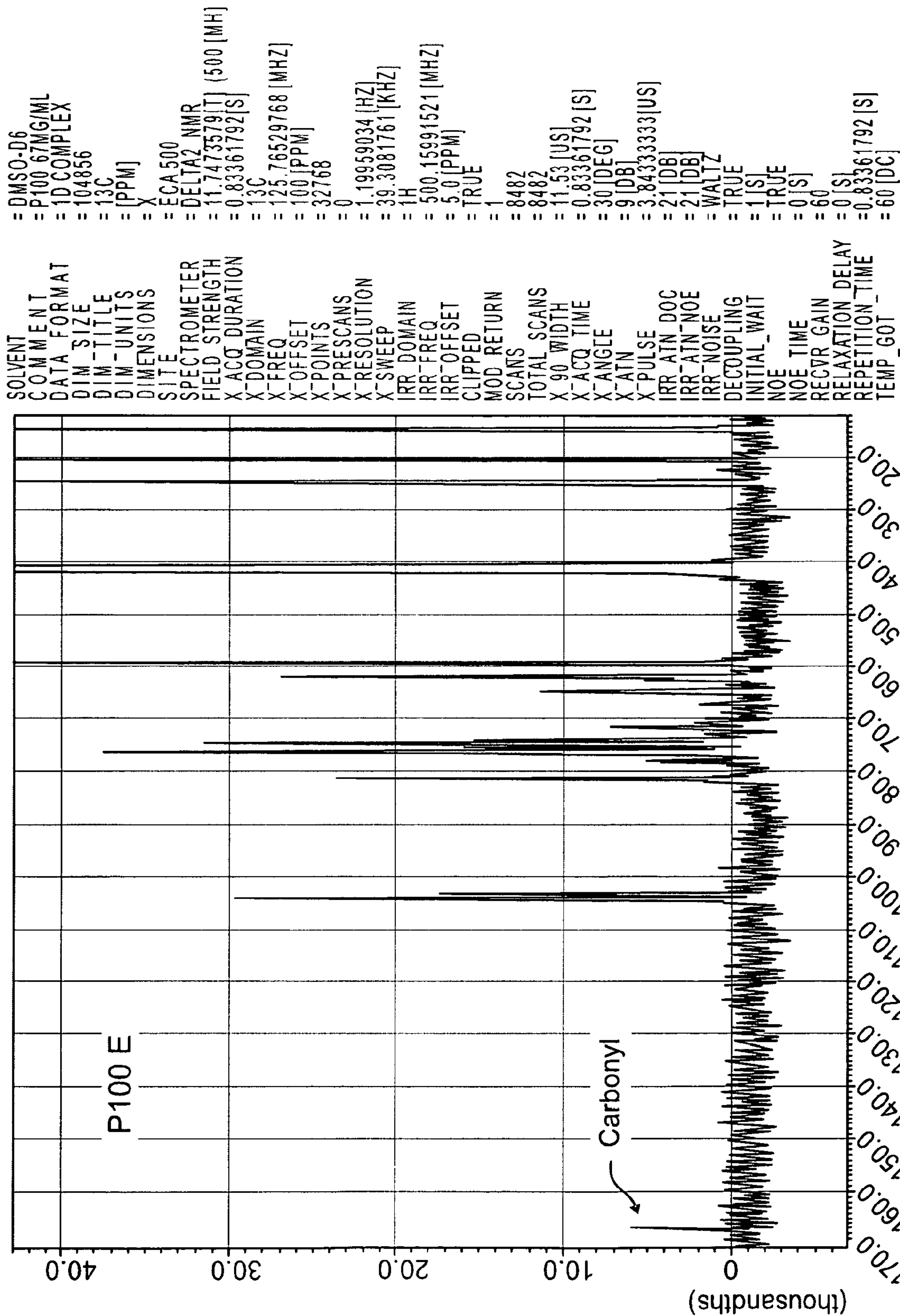
FIG. 6K X: parts per Million : 13C
