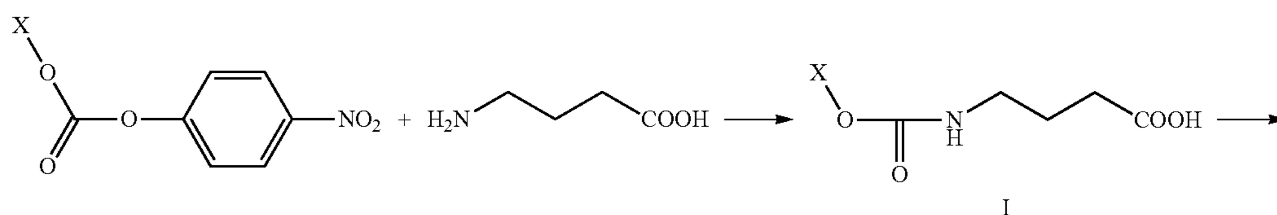
Reaction scheme 1
