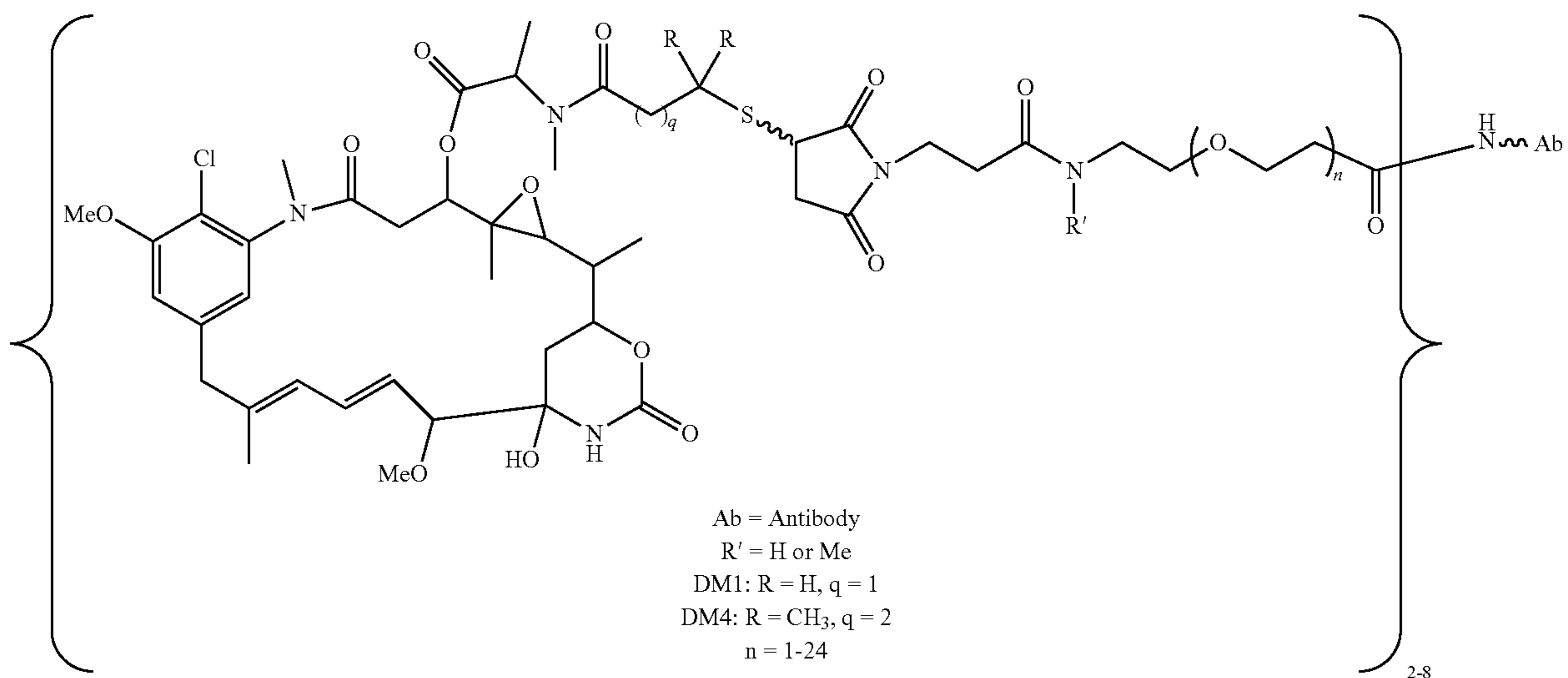
Ab-PEG-Mal-DM1/DM4
