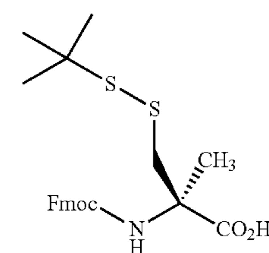
R- \alpha -methyl
