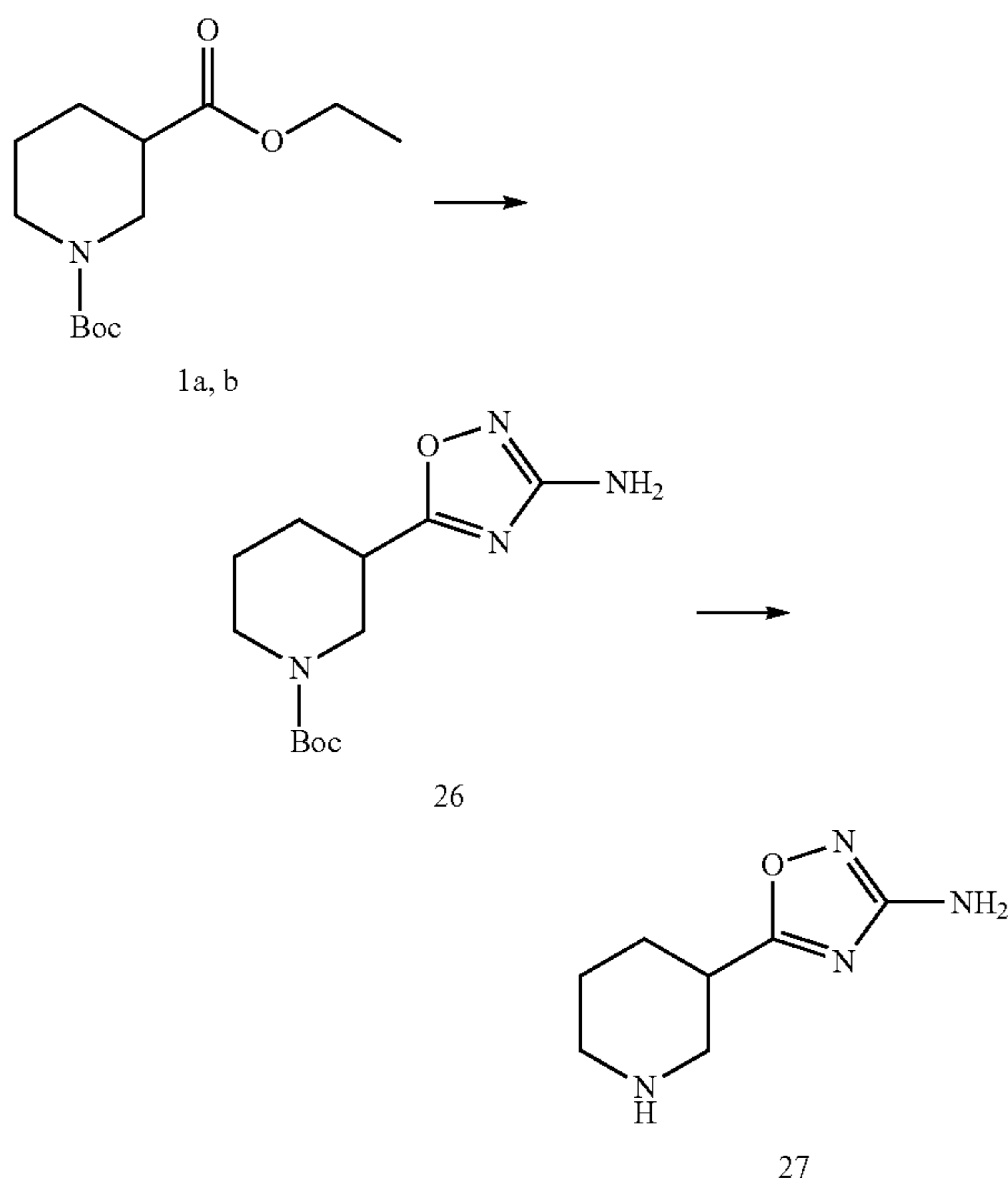
tert-Butyl 3-(3-amino-1,2,4-oxadiazol-5-yl)piperidine-1-carboxylate (26)
