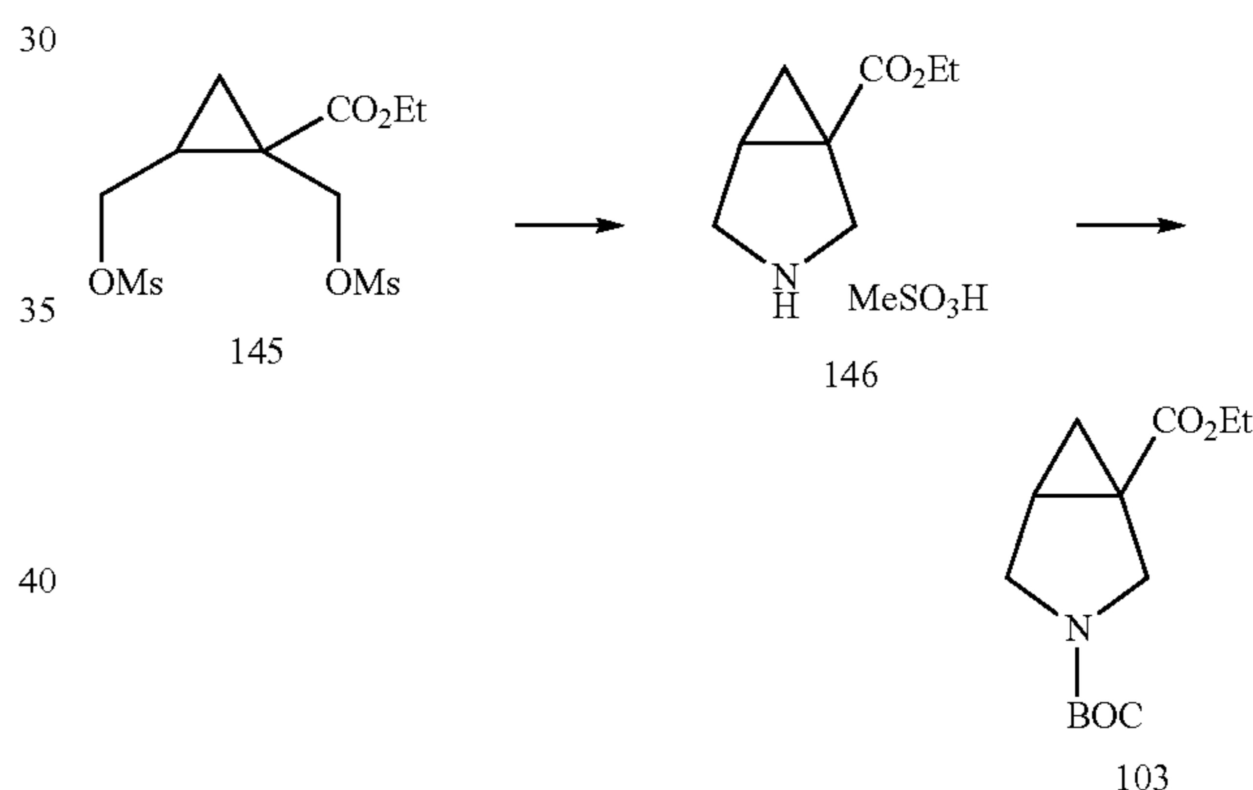
Ethyl 3-azabicyclo[3.1.0]hexane-1-carboxylate (146)
