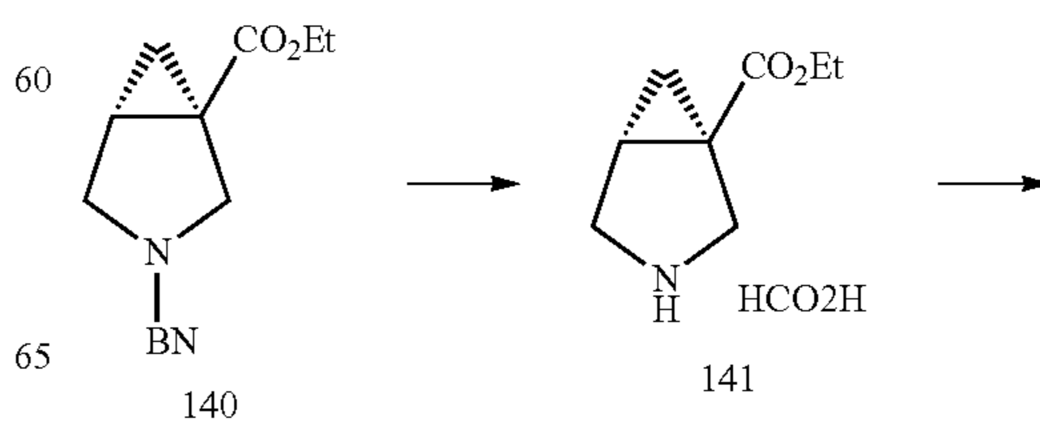
Scheme 104: Enantiospecific synthesis of azabicyclo compounds.
