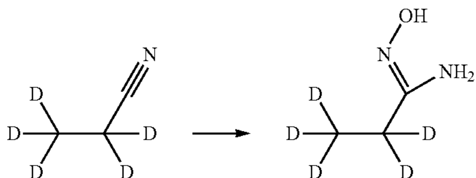
Step 1: 2,3,3,3-d 5 -Propionamideoxime
