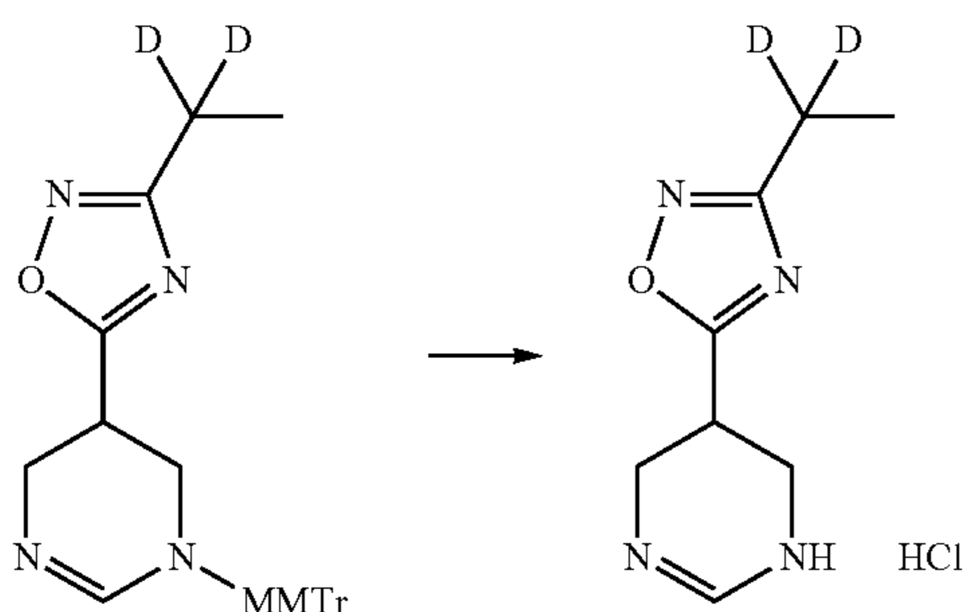
Step 4: 3-(2,2-d 2 -Ethyl)-5-(1,4,5,6-tetrahydropyrimidin-5-yl)-1,2,4-oxadiazole hydrochloride
