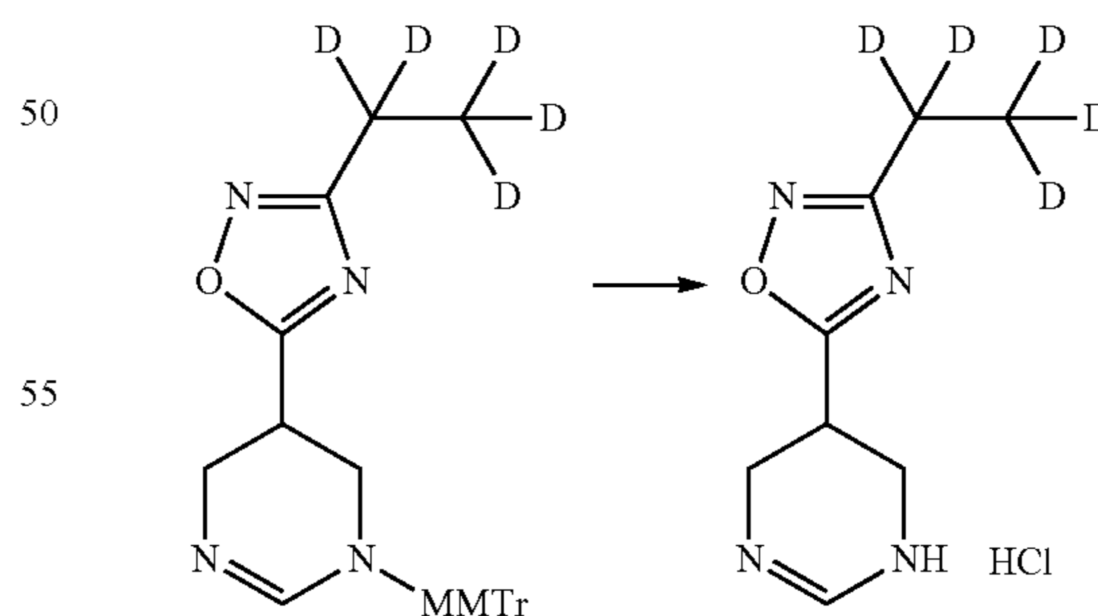
Step 3: 3-(1,1,2,2,2-d 5 -ethyl)-5-(1,4,5,6-tetrahydropyrimidin-5-yl)-1,2,4-oxadiazole hydrochloride
