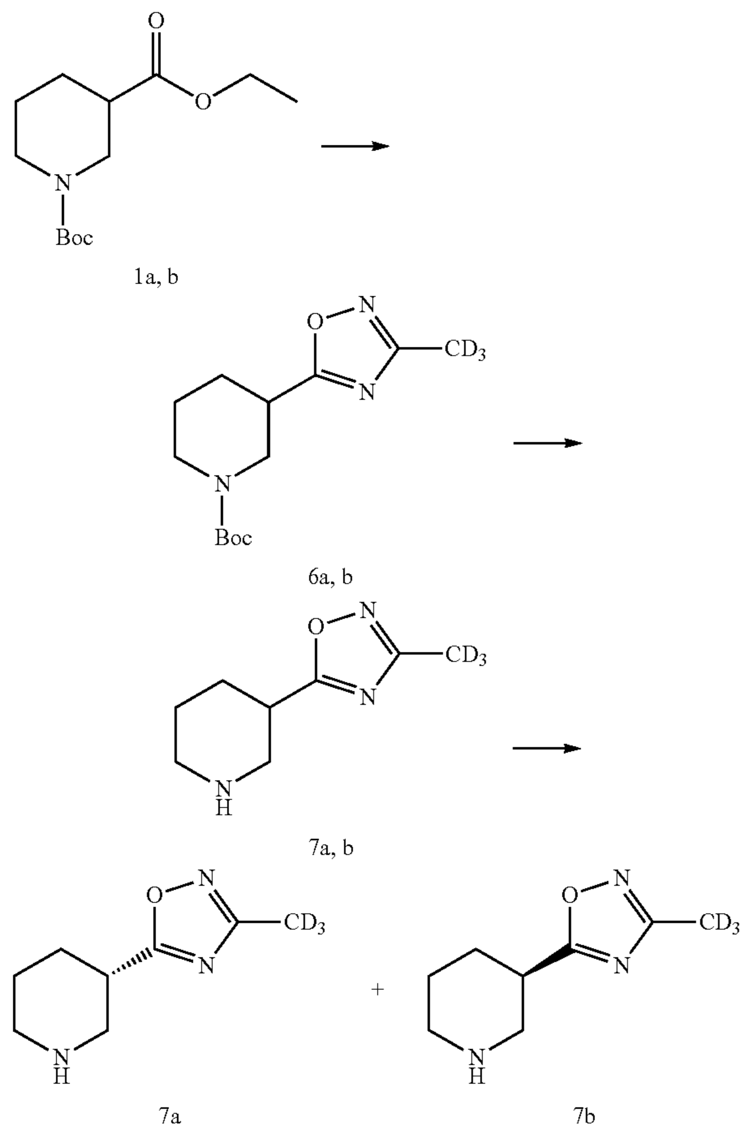
tert-Butyl 3-(3-D3-methyl-1,2,4-oxadiazol-5-yl)piperidine-1-carboxylate (6a,b)
