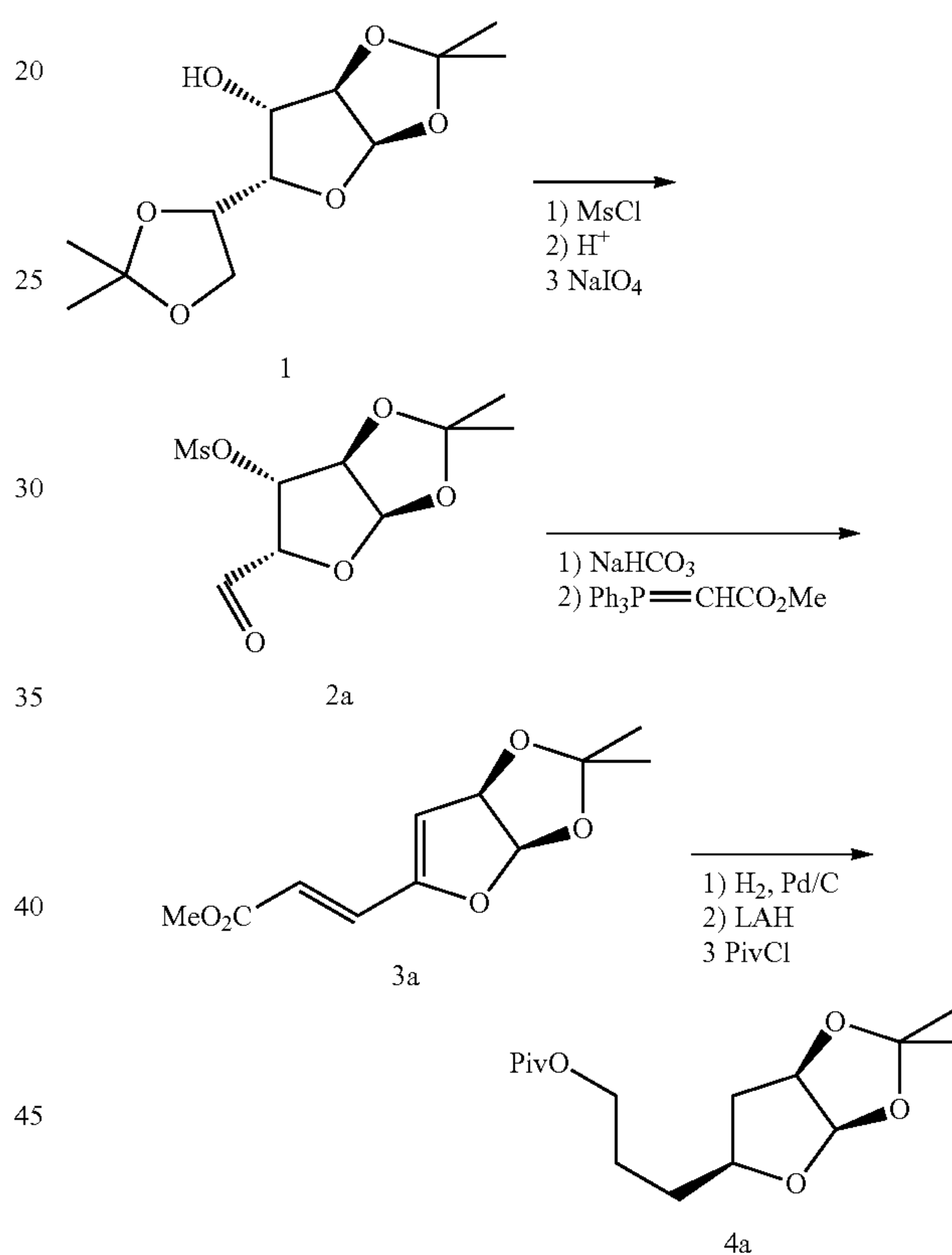
Scheme 1: Schematic representation of a process for preparation of compound of formula 4a.
