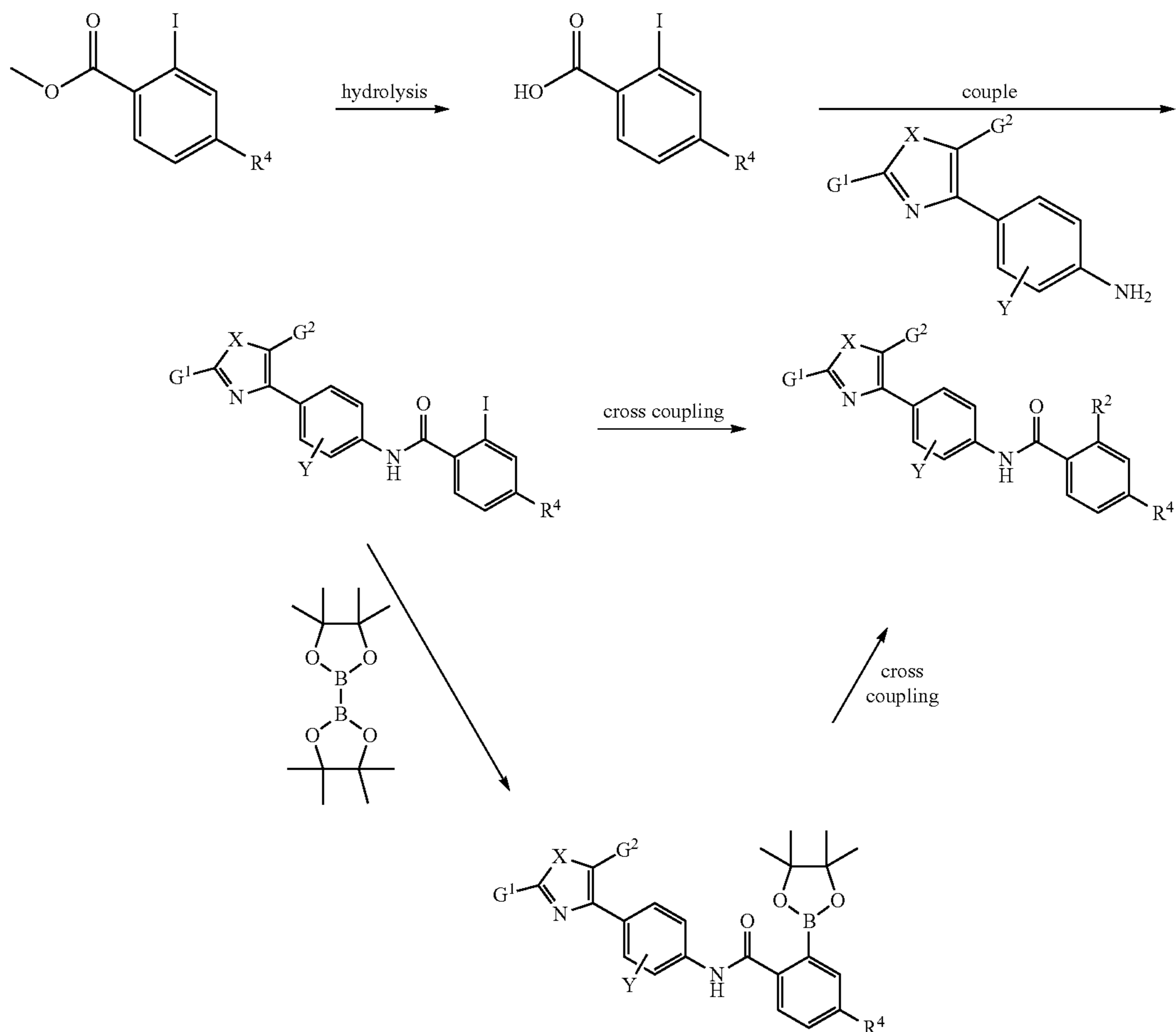
Scheme 1
