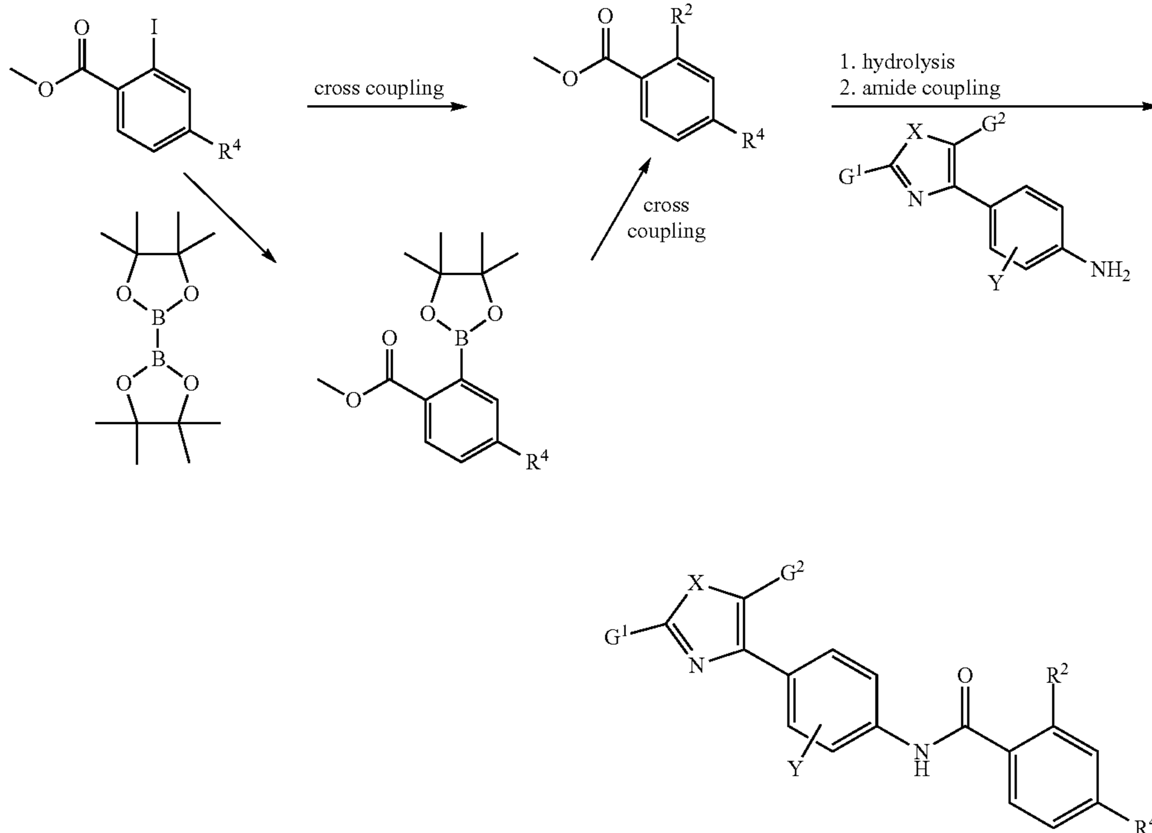
Scheme 3
