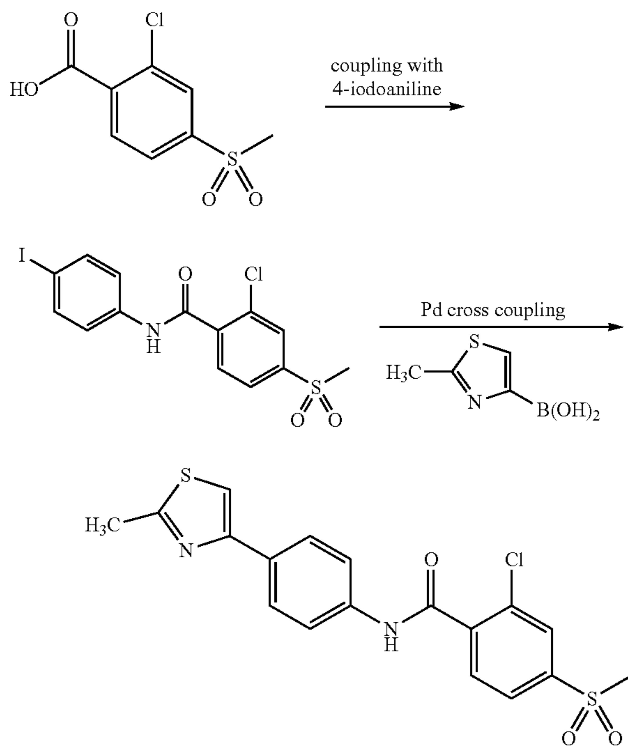
Scheme 2
