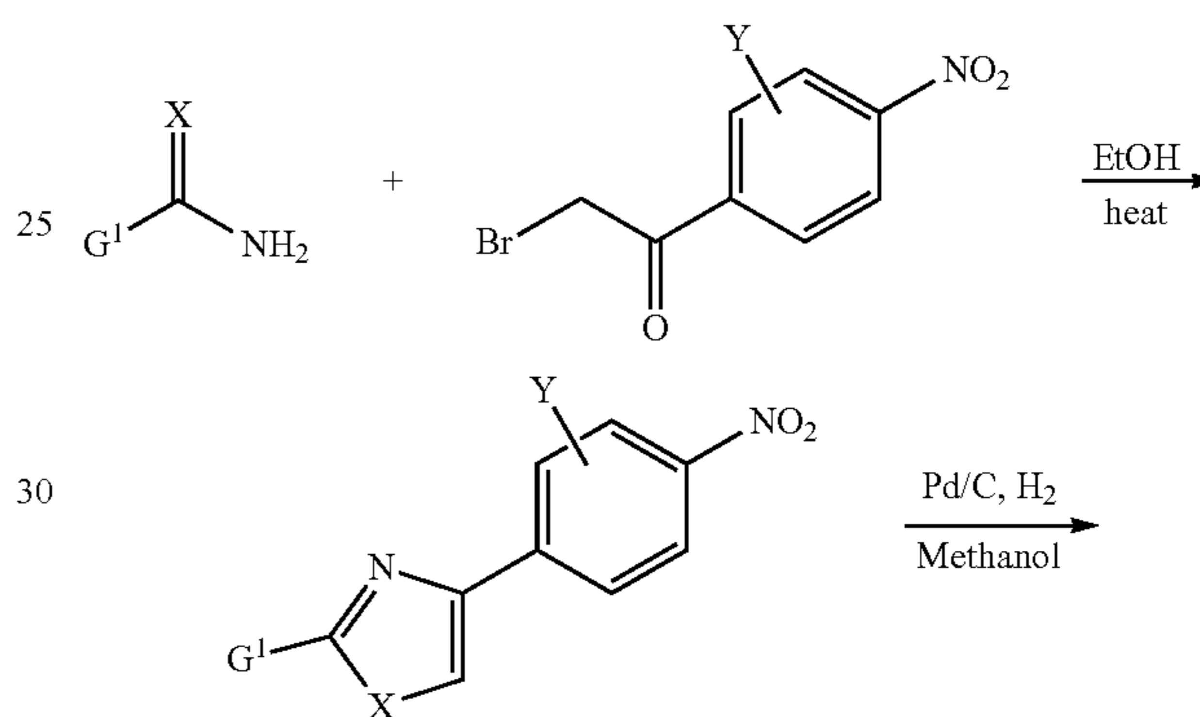
Scheme 4
