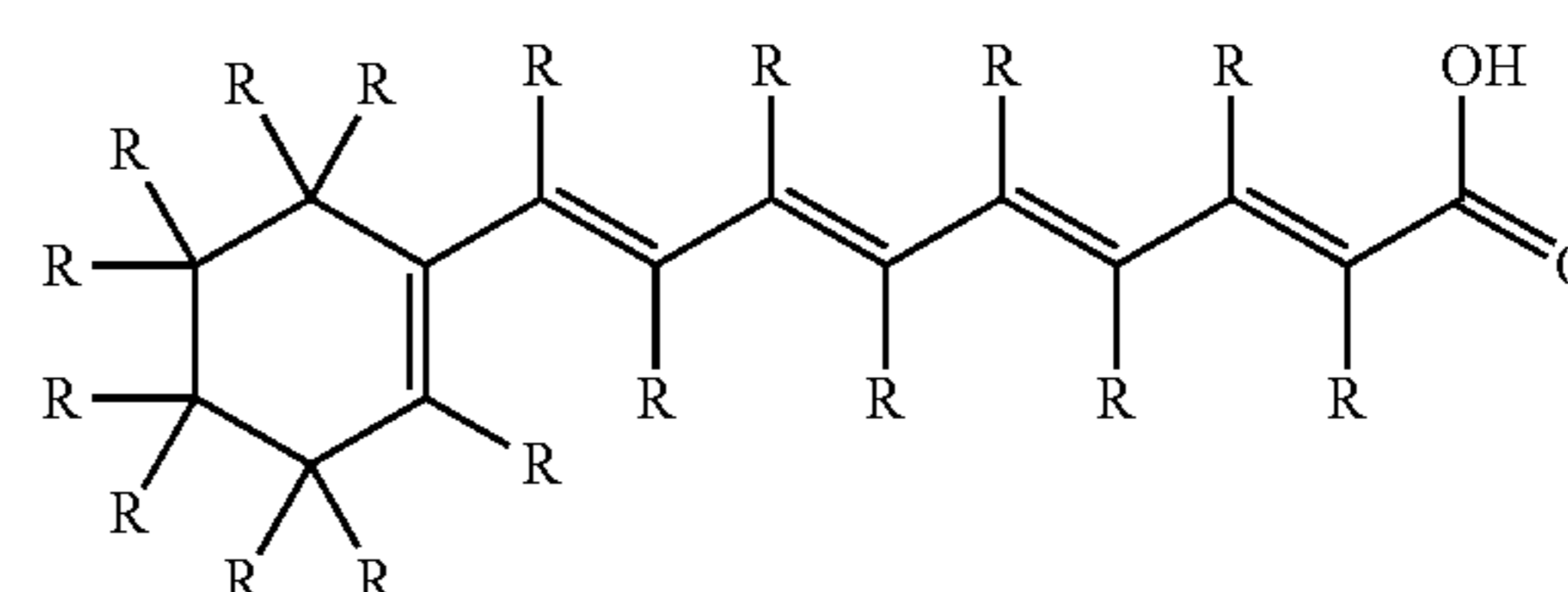
all-trans-retinoic acids
