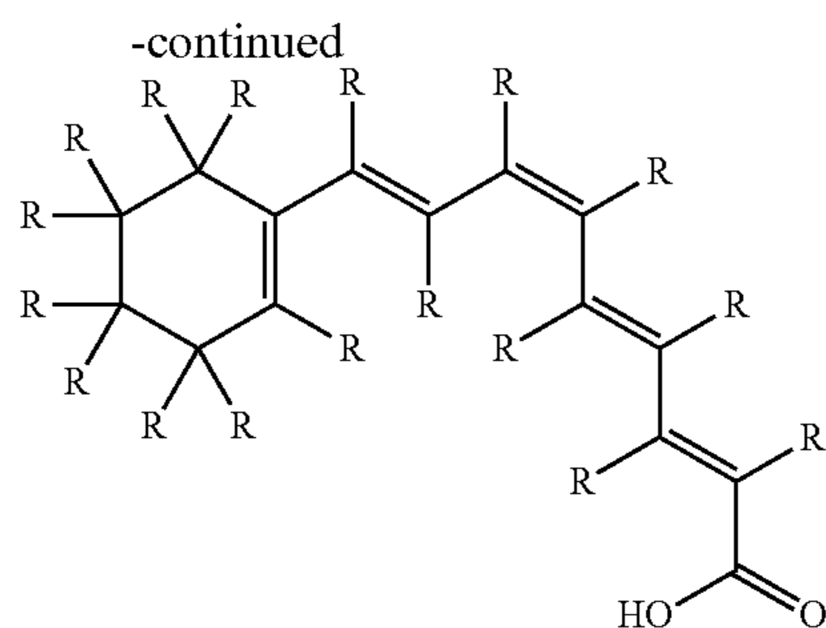
9-cis-retinoic acids
