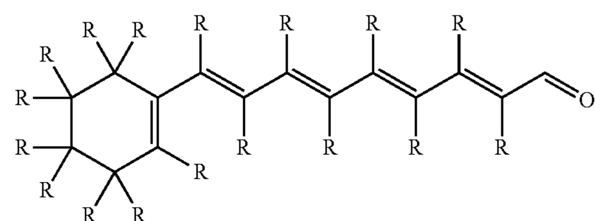
all-trans-retinals
