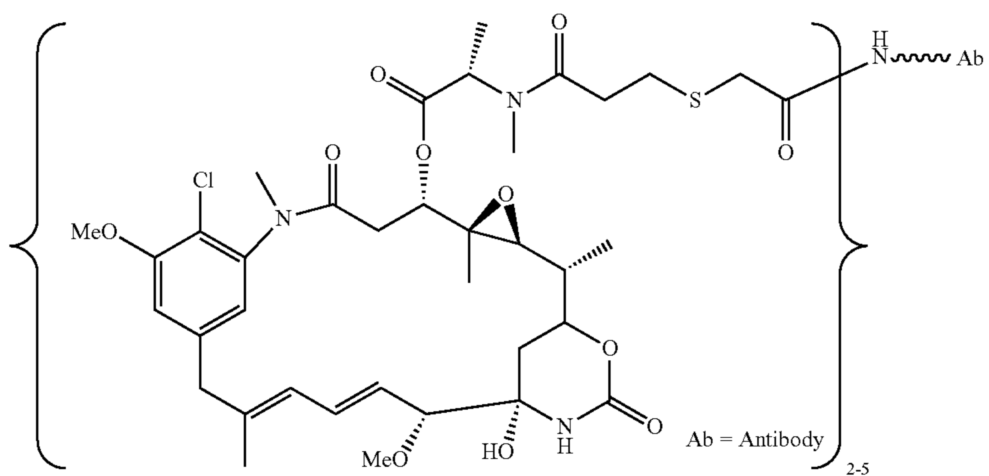
Ab-SIA-SM1
