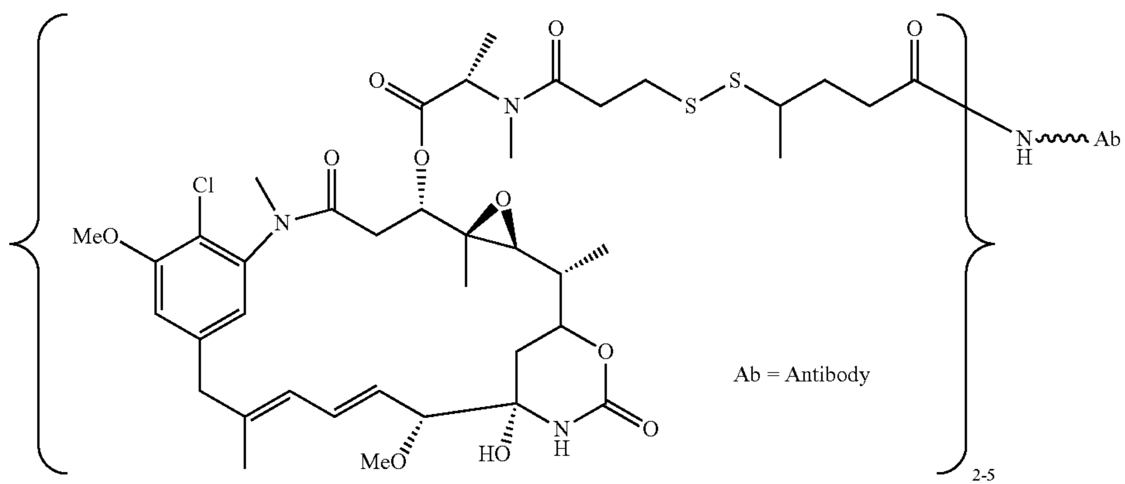
Ab-SPP-DM1
