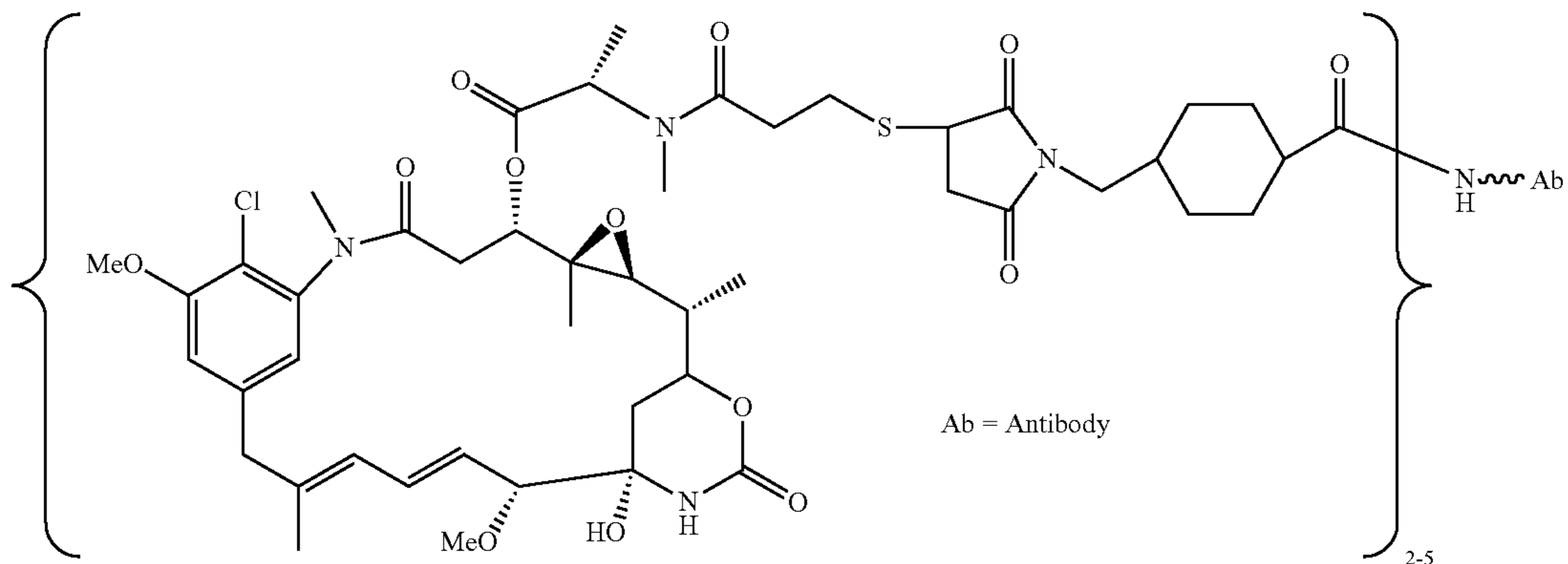
Ab-SMCC-DM1
