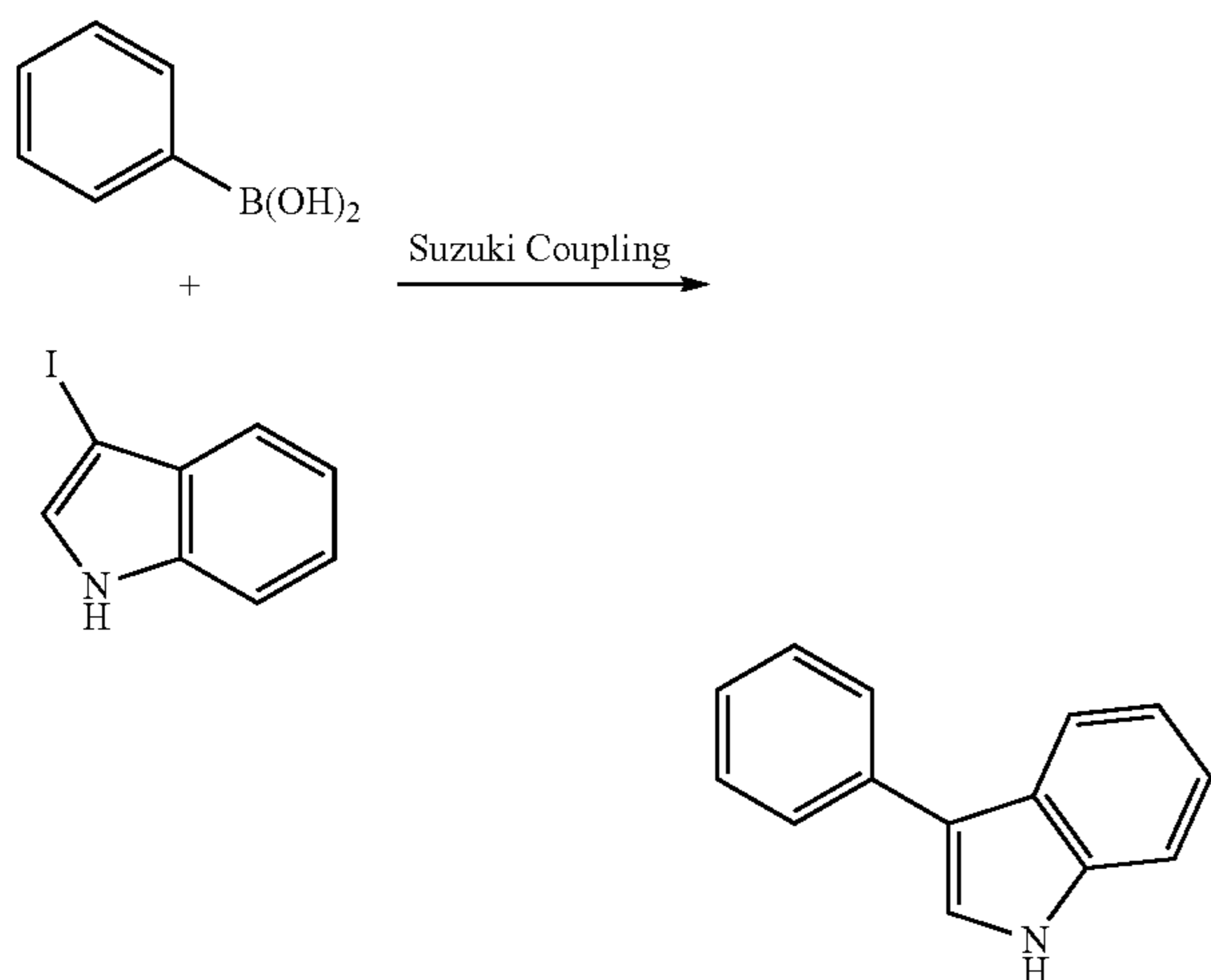
Suzuki Coupling No. 1:
