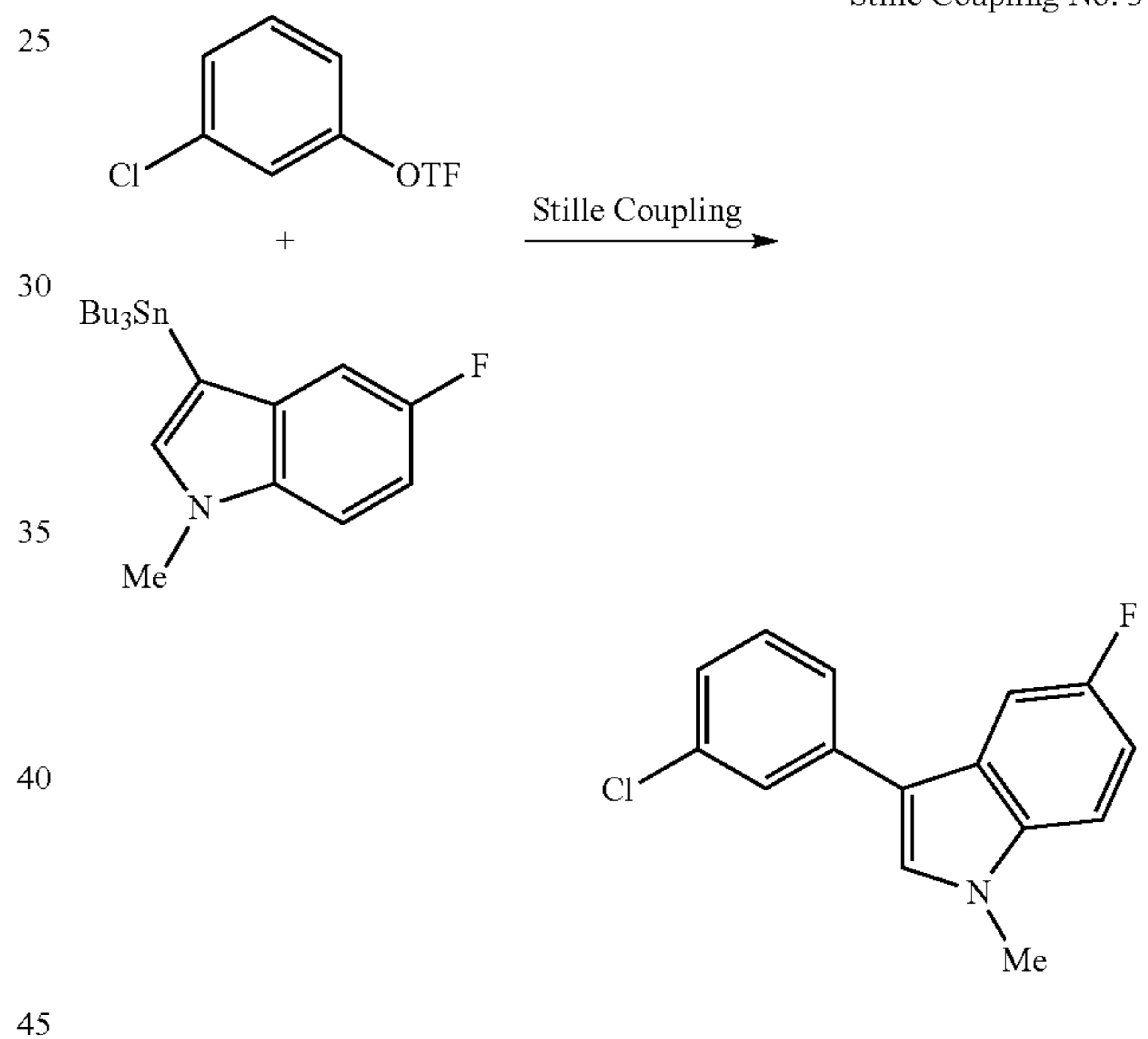
Stille Coupling No. 3
