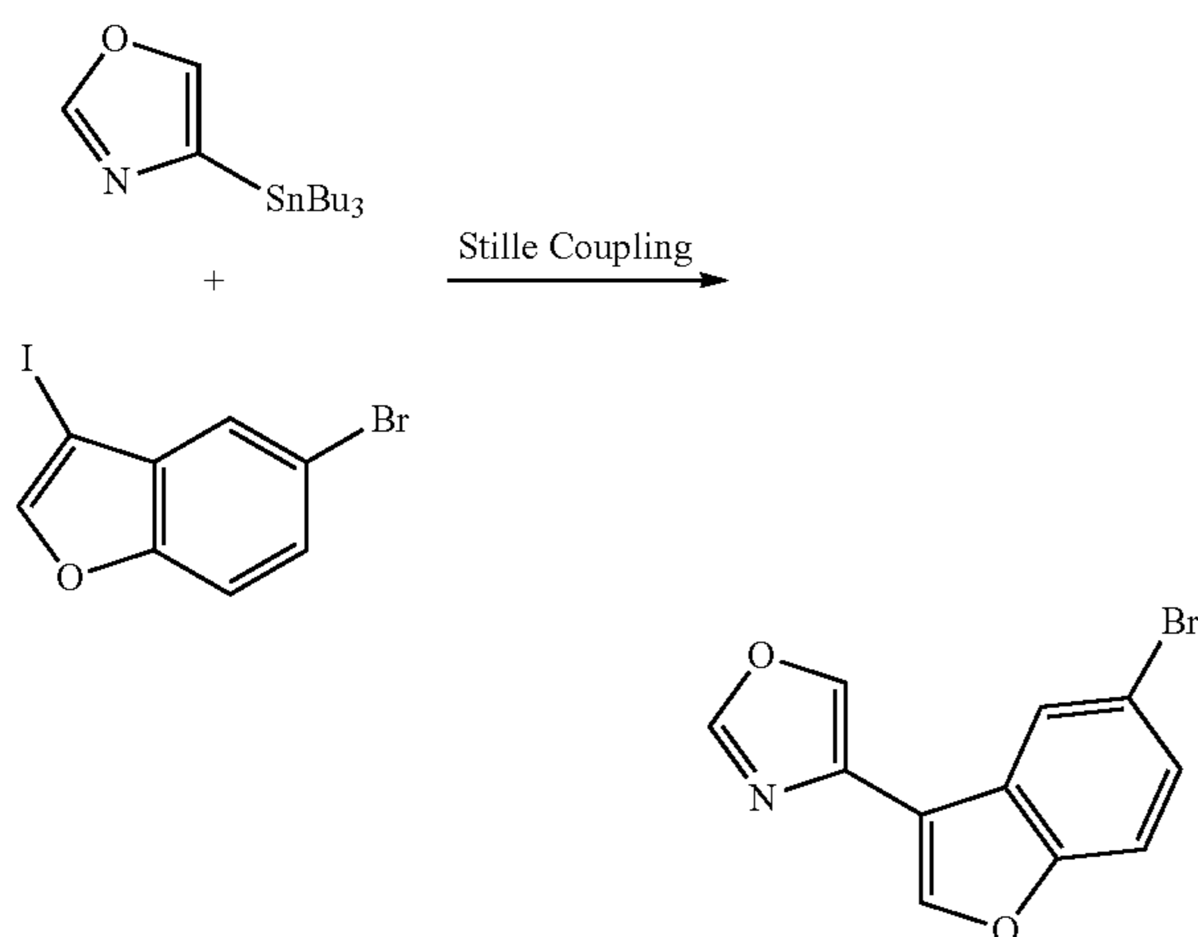
Stille Coupling No. 1:
