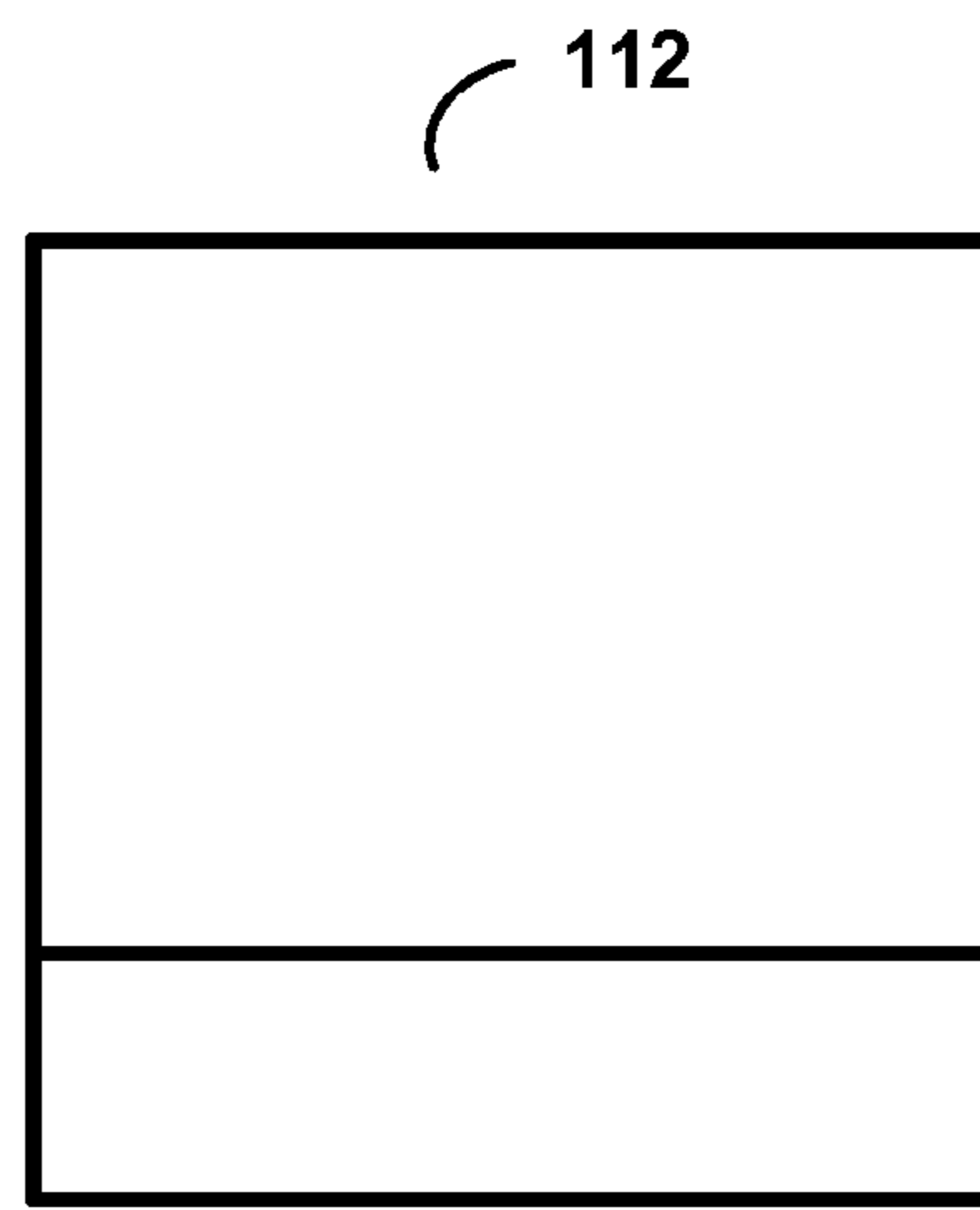
2NxnD (Inter-Prediction)
