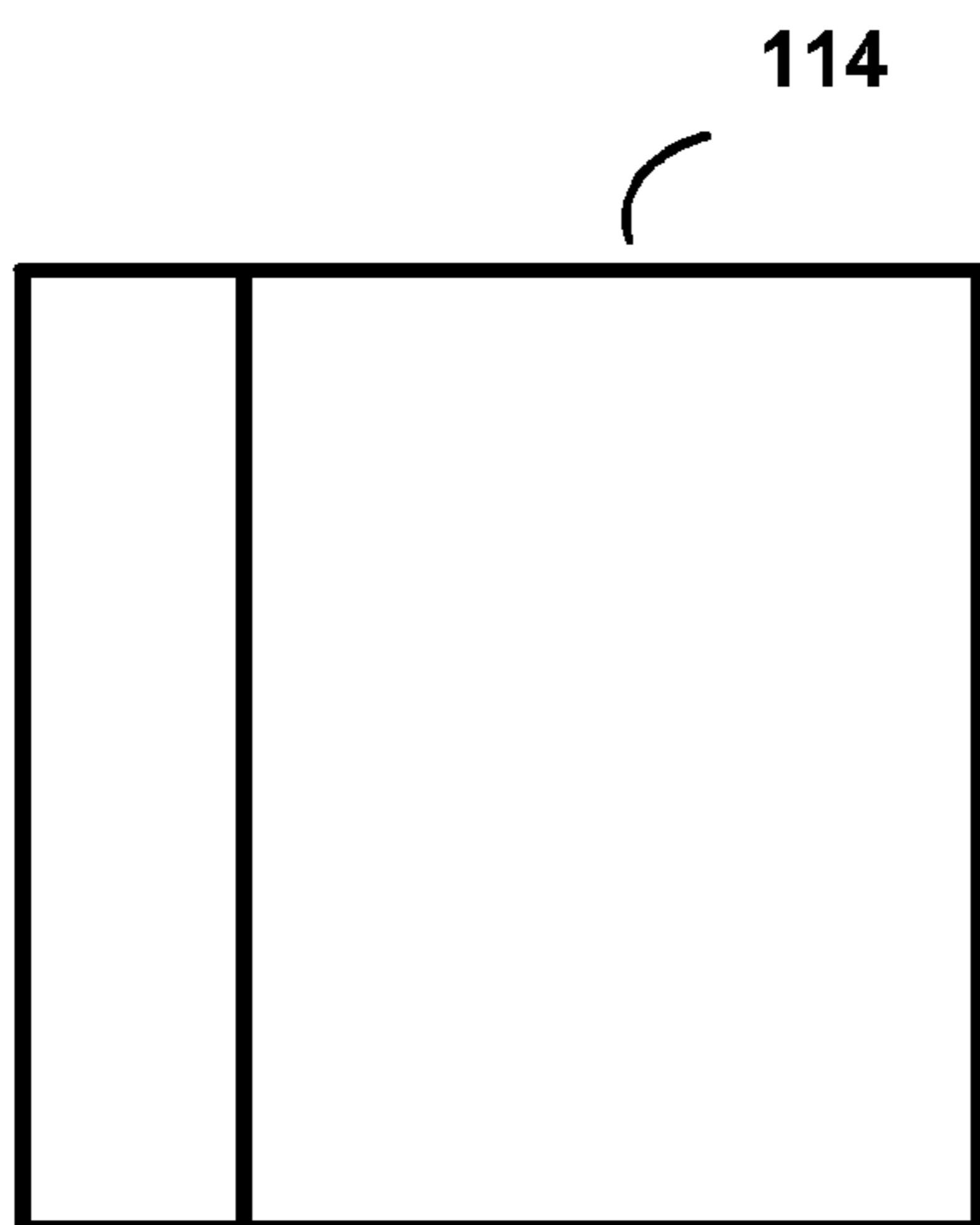
nLx2N (Inter-Prediction)
