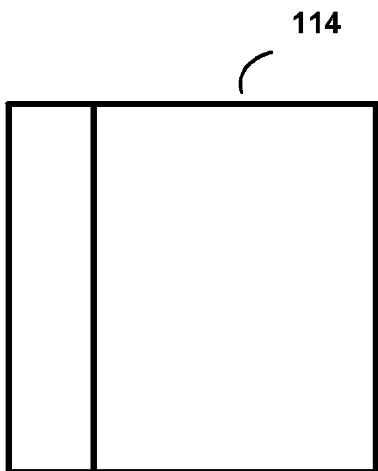
nLx2N (Inter-Prediction)
