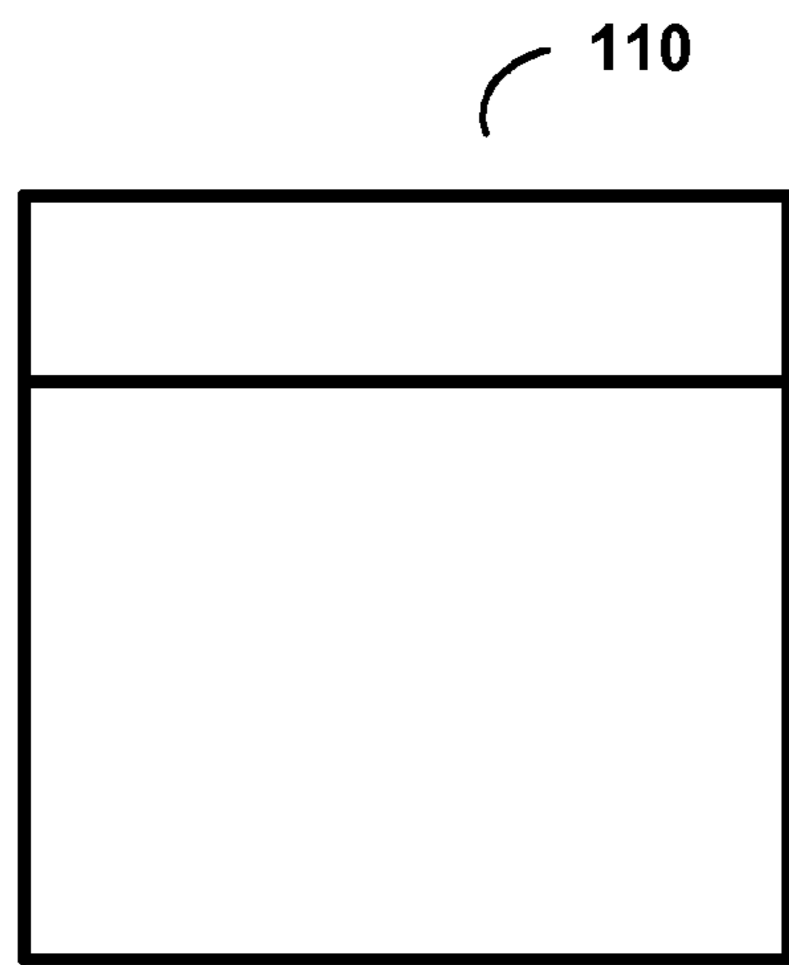
2NxnU (Inter-Prediction)
