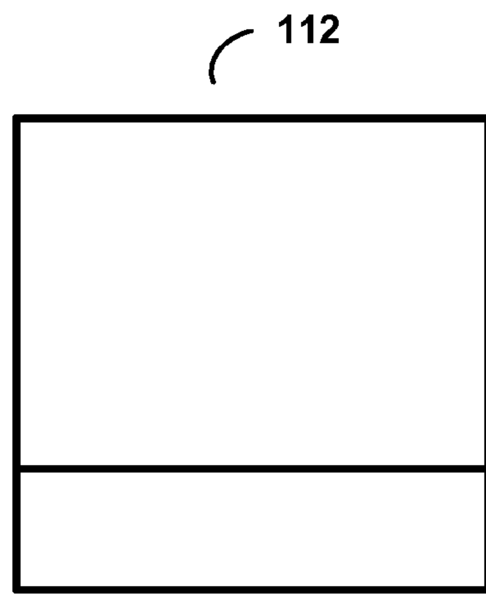
2NxnD (Inter-Prediction)
