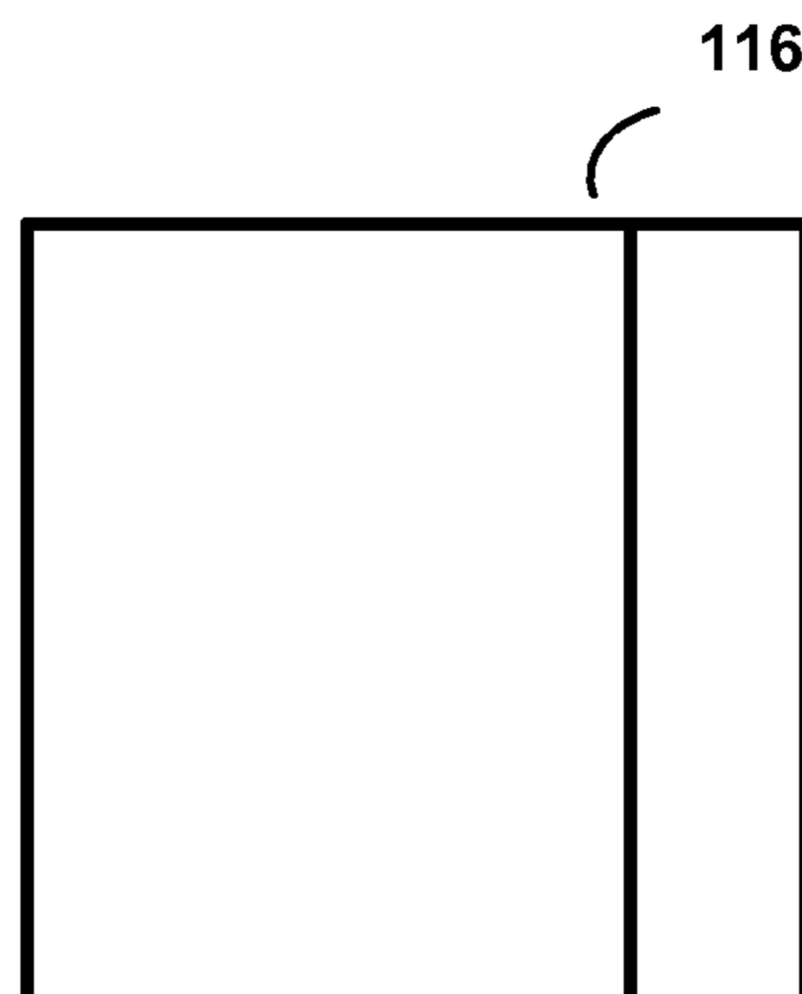
nRx2N (Inter-Prediction)
