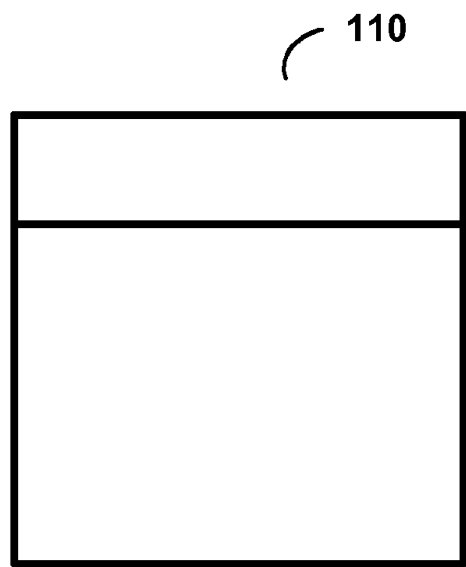
2NxnU (Inter-Prediction)
