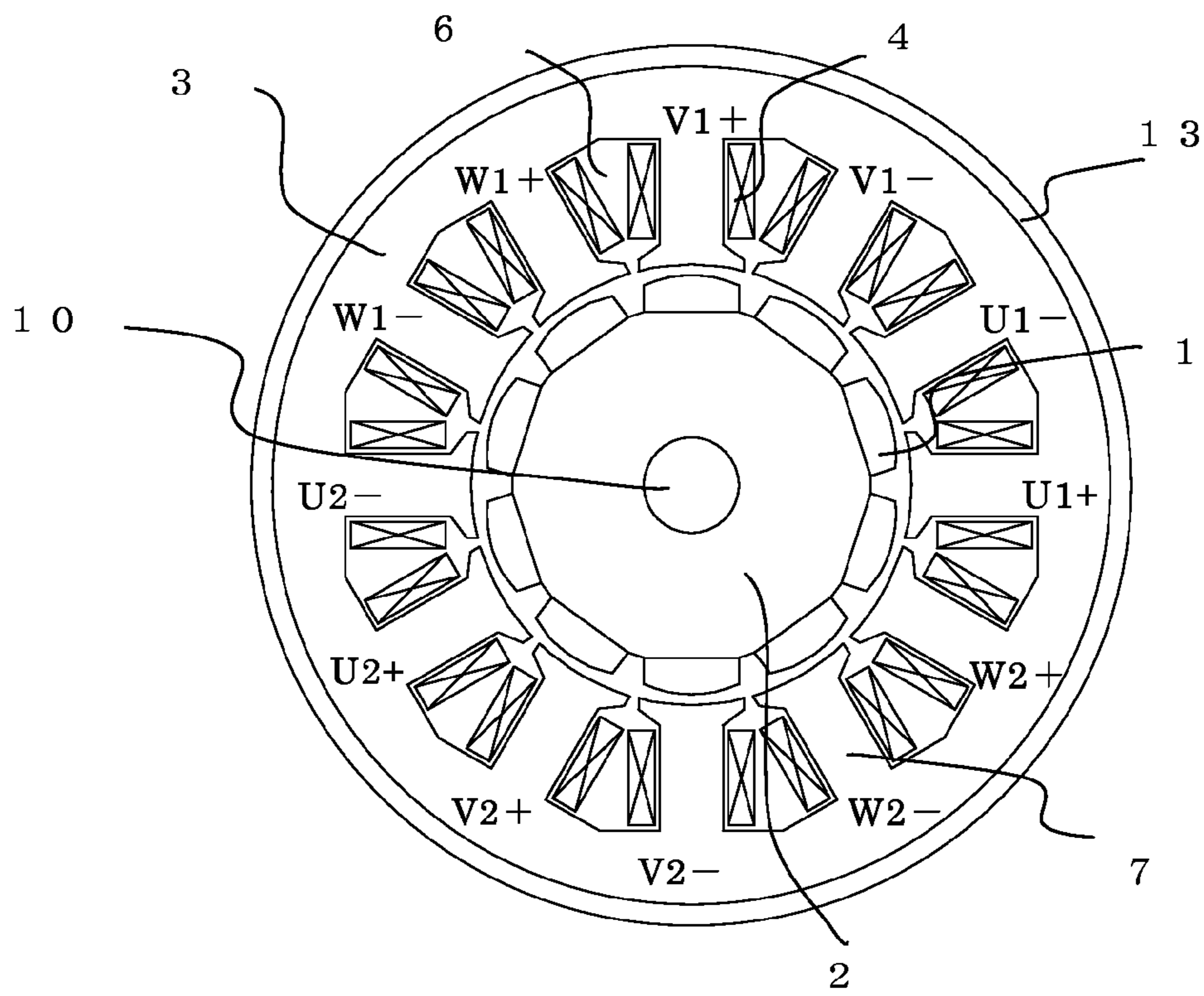
C1—C2 cross-section
