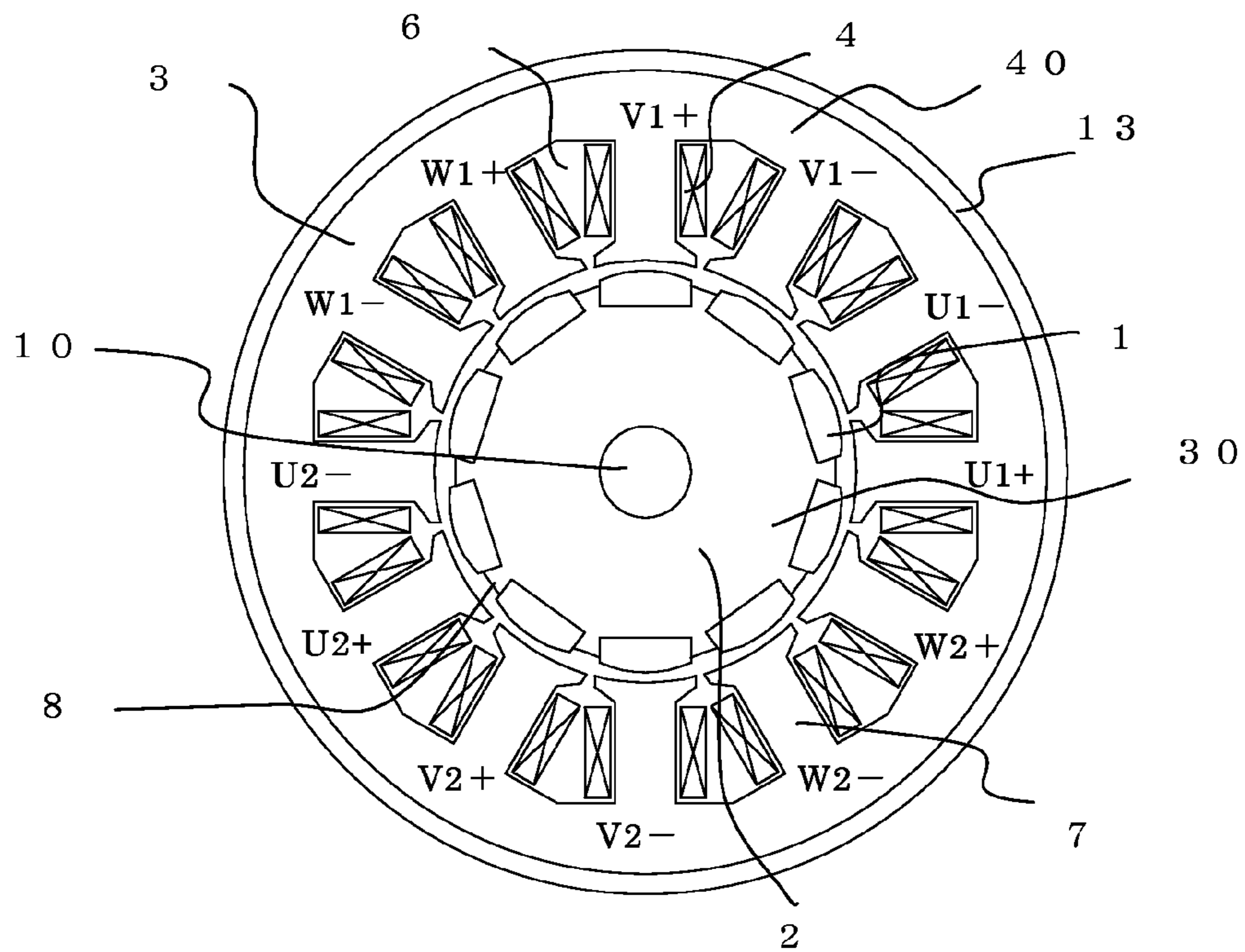
A1-A2 cross-section
