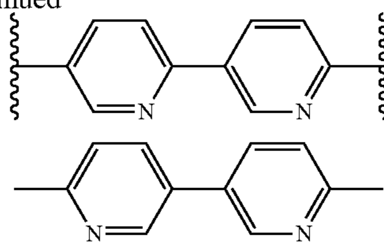
bipyridinyl
