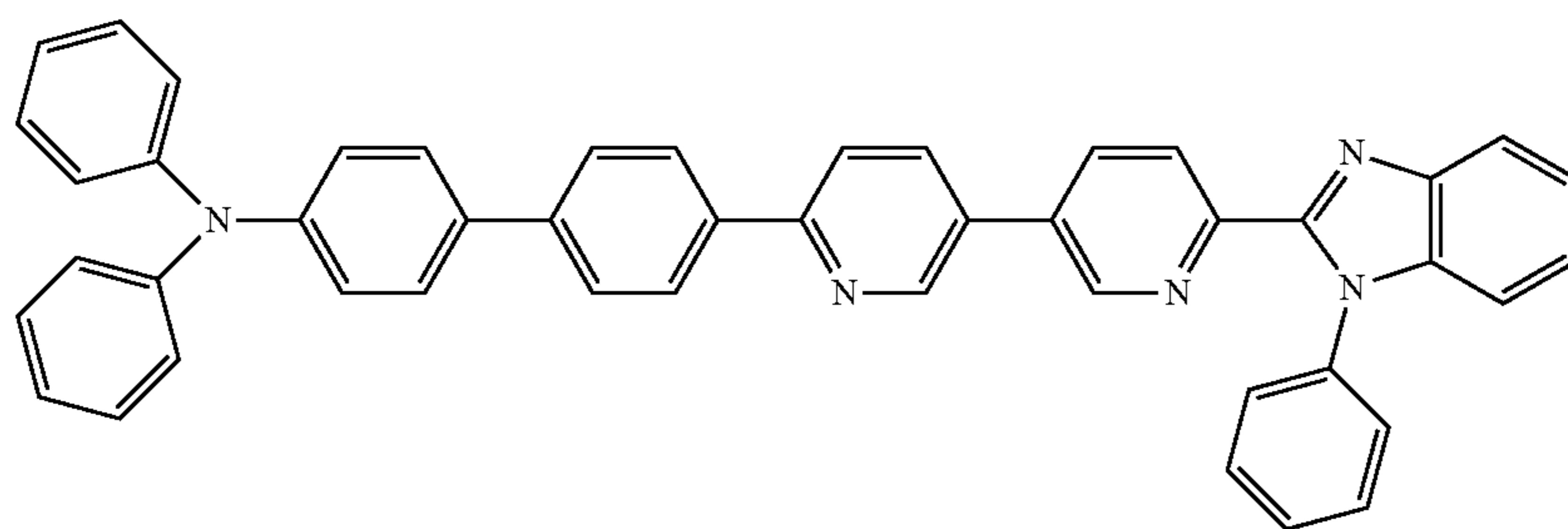
N,N-diphenyl-4'-(6'-(1-phenyl-1H-benzo[d]imidazol-2-yl)-[3,3'-bipyridin]-6-yl)-[1,1'-biphenyl]-4-amine,
