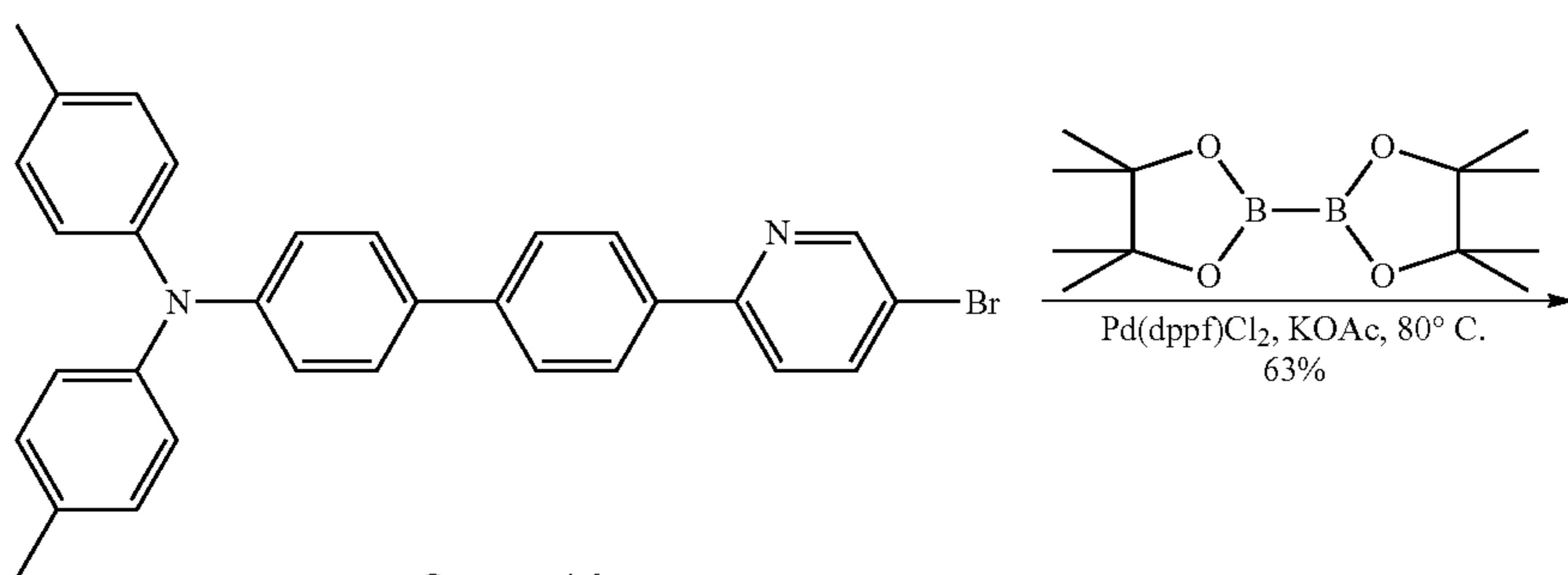
Compound 6
