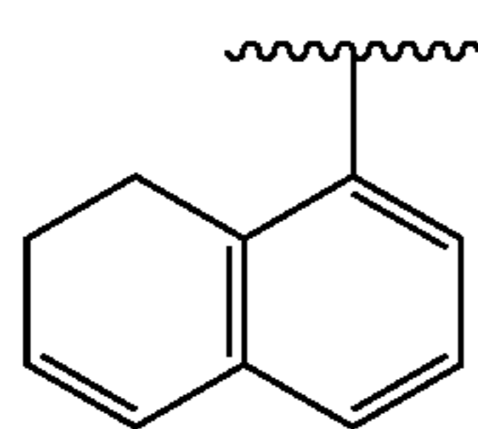
naphth-1-yl
