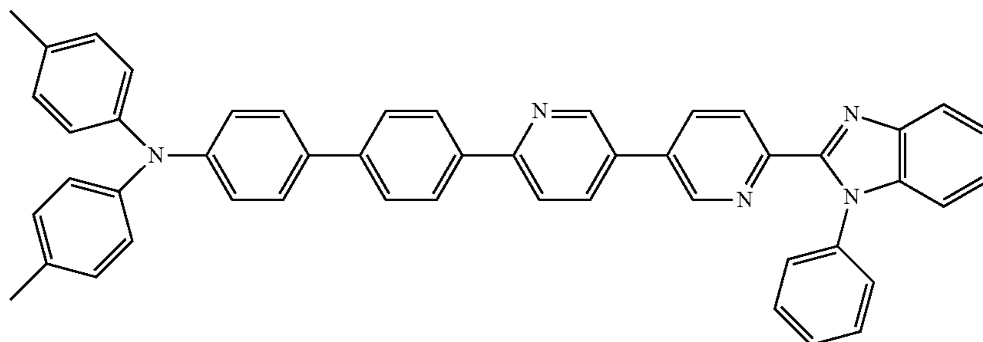
4'-(6'-(1-phenyl-1H-benzo[d]imidazol-2-yl)-[3,3'-bipyridin]-6-yl)-N,N-di-p-tolyl-[1,1'-biphenyl]-4-amine,
