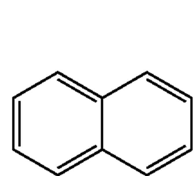
naphthyl
