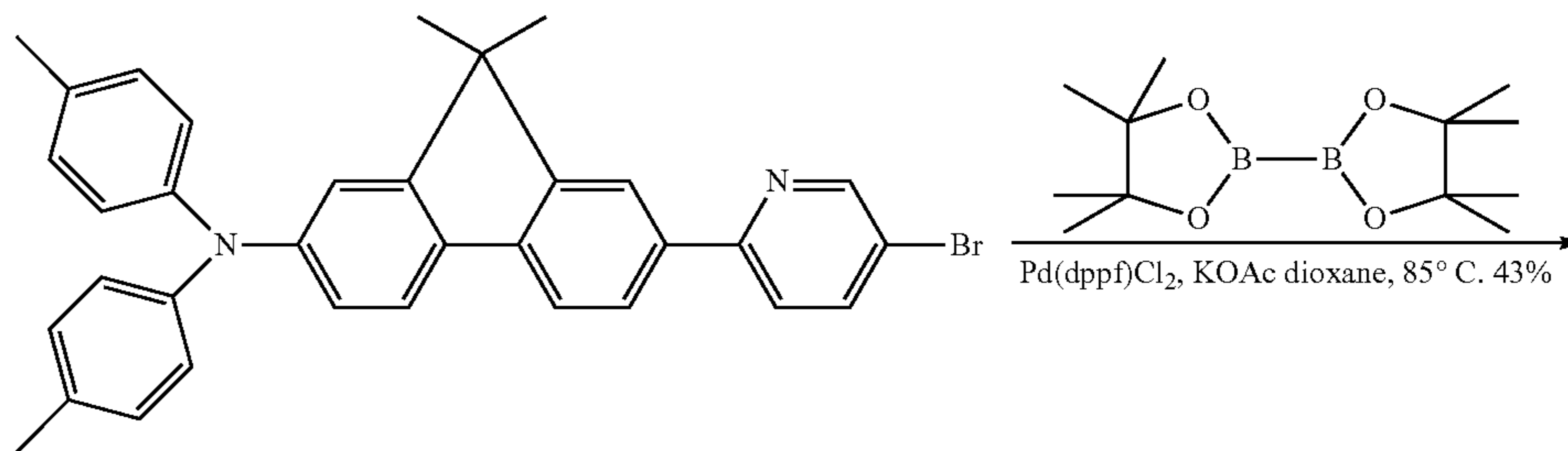
Compound 34
