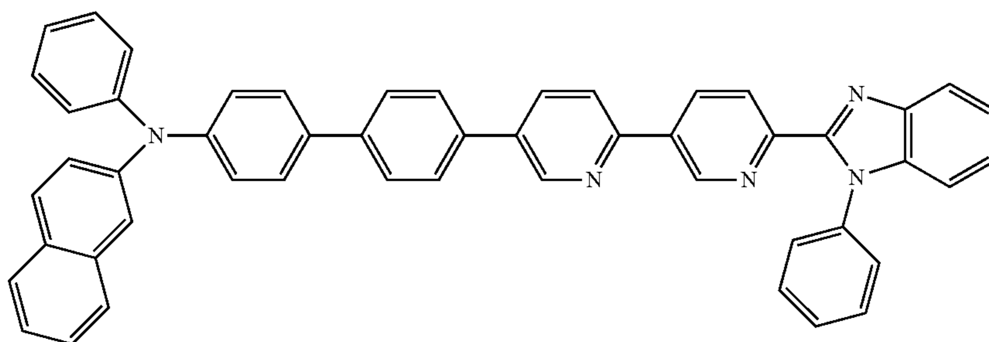
N-phenyl-N-(4'-(6'-(1-phenyl-1H-benzo[d]imidazol-2-yl)-[2,3'-bipyridin]-5-yl)-[1,1'-biphenyl]-4-yl)naphthalen-2-amine,
