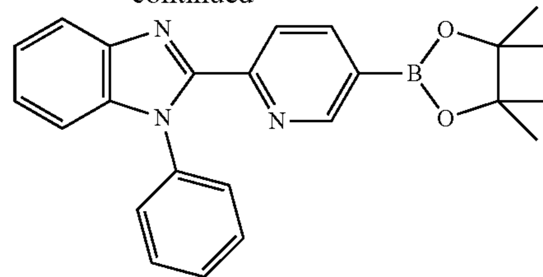
Compound 10
