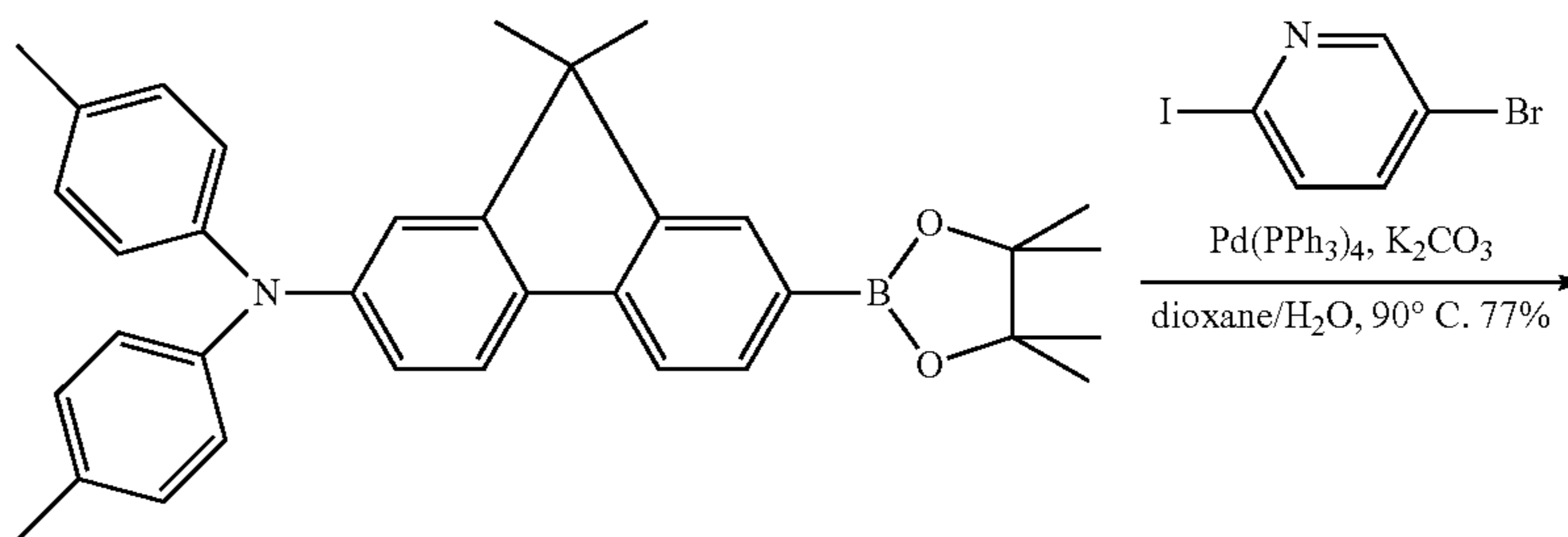
Compound 33
