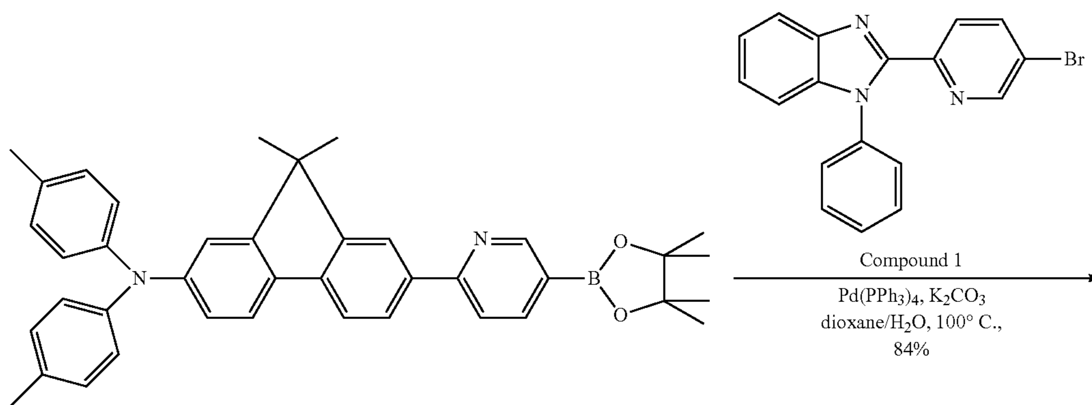
Compound 35
