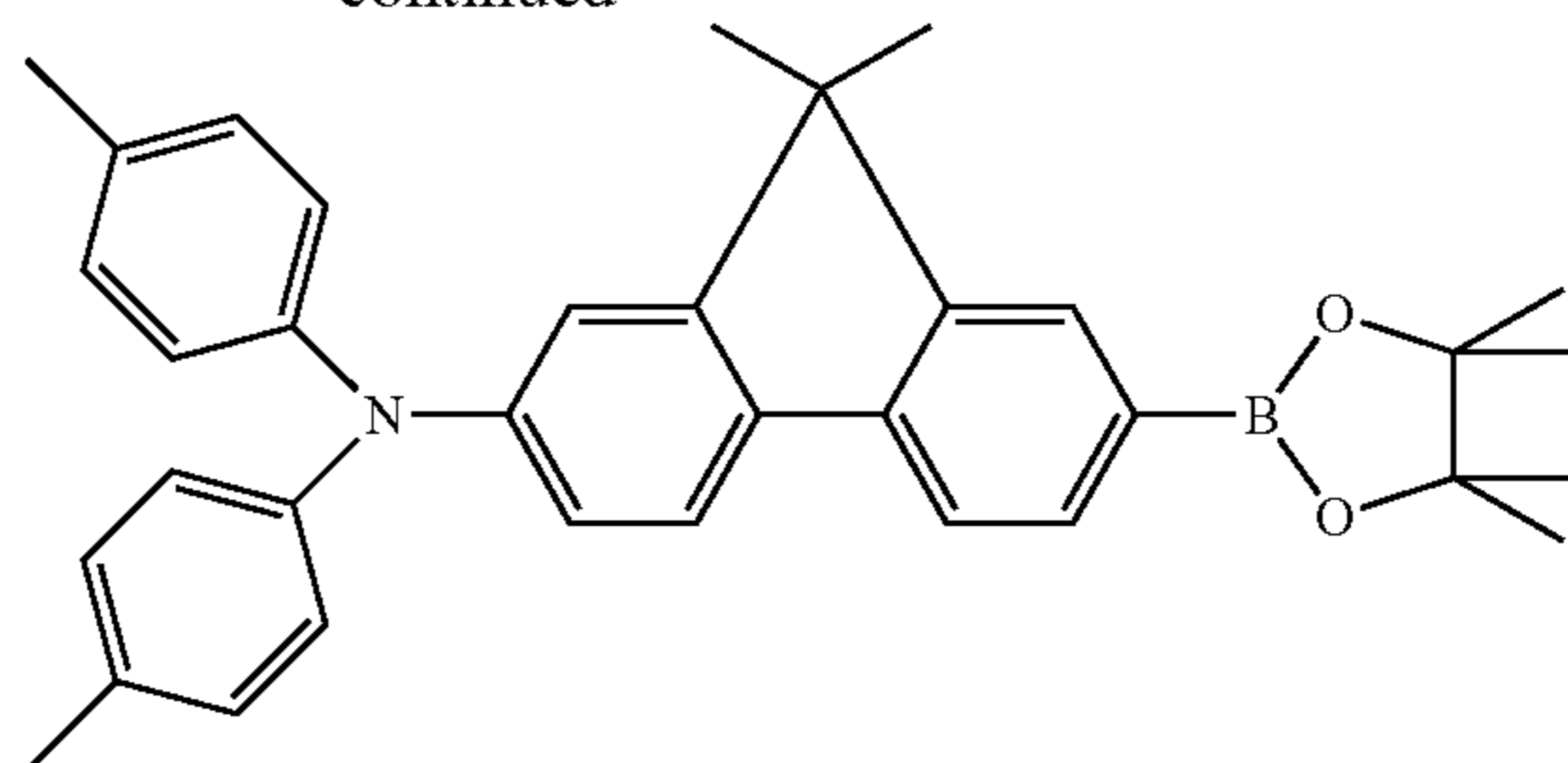
Compound 33
