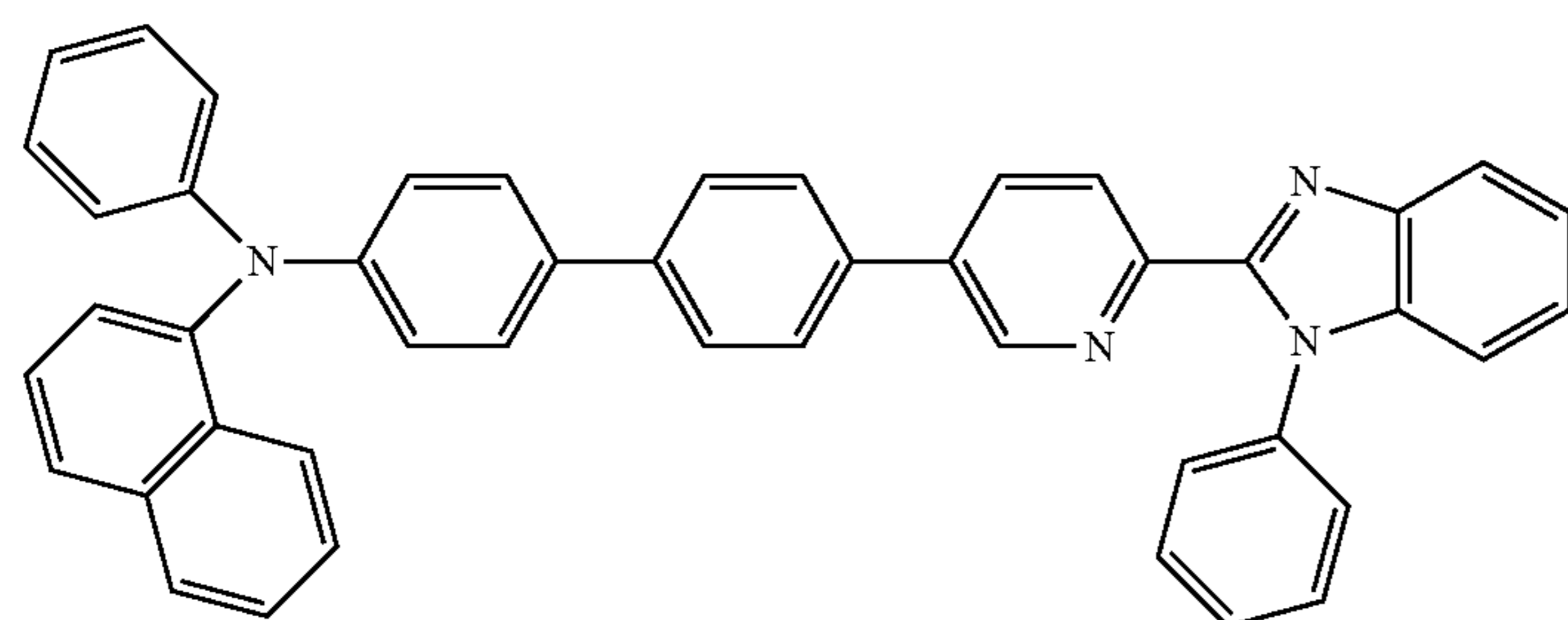
N-phenyl-N-(4'-(6-(1-phenyl-1H-benzo[d]imidazol-2-yl)pyridin-3-yl)-[1,1'-biphenyl]-4-yl)naphth-1-amine,
