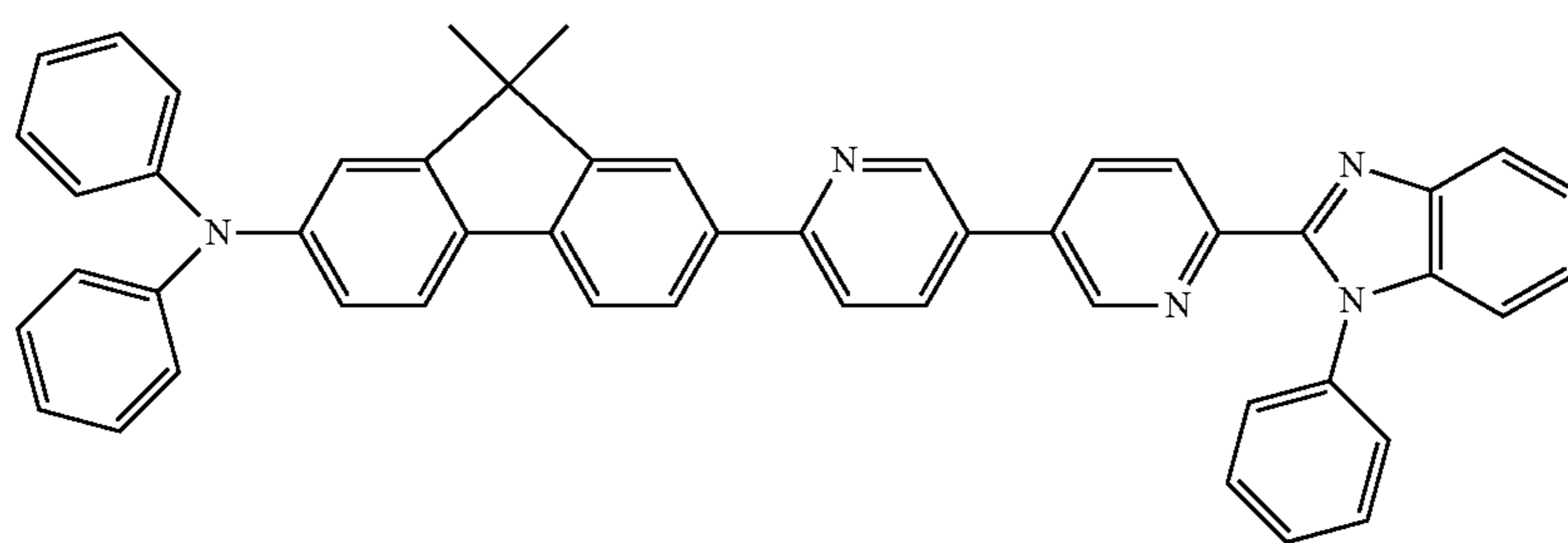
9,9-dimethyl-N,N-diphenyl-7-(6'-(1-phenyl-1H-benzo[d]imidazol-2-yl)-[3,3'-bipyridin]-6-yl)-9H-fluoren-2-amine,
