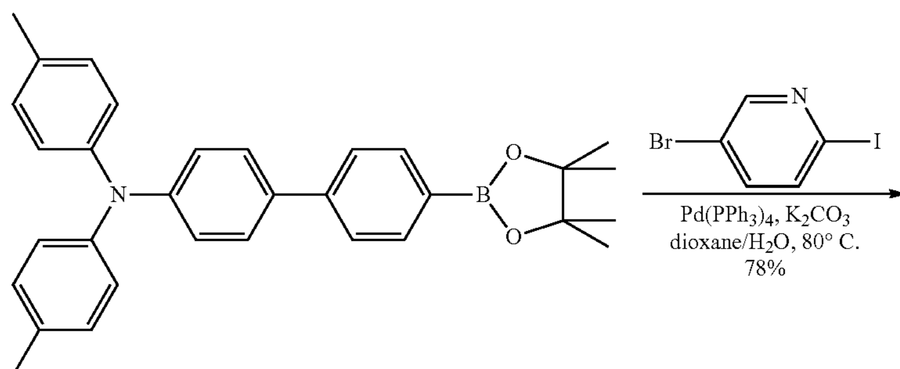
Compound 3
