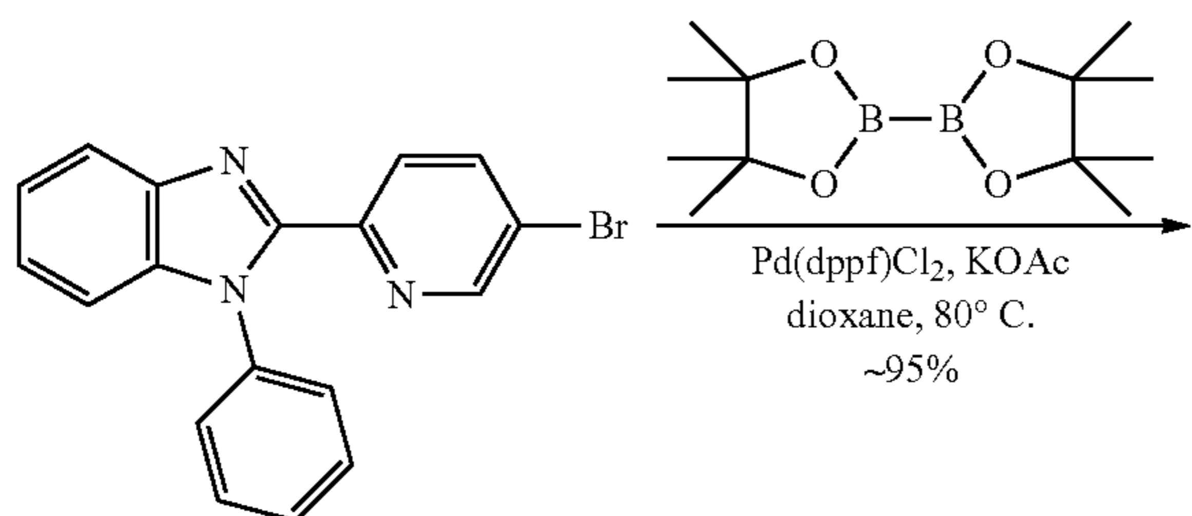
Compound 1
