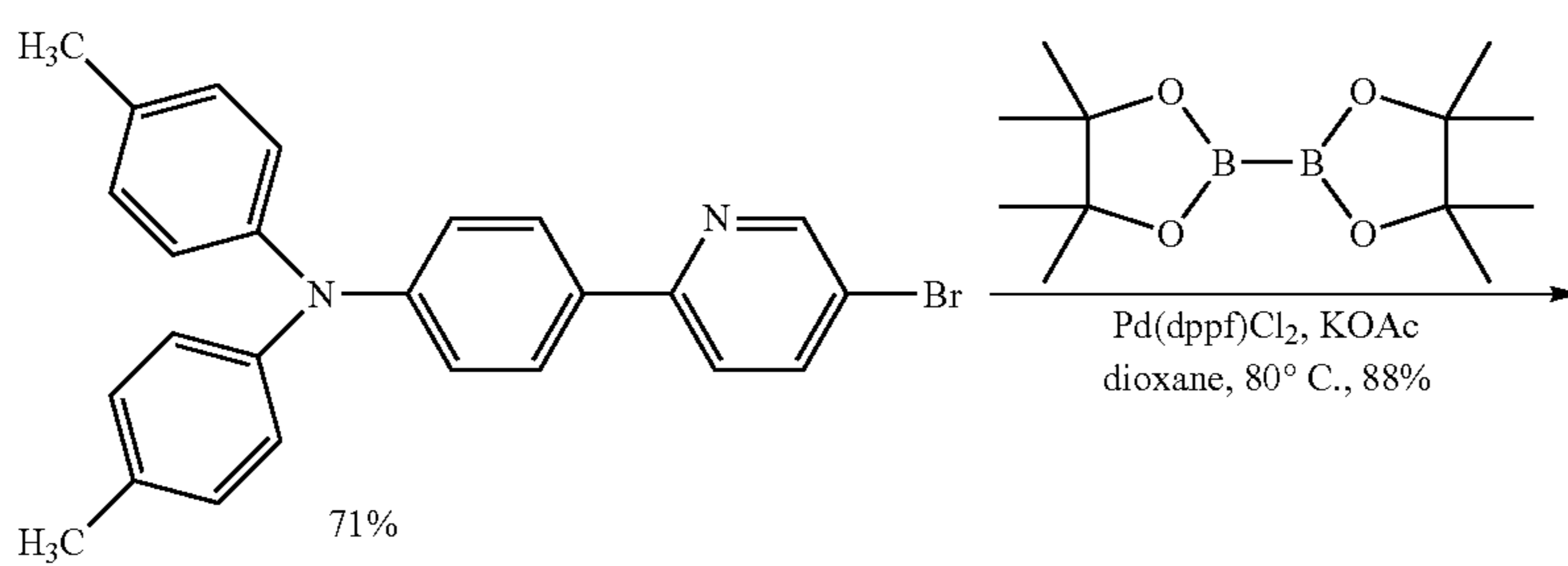
Compound 27
