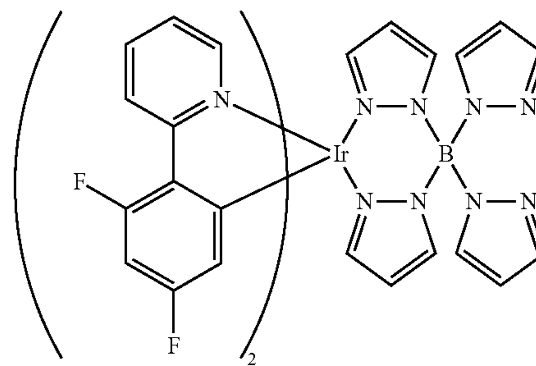
bis[2-(4,6-difluorophenyl)pyridinato-N,C 2' ]iridium(III)tetra(1-pyrazolyl)borate (Fir6)
