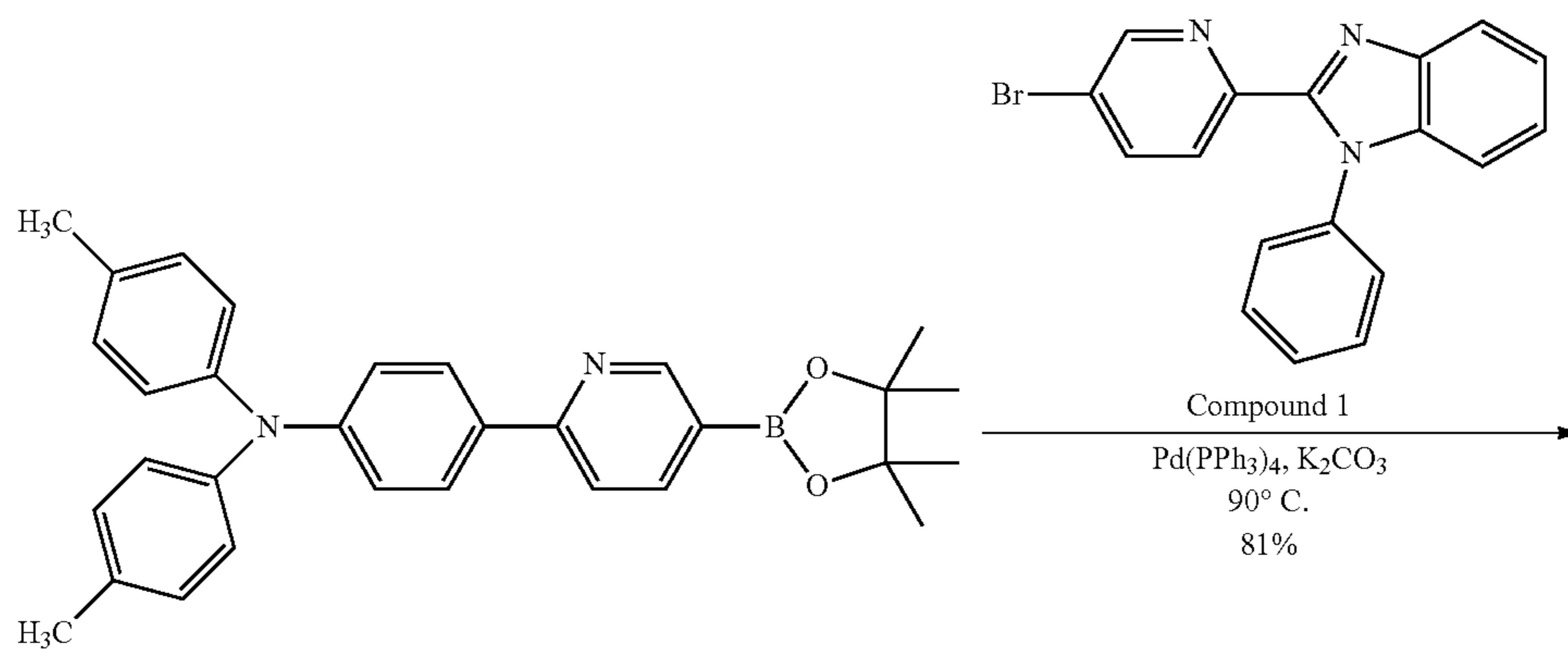
Compound 28
