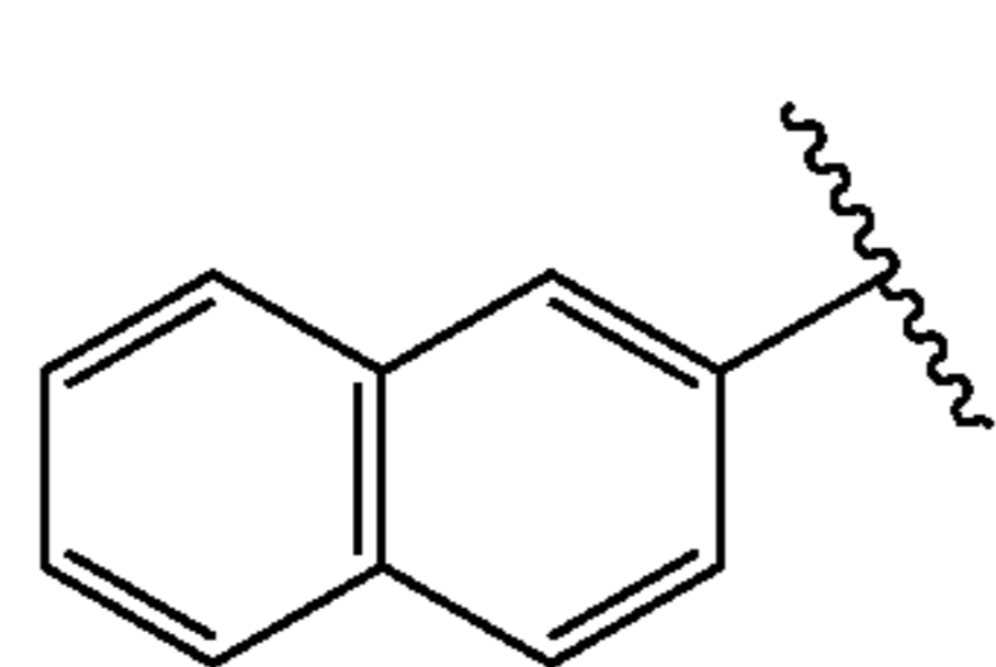
naphth-2-yl
