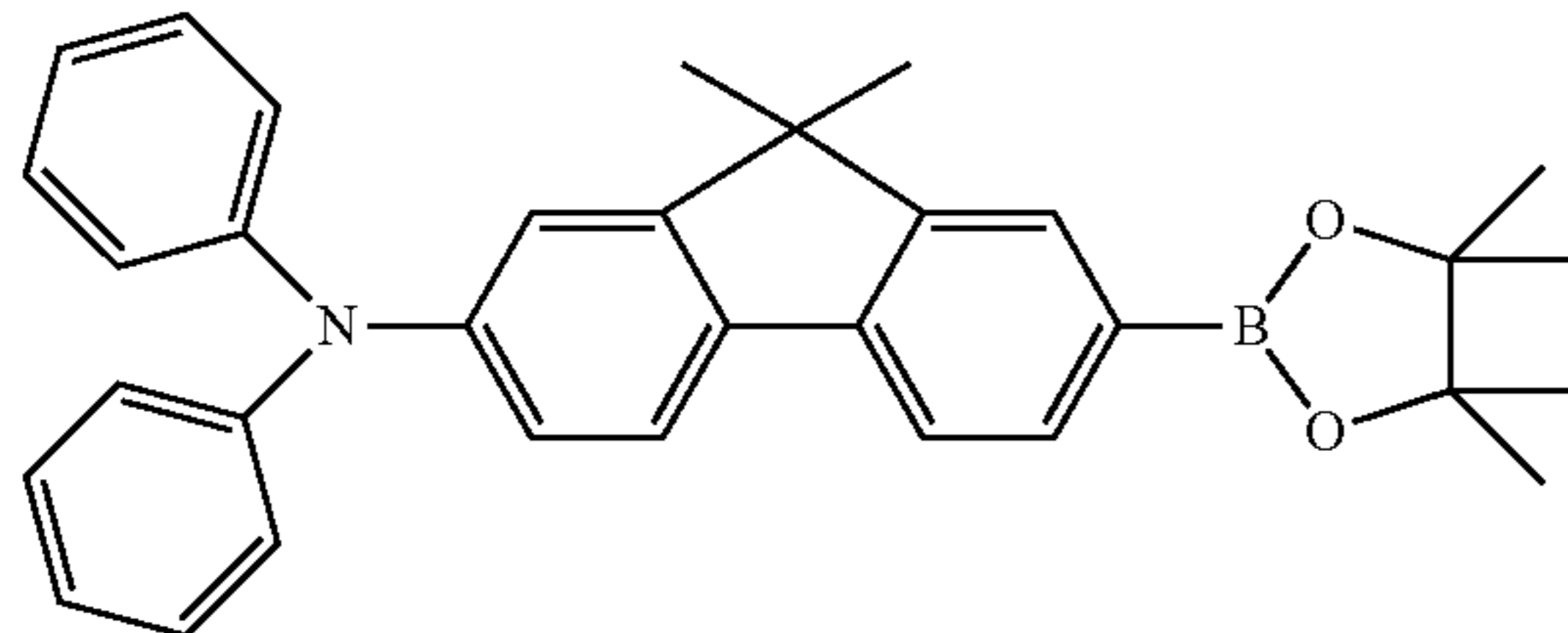
Compound 9
