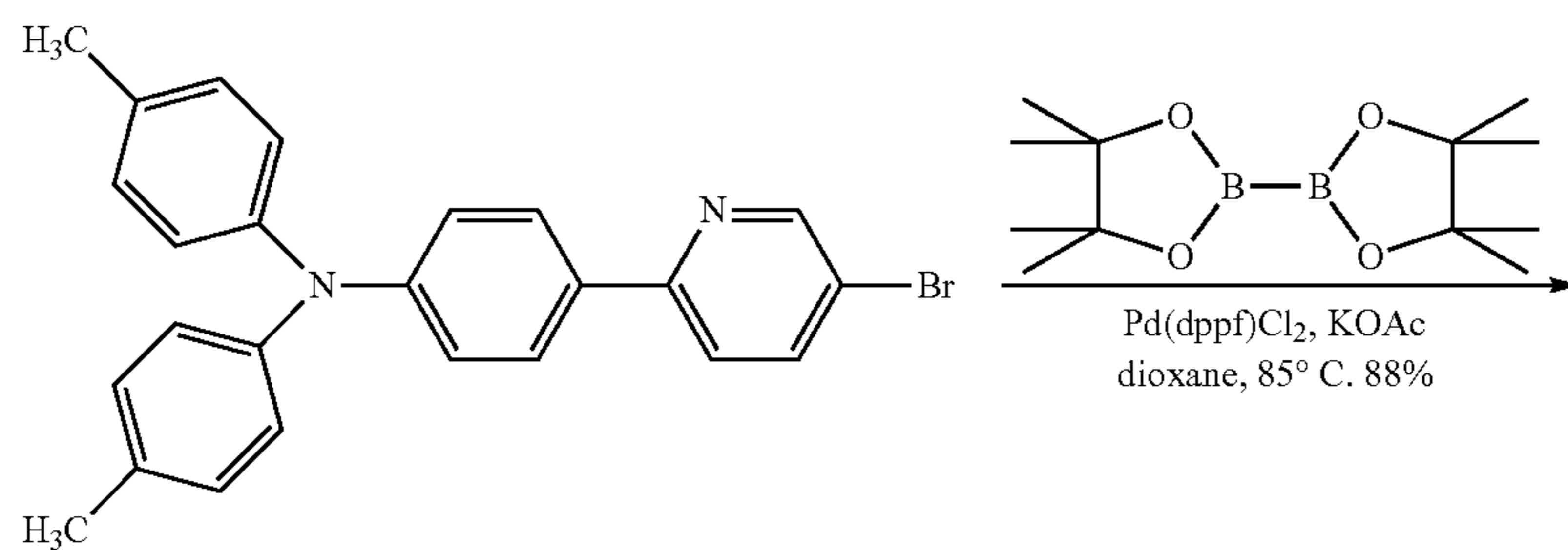
Compound 27
