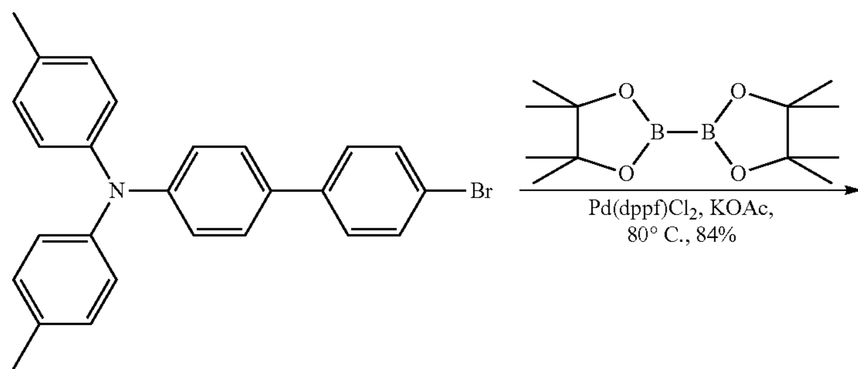
Compound 2
