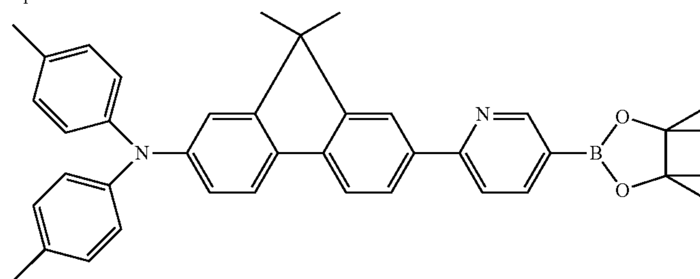
Compound 35
