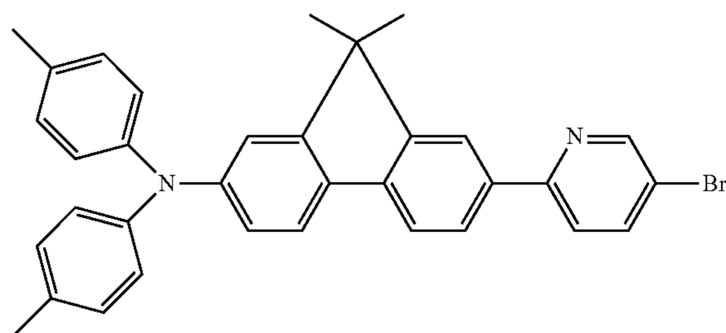
Compound 34
