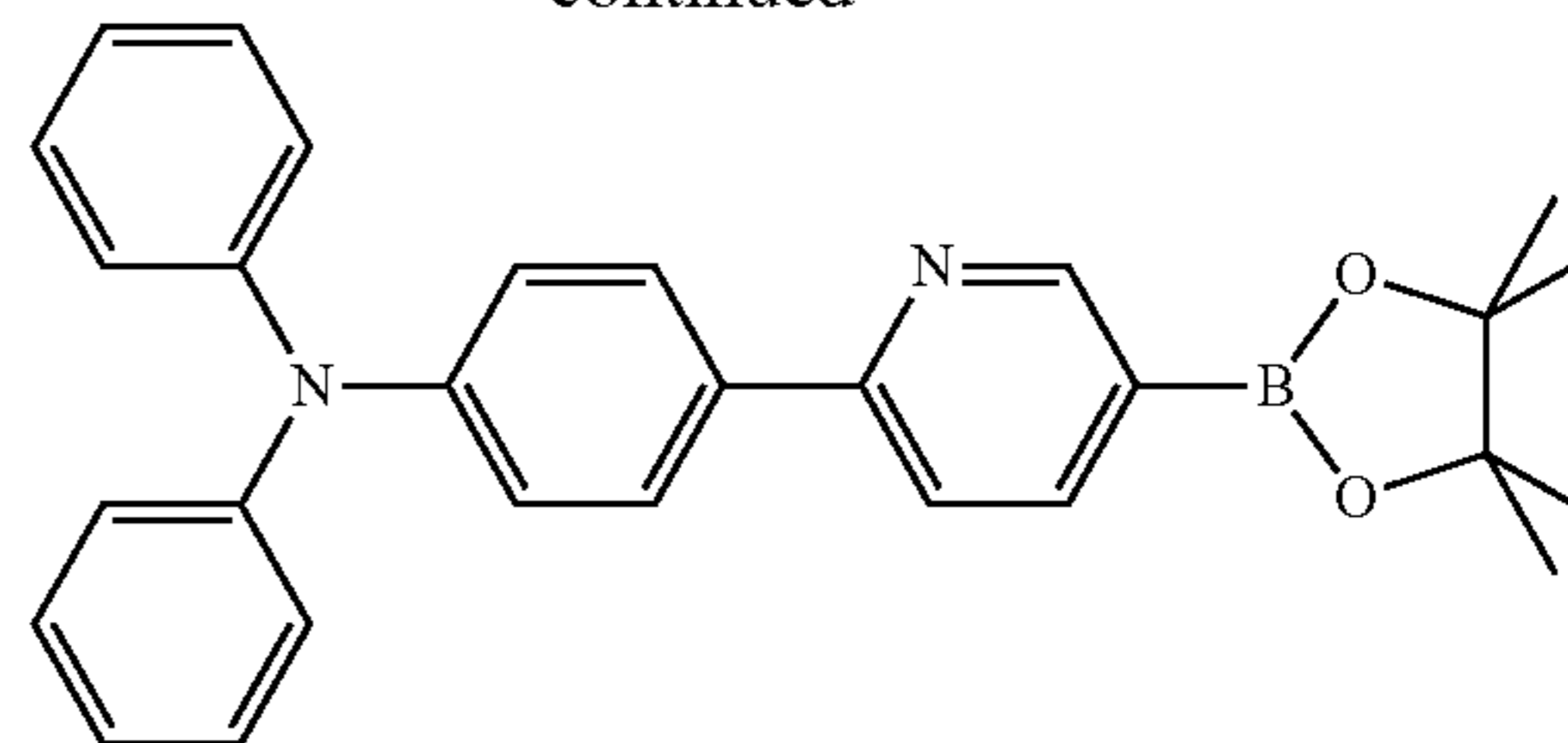
Compound 24
