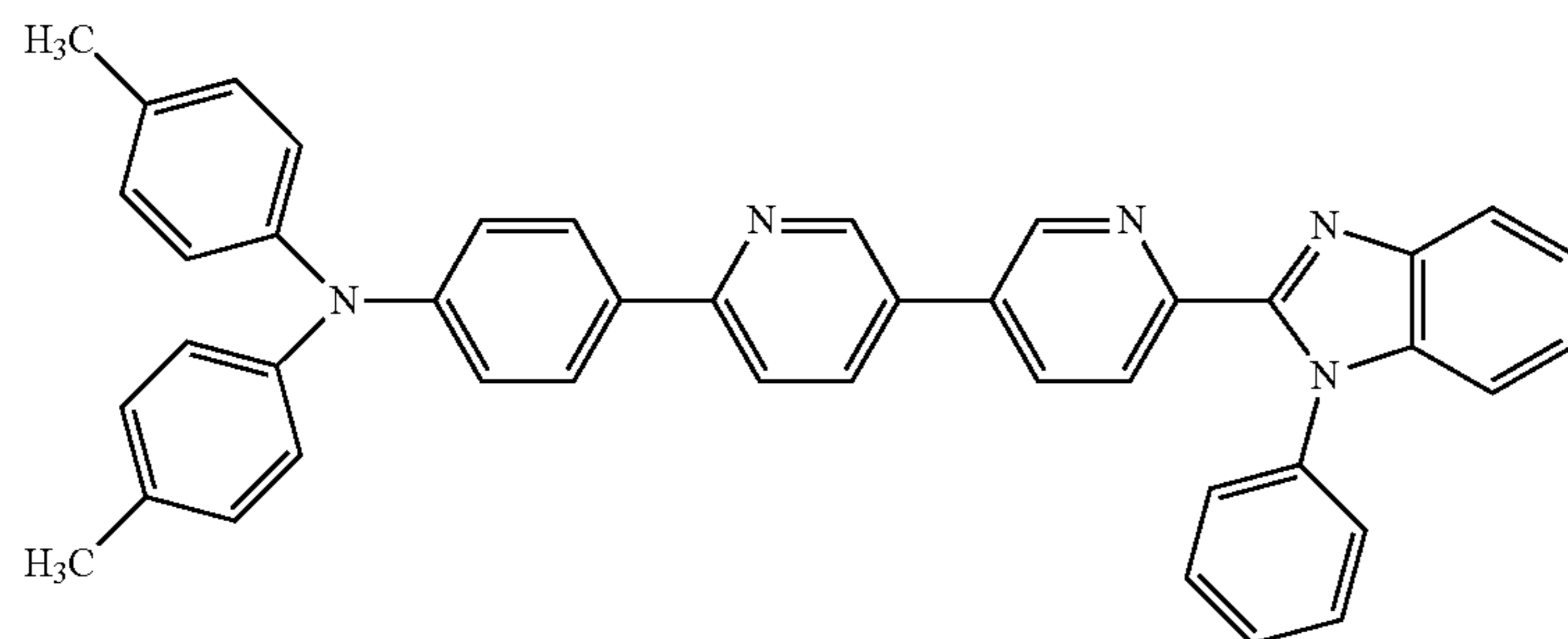
4-methyl-N-(4-(6'-(1-phenyl-1H-benzo[d]imidazol-2-yl)-[3,3'-bipyridin]-6-yl)phenyl)-N-(p-tolyl)aniline,
