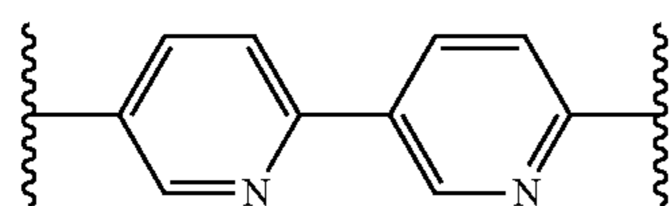
2,3'-bipyridinyl
