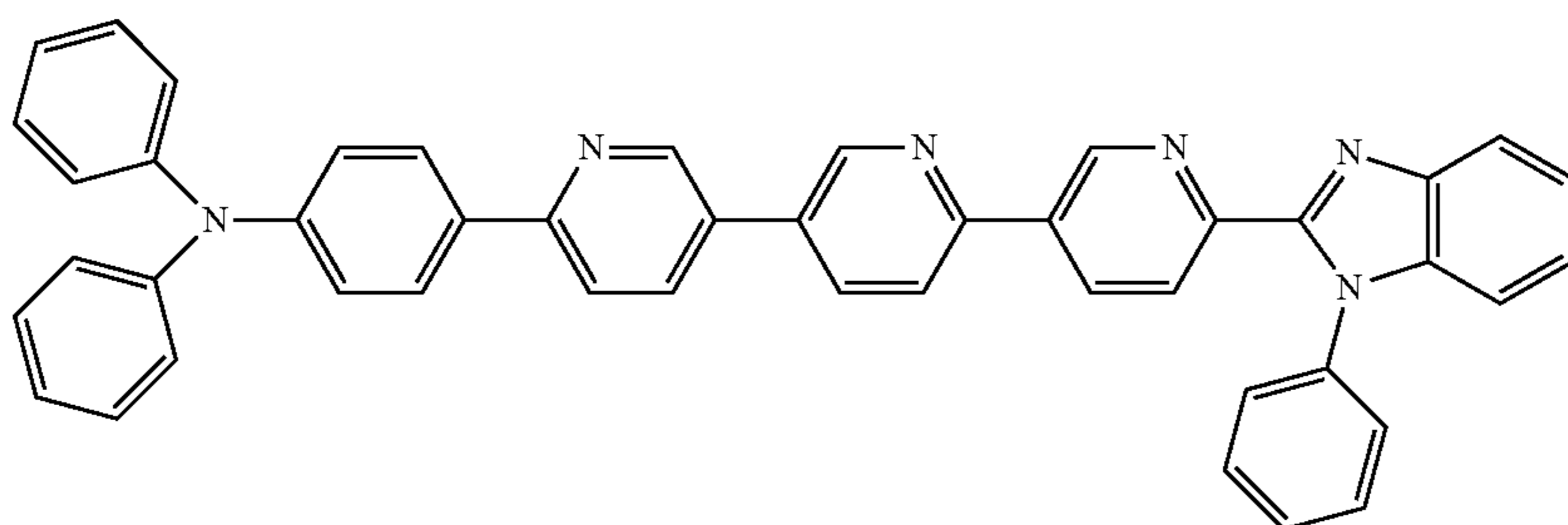
N,N-diphenyl-4-(6-(1-phenyl-1H-benzo[d]imidazol-2-yl)-[3,2':5',3''-terpyridin]-6''-yl)aniline,
