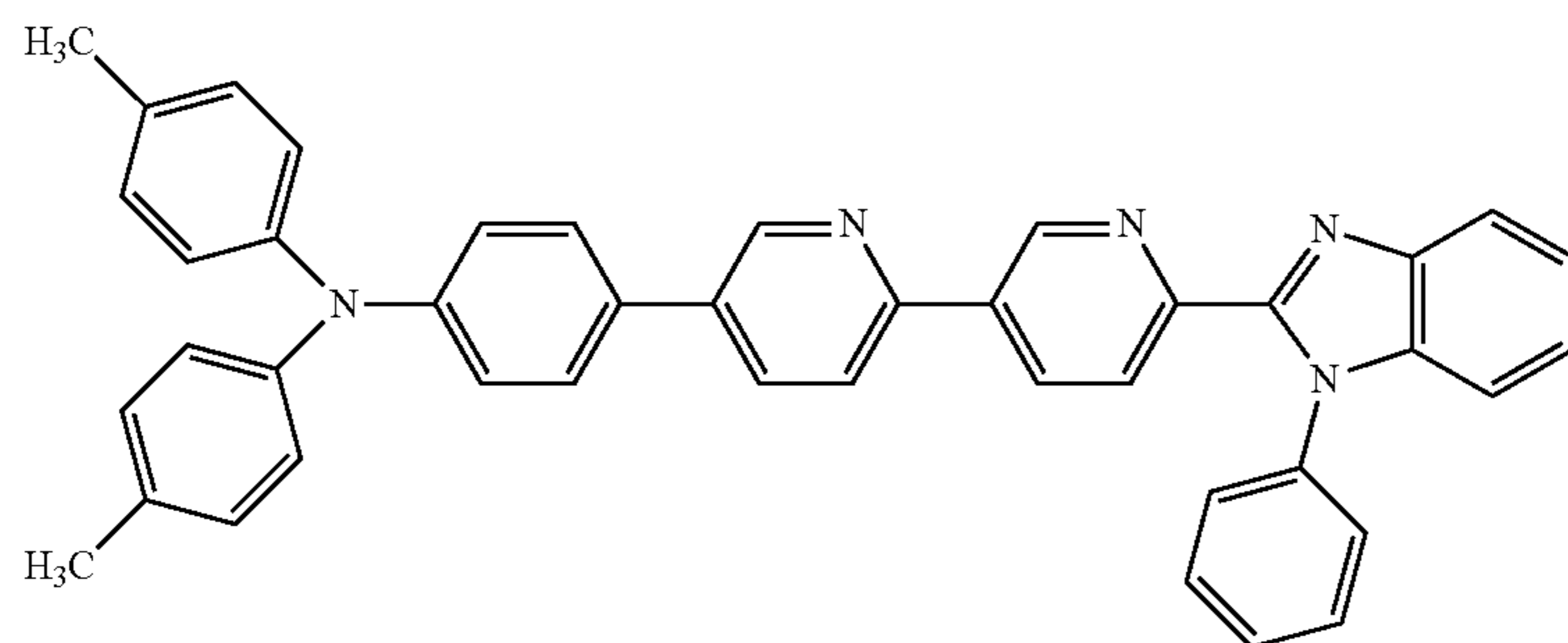
4-methyl-N-(4-(6'-(1-phenyl-1H-benzo[d]imidazol-2-yl)-[2,3'-bipyridin]-5-yl)phenyl)-N-(p-tolyl)aniline,
