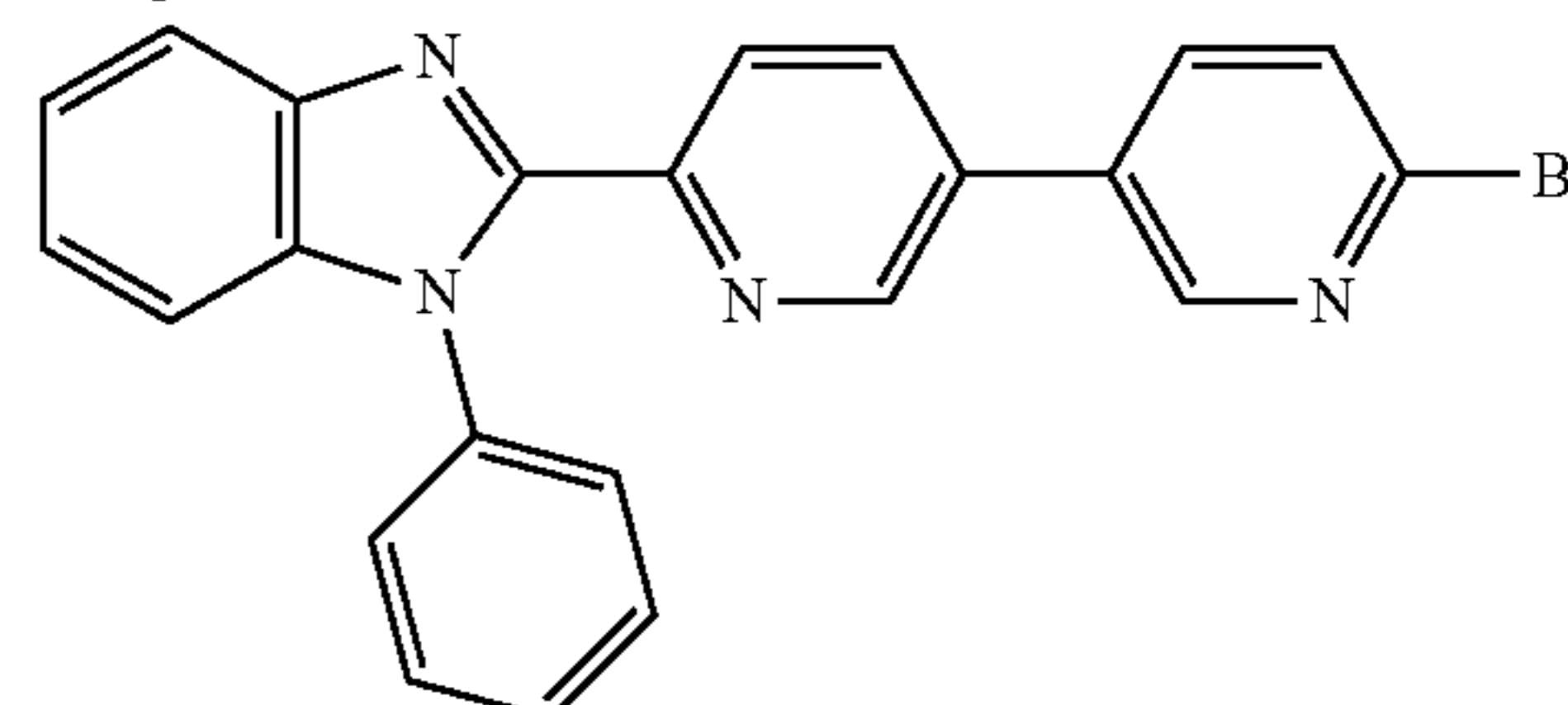
Compound 11
