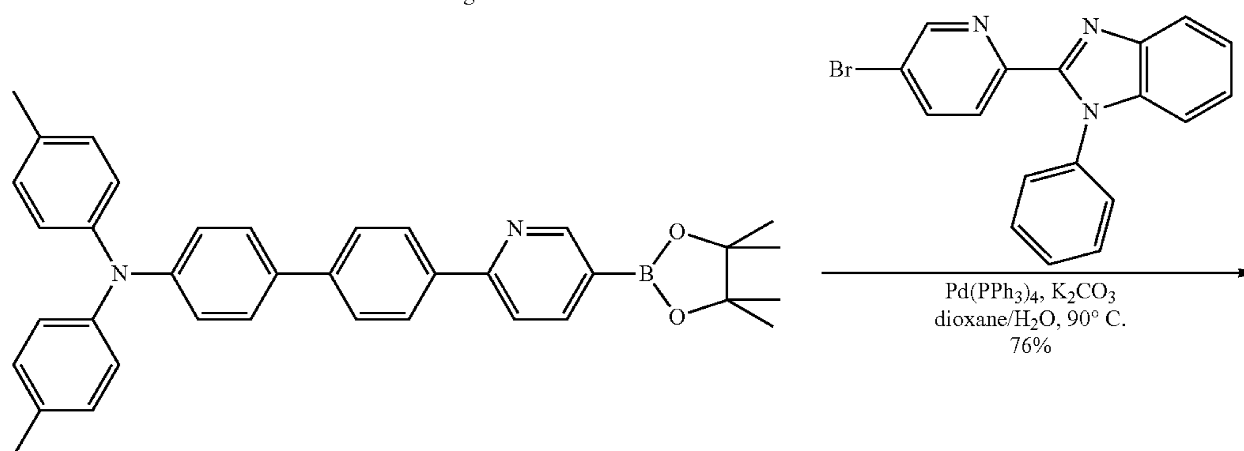
Compound 7
