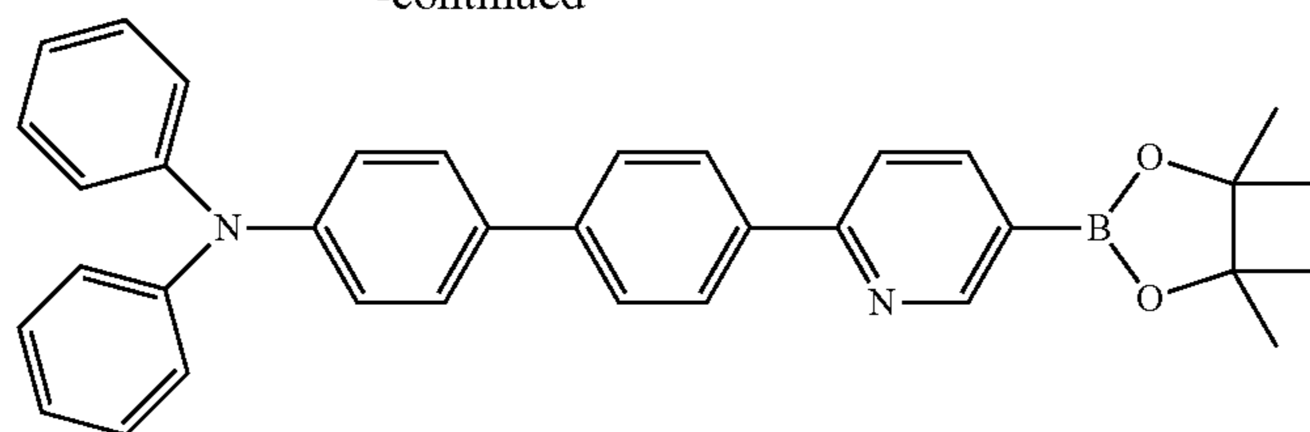
Compound 15
