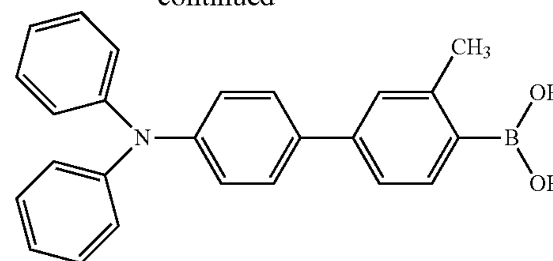
Compound 19 Molecular Weight: 414.34
