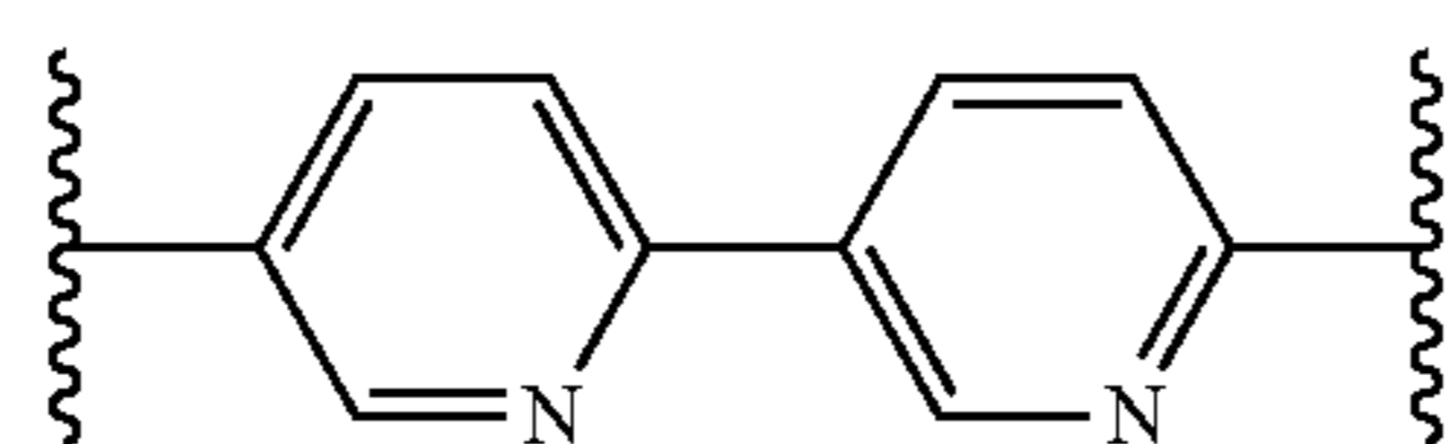
3,3'-bipyridinyl
