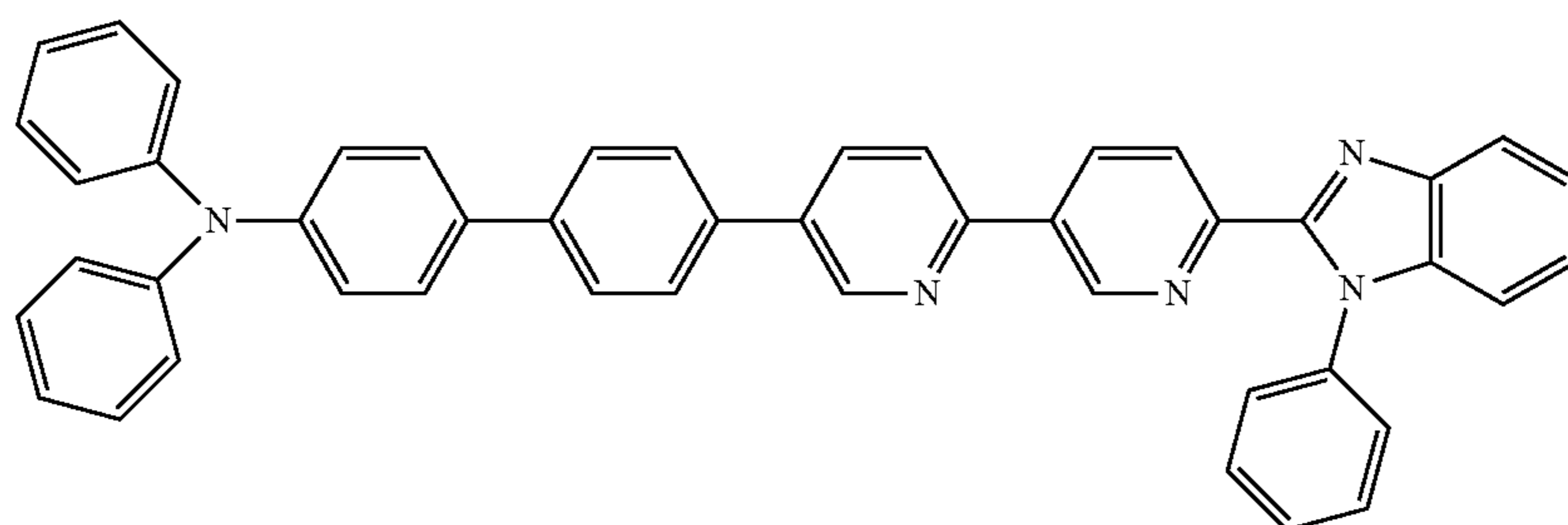
N,N-diphenyl-4'-(6'-(1-phenyl-1H-benzo[d]imidazol-2-yl)-[2,3'-bipyridin]-5-yl)-[1,1'-biphenyl]-4-amine,
