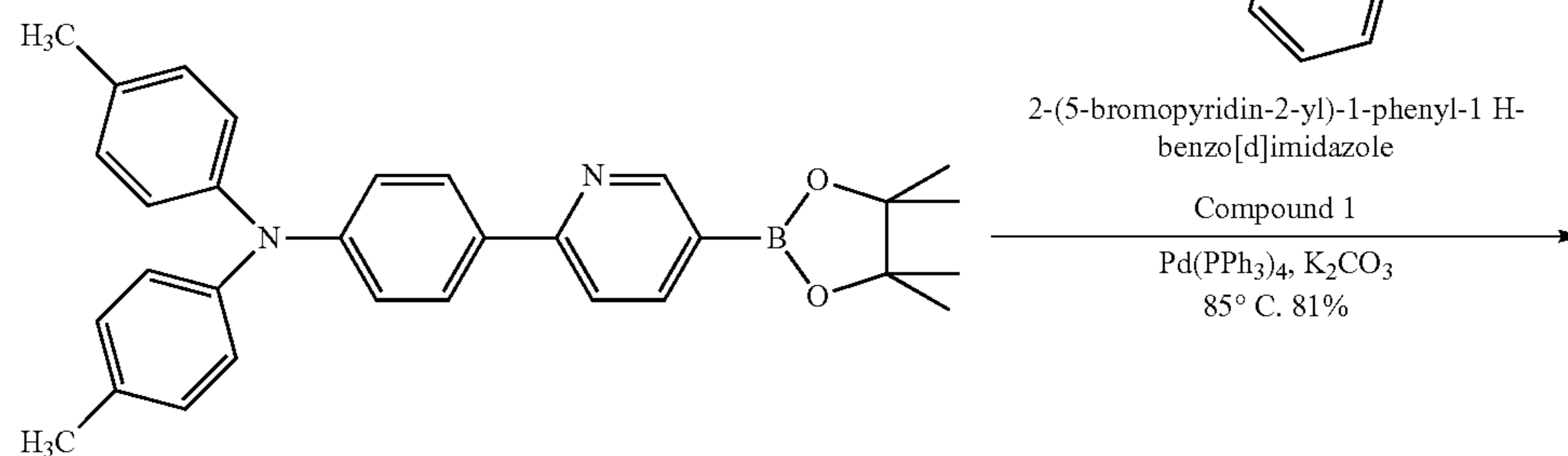
Compound 28
