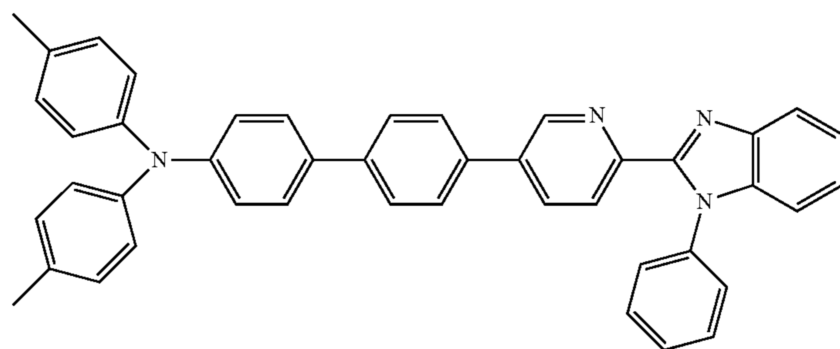
N,N-diphenyl-4-(6-(1-phenyl-1H-benzo[d]imidazol-2-yl)pyridin-3-yl)aniline,
