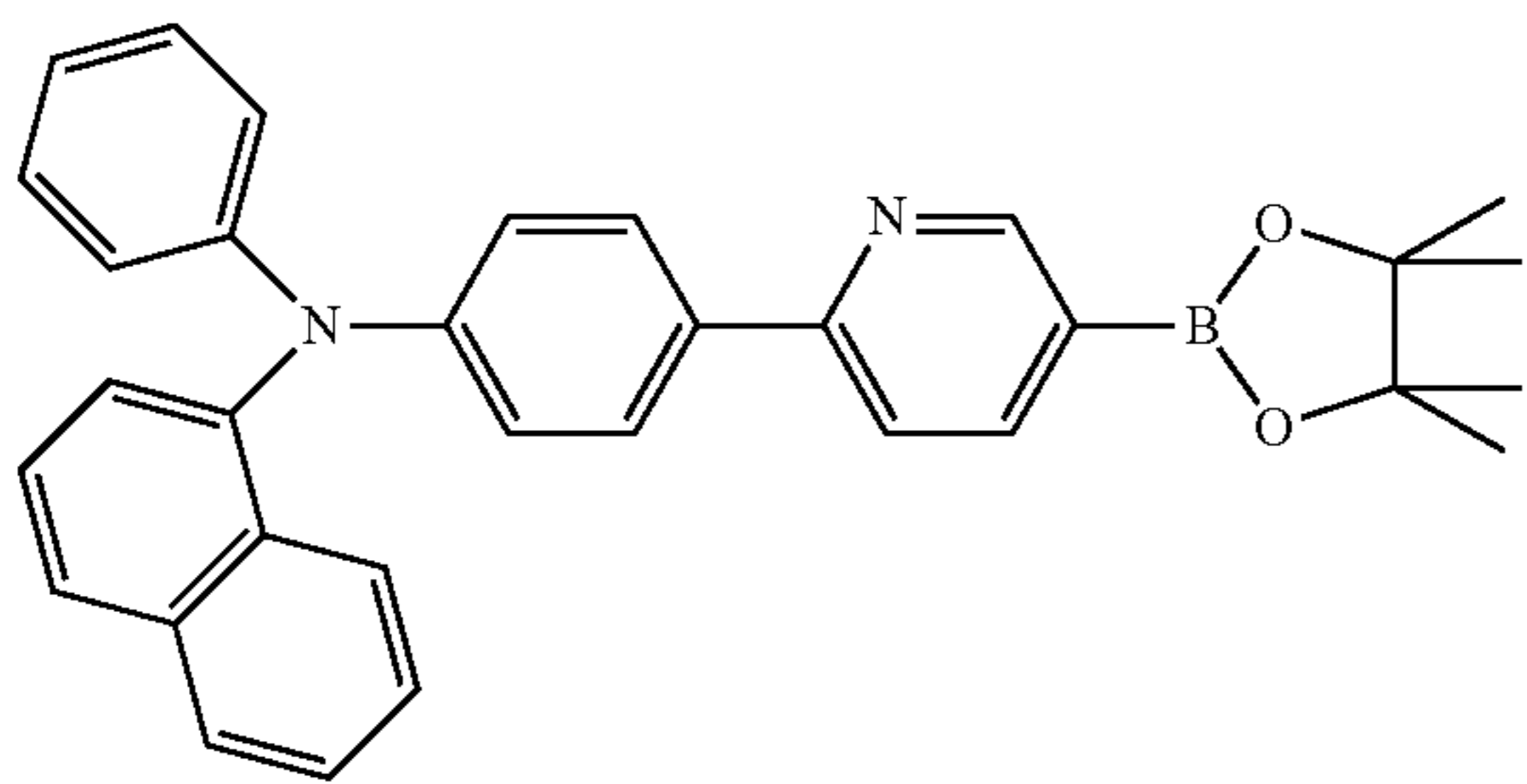
Compound 31
