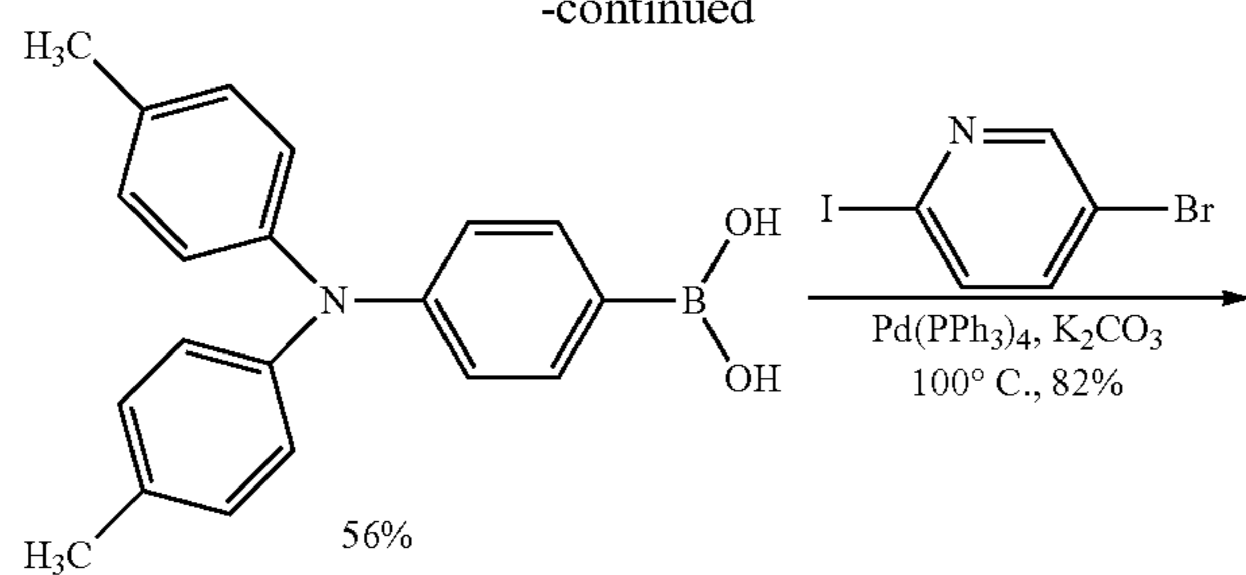
Compound 26
