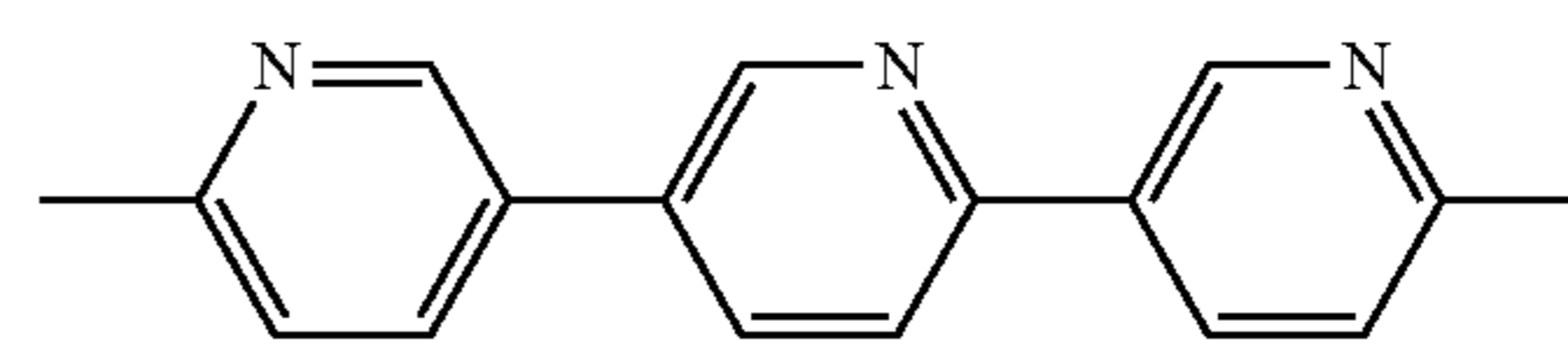
3,2':5', 3''-terpyridinyl
