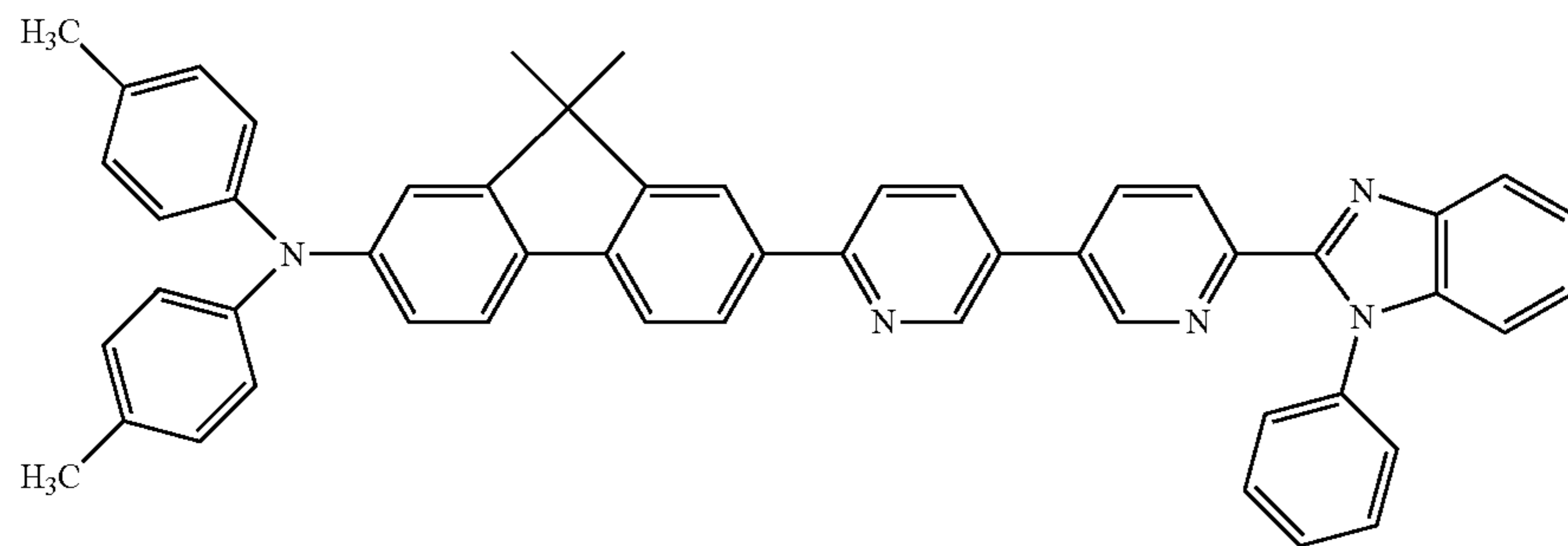
9,9-dimethyl-7-(6'-(1-phenyl-1H-benzo[d]imidazol-2-yl)-[3,3'-bipyridin]-6-yl)-N,N-di-p-tolyl-9H-fluoren-2-amine
