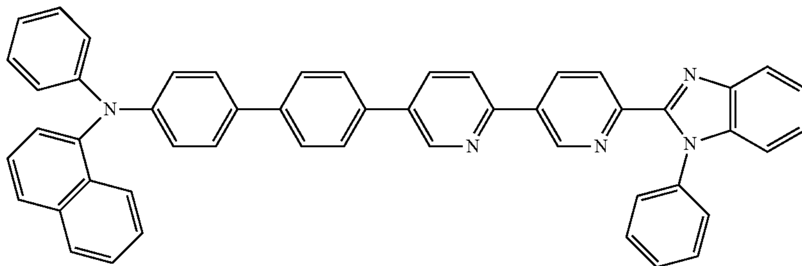
N-phenyl-N-(4'-(6'-(1-phenyl-1H-benzo[d]imidazol-2-yl)-[2,3'-bipyridin]-5-yl)-[1,1'-biphenyl]-4-yl)naphthalen-1-amine,
