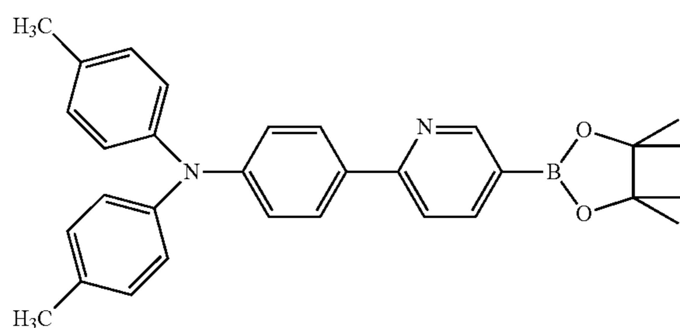
Compound 28
