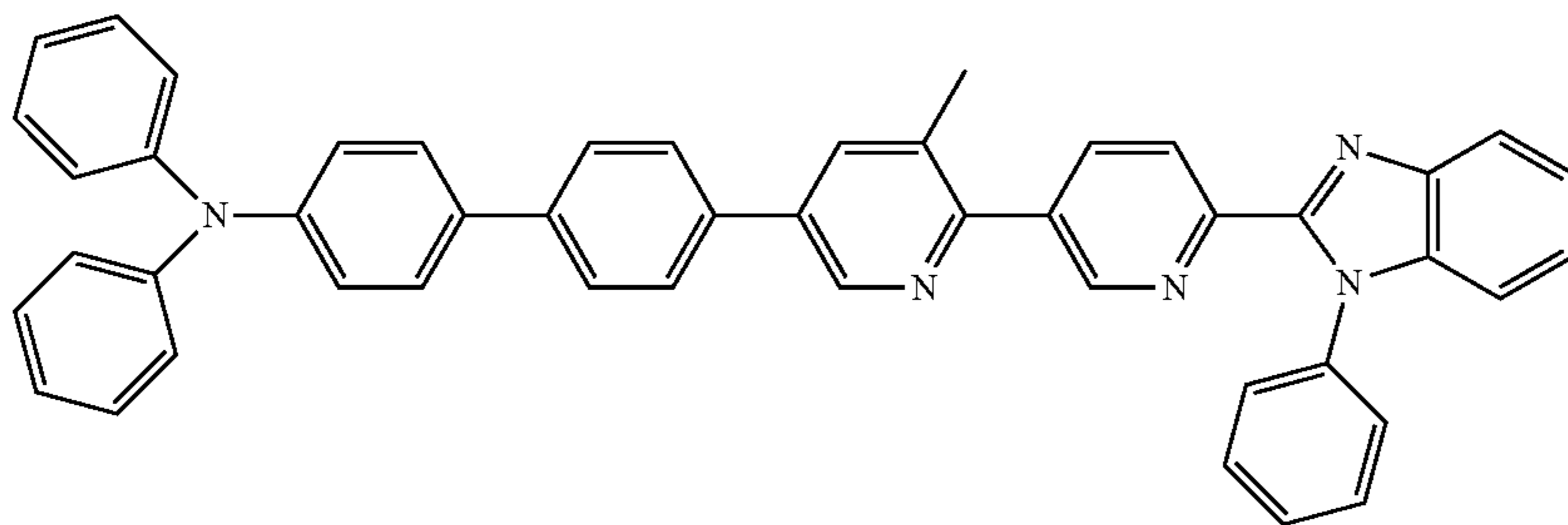
4'-(3-methyl-6'-(1-phenyl-1H-benzo[d]imidazol-2-yl)-[2,3'-bipyridin]-5-yl)-N,N-diphenyl-[1,1'-biphenyl]-4-amine,
