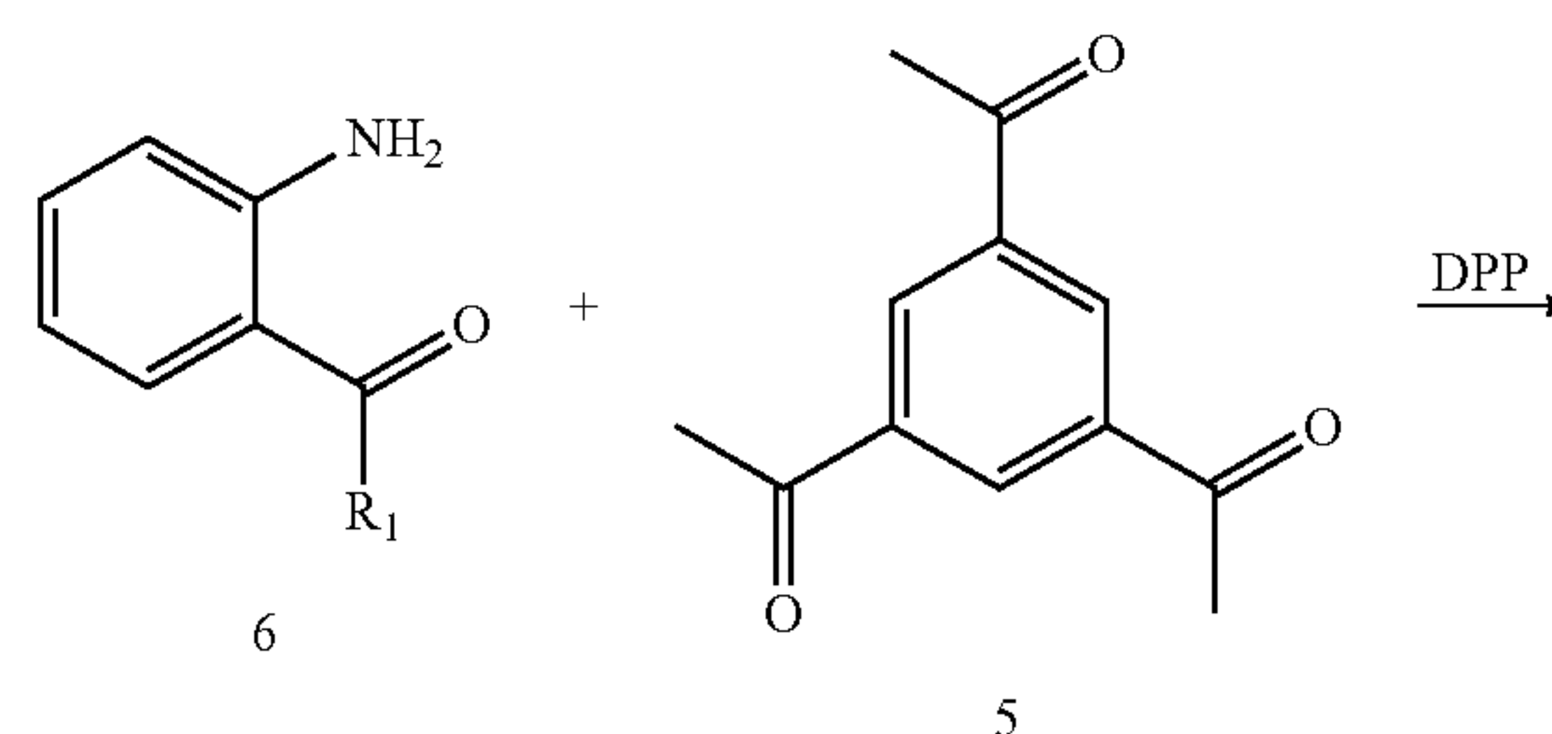
Scheme 2. Synthesis of 2.
