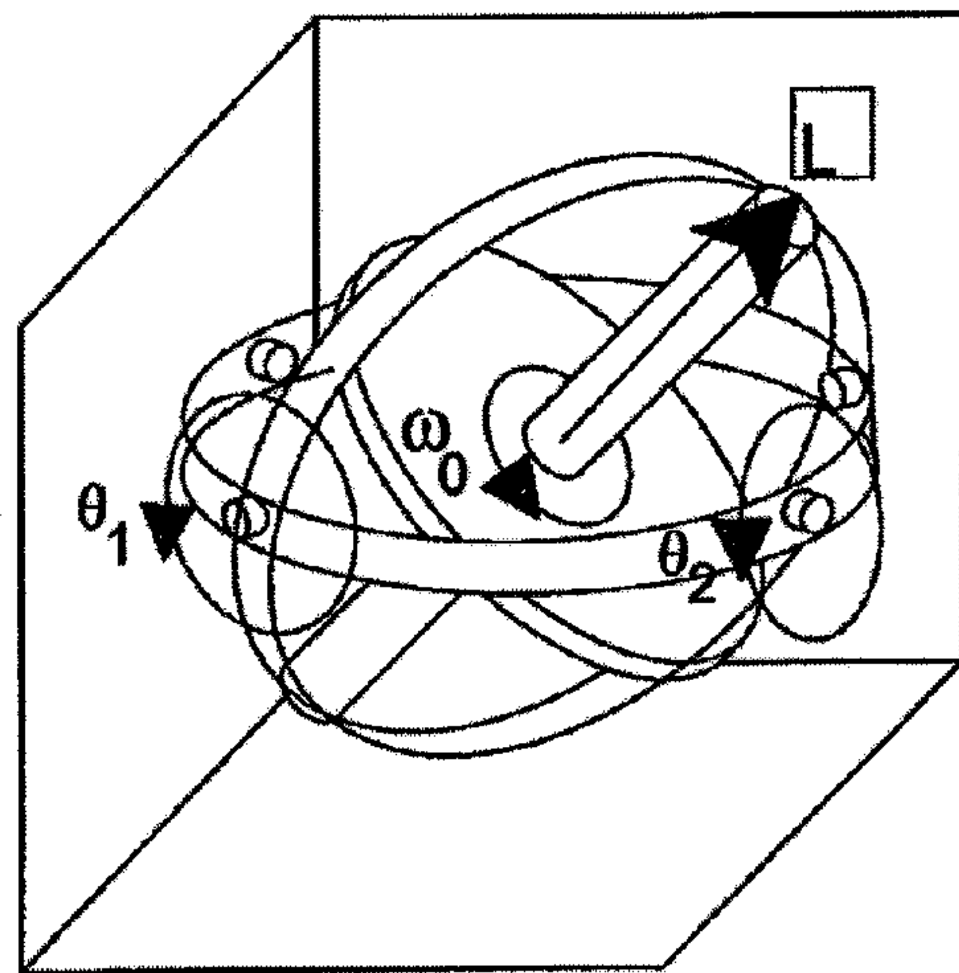
1311 GYROSCOPE TYPE
