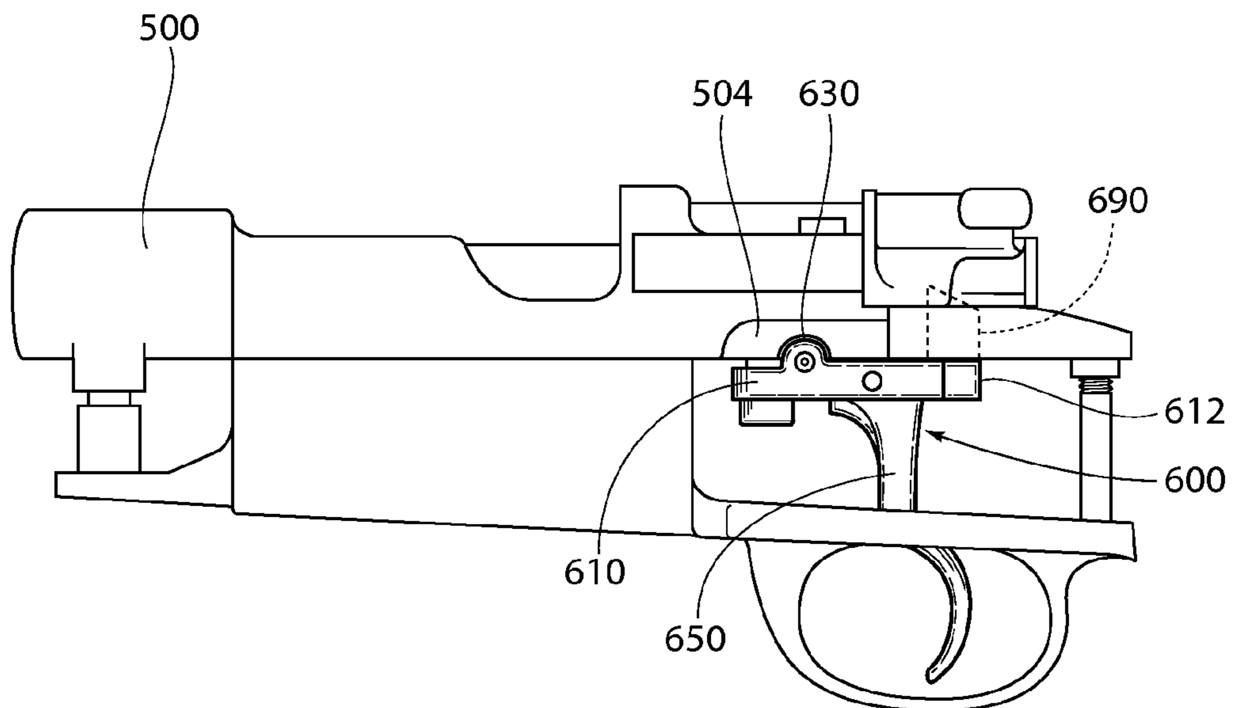
Fig. 4 PRIOR ART
