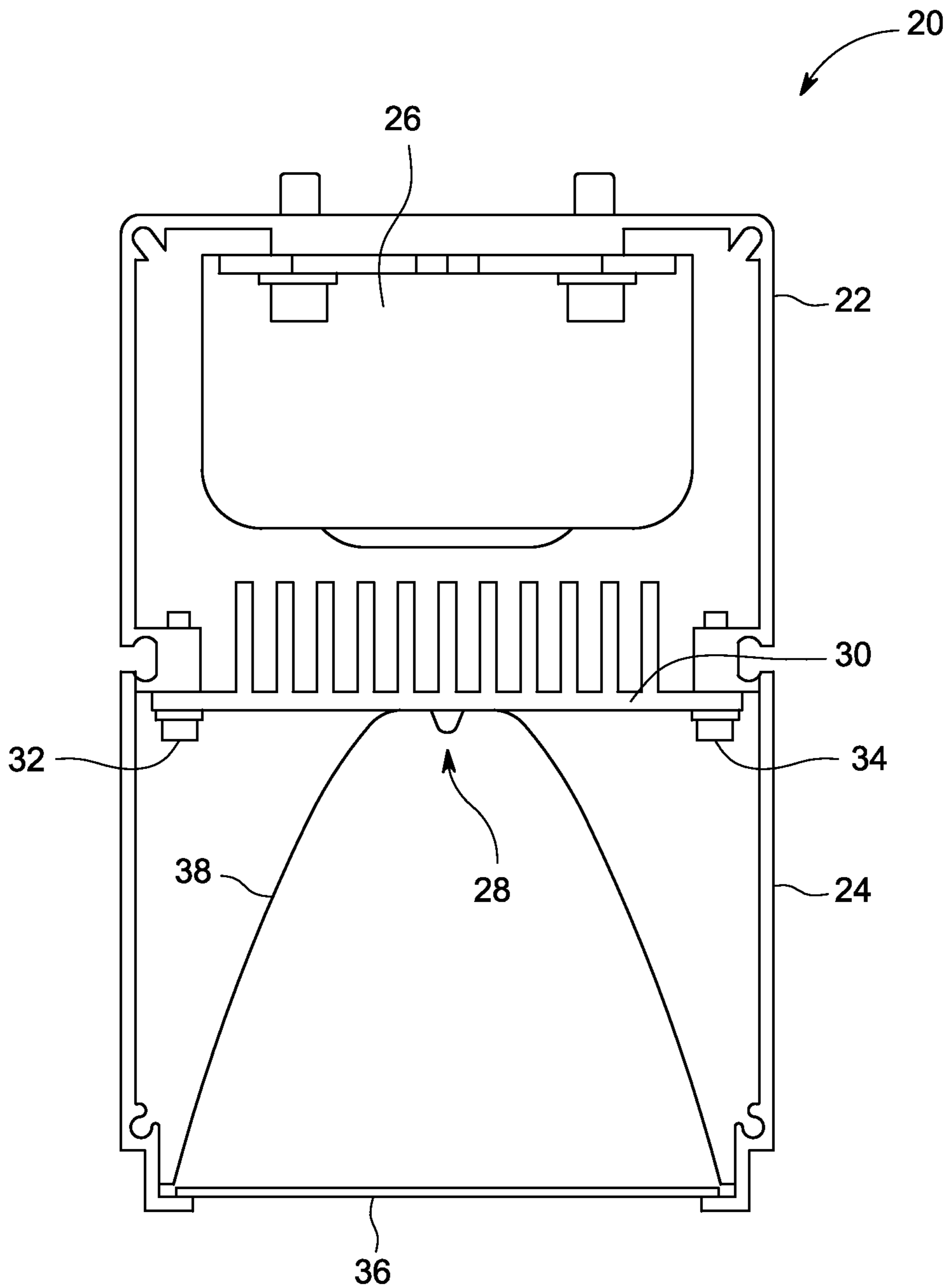
FIG. 2 (PRIOR ART)
