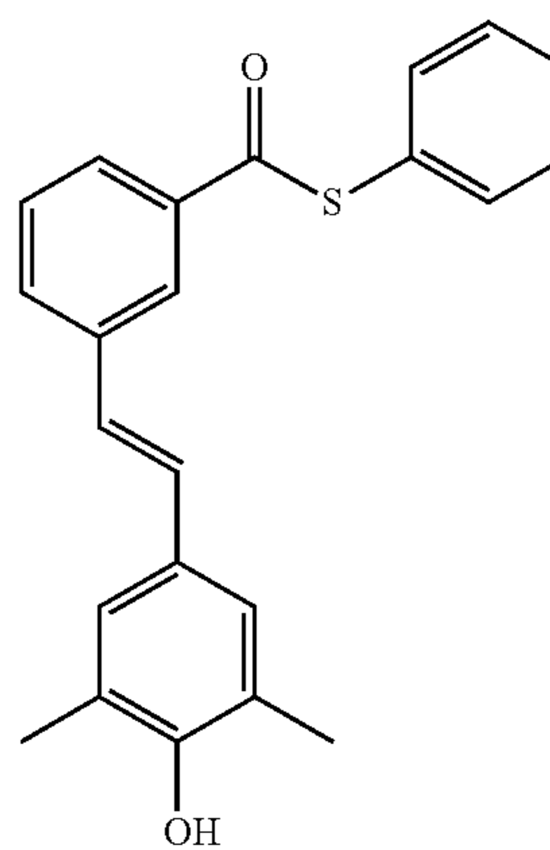
Covalent probe 6
