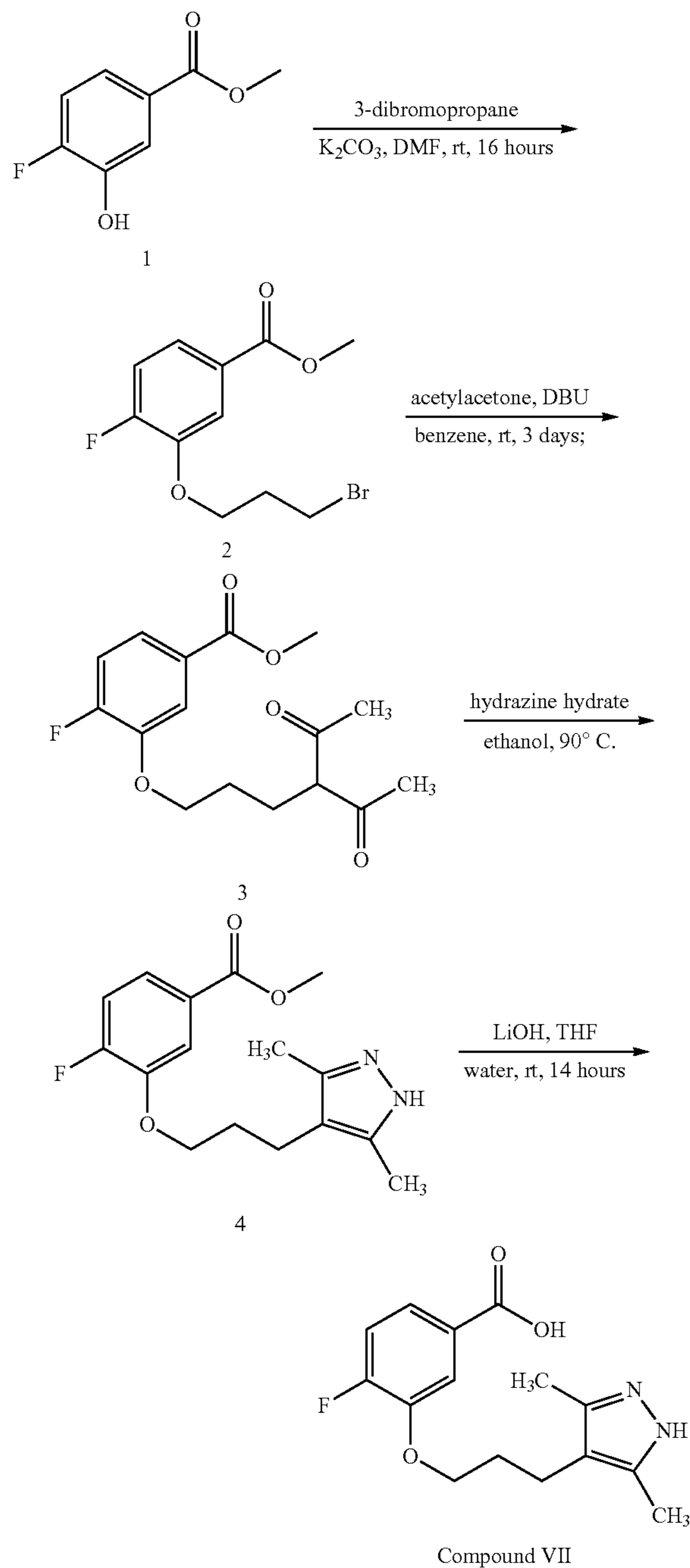
Scheme 1
