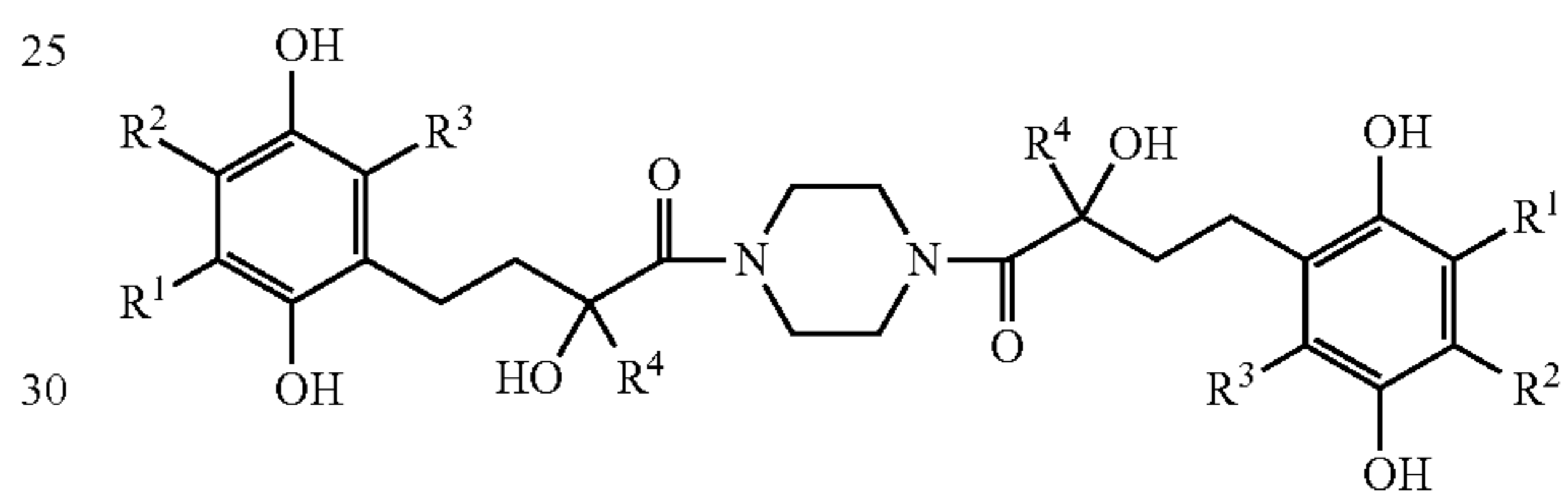
Formula Ibb
