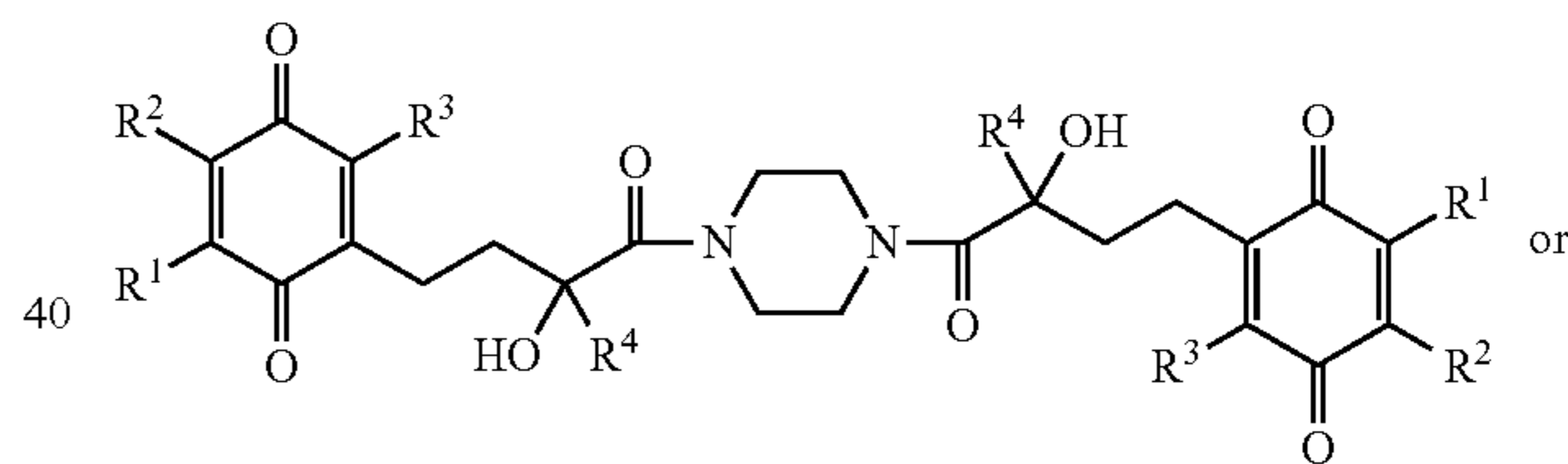
Formula I-Sbb
