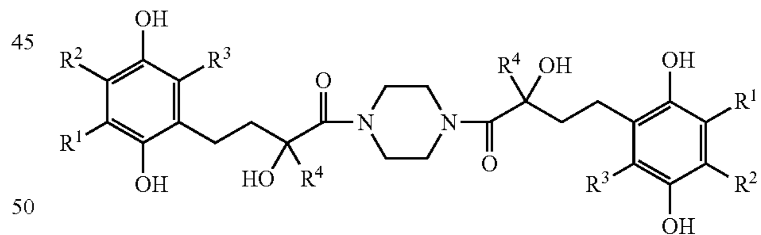
Formula I-S
