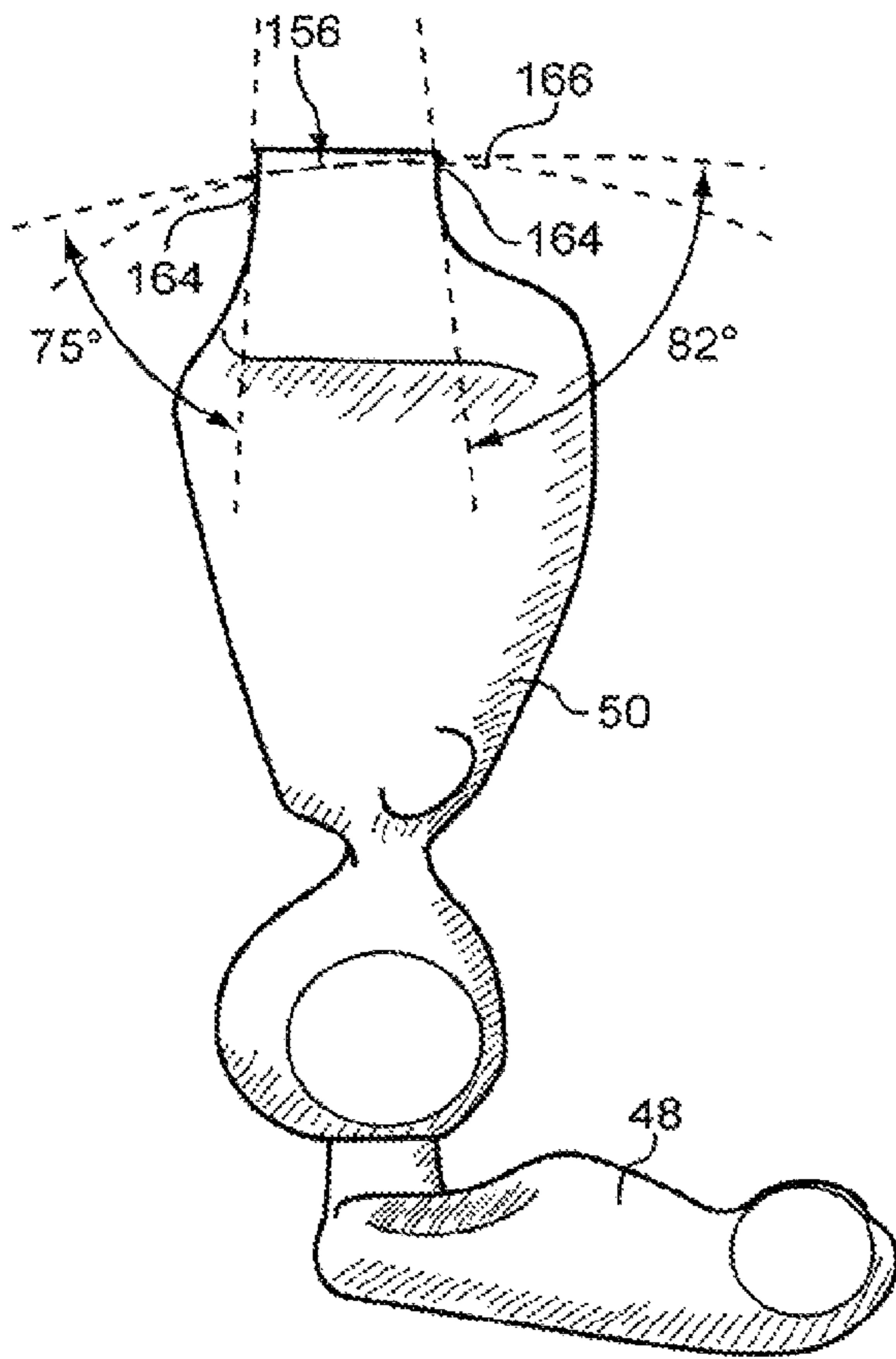
FIG. 26 PRIOR ART
