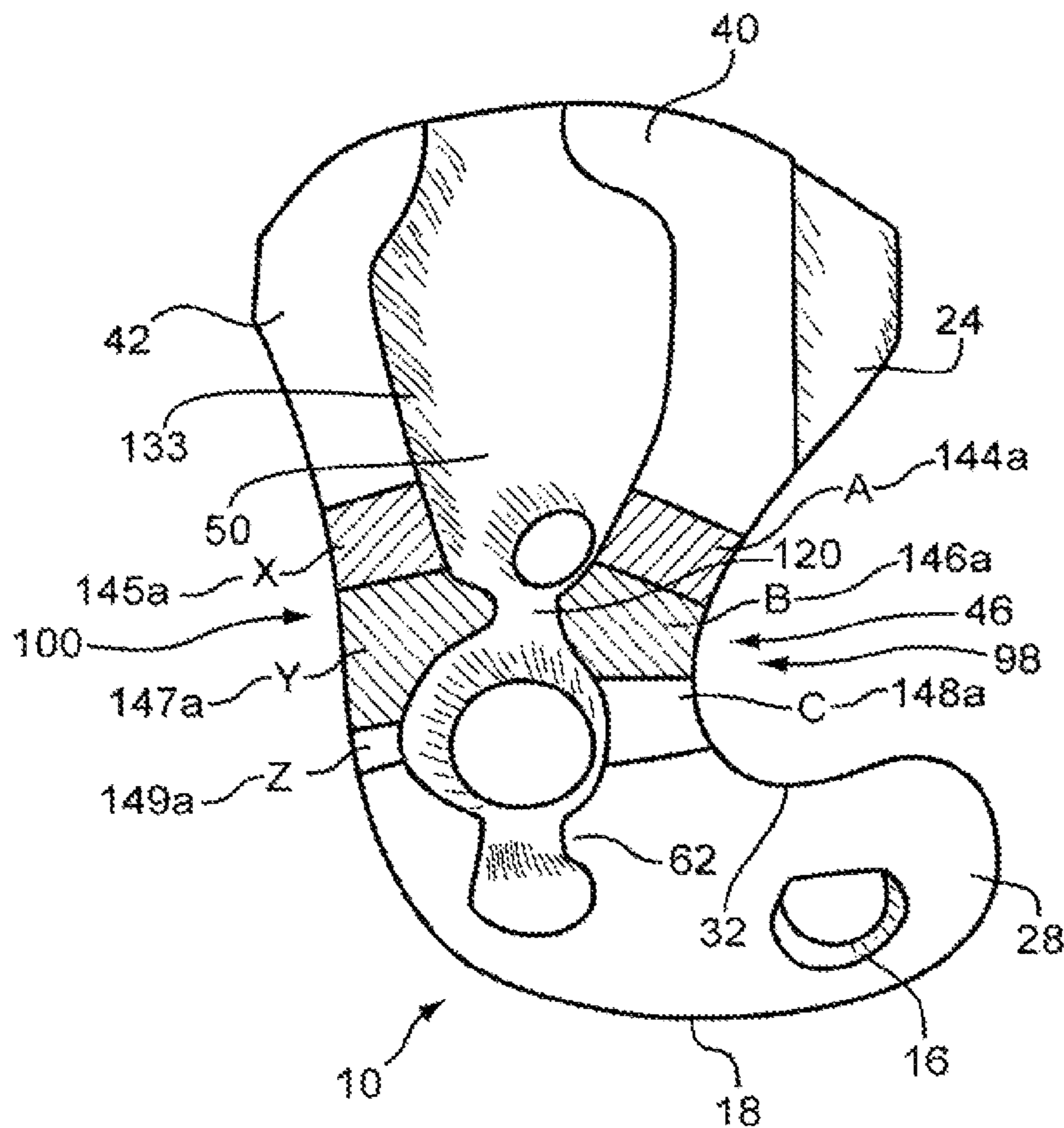
FIG. 16 PRIOR ART
