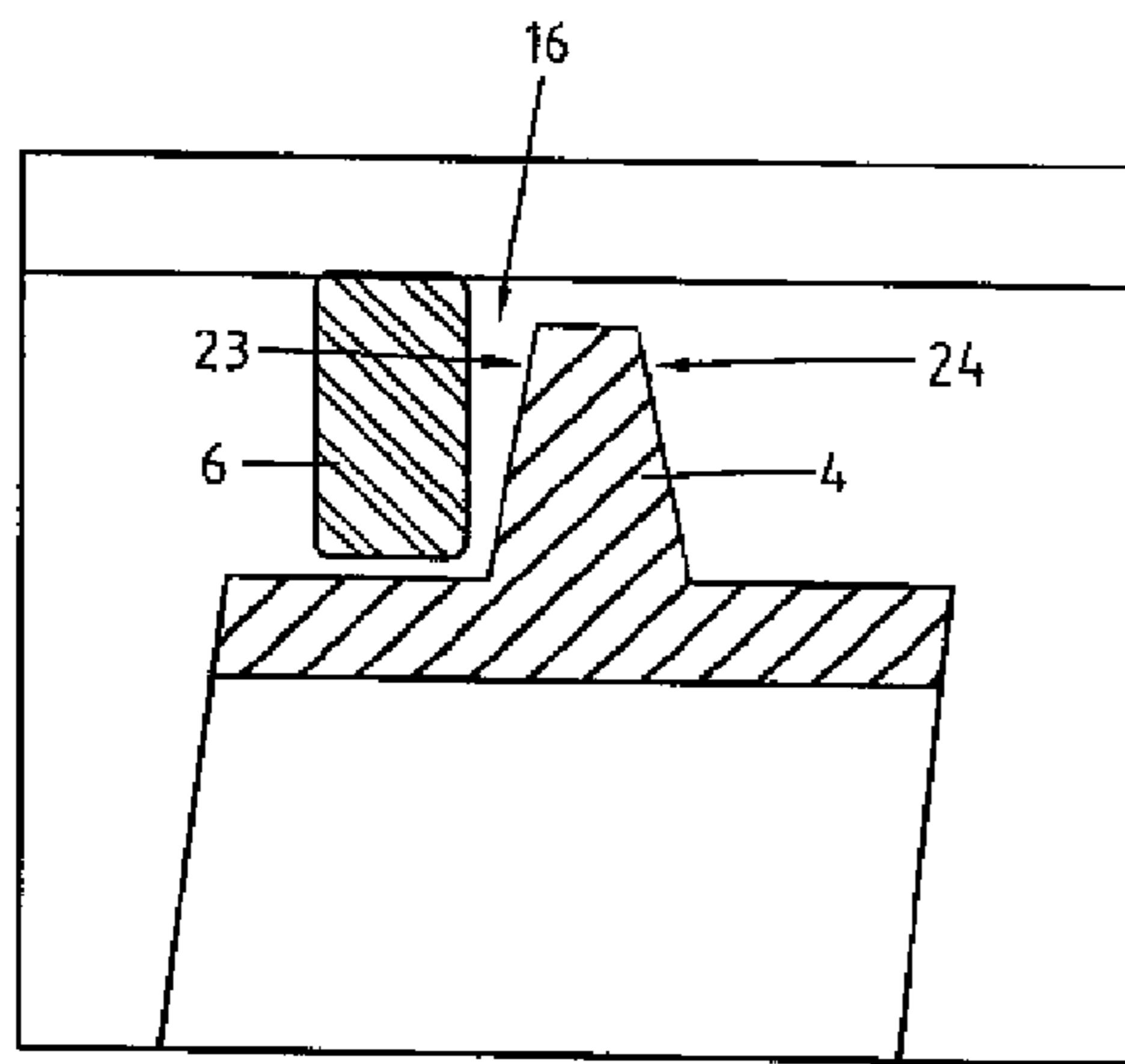
Fig. 8 (PRIOR ART)
