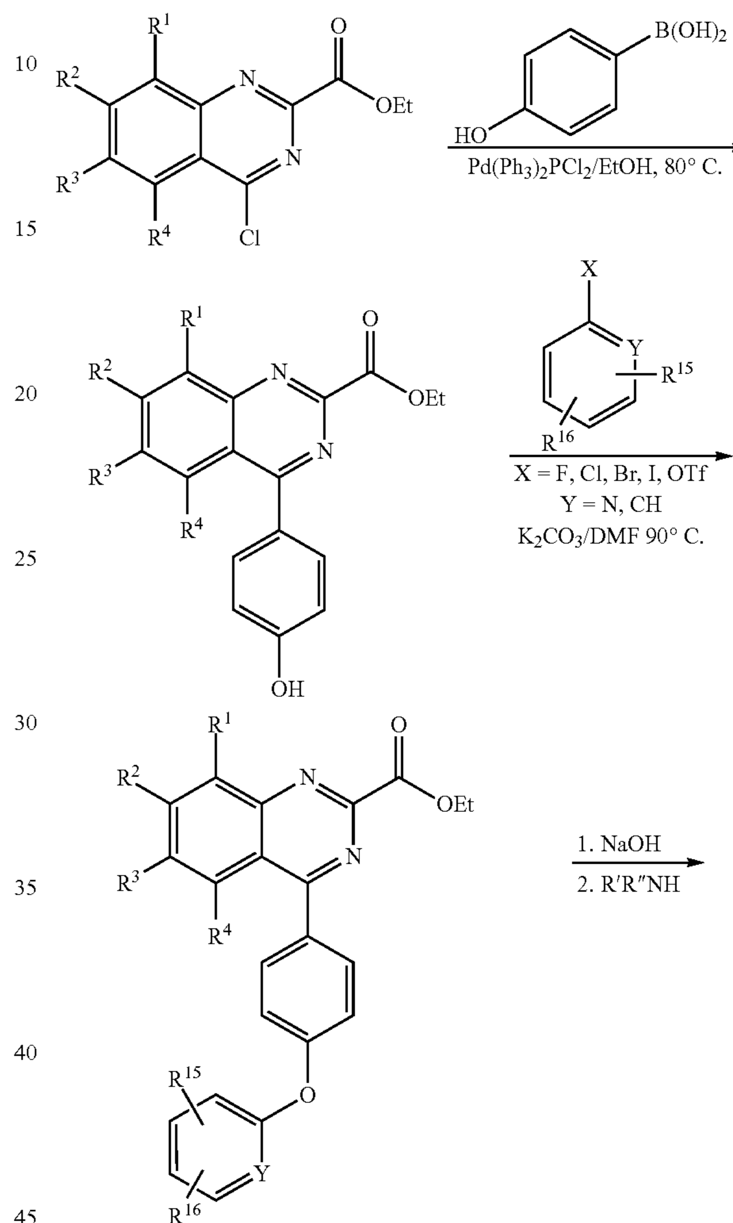
Scheme 3
