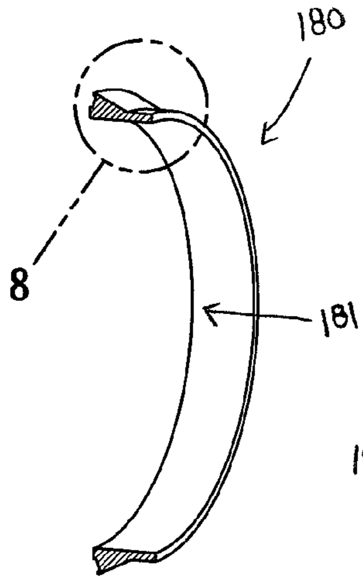
knife ring FIG. 7
