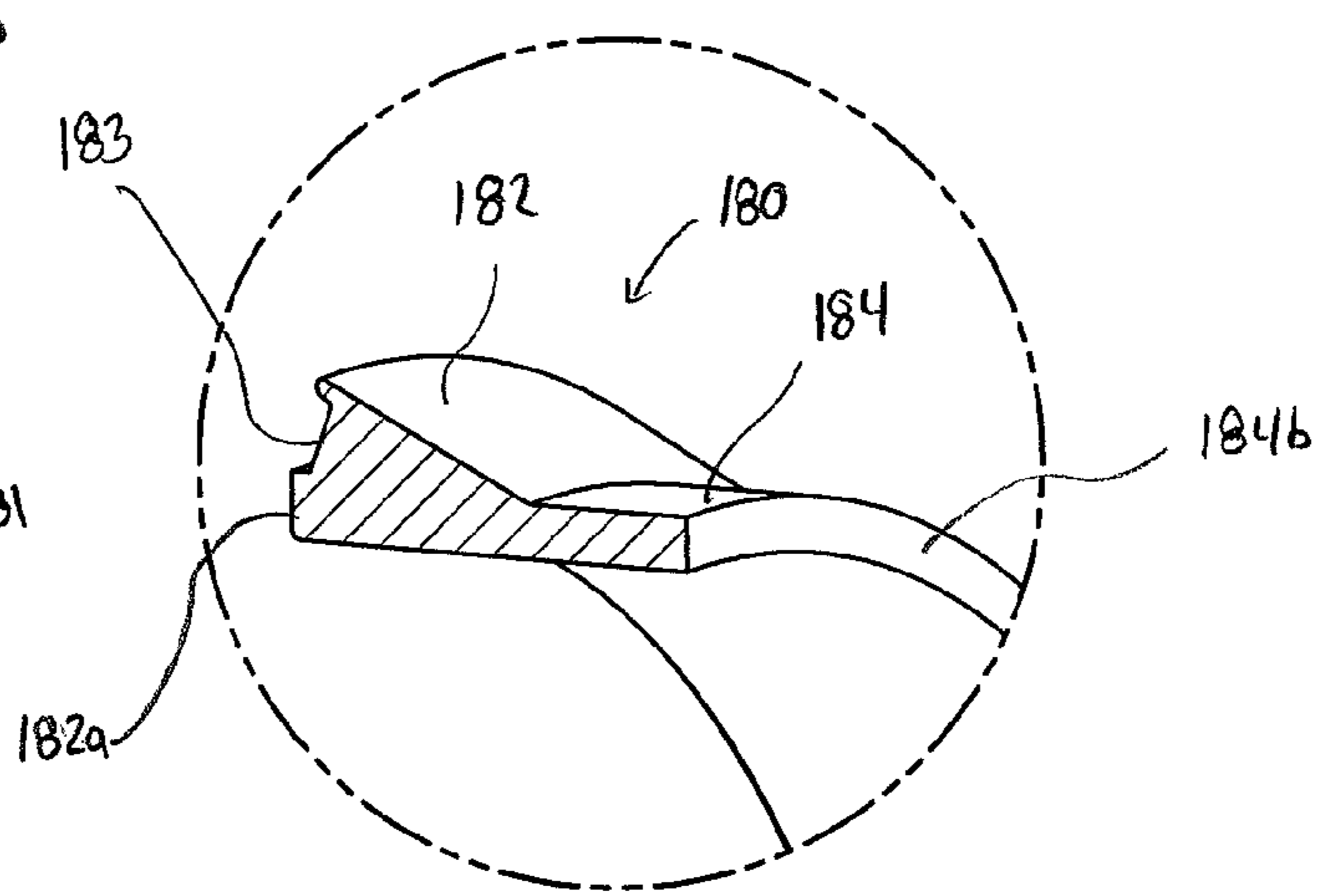
knife ring FIG. 8
