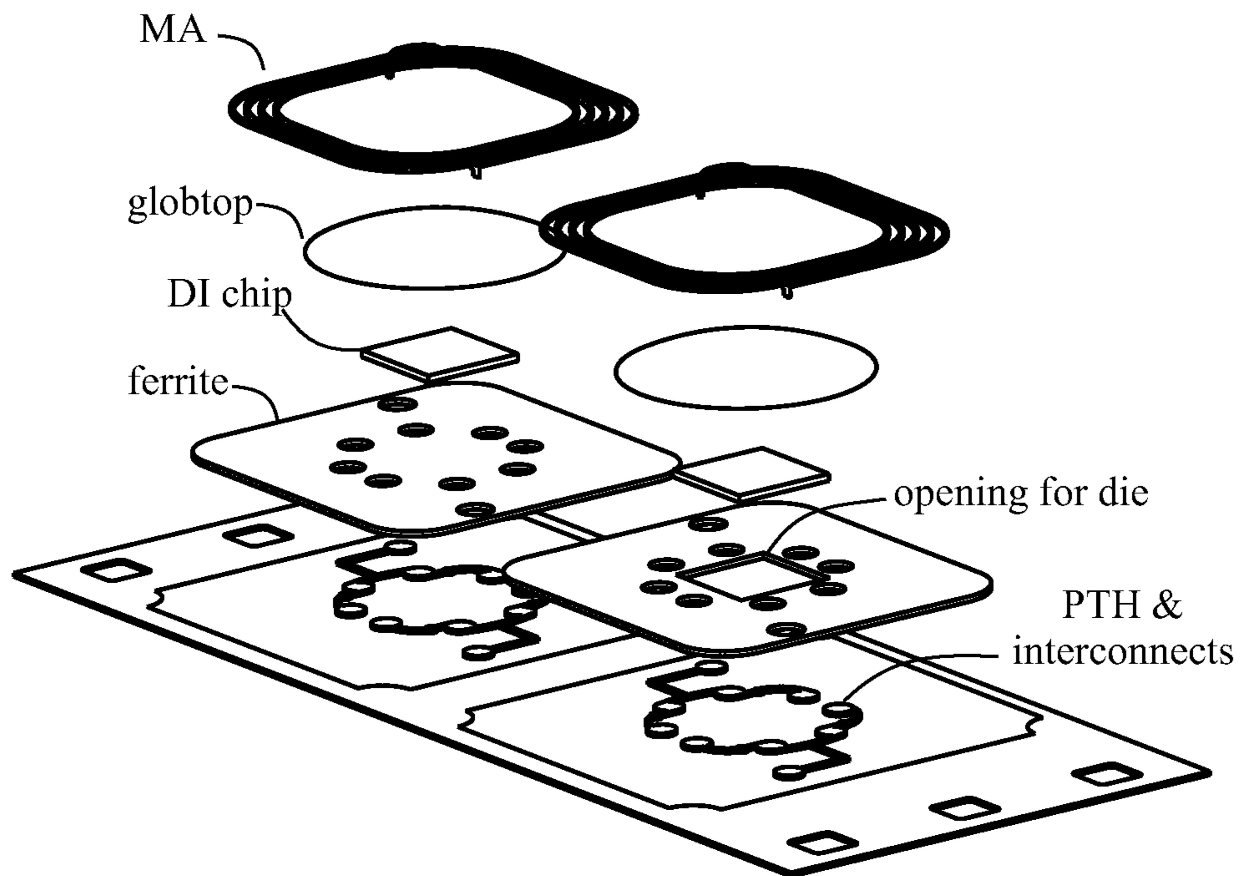
DIF Module with Ferrite Layer
