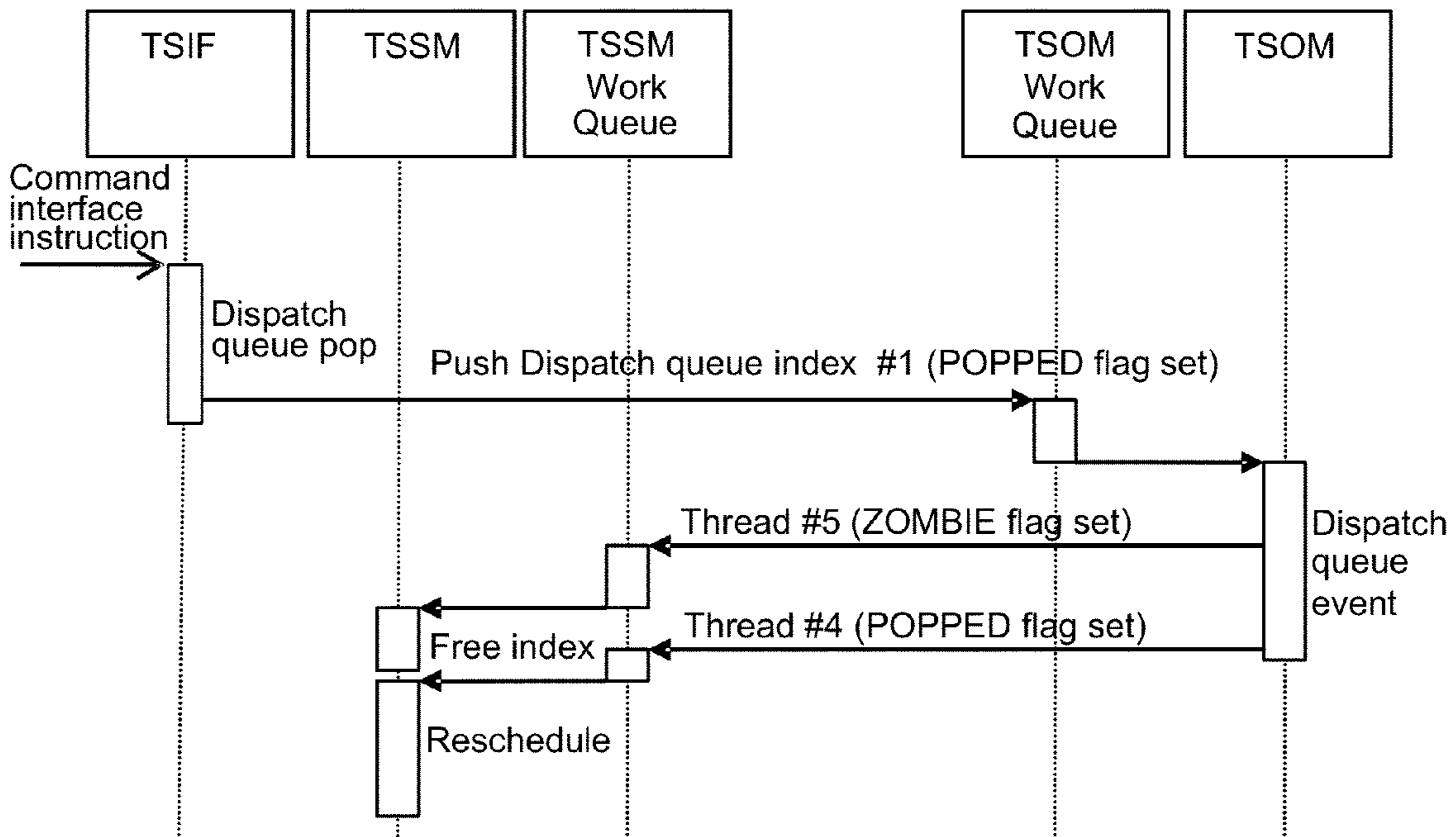
Figure 73: Pop event TSOM, TSSM interaction
