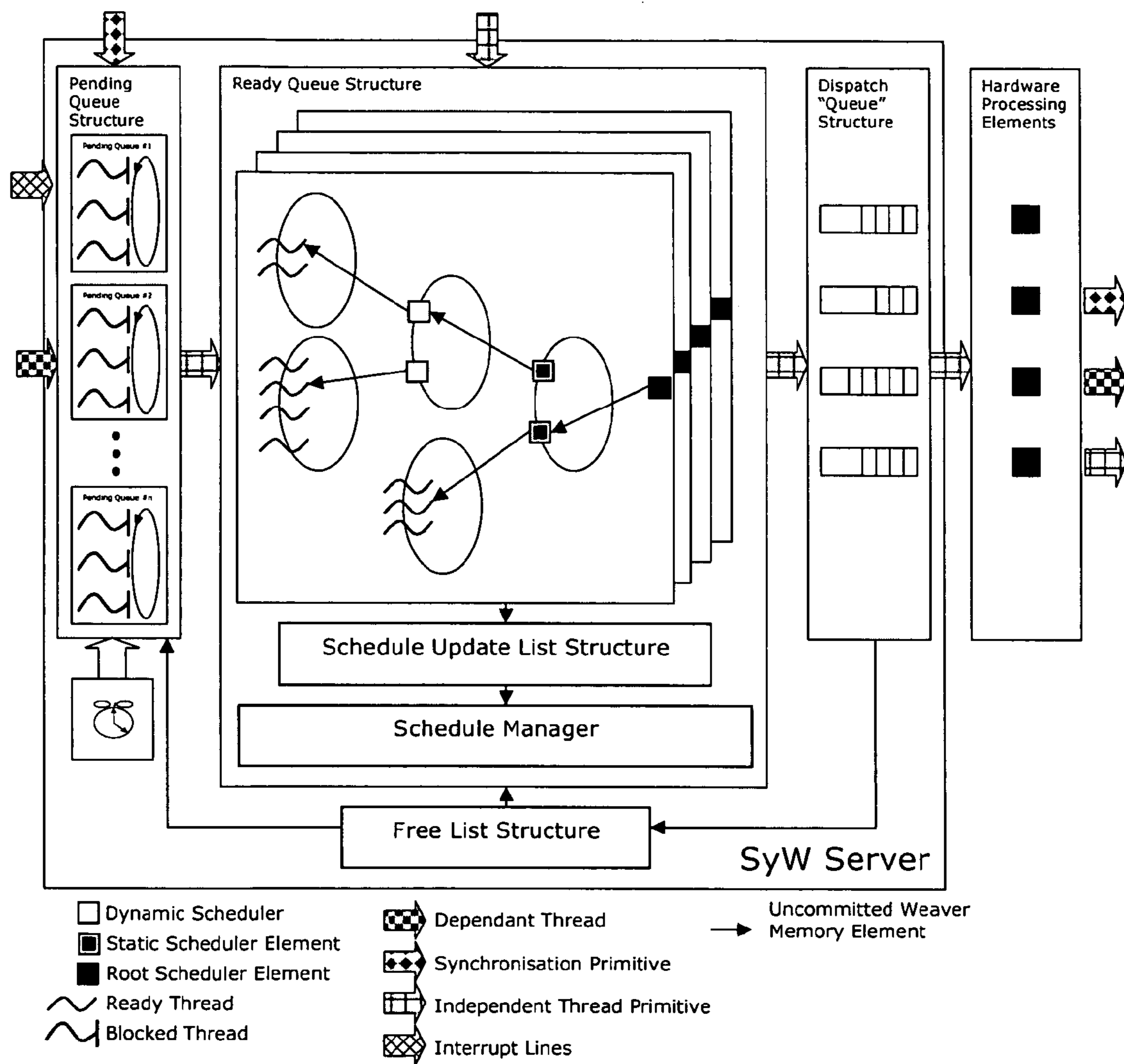
Figure 39: SystemWeaver server conceptual diagram
