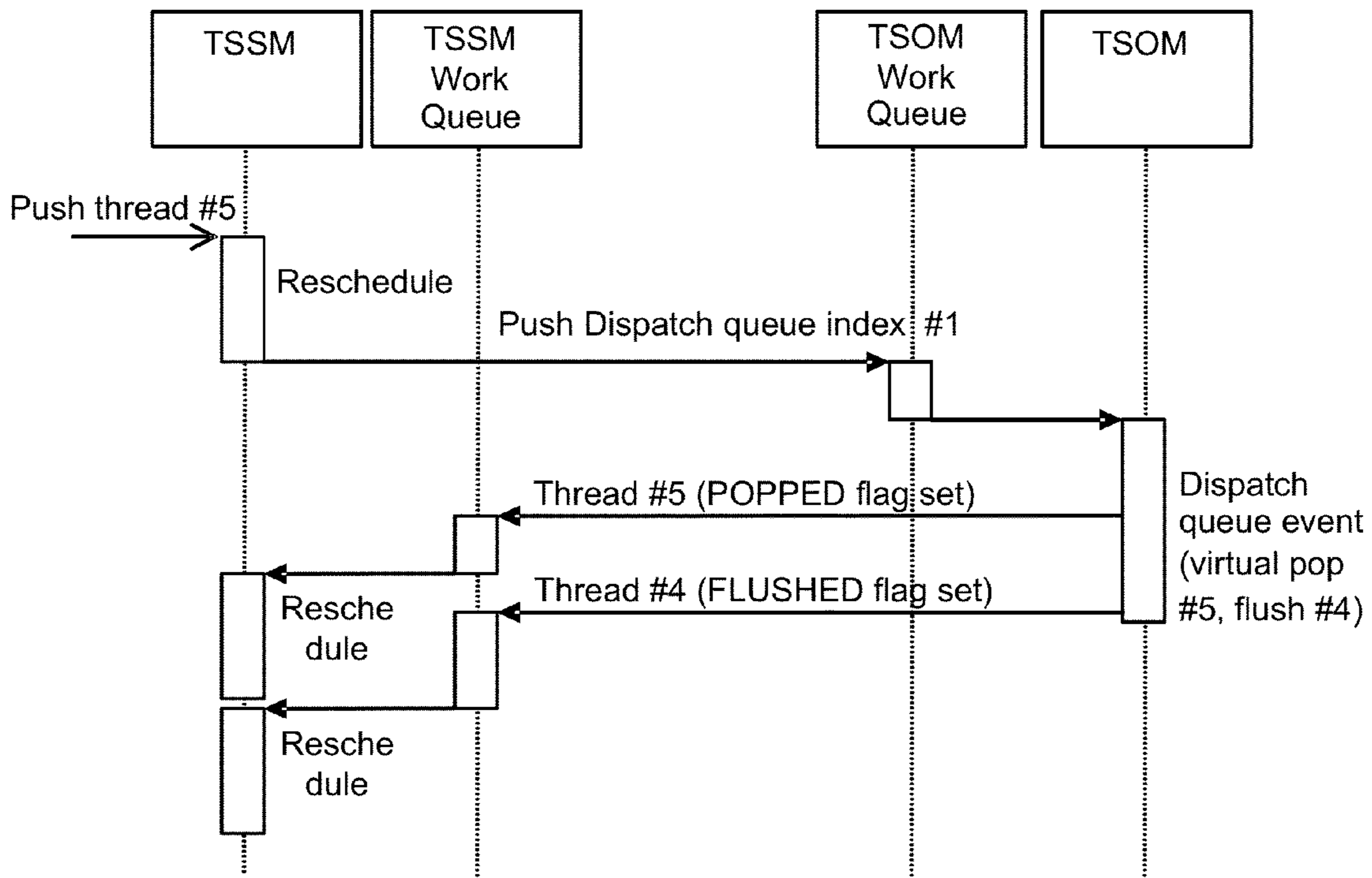
Figure 72: Push event TSOM, TSSM interaction
