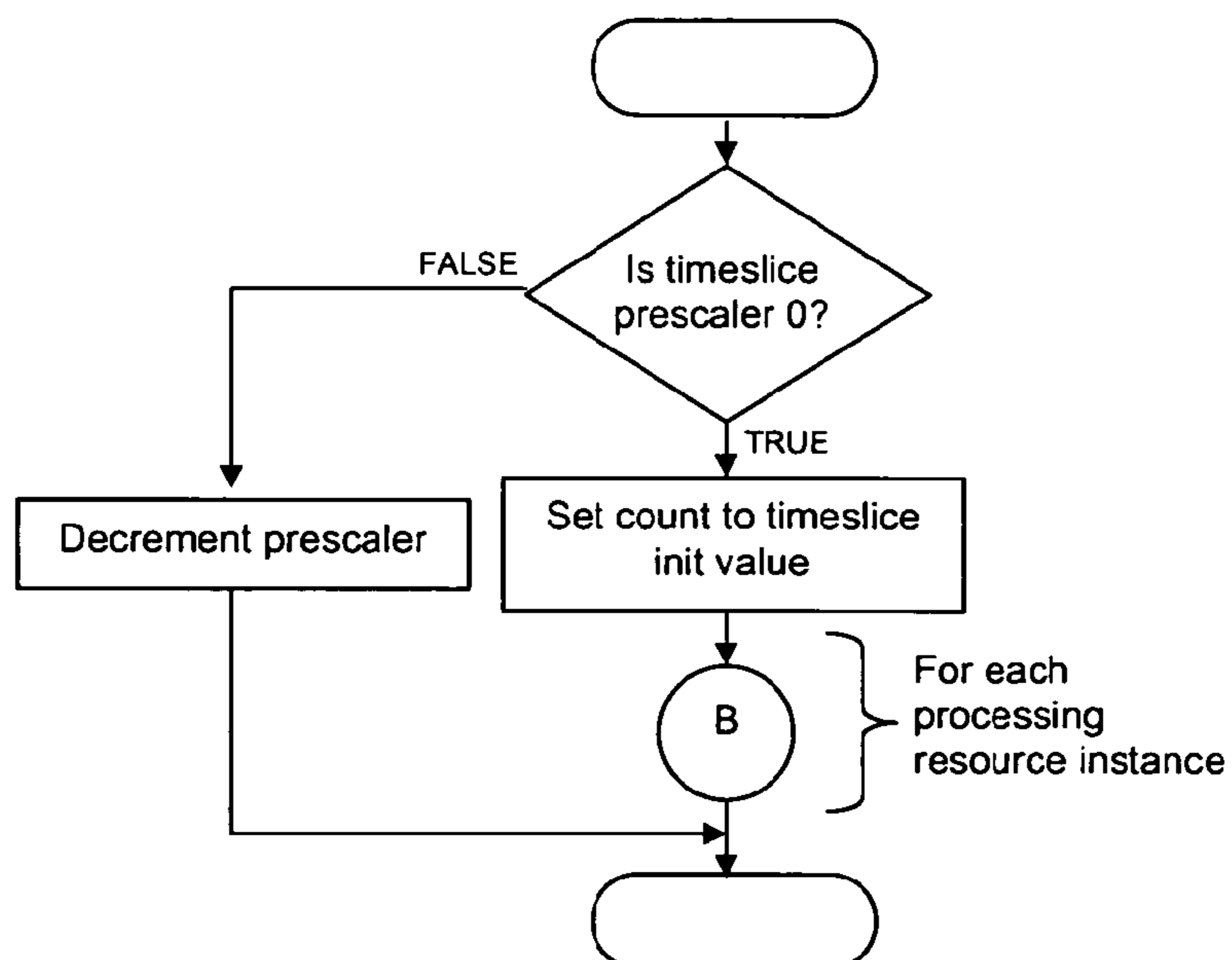
Figure 45: Timeslice control
