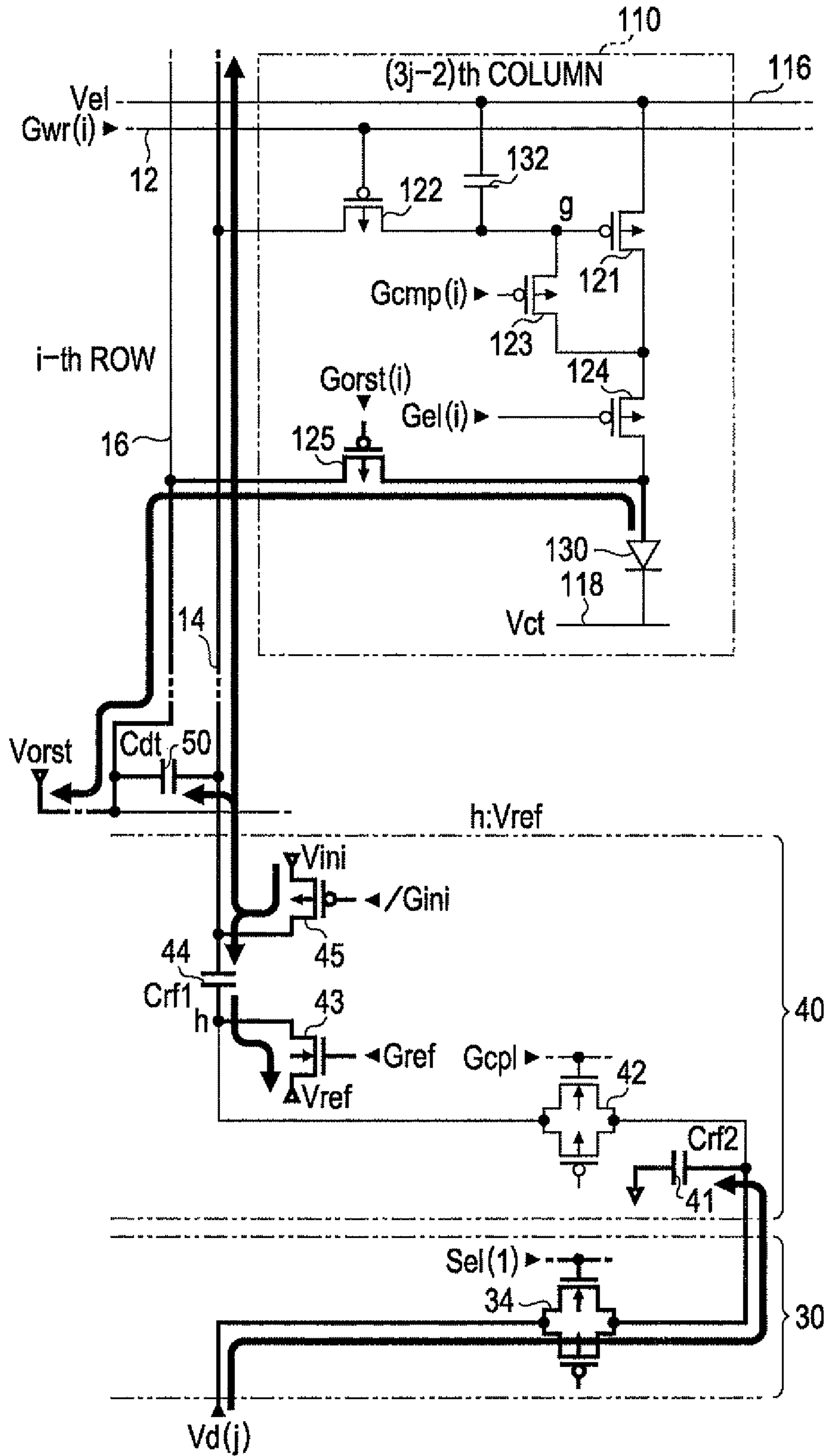
FIG. 6 <(b) INITIALIZATION PERIOD>
