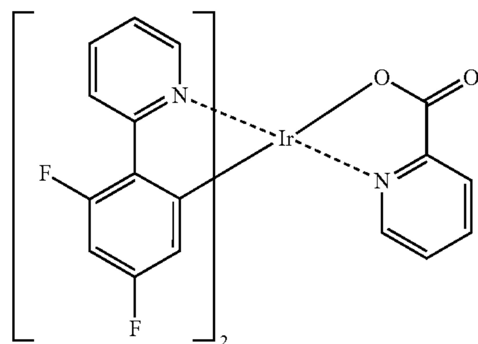
F_2\text{Irpic}
