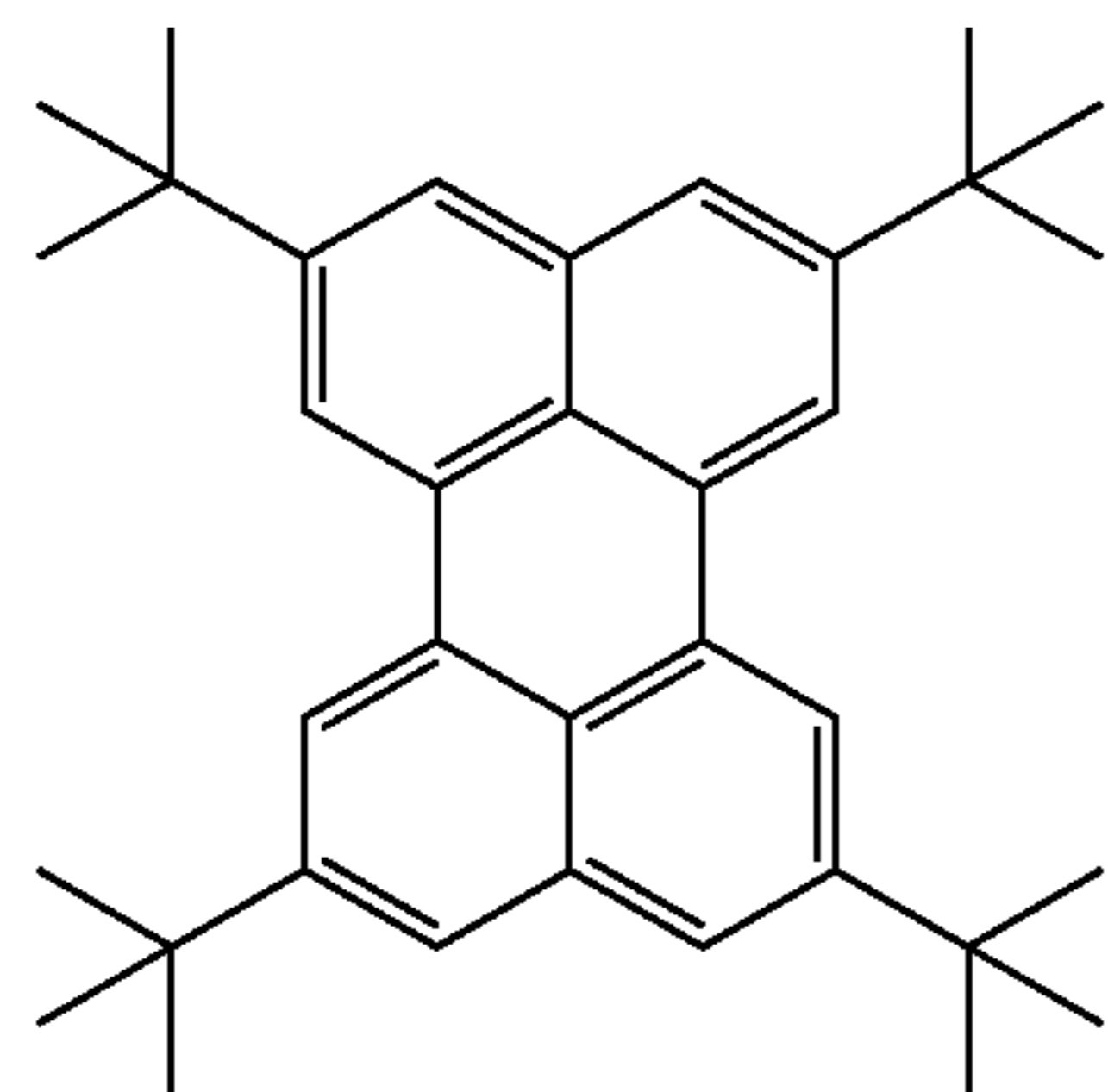
TBP
