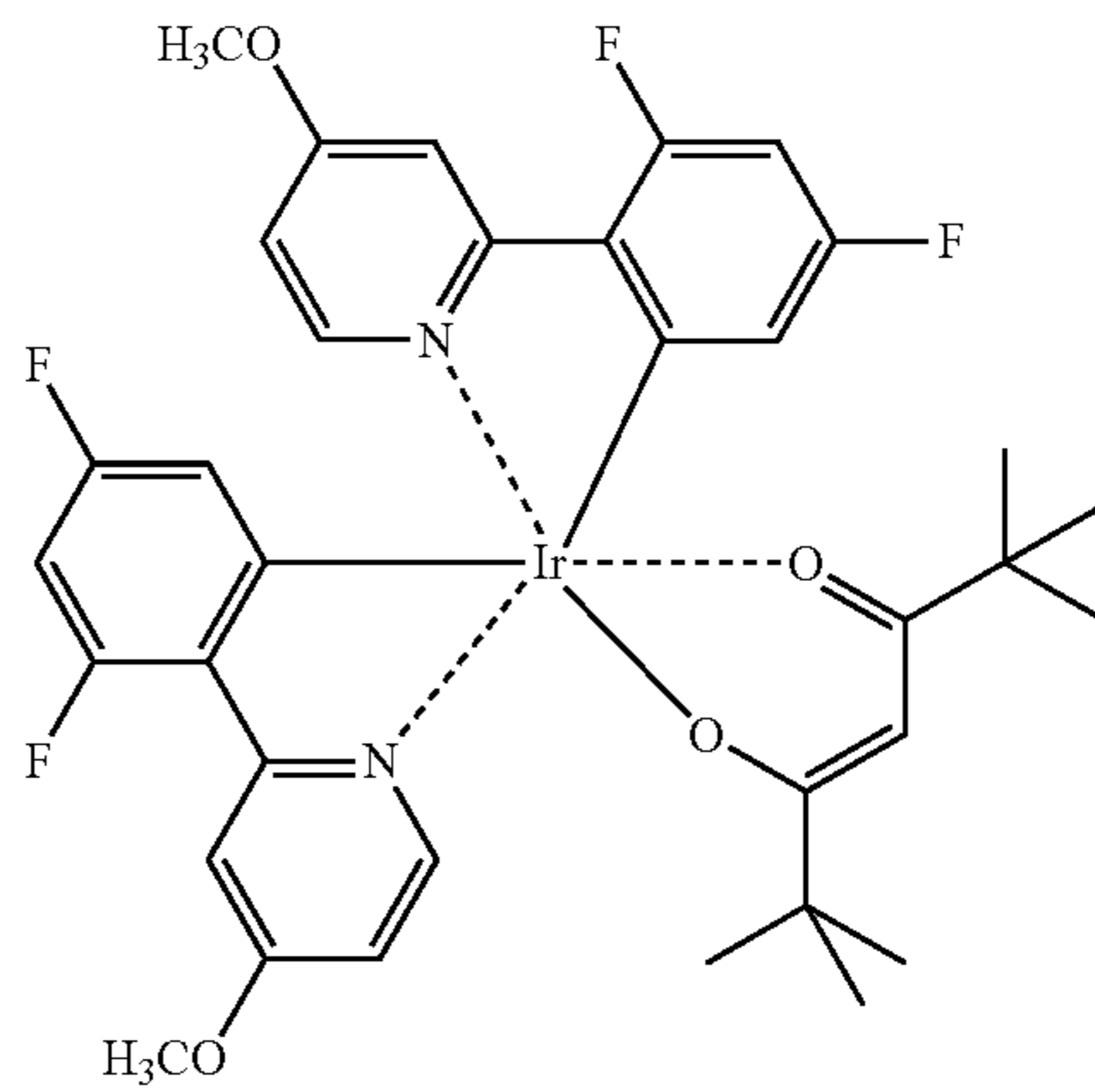
(F_2\text{ppy})_2\text{Ir}(\text{tmd})
