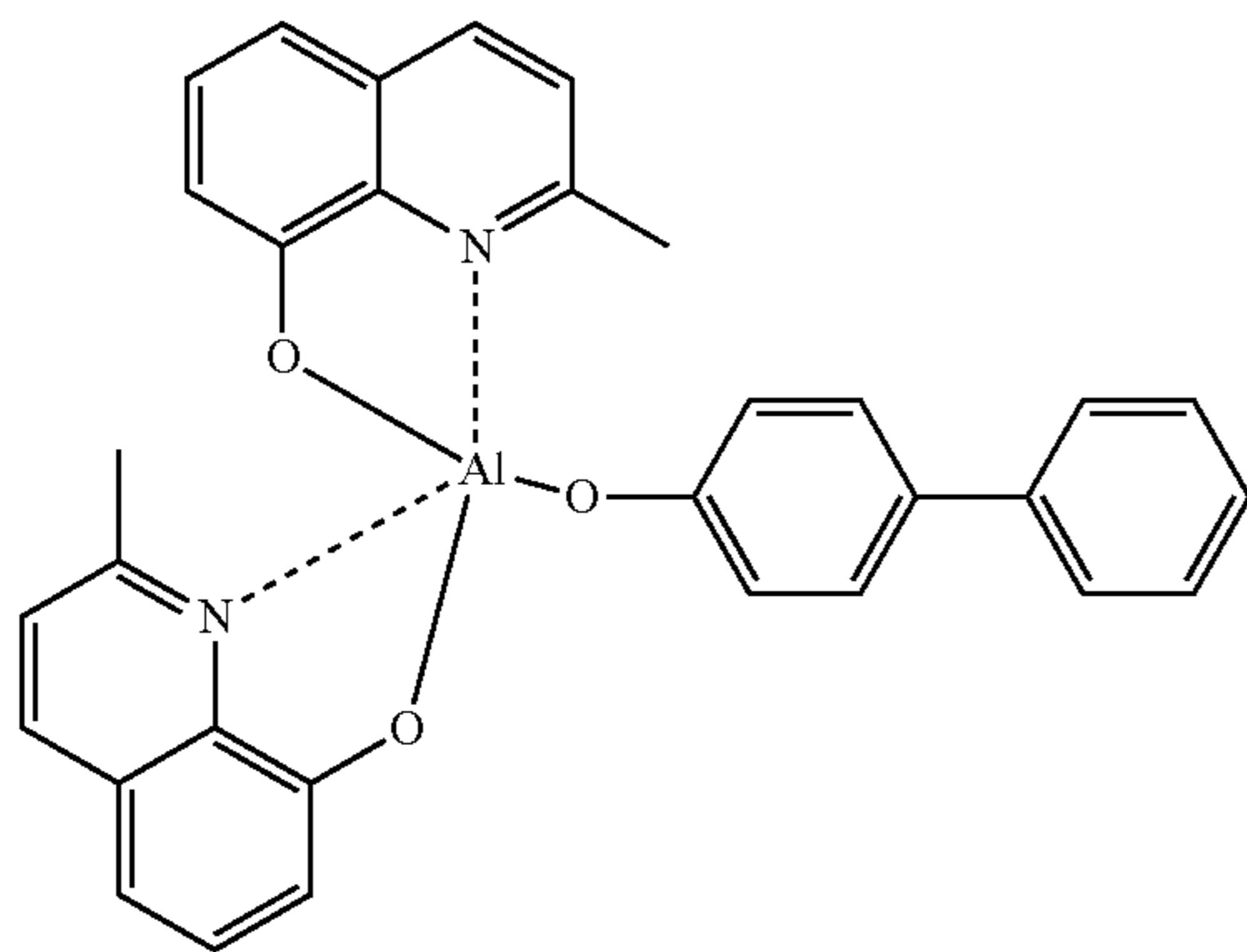
BA1q
