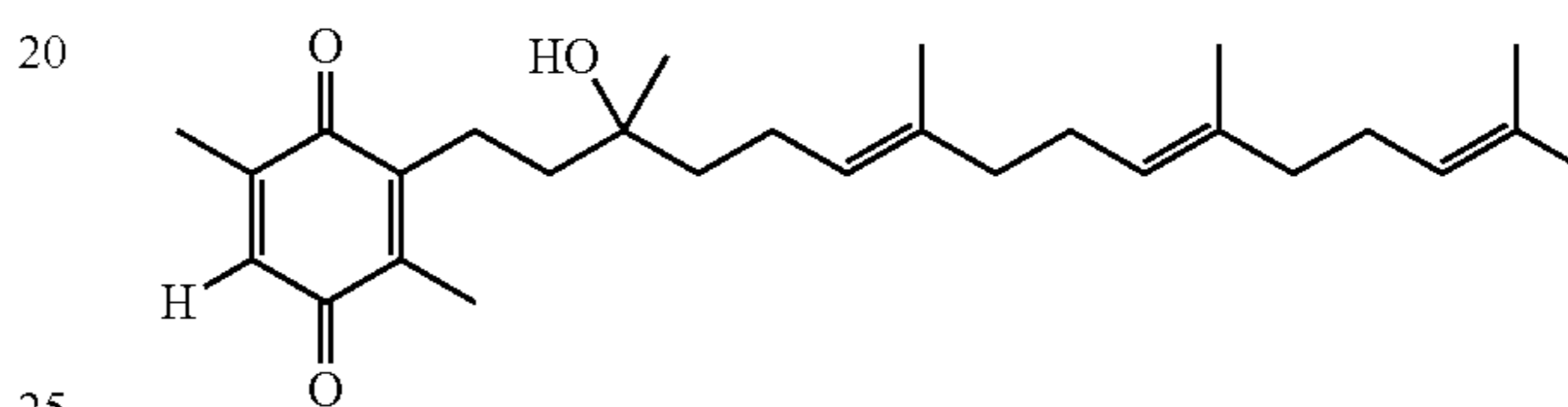
Beta-tocotrienol quinone
