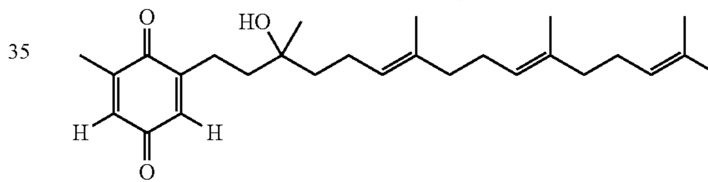
Delta-tocotrienol quinone
