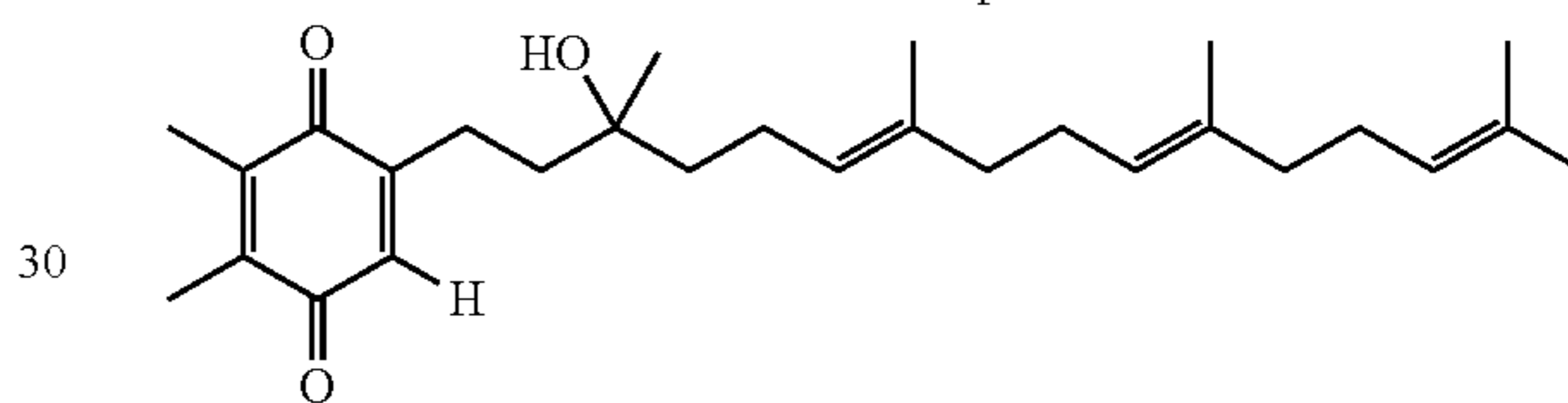
Gamma-tocotrienol quinone
