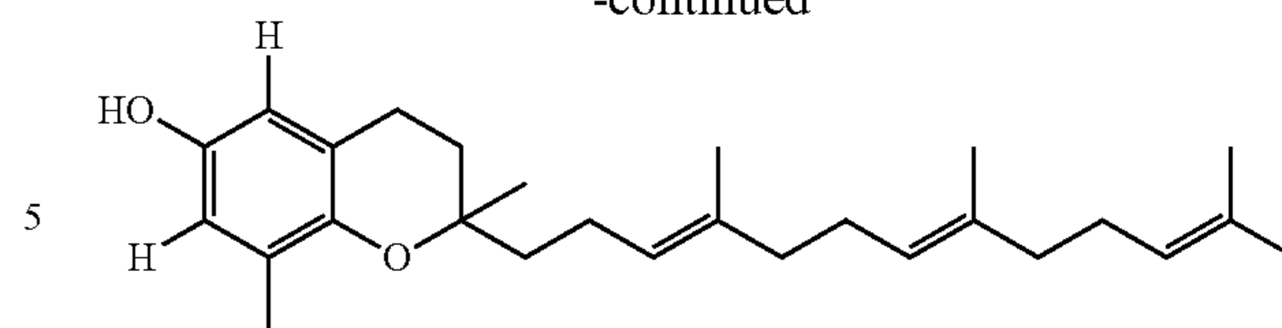
Delta-tocotrienol
