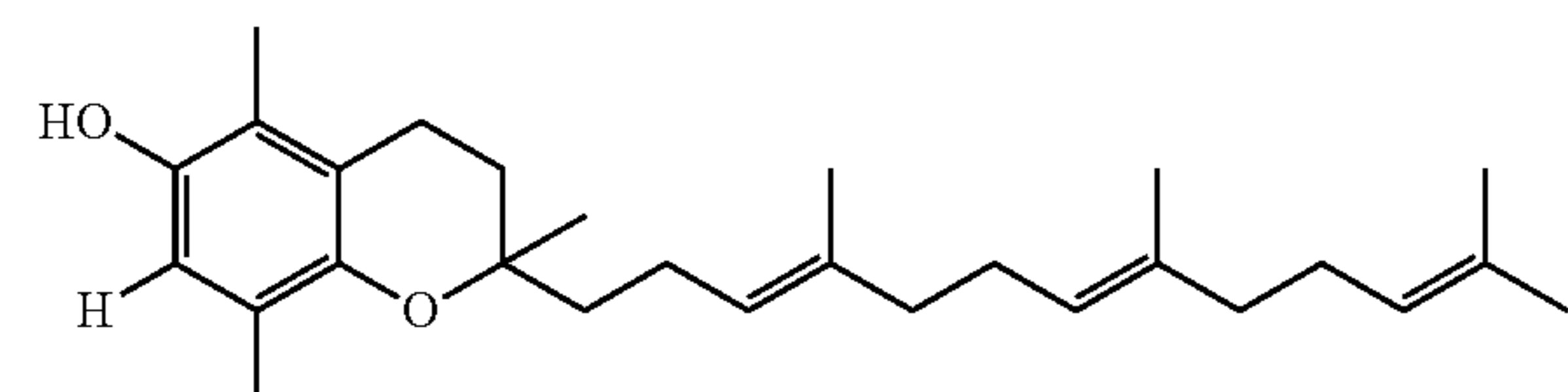
Beta-tocotrienol
