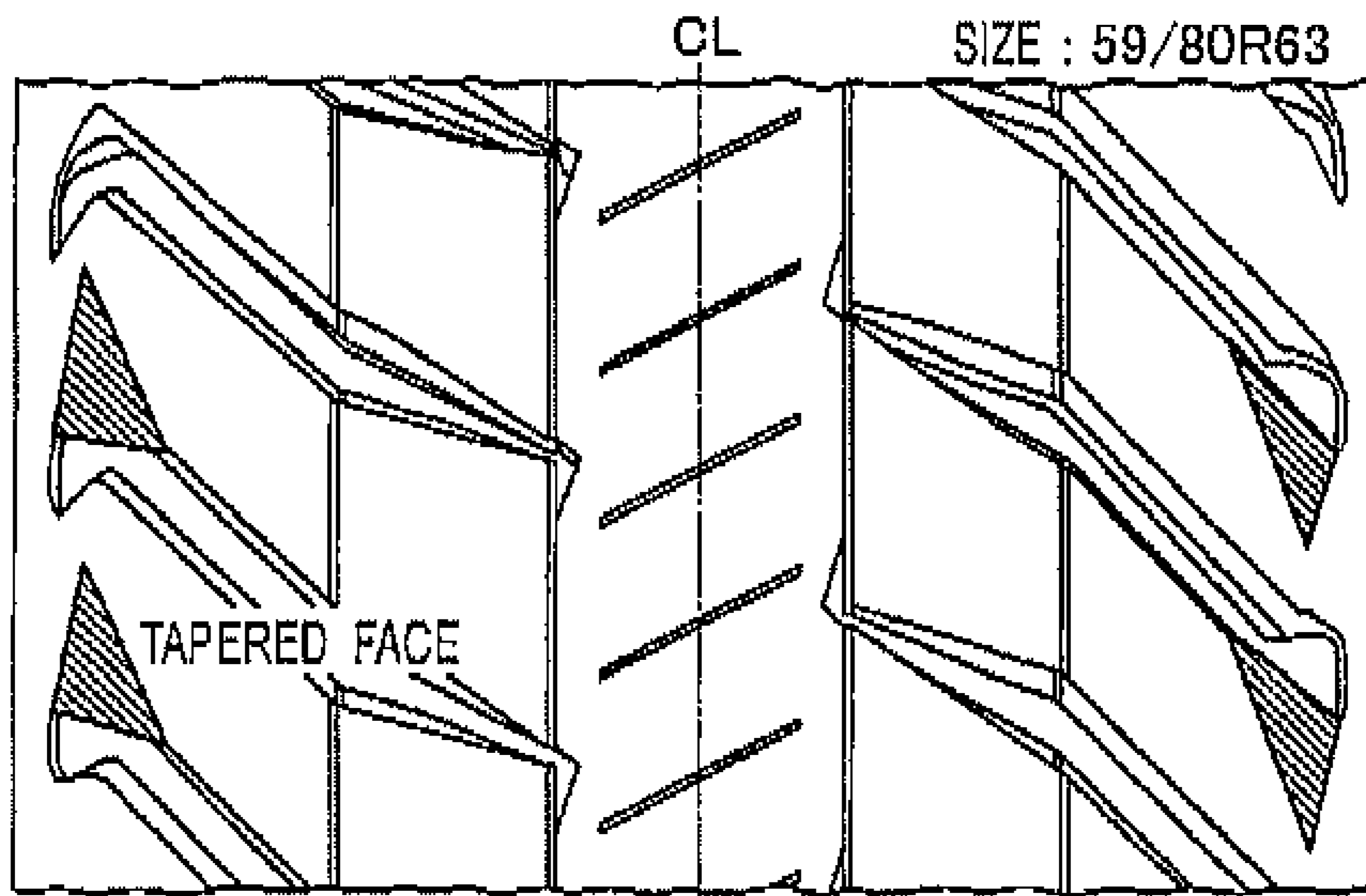
(b) EXAMPLE 1 : WITH TAPERED FACE
