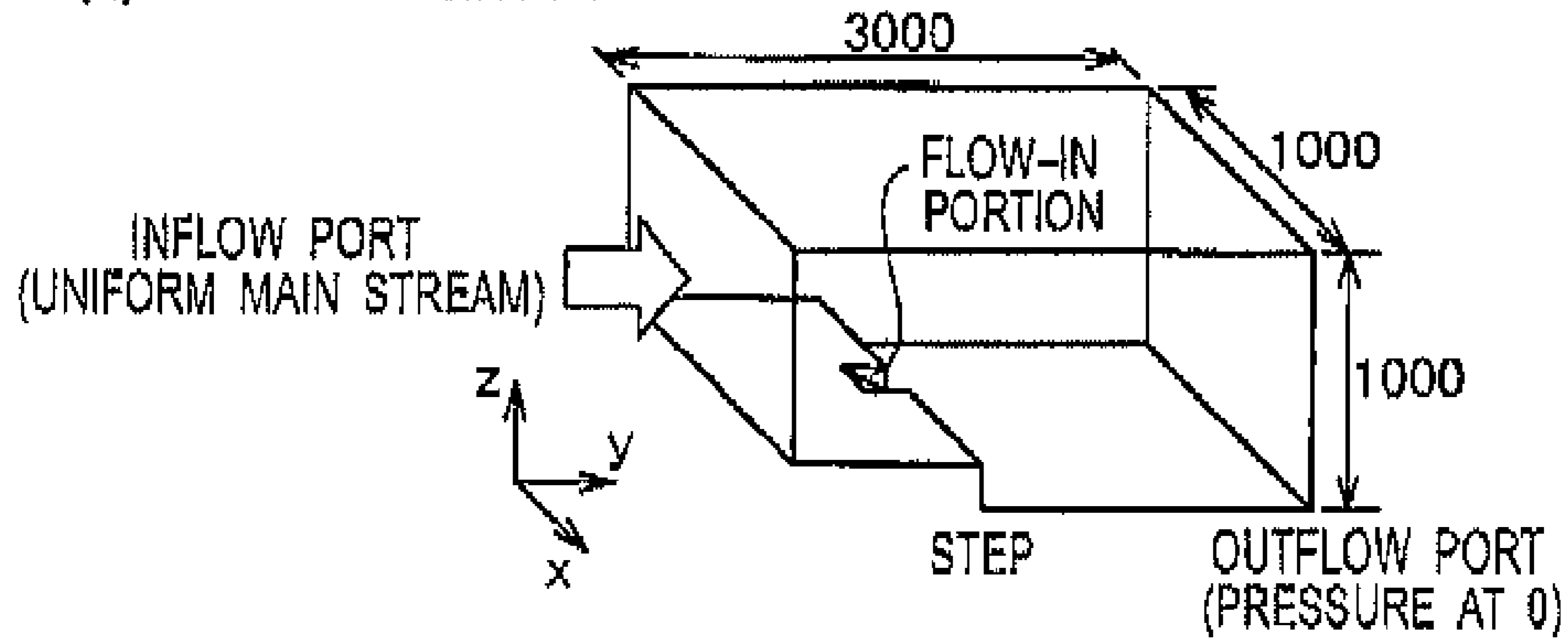
(a) OUTLINE OF SIMULATION MODEL
