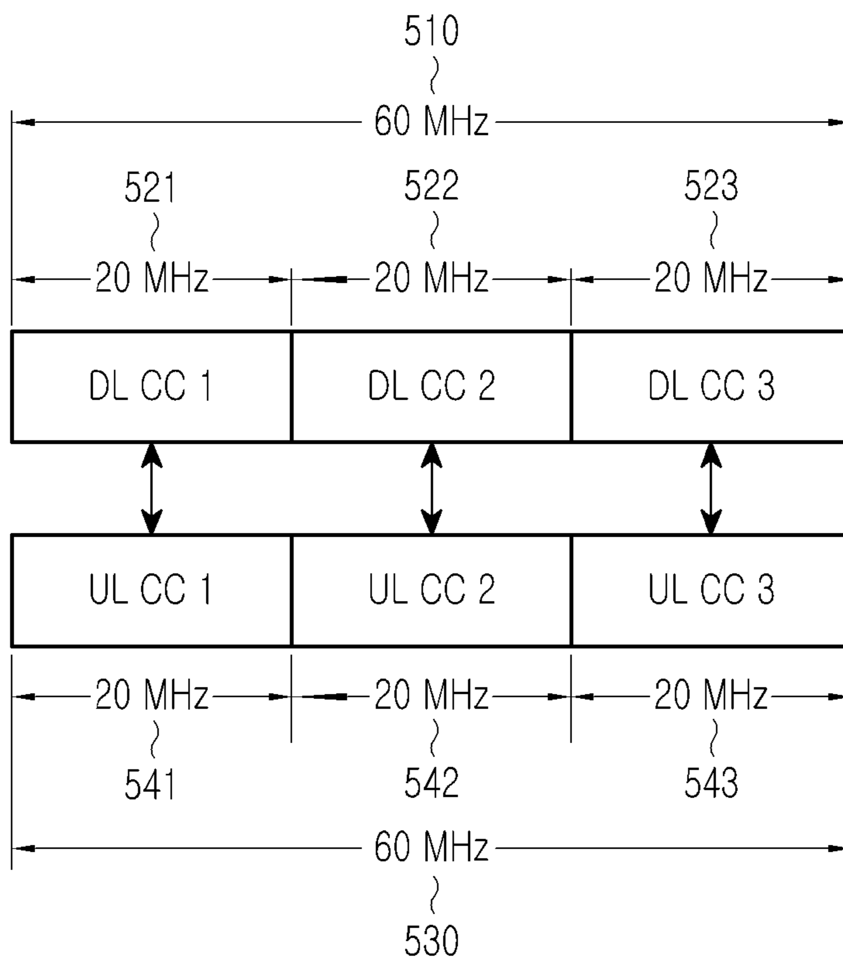
FIG.5 (PRIOR ART)
