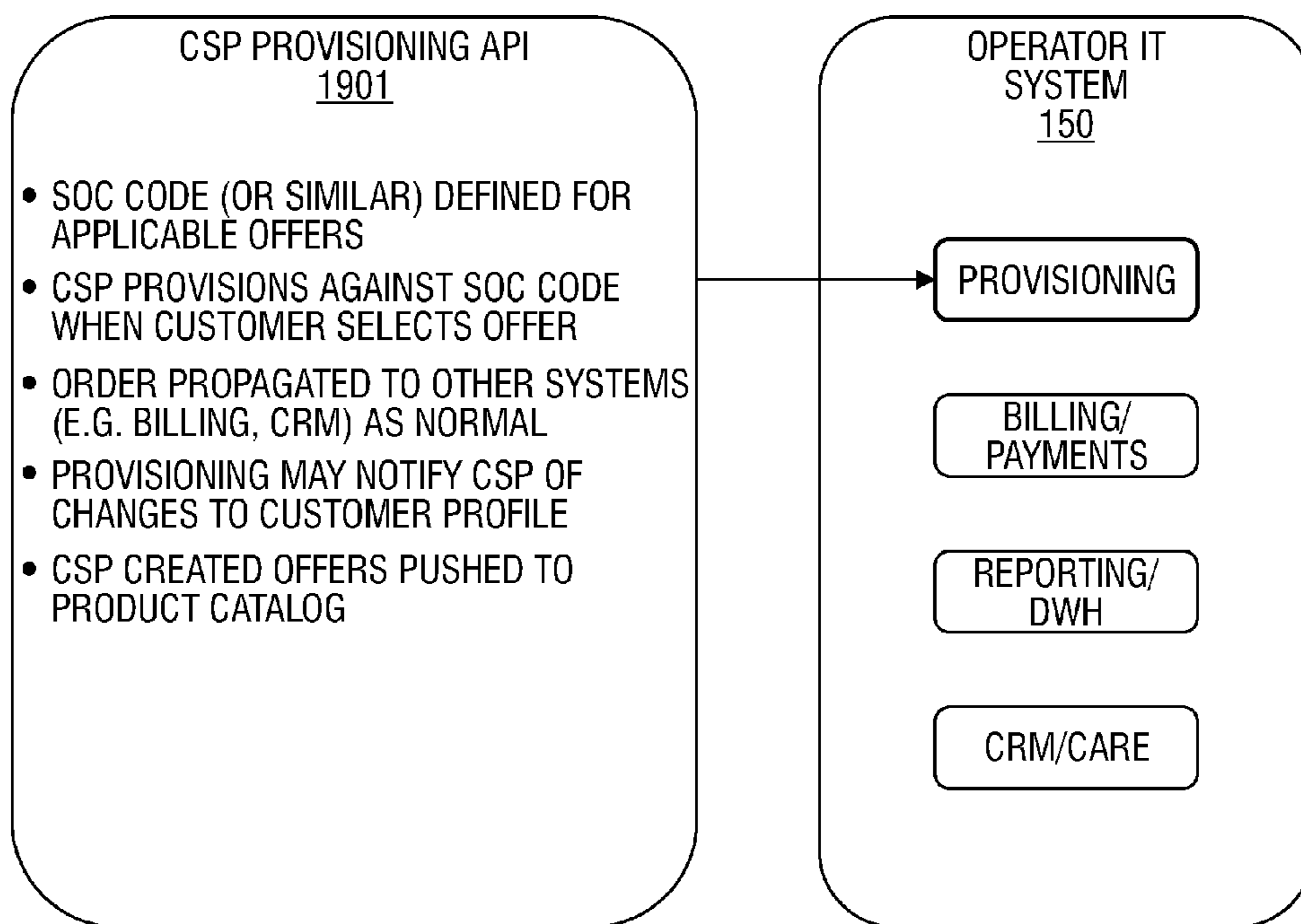
PROVISIONING INTEGRATION
