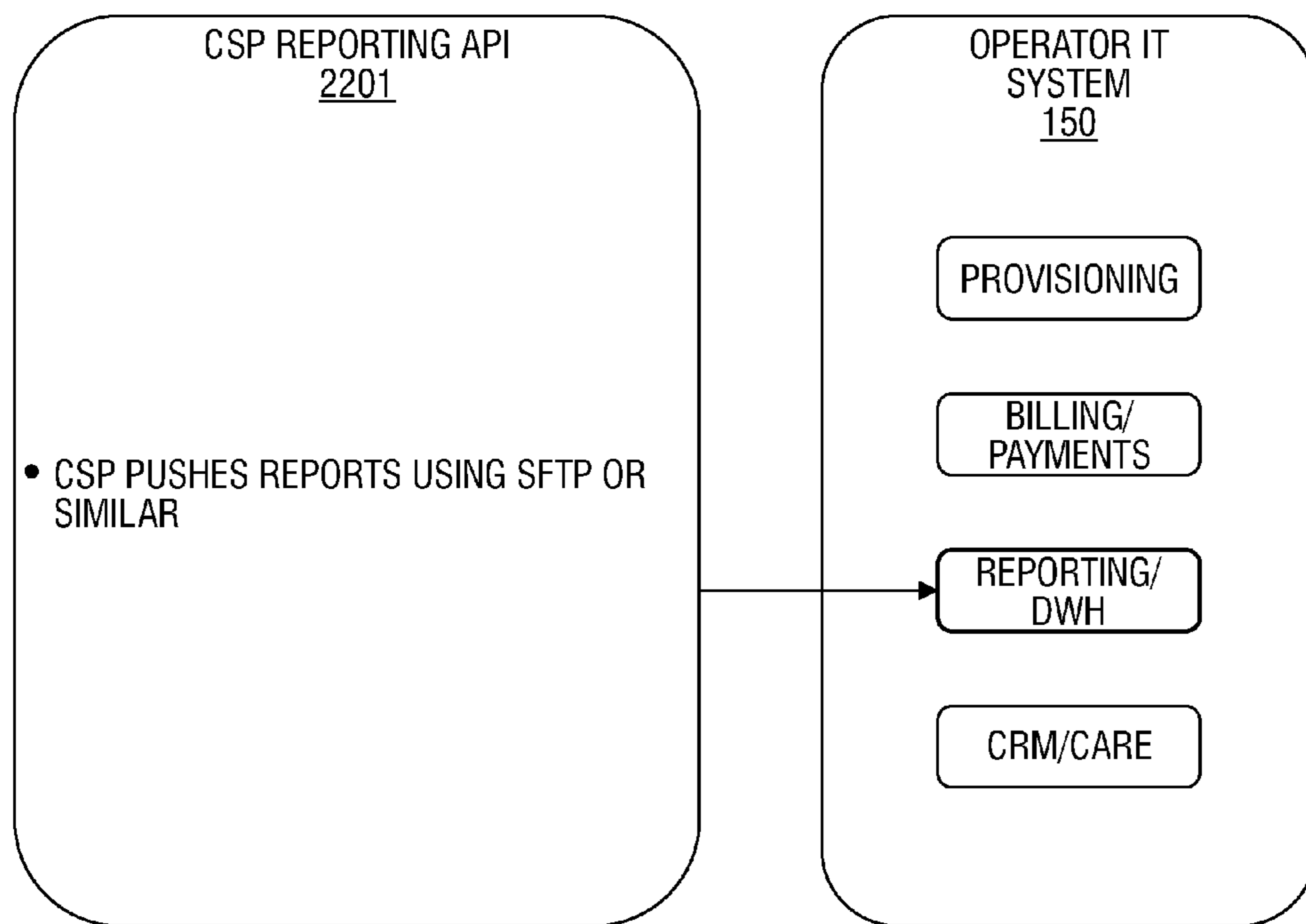
REPORTING INTEGRATION
