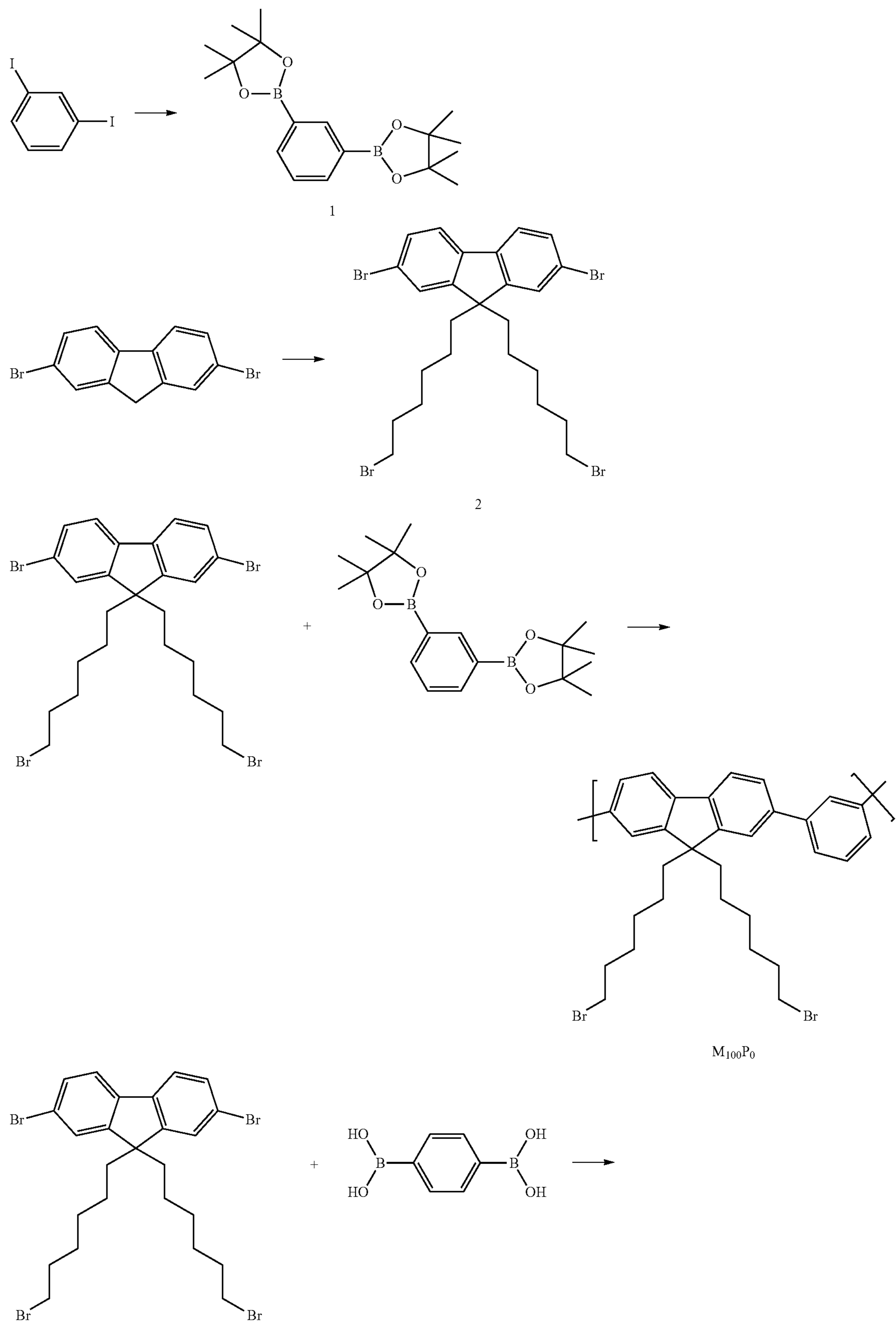
Scheme 1. Synthetic procedure for cationic water-soluble polymers.
