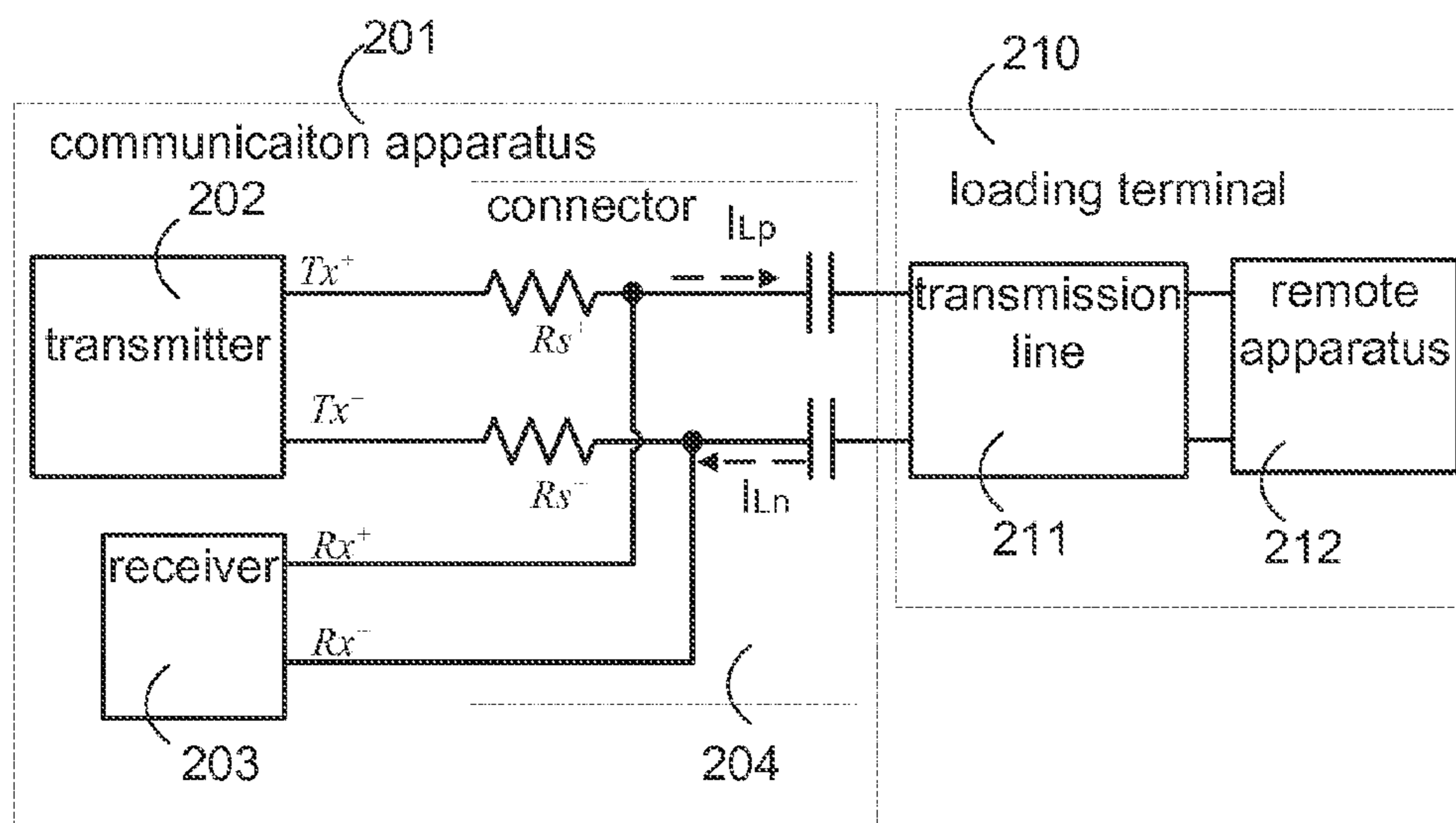
FIG. 2 (PRIOR ART)
