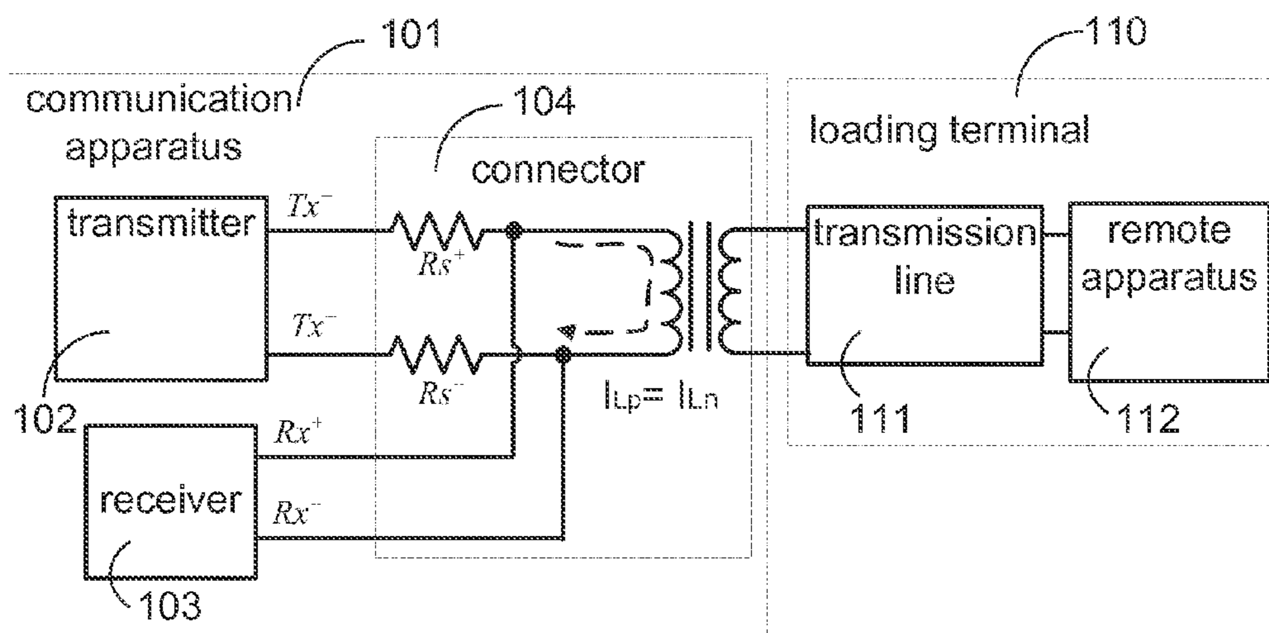
FIG. 1 (PRIOR ART)
