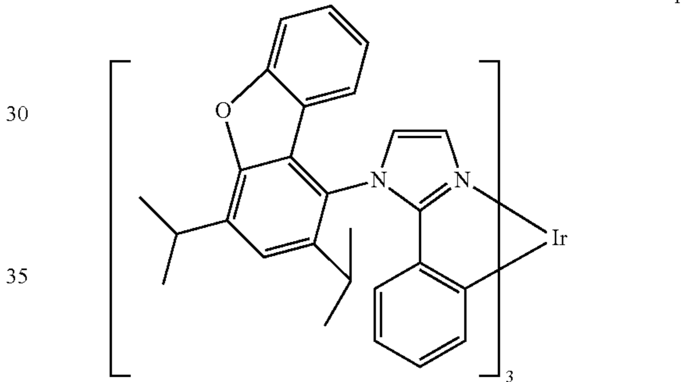
Compound 3
