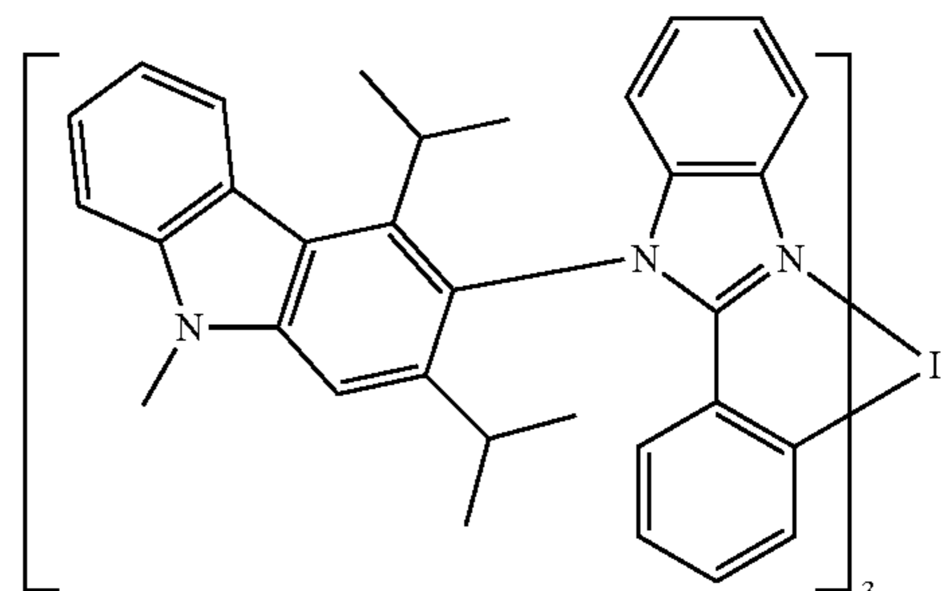
Compound 63
