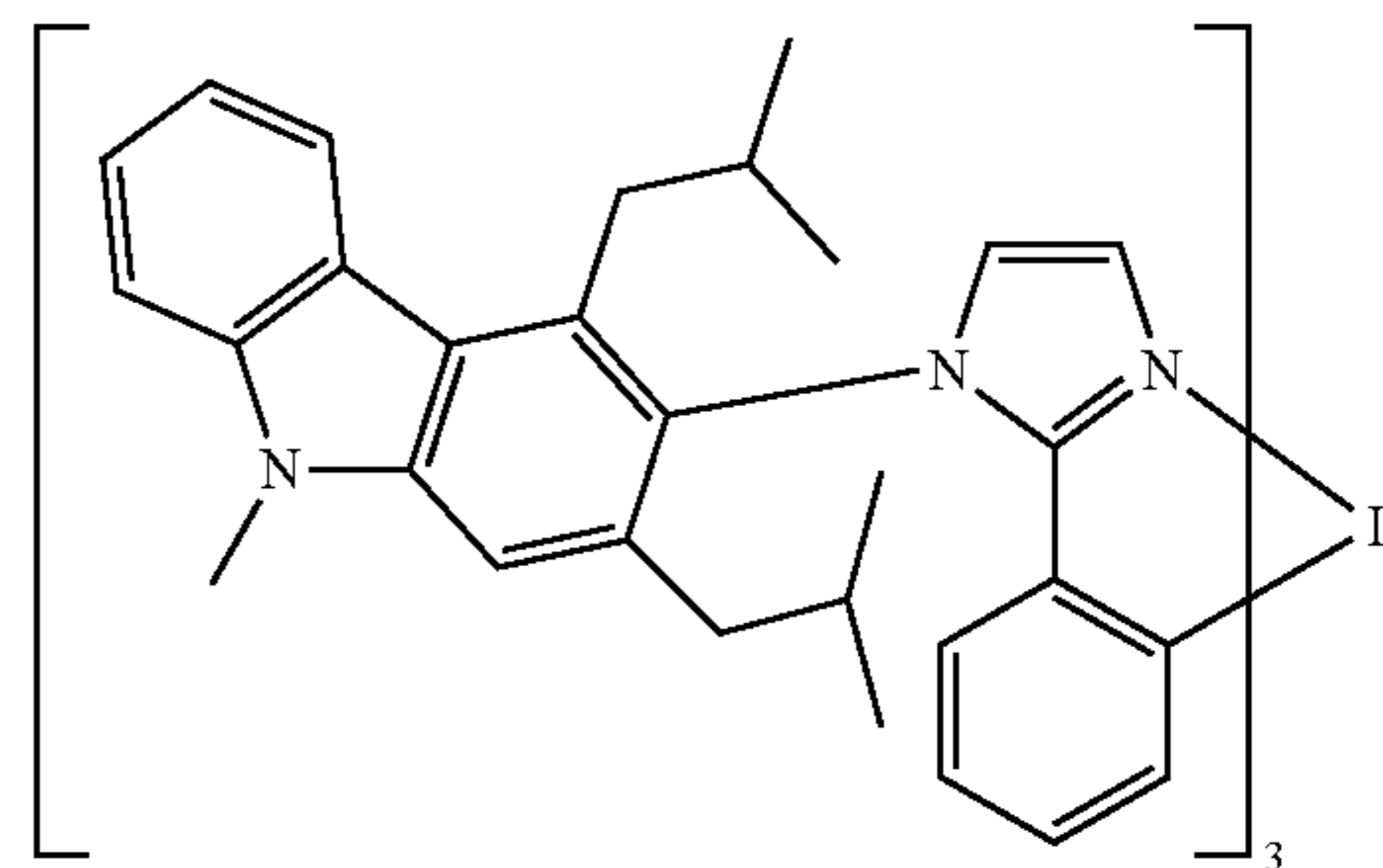
Compound 30
