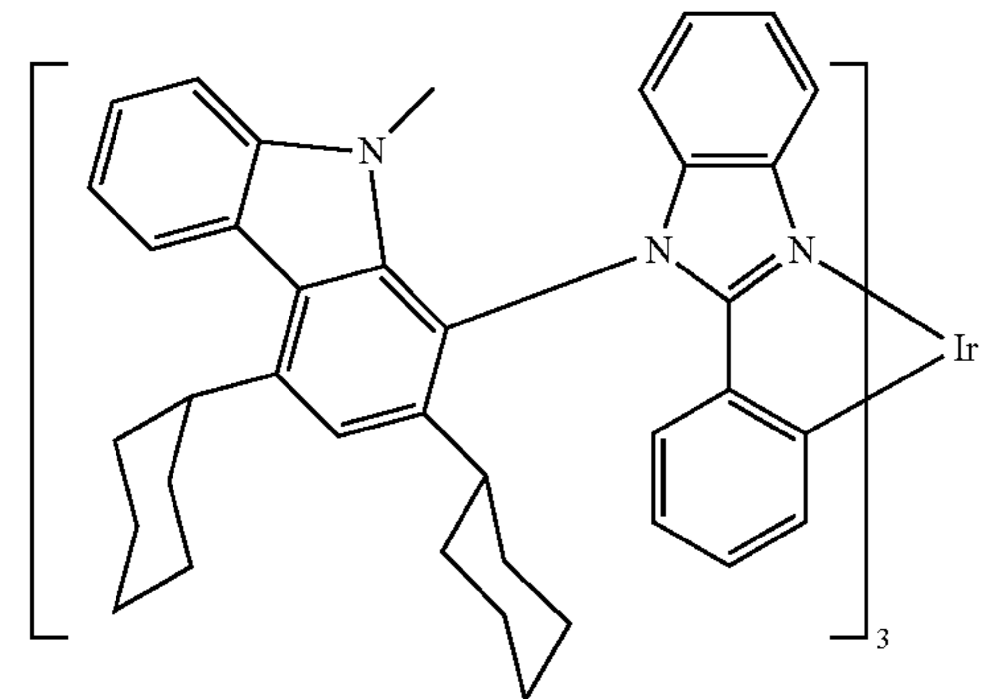
Compound 72
