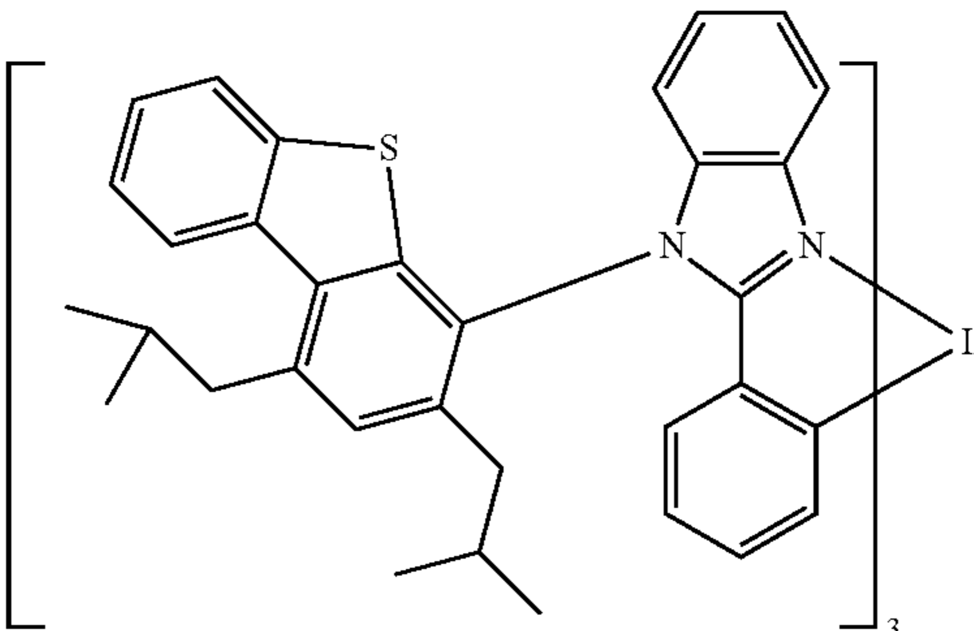
Compound 56
