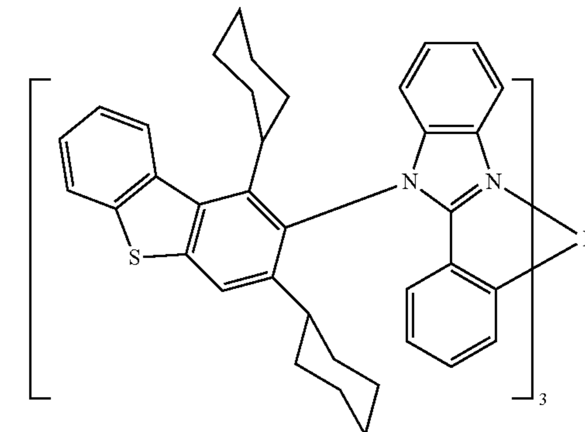
Compound 58
