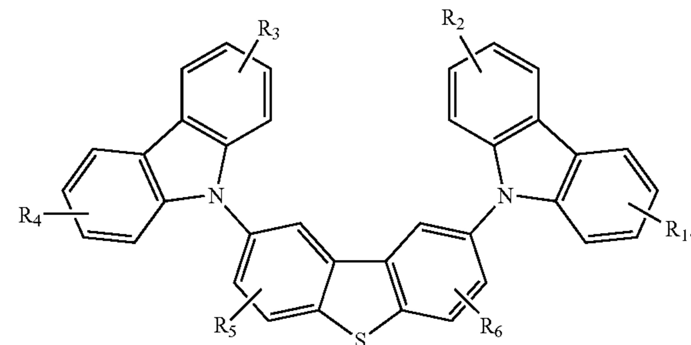
Formula II
