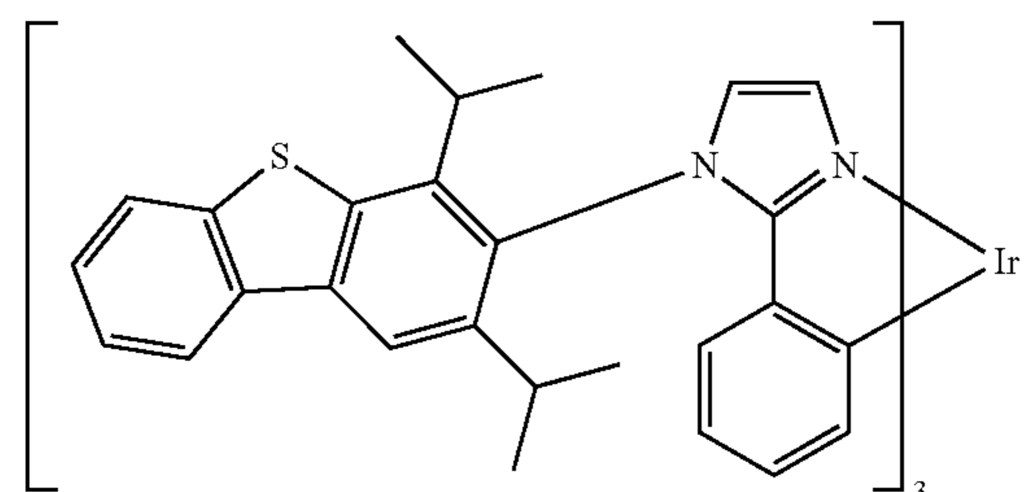
Compound 13
