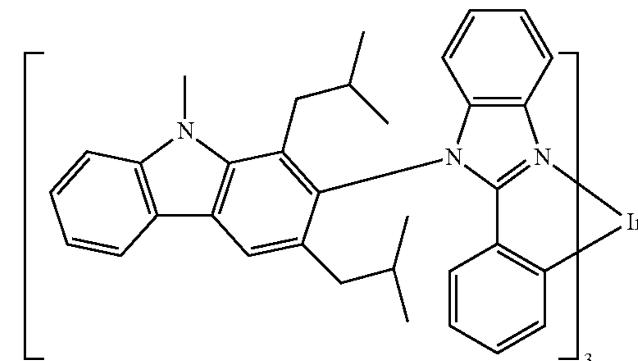
Compound 66
