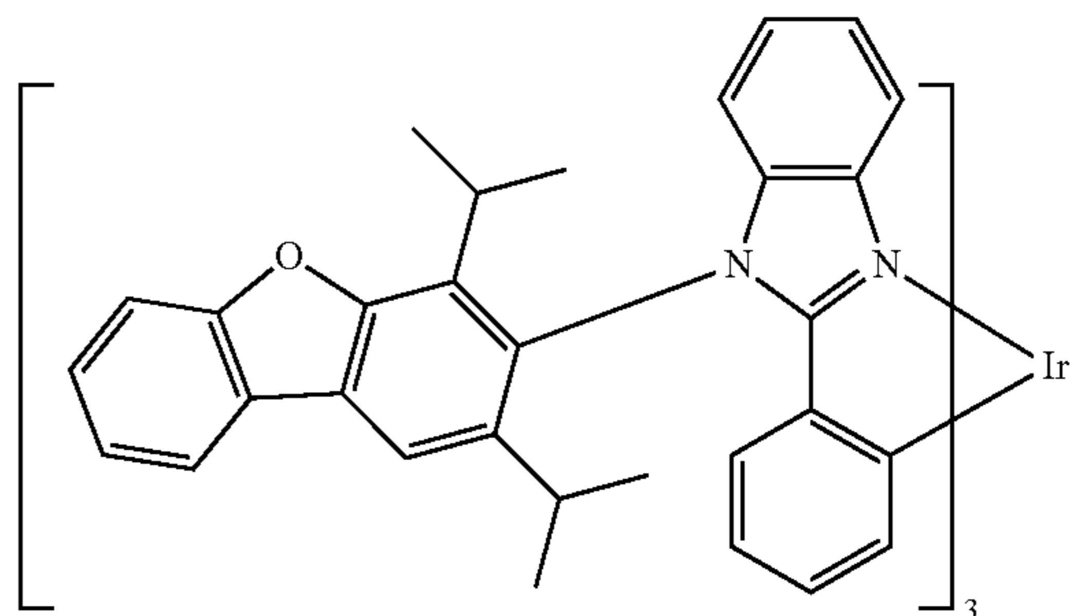
Compound 37
