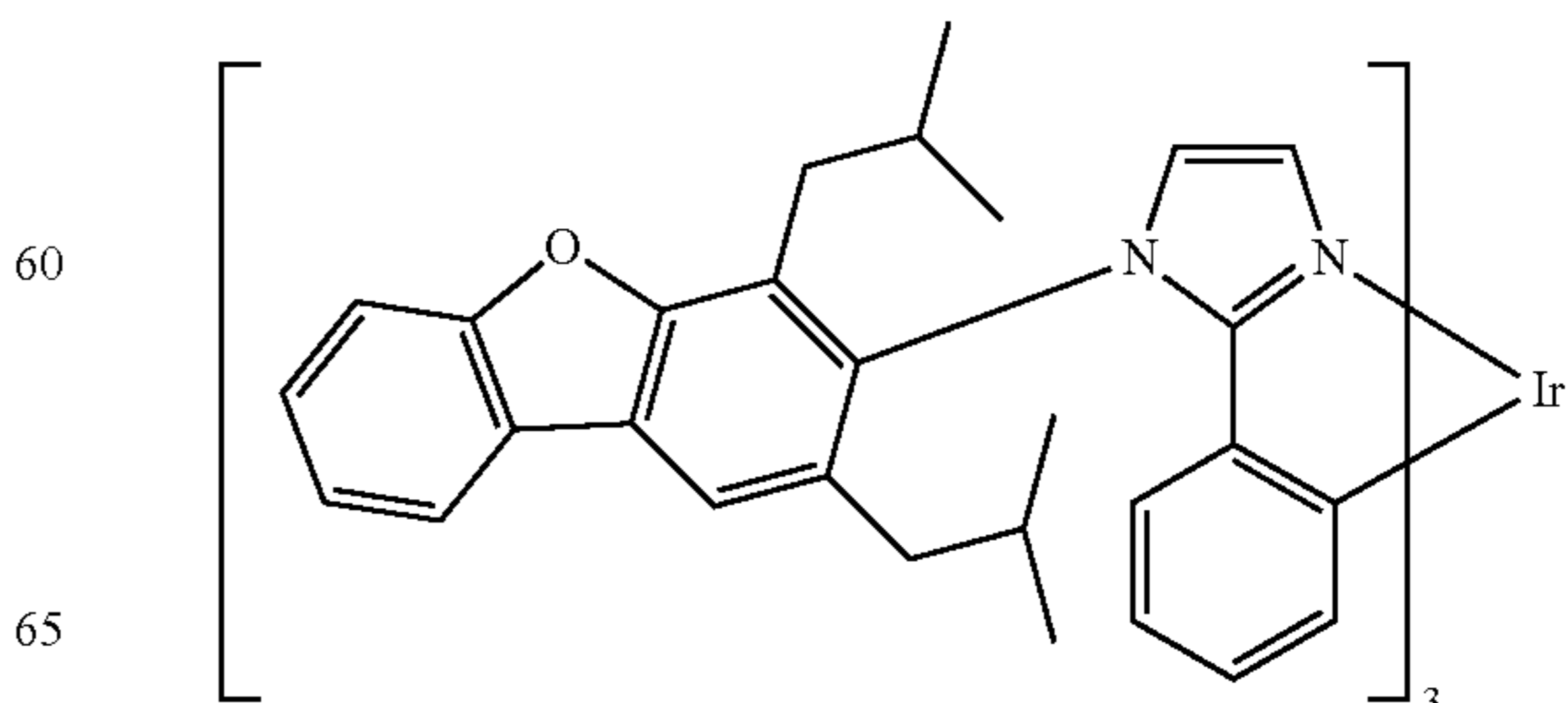
Compound 5
