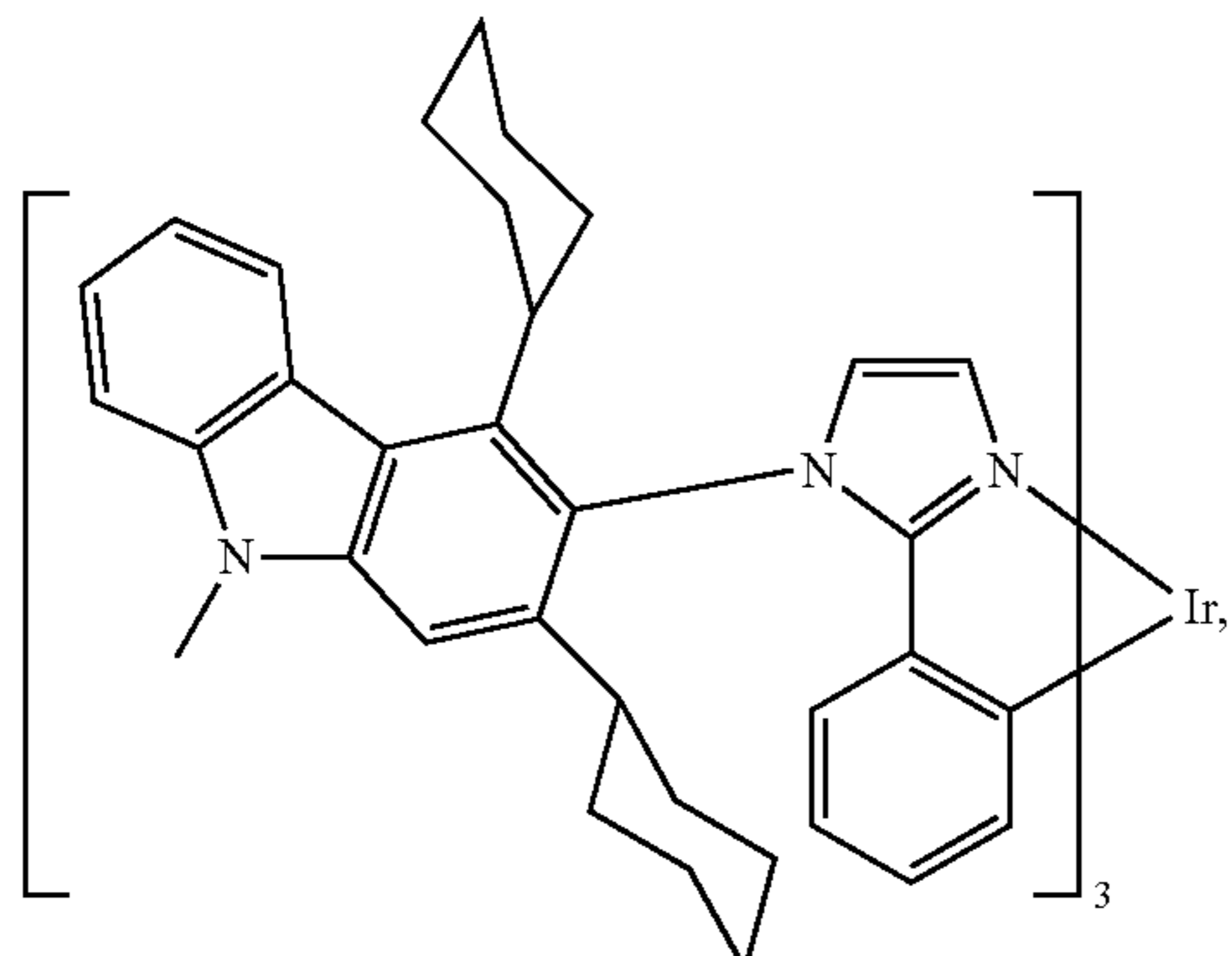
Compound 34
