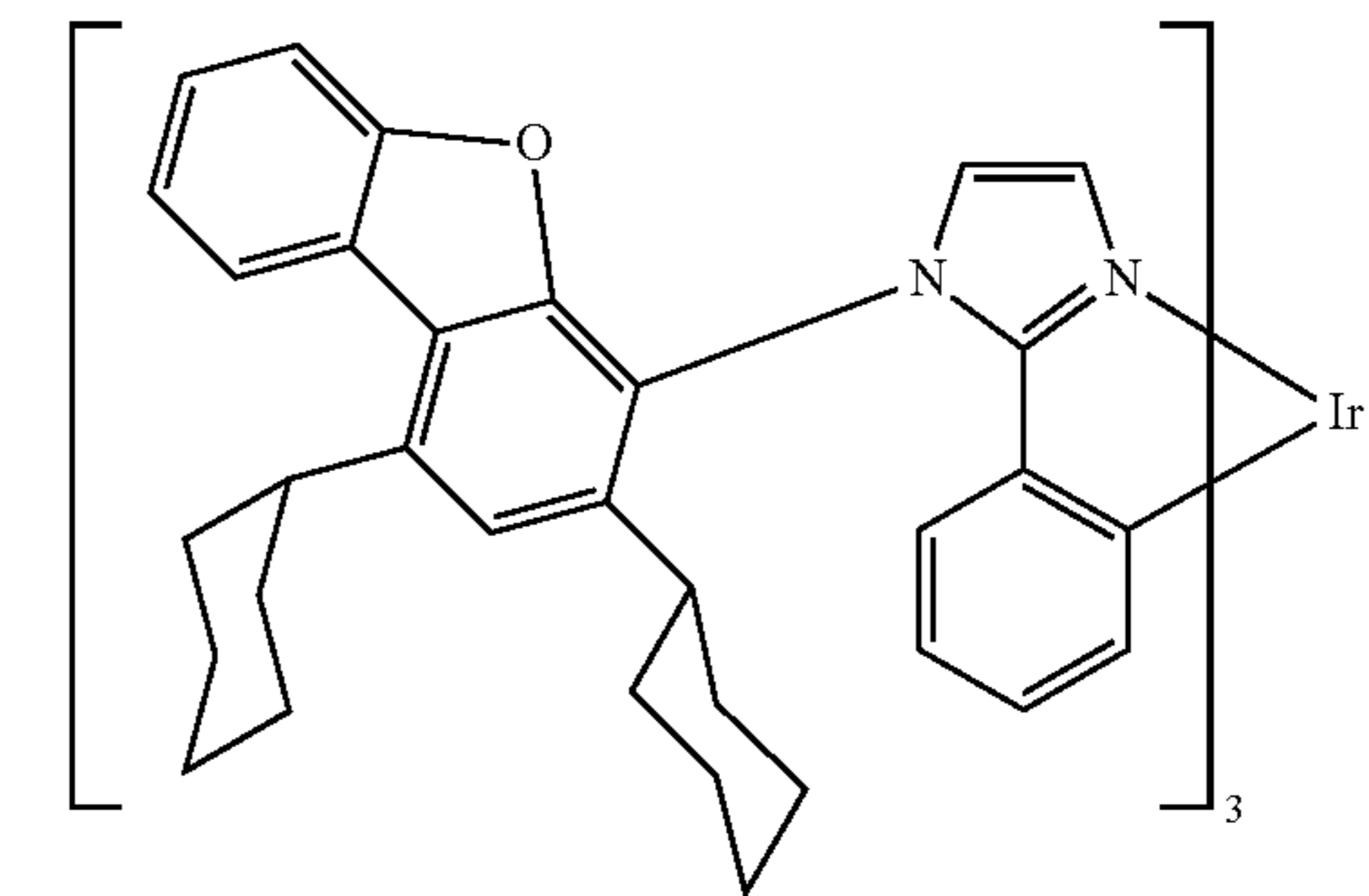
Compound 12
