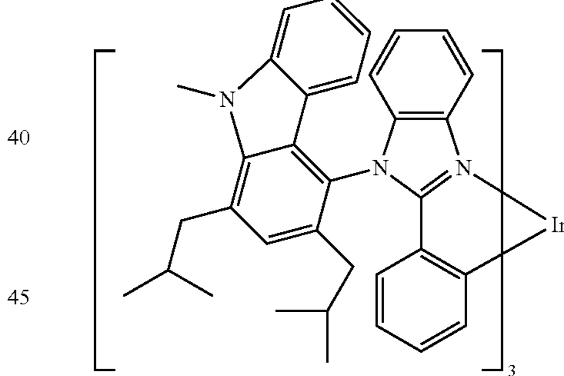
Compound 63
