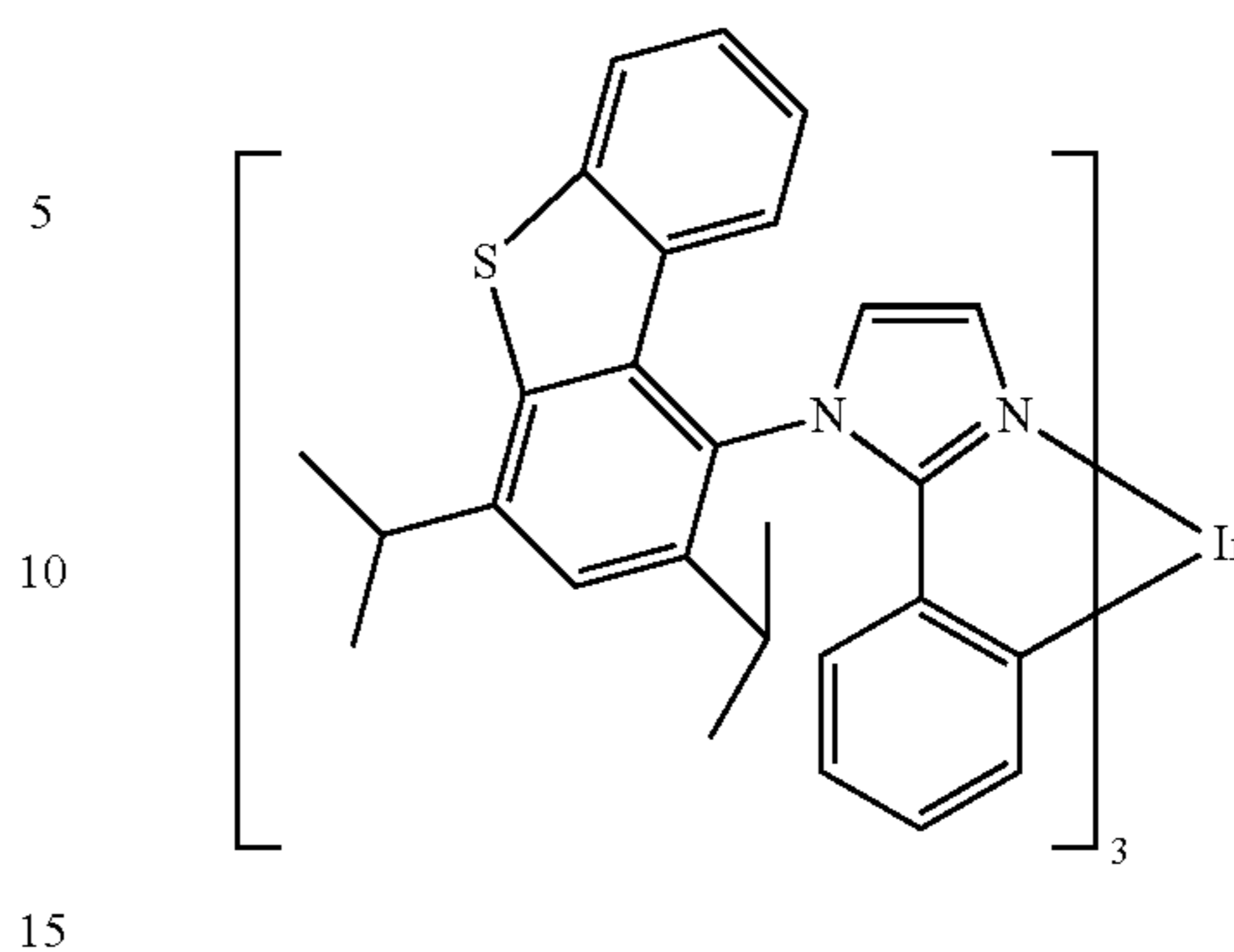
Compound 47
