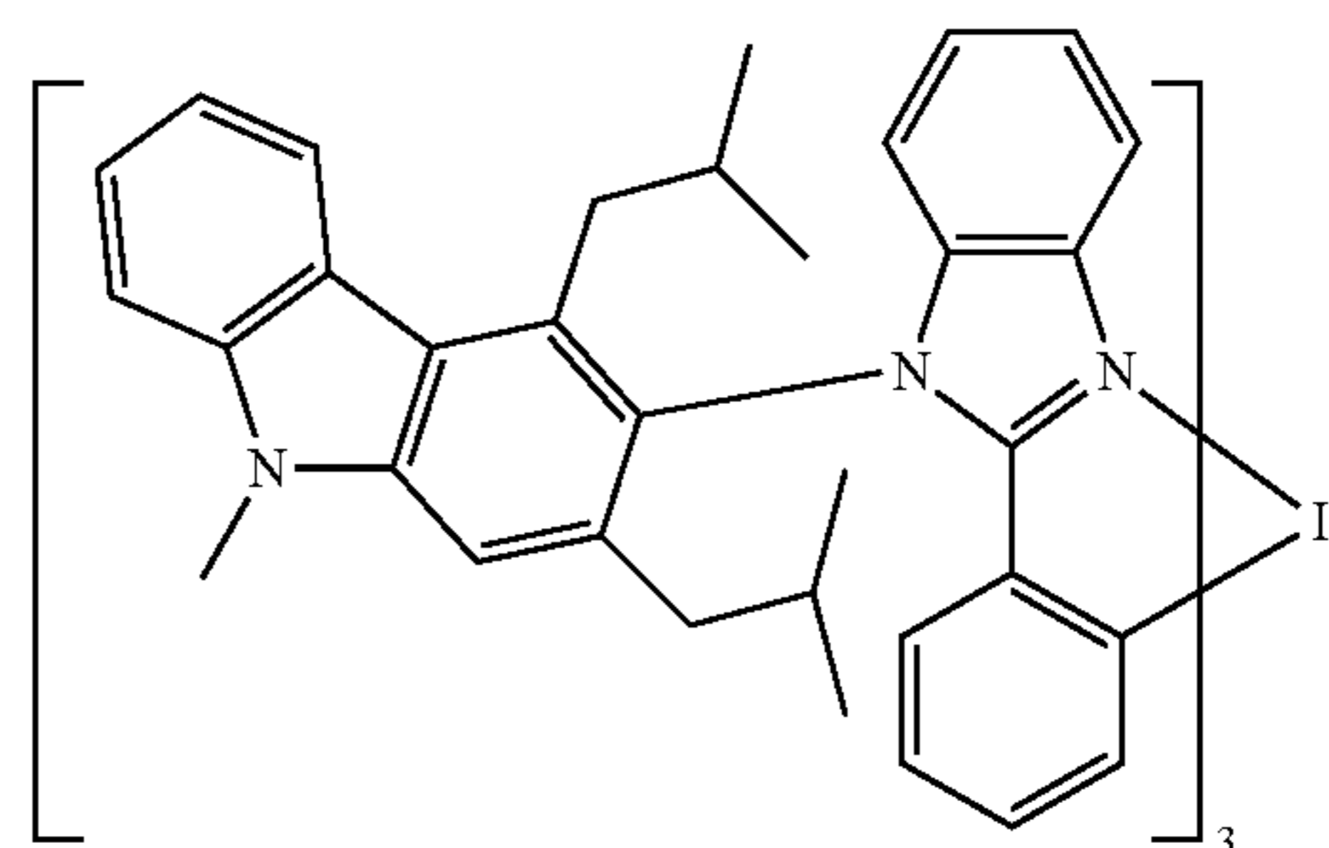
Compound 66
