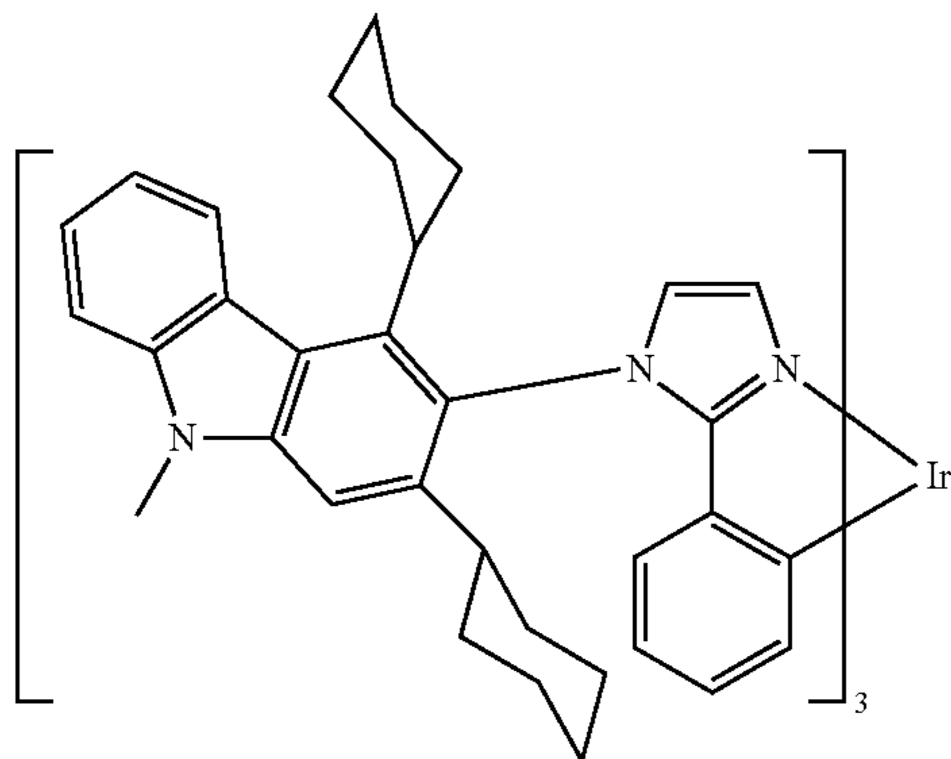
Compound 34
