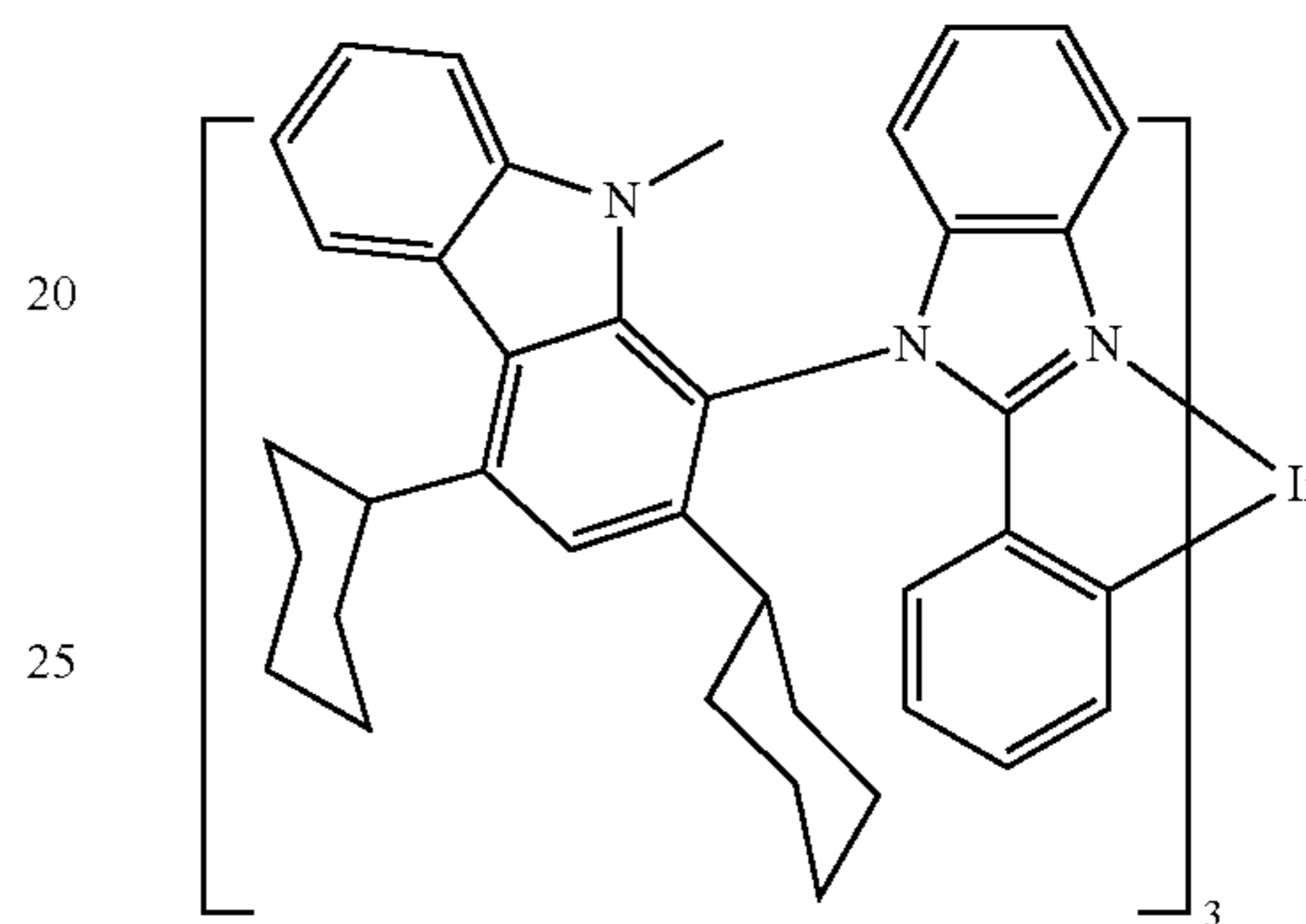
Compound 68
