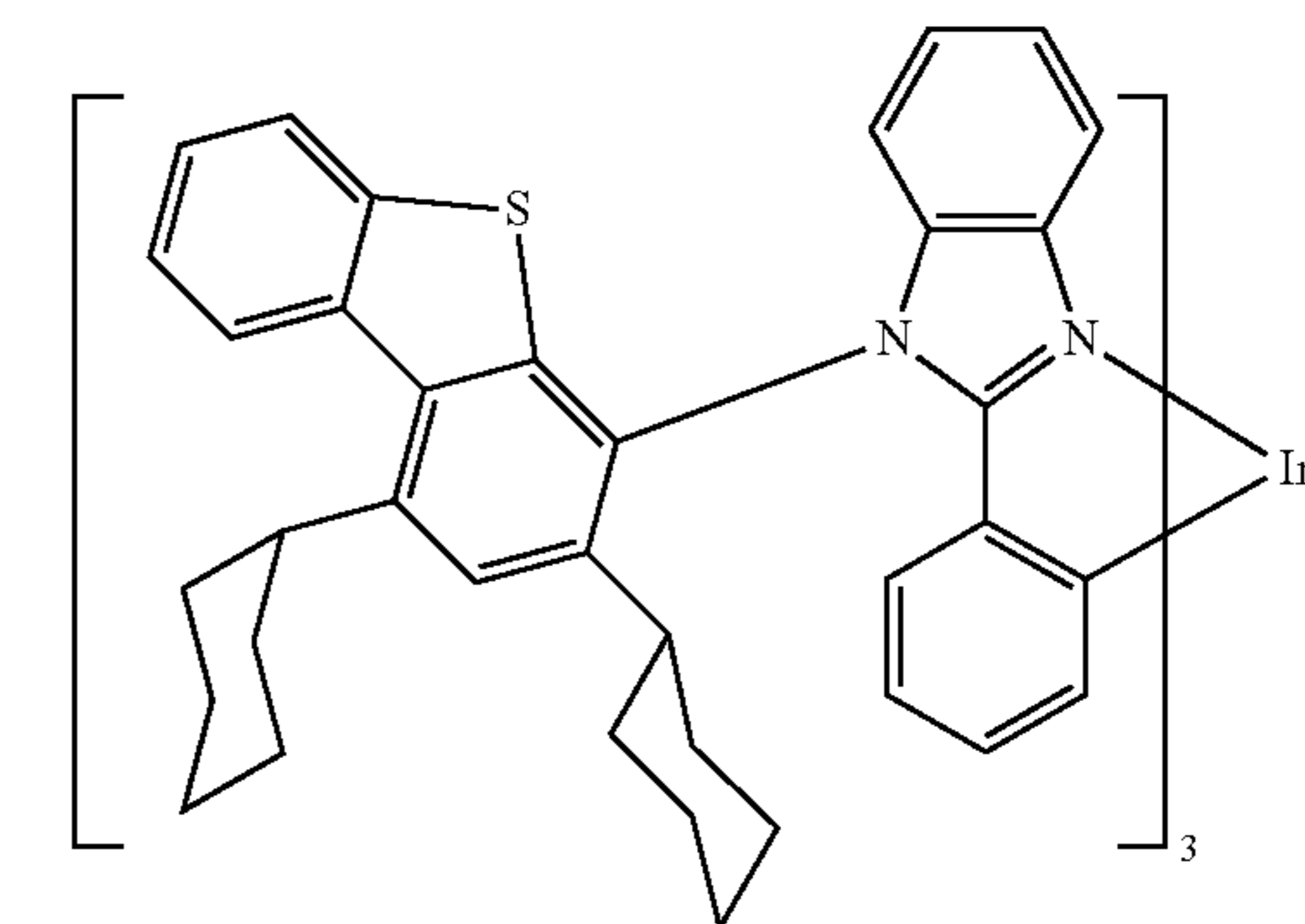
Compound 60
