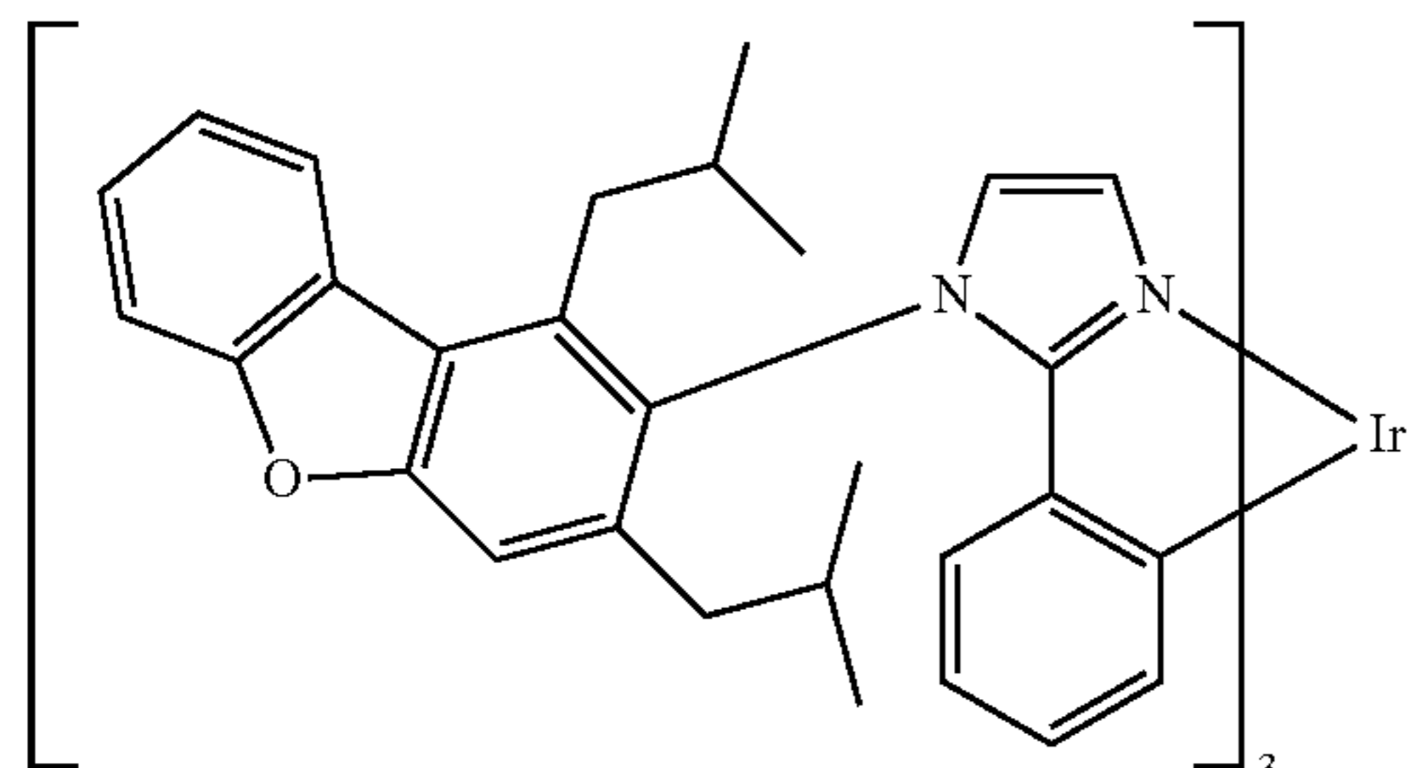
Compound 7
