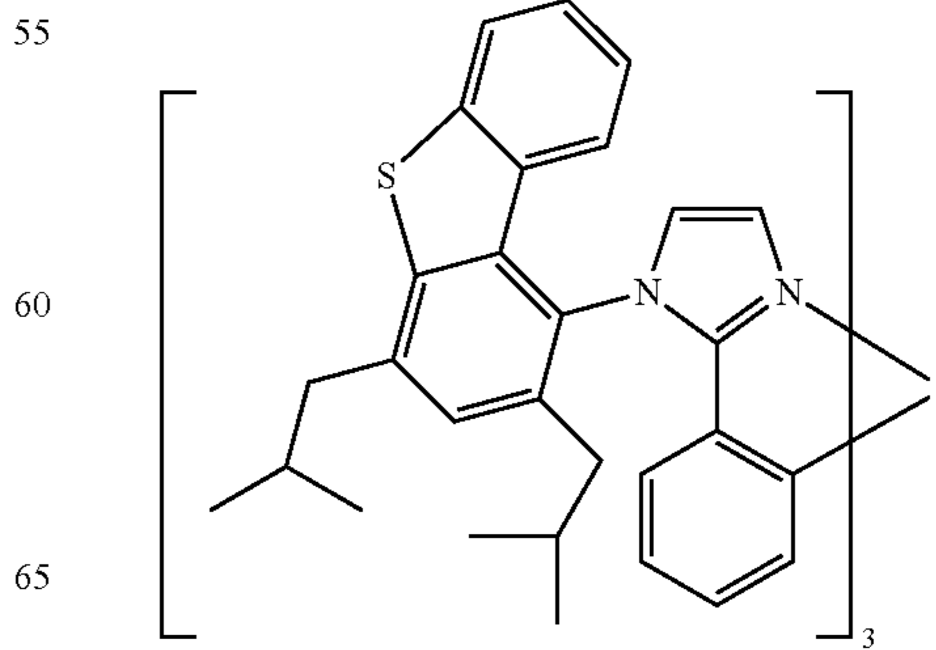
Compound 14
