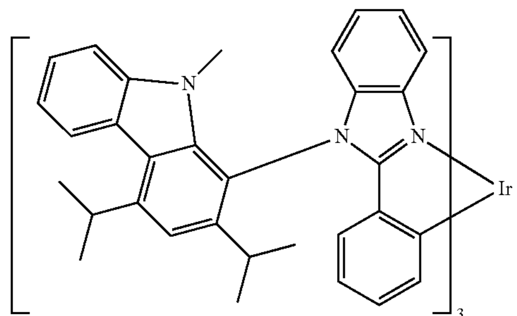
Compound 64
