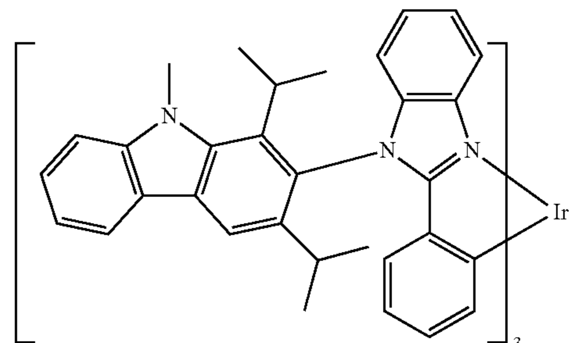
Compound 62
