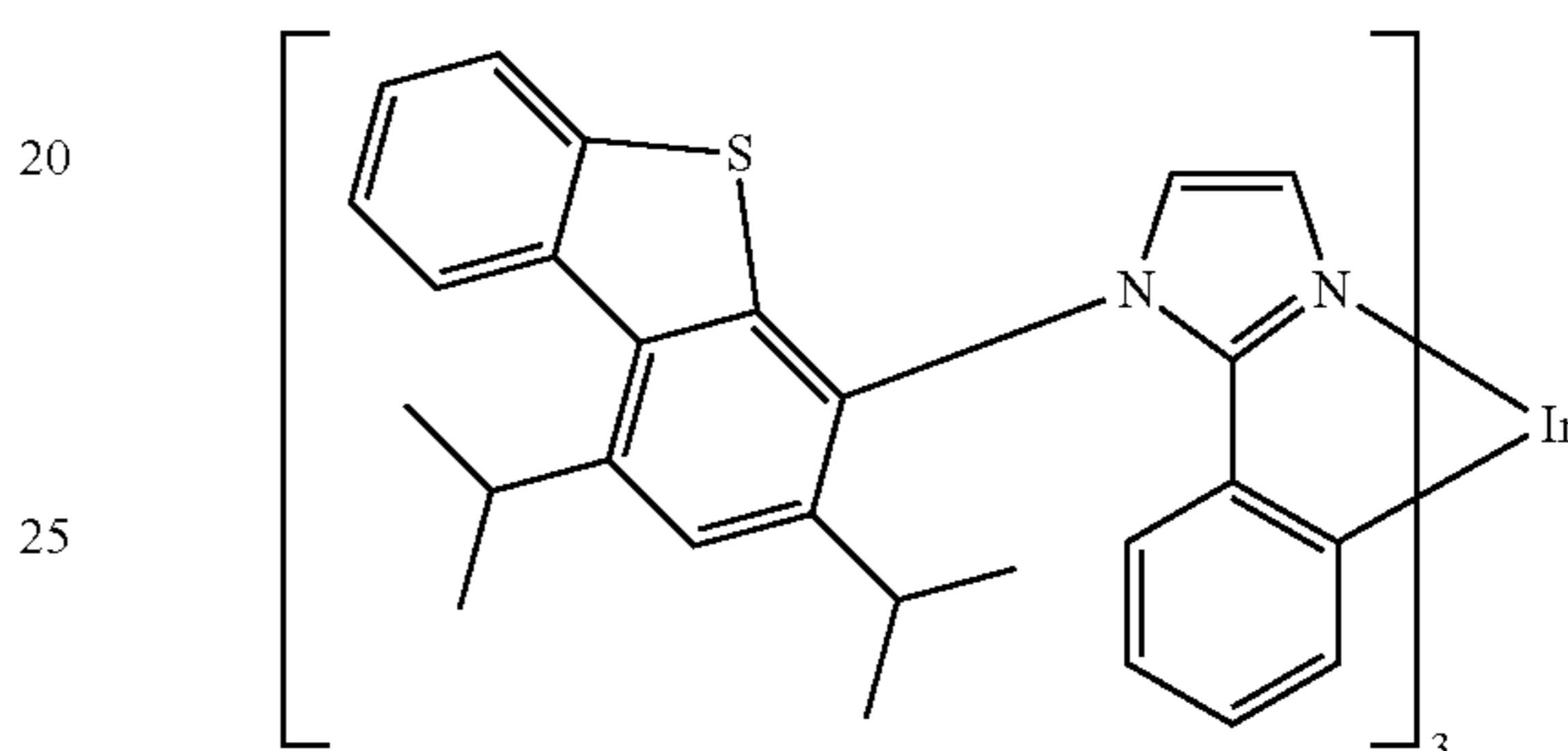
Compound 17
