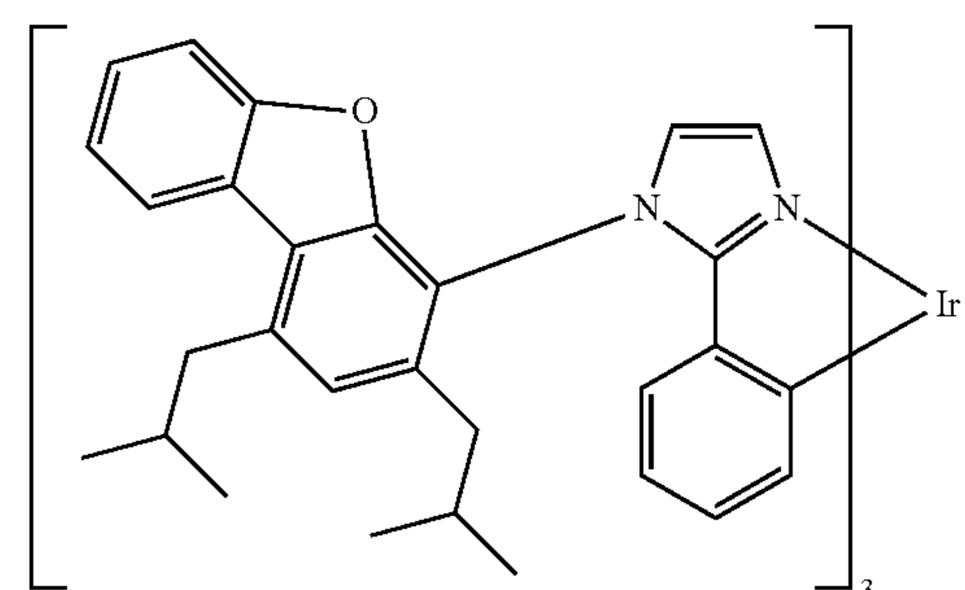
Compound 9
