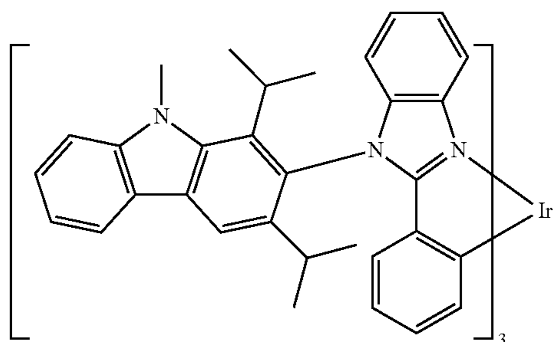
Compound 61
