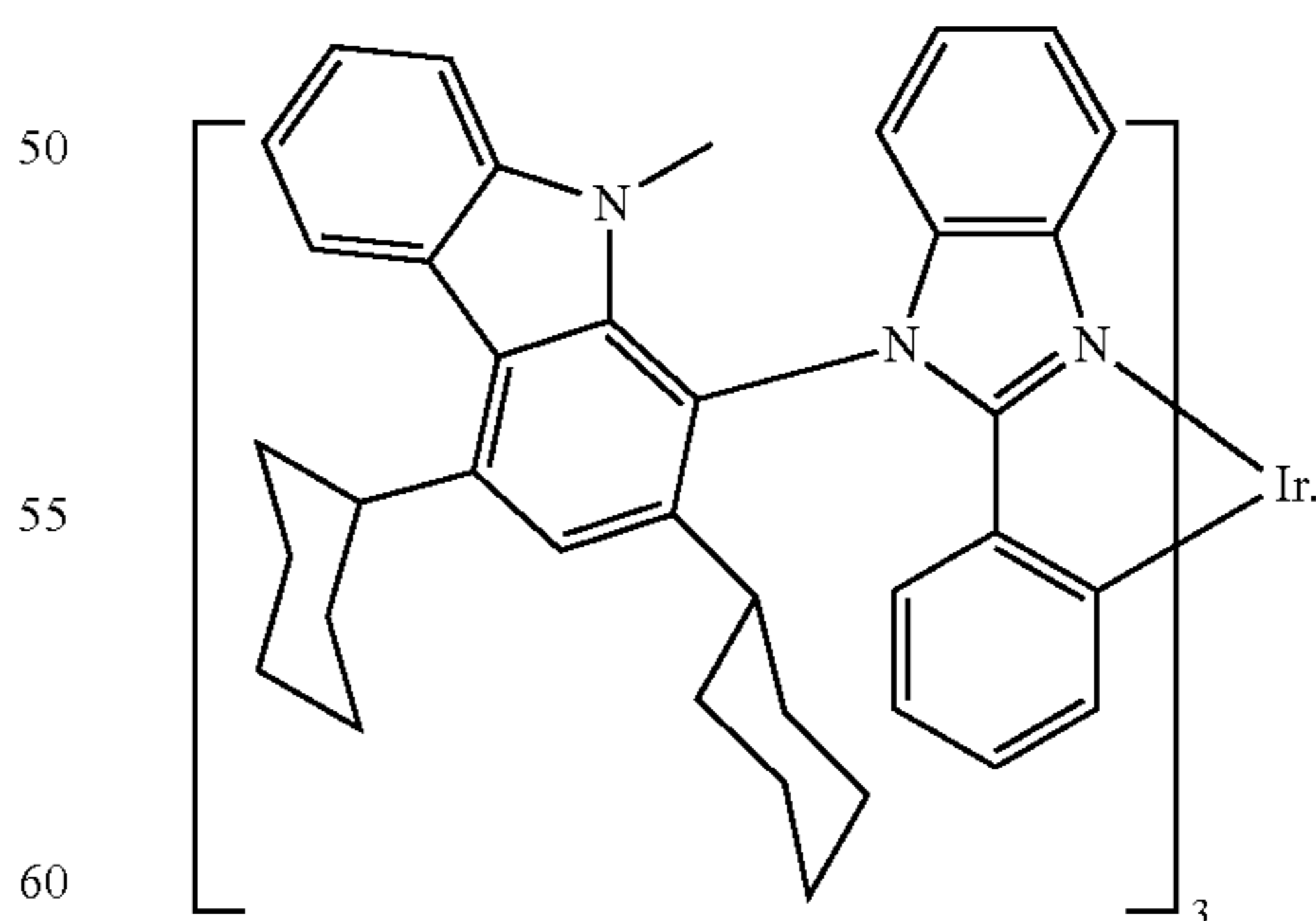
Compound 68
