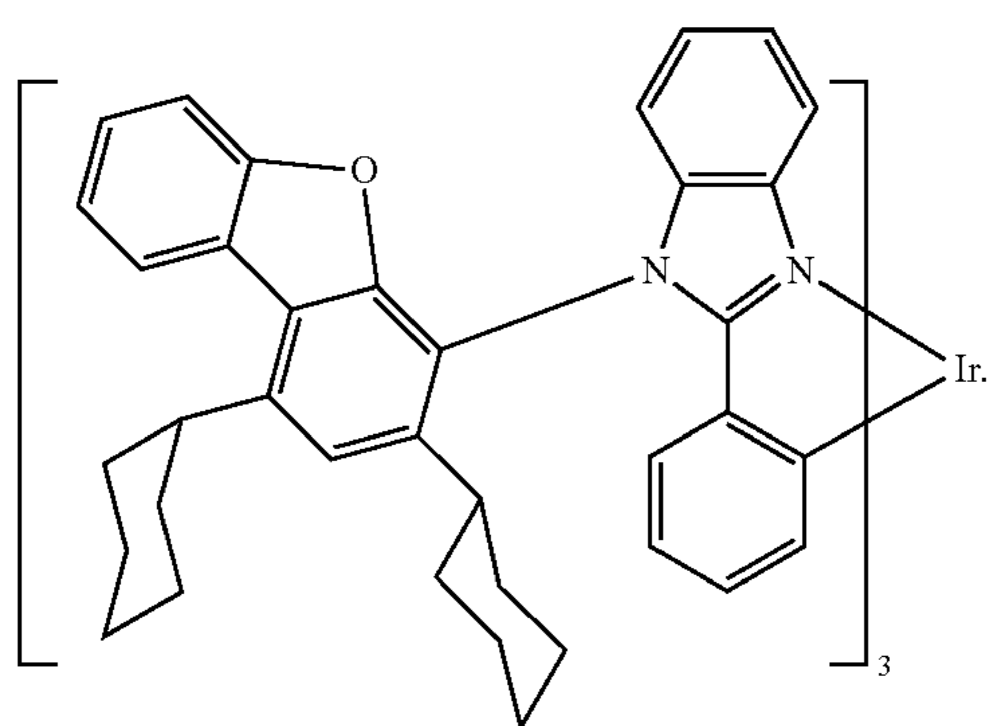
Compound 48
