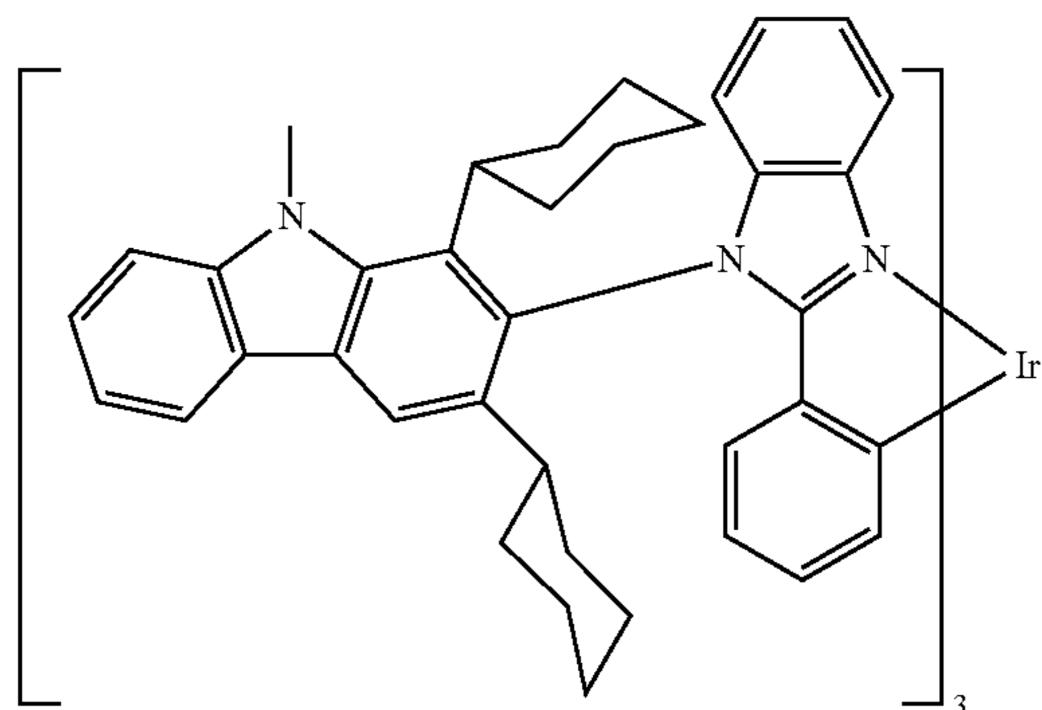
Compound 69
