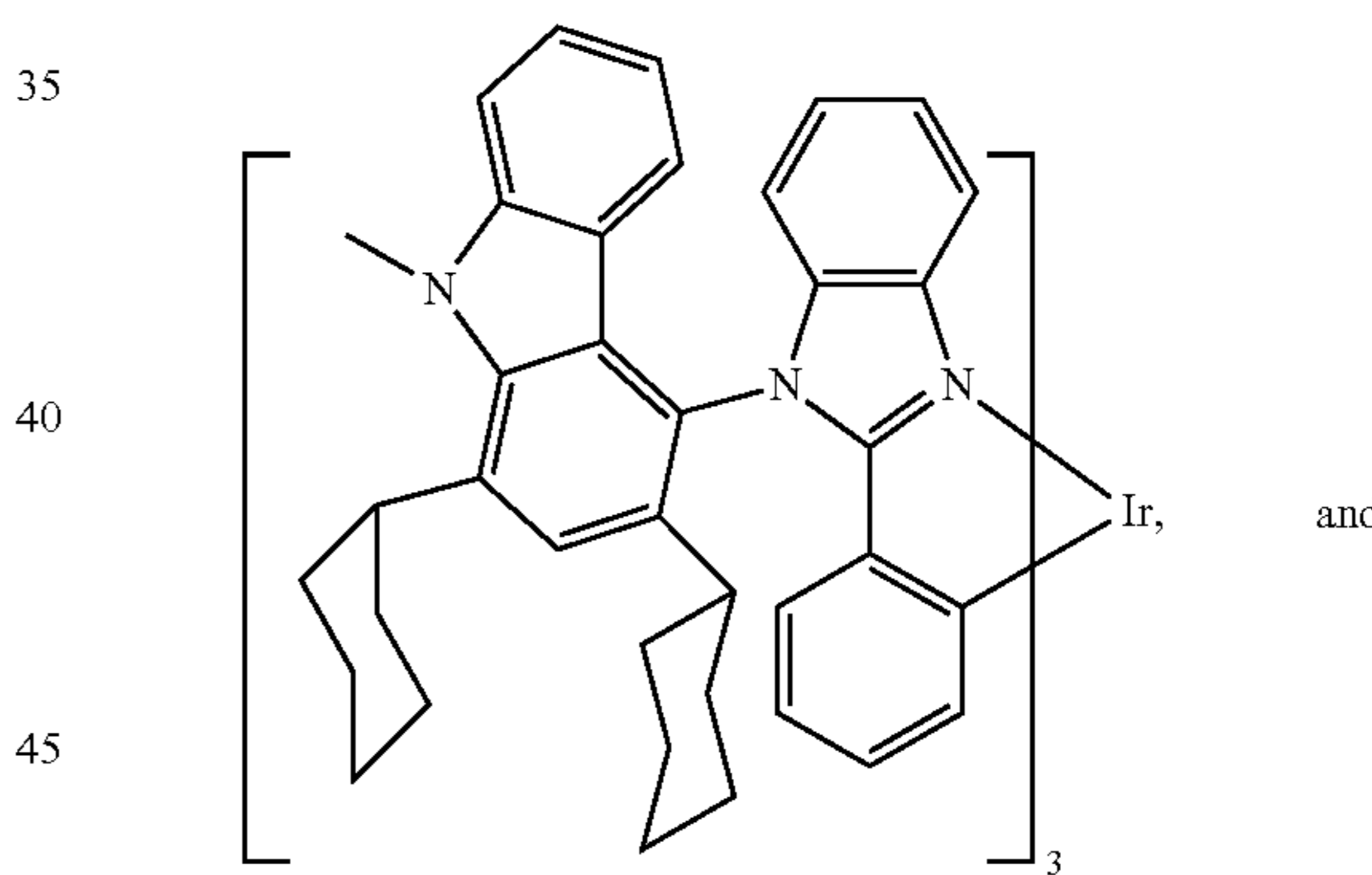
Compound 72
