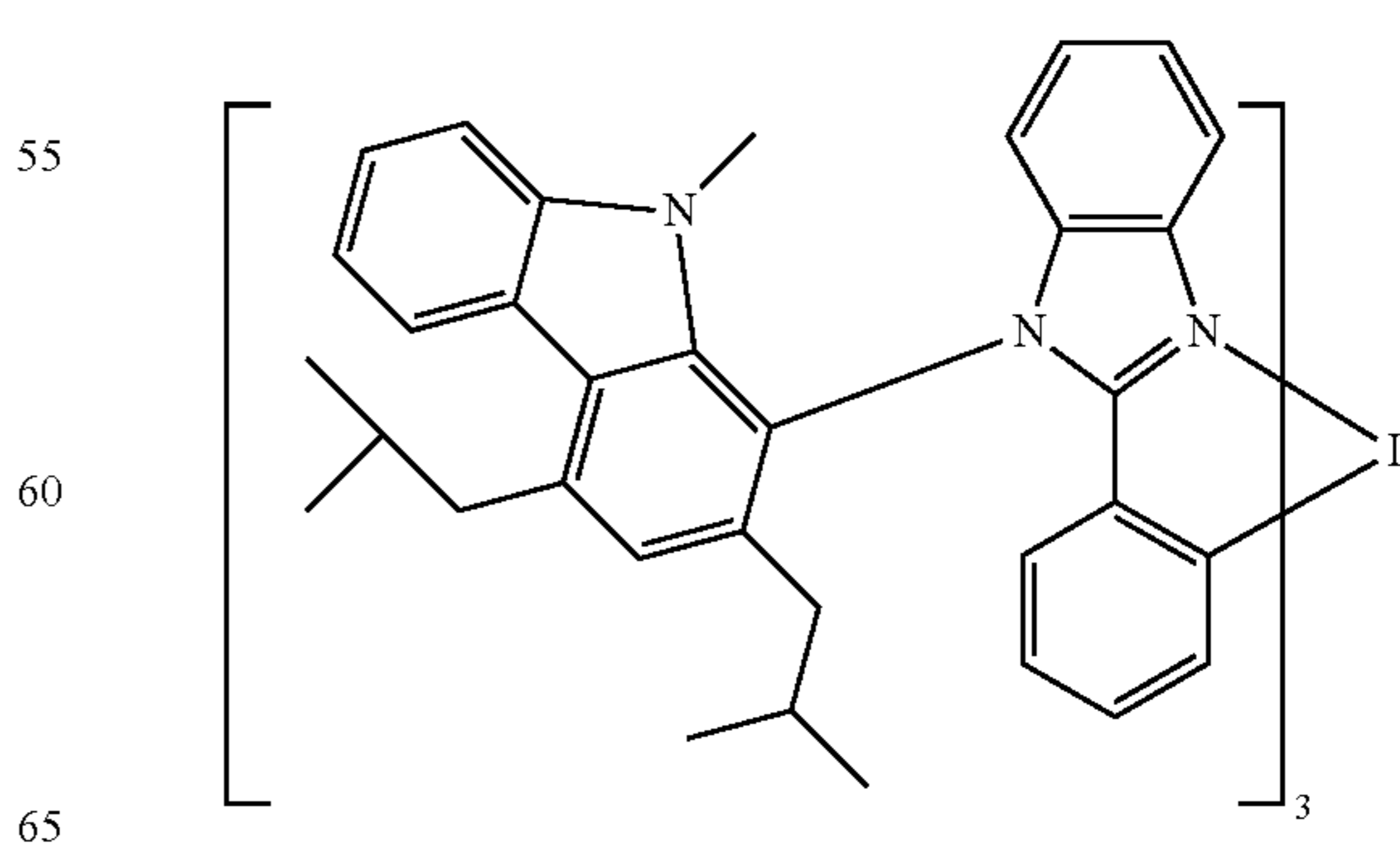
Compound 68
