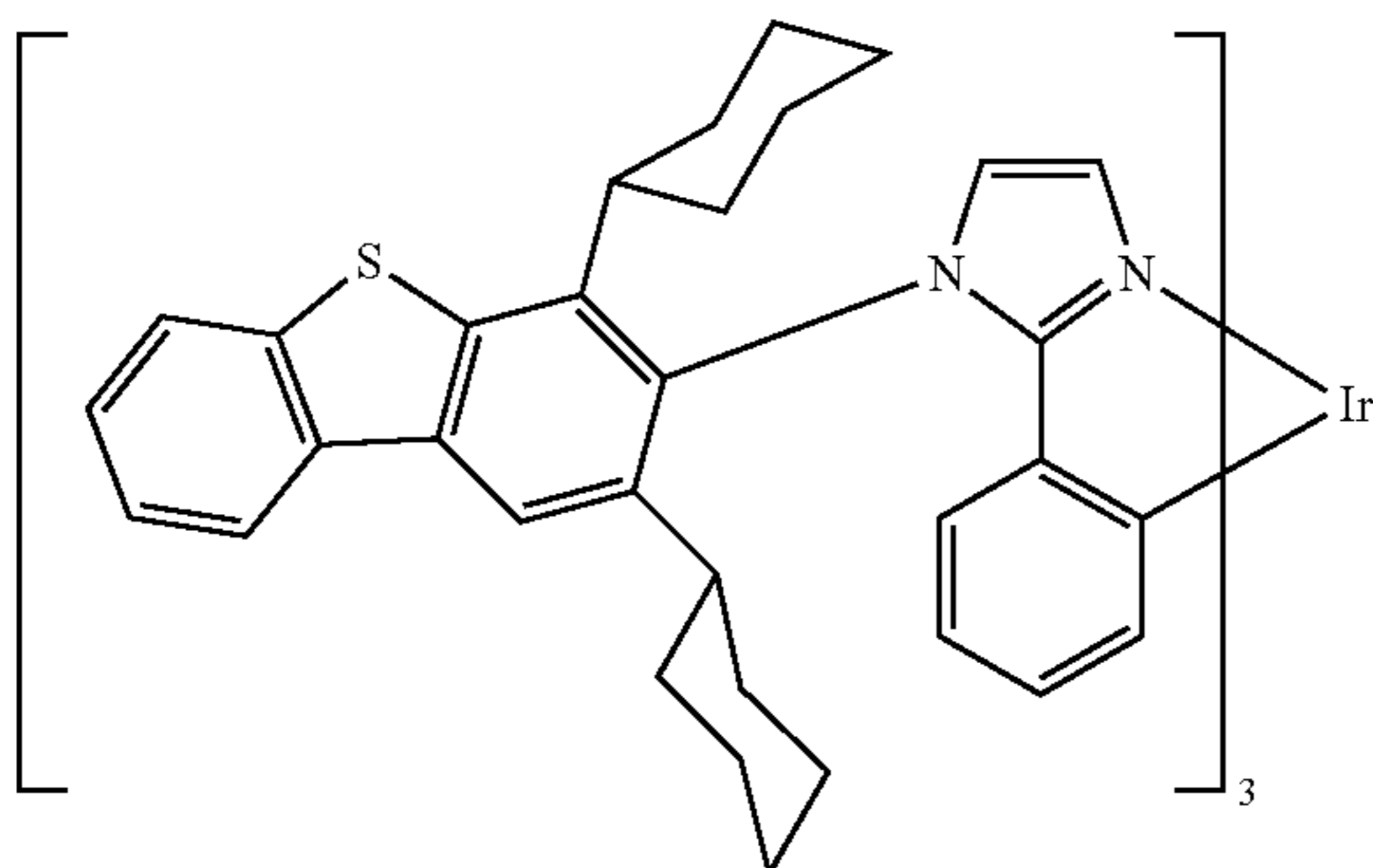
Compound 21
