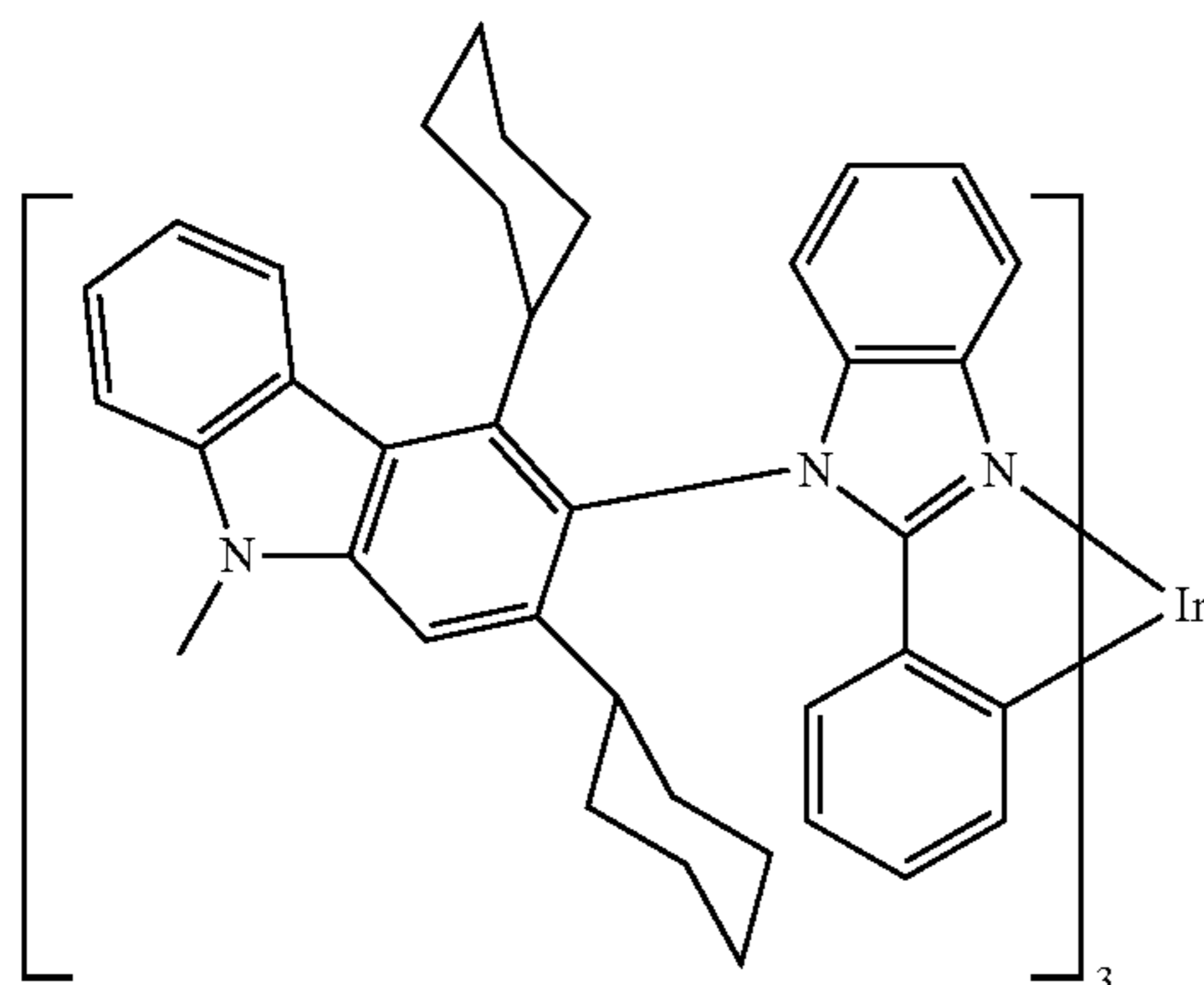
Compound 70
