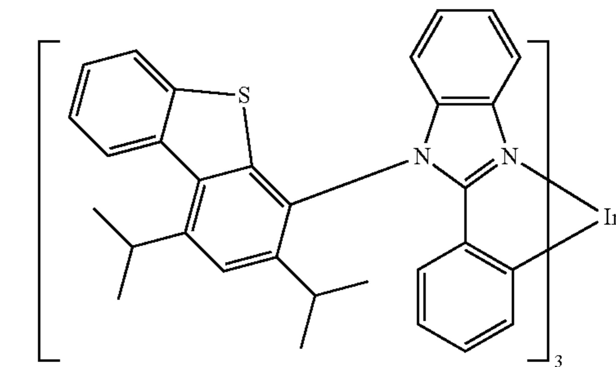
Compound 52
