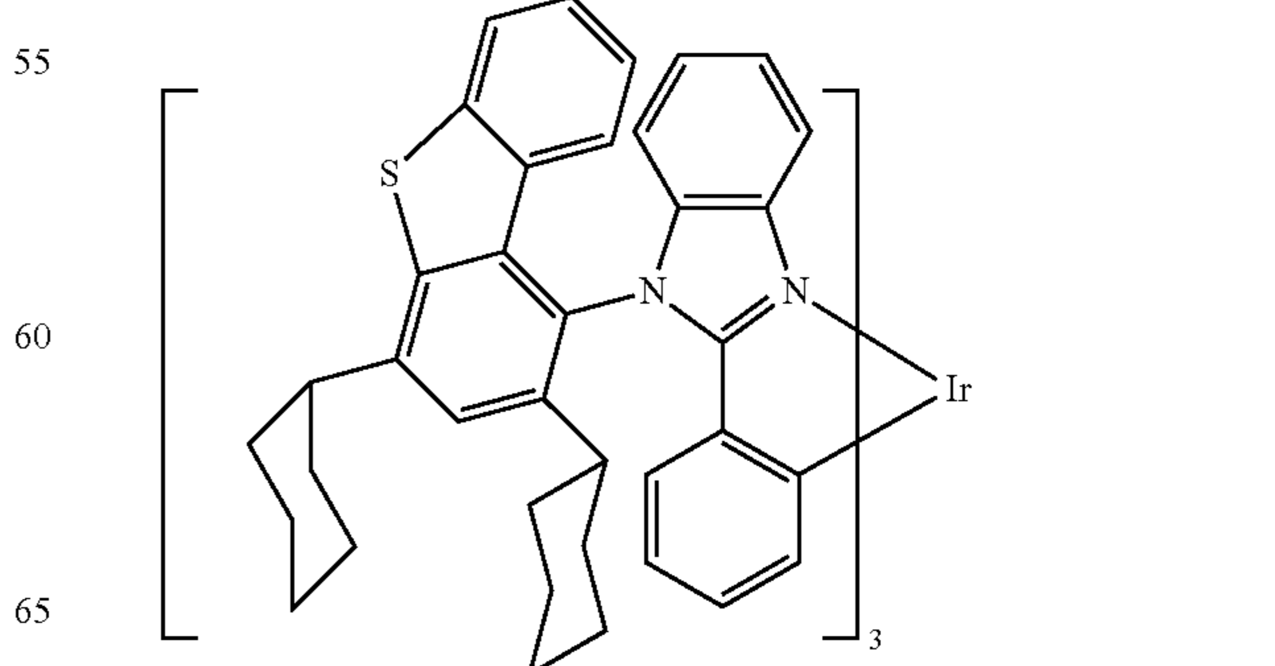
Compound 59
