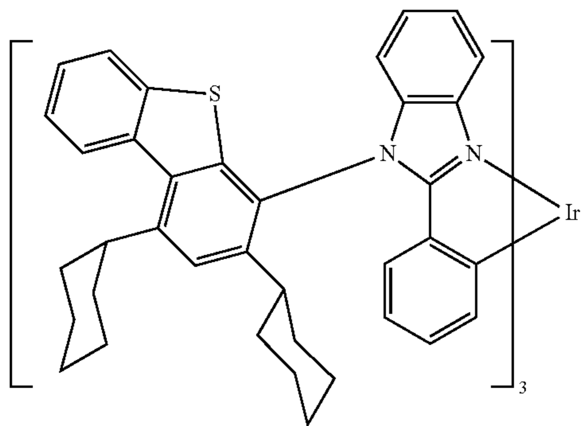
Compound 61
