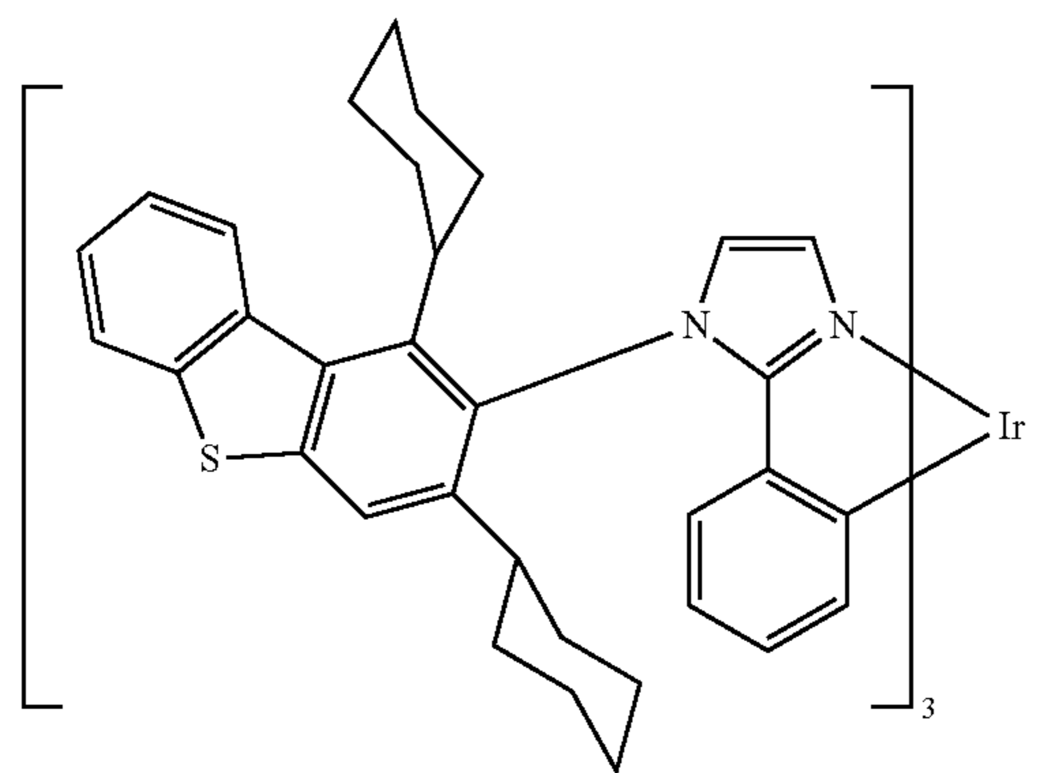
Compound 22
