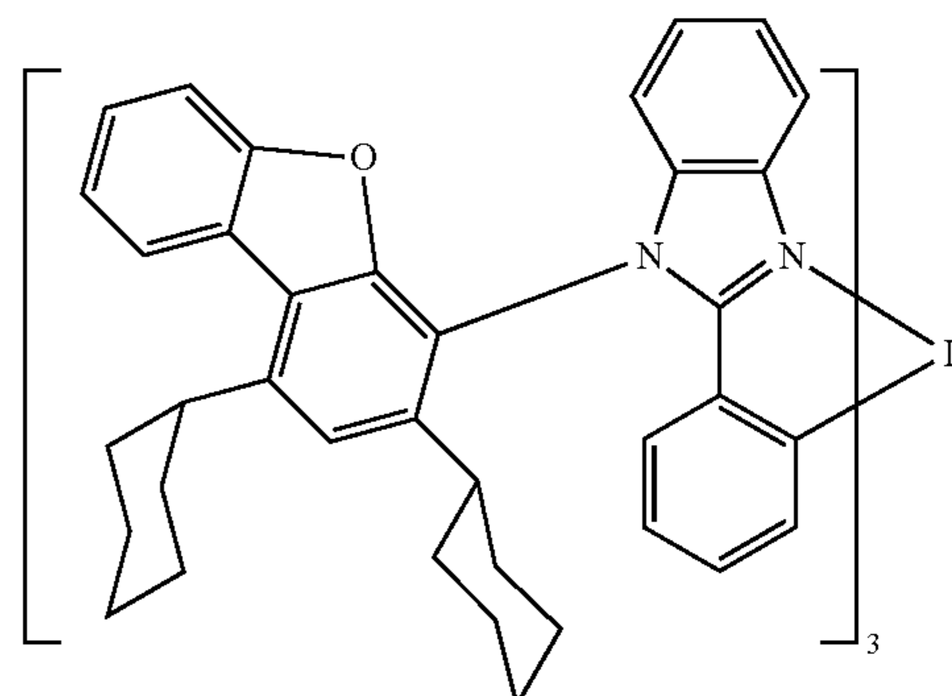
-continued Compound 47
