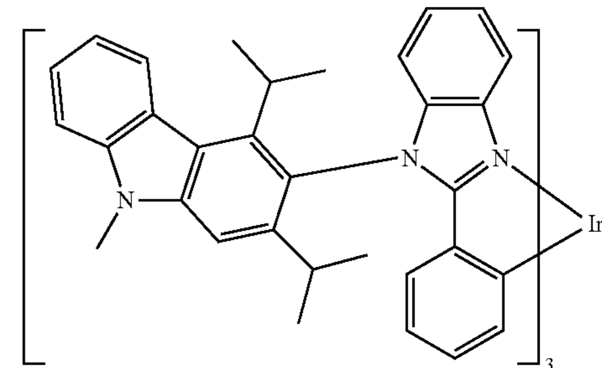
Compound 63
