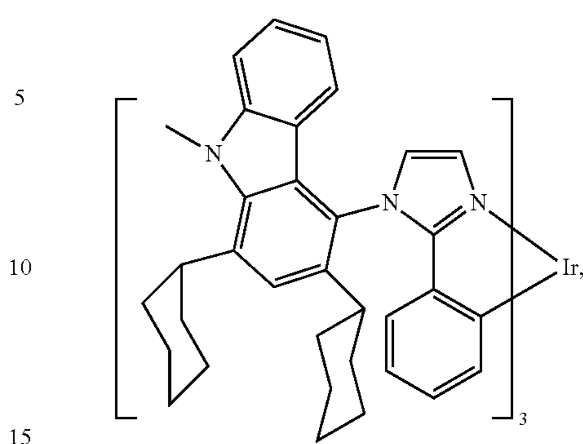
Compound 35
