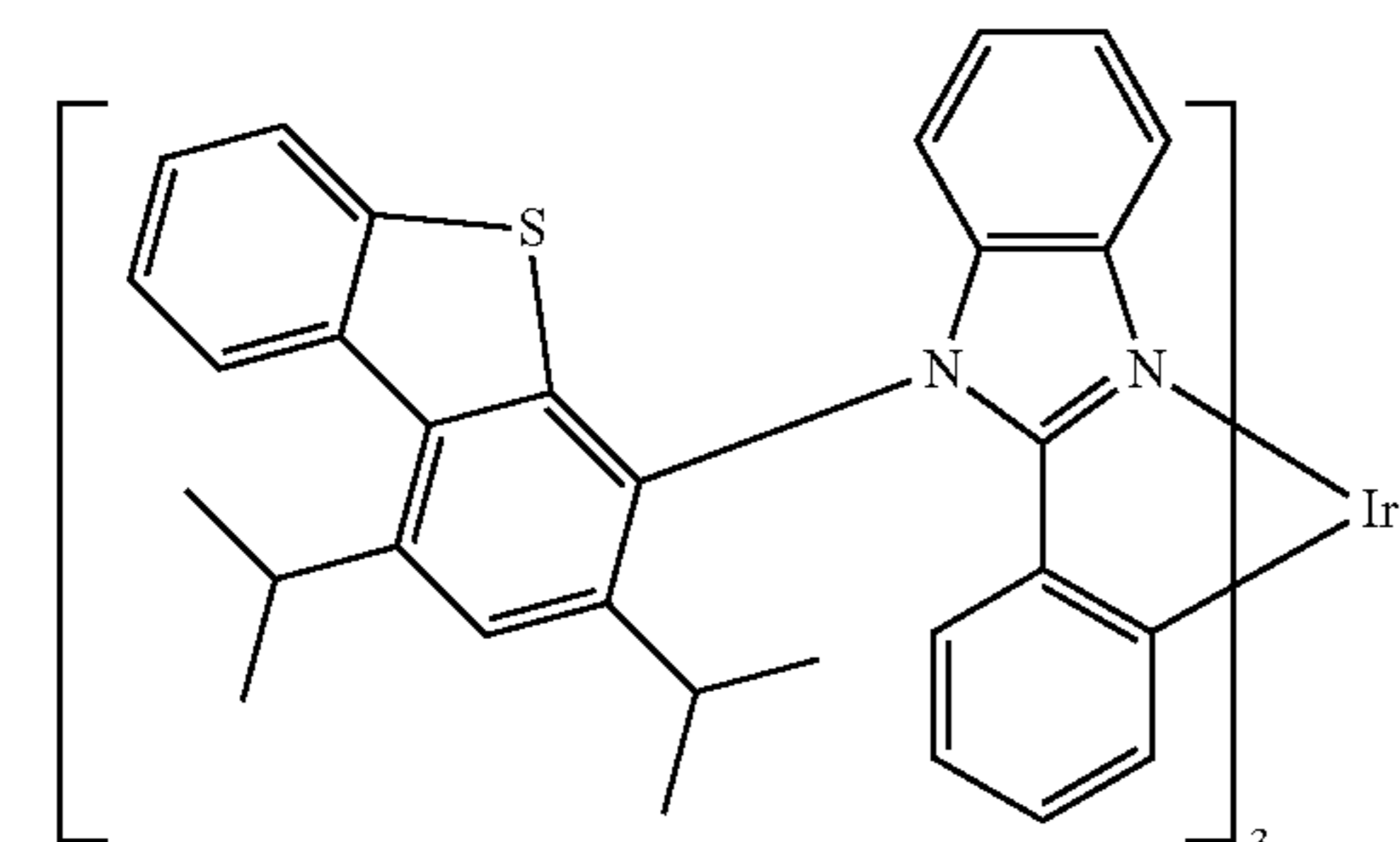
Compound 53
