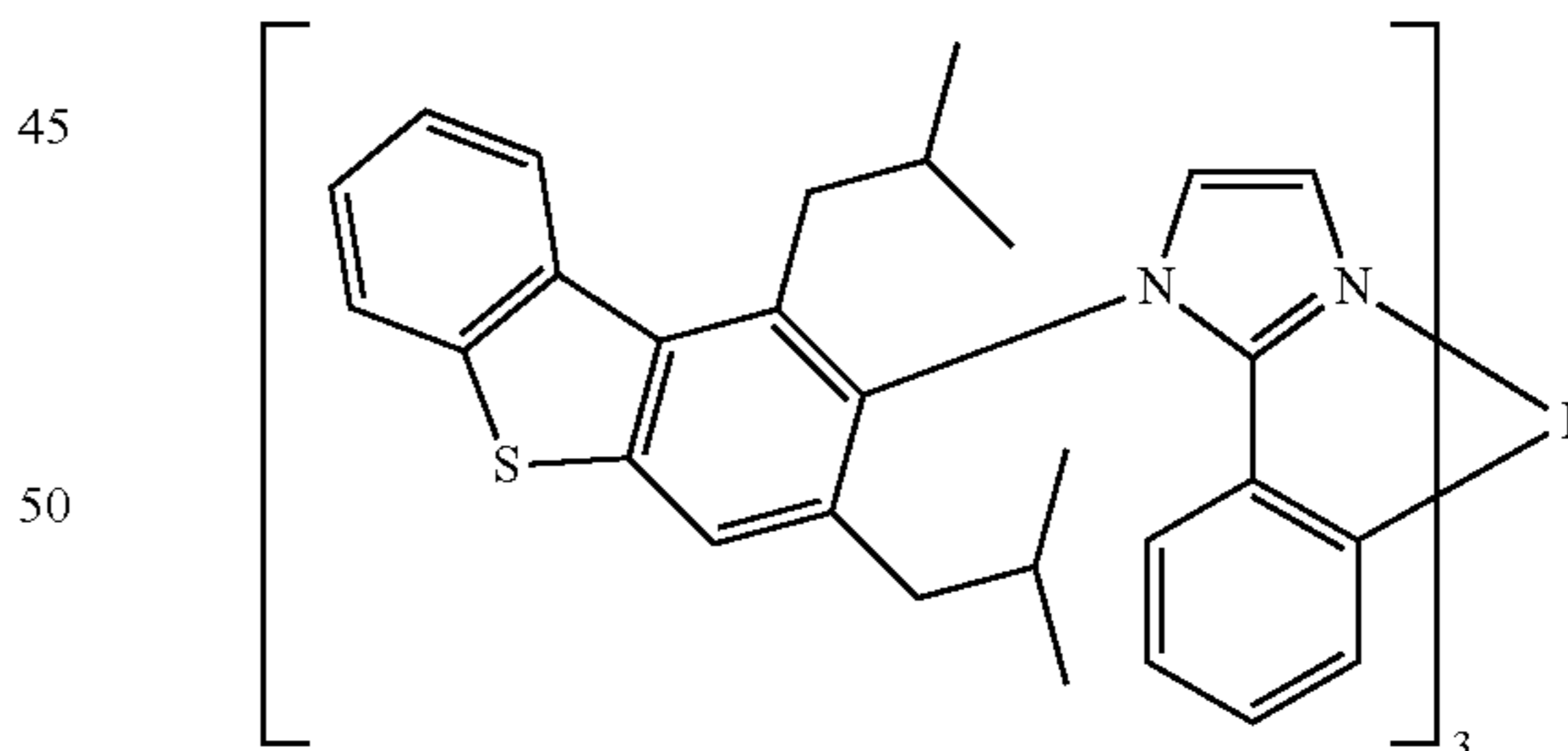
Compound 19
