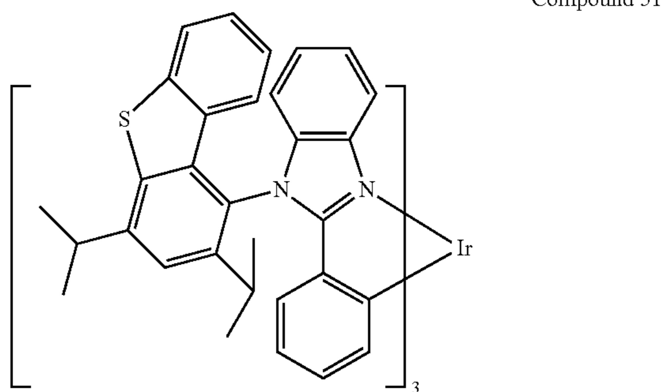
Compound 52
