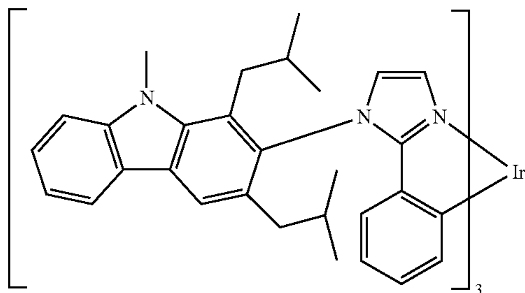
Compound 29
