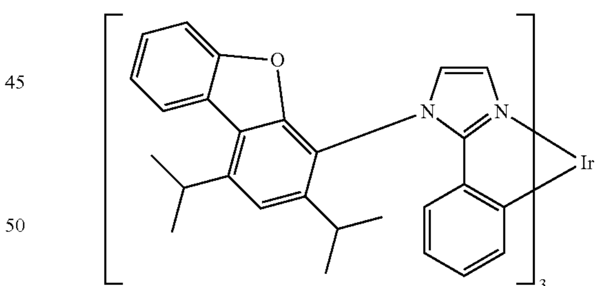
Compound 4
