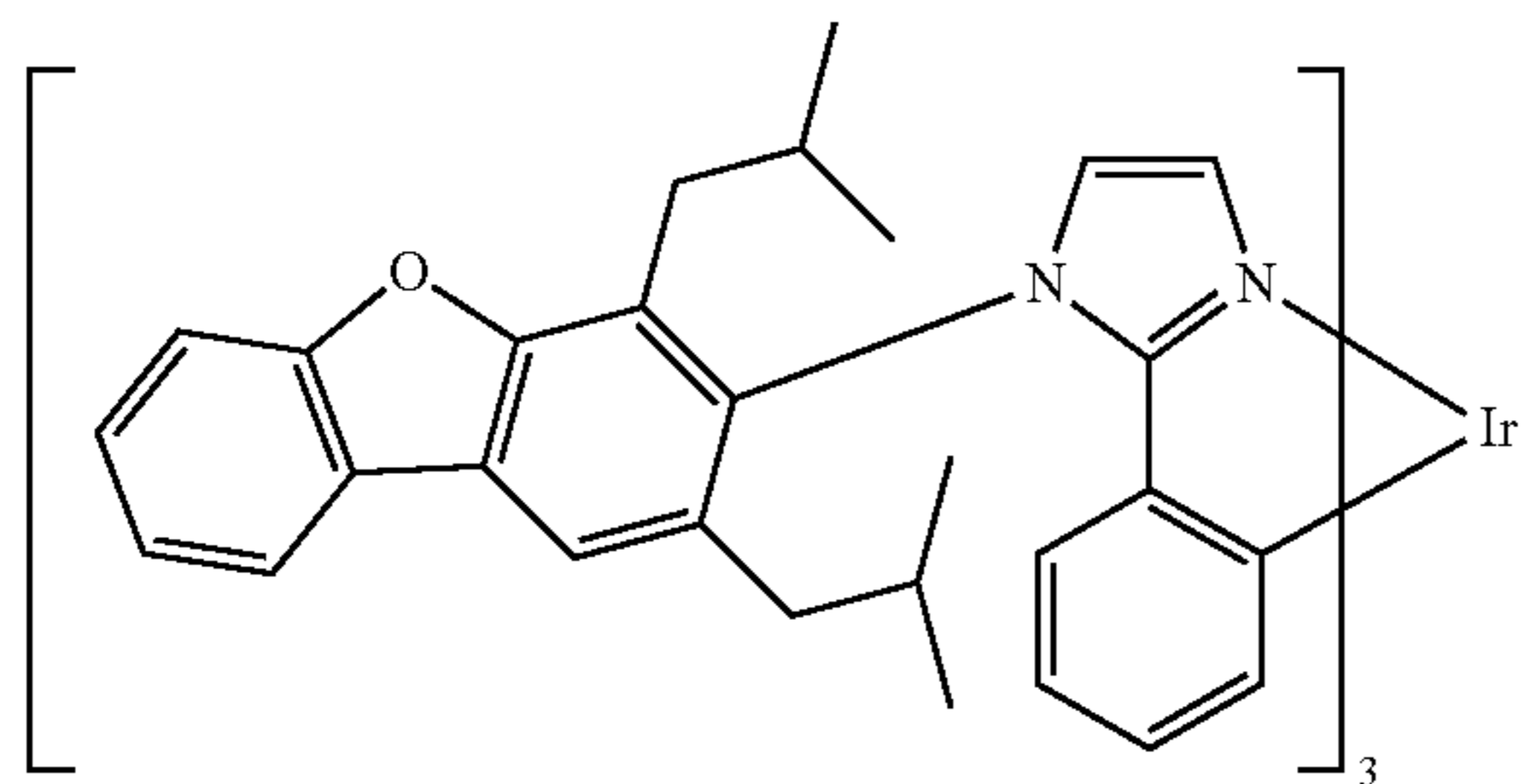
Compound 6
