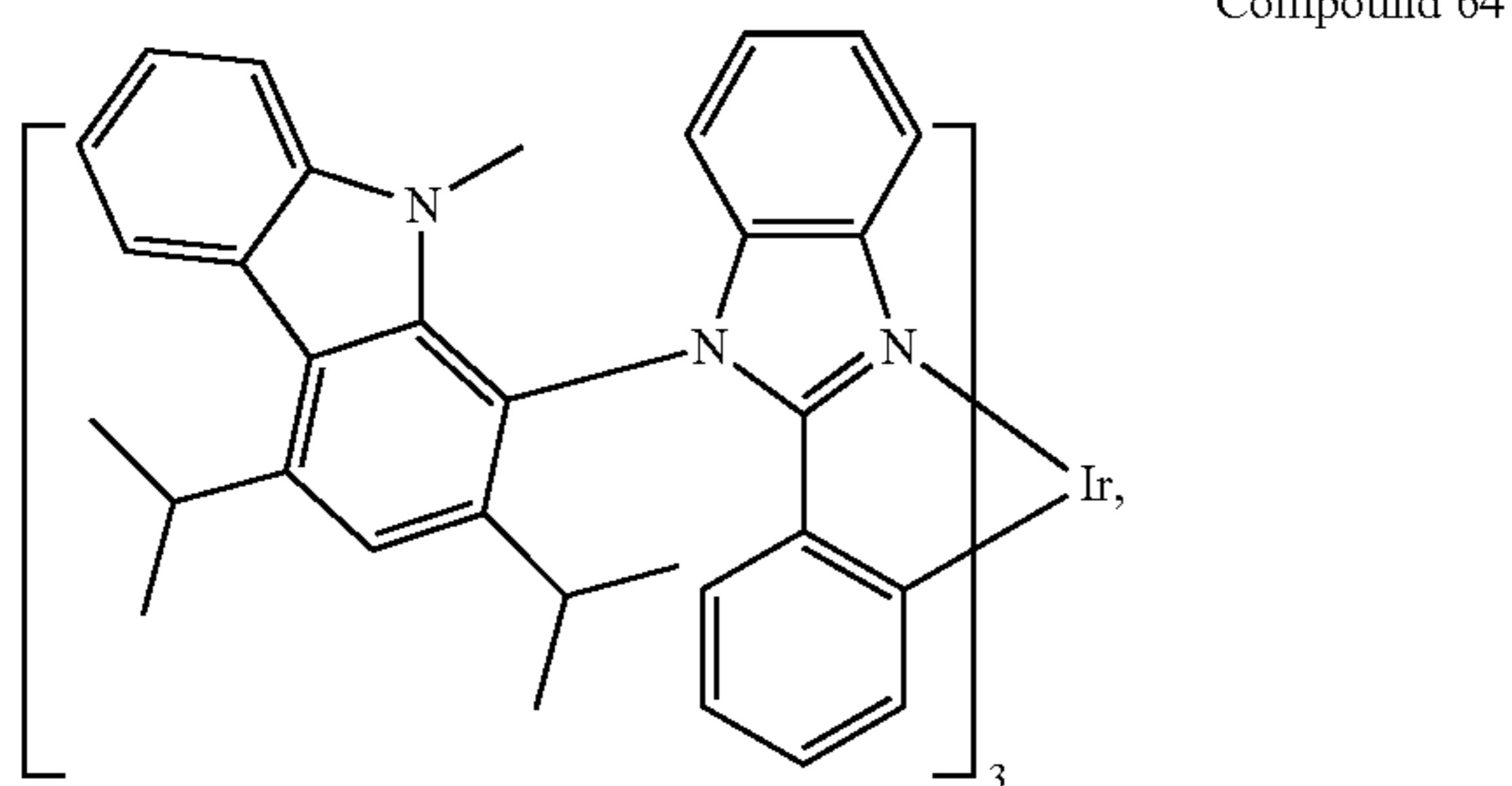
Compound 65
