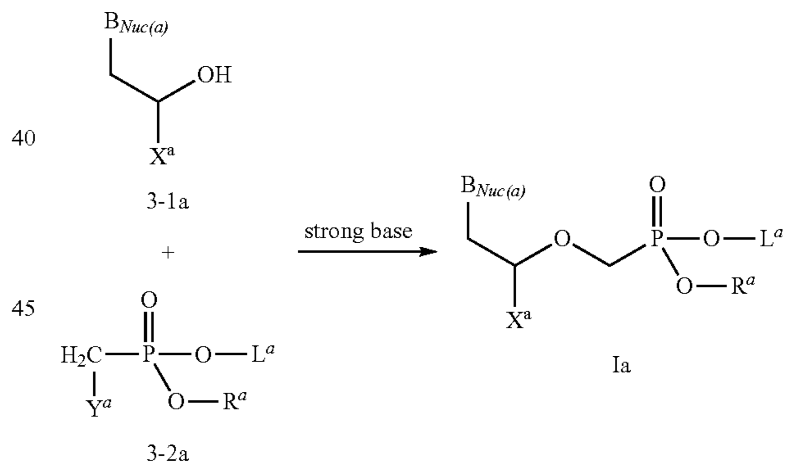
Scheme 3a
