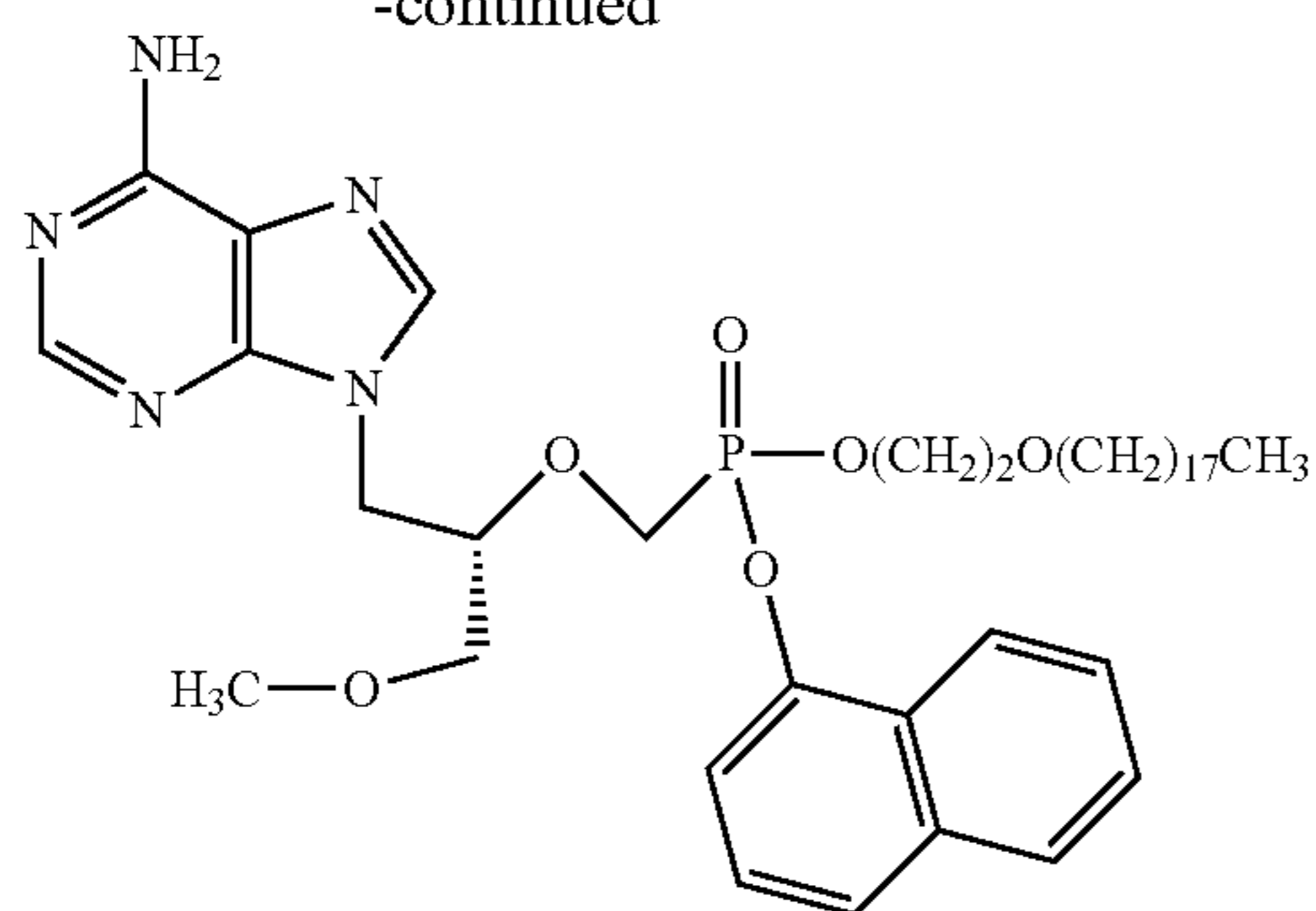
Npt-ODE-(S)-MPMPA
