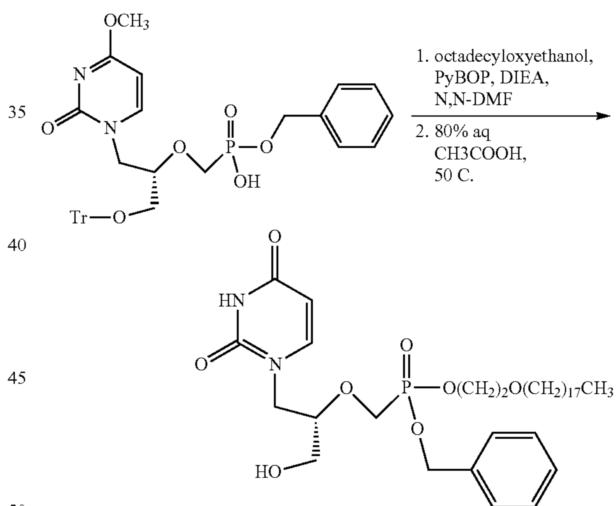
Bn-ODE-(S)-HPMPU
