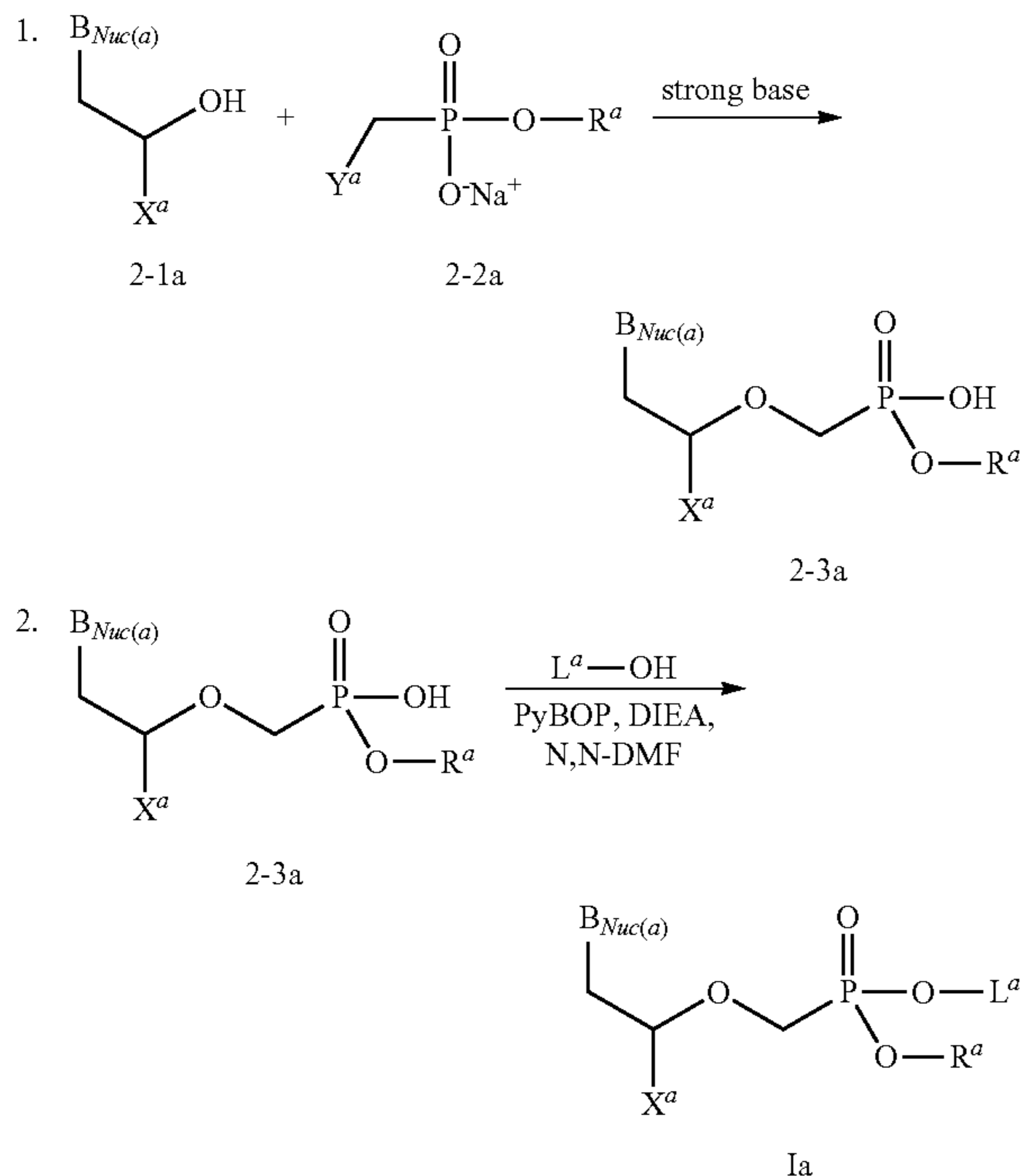
Scheme 2-1a
