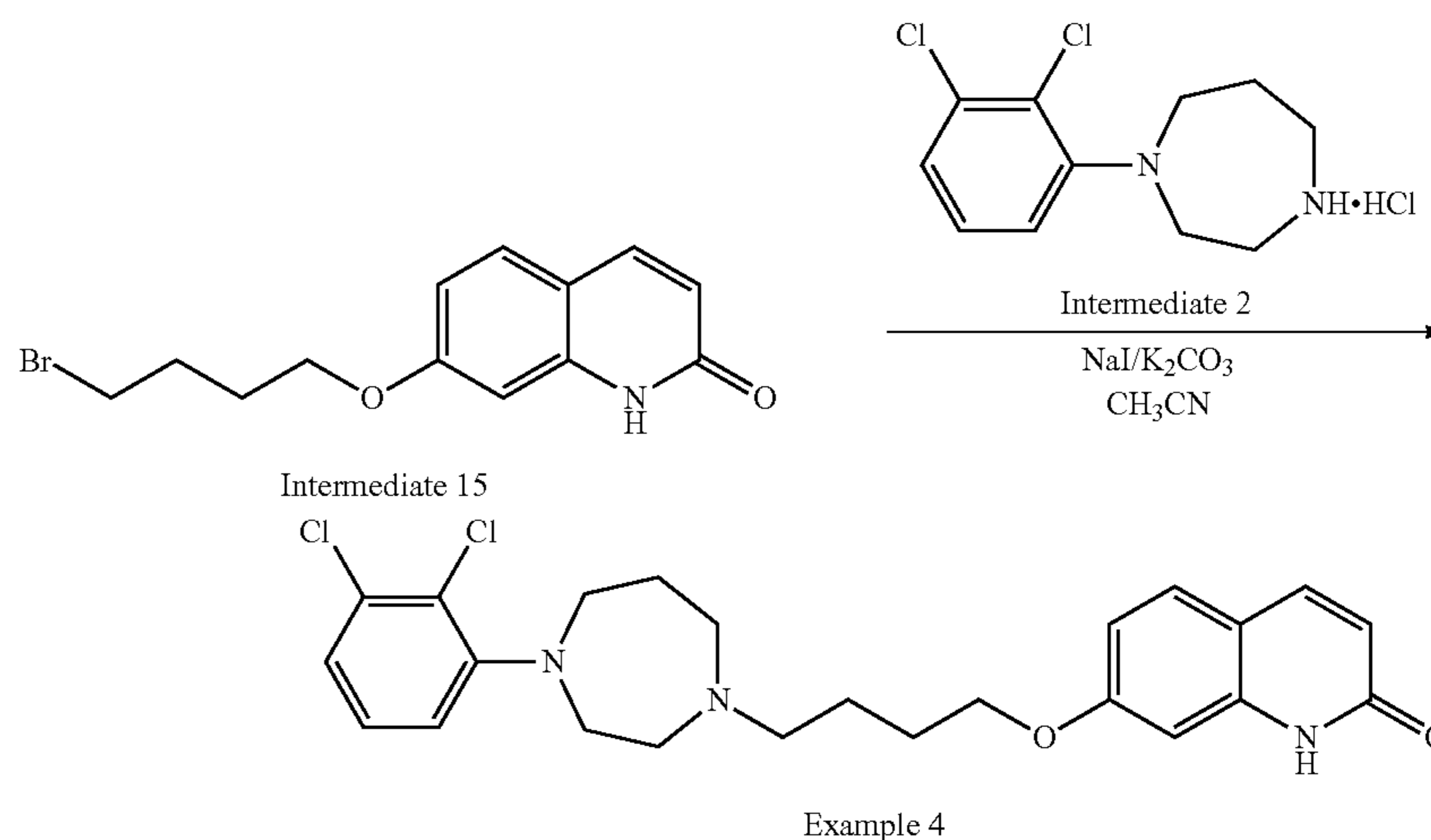
Scheme 9. Synthesis of compound 4
