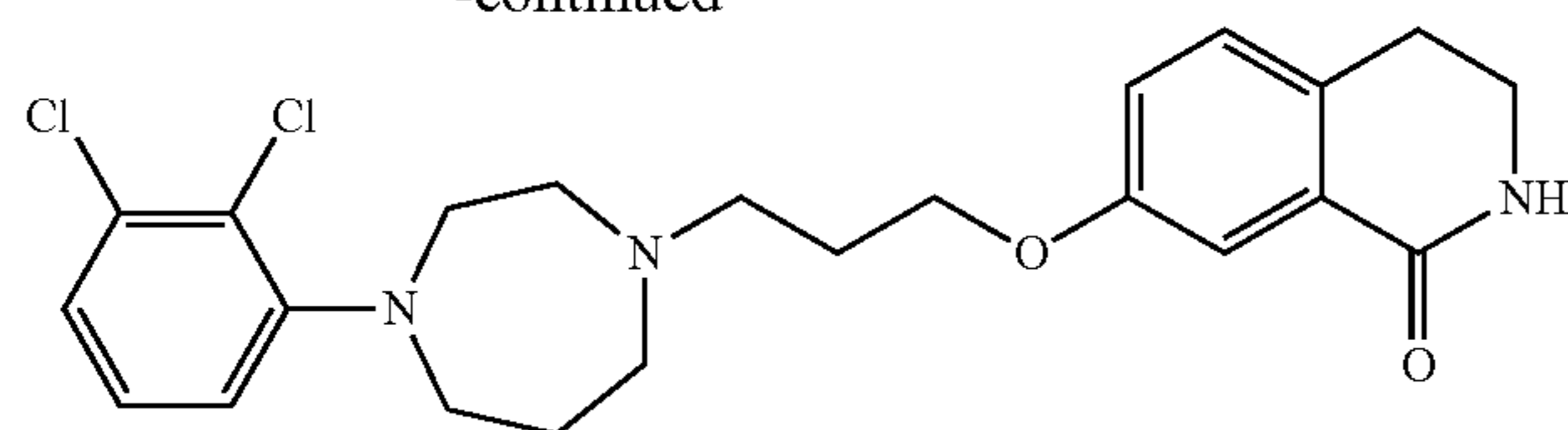
Example 5
