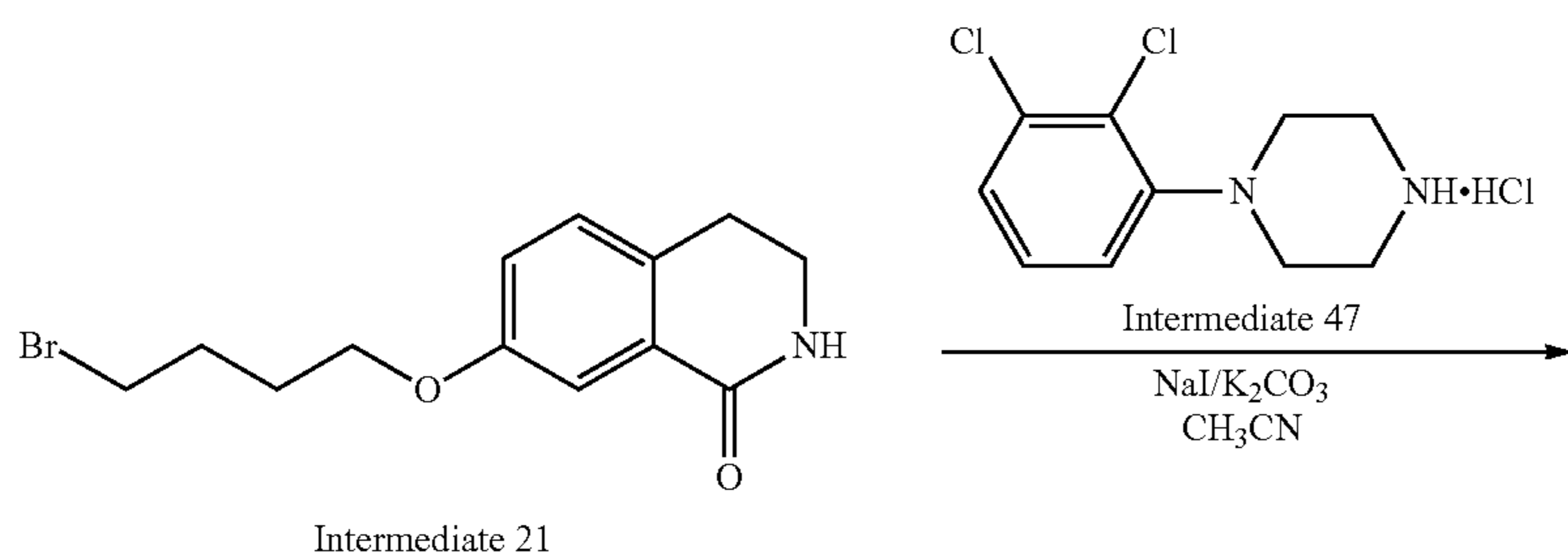
Scheme 57. Synthesis of compound 33
