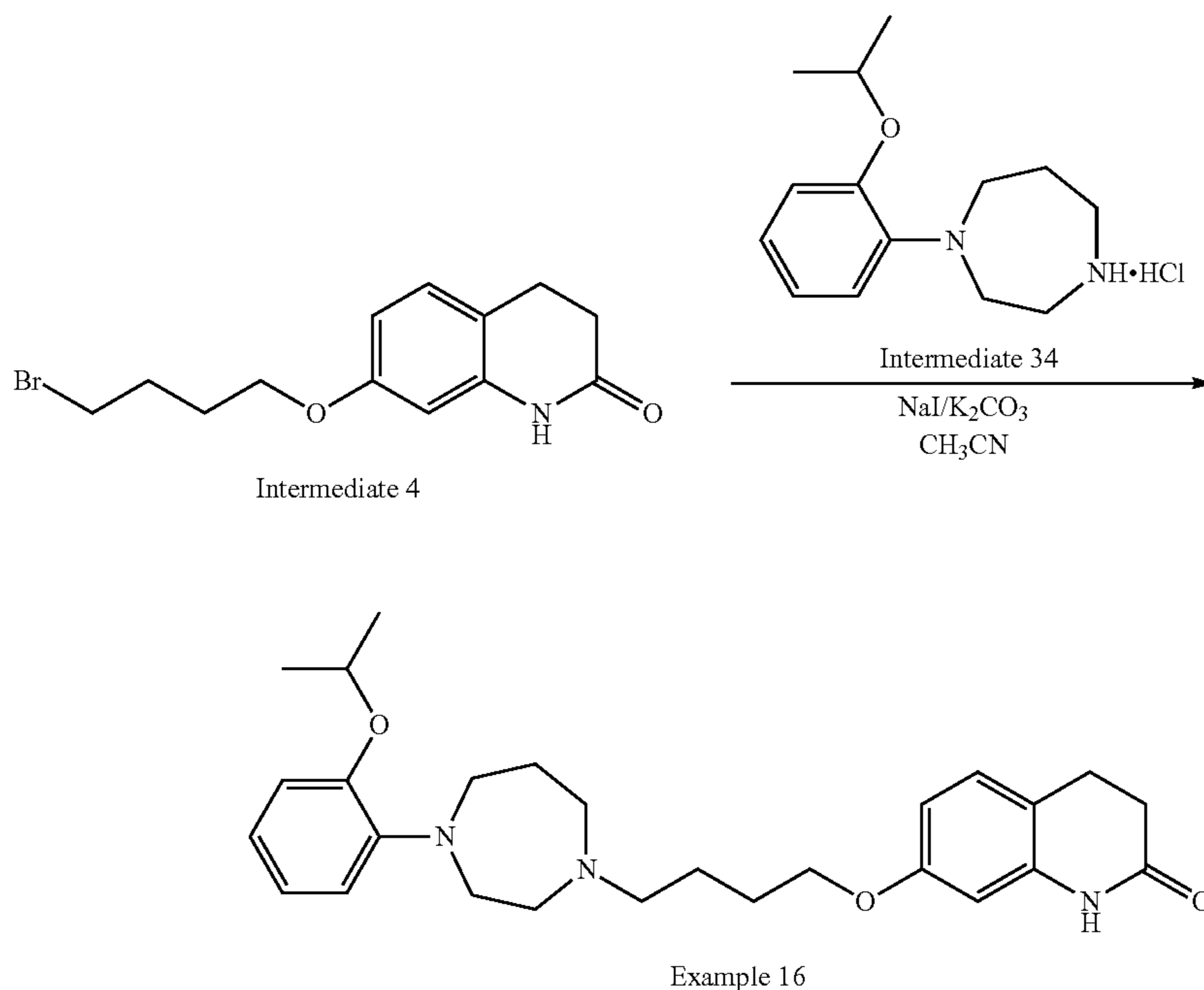
Scheme 29. Synthesis of compound 16
