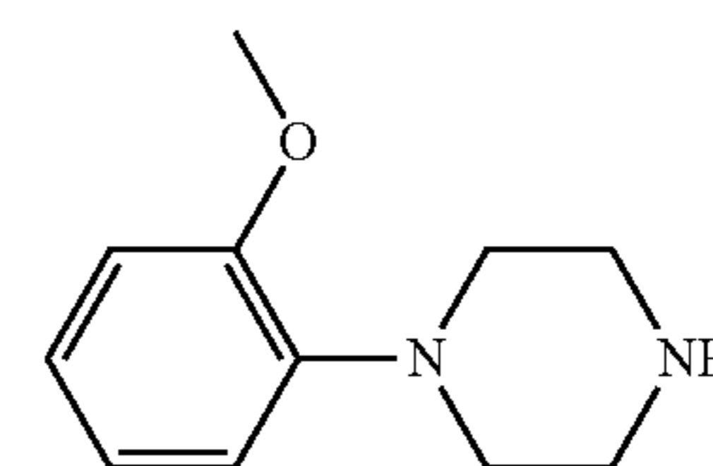
Intermediate 65
