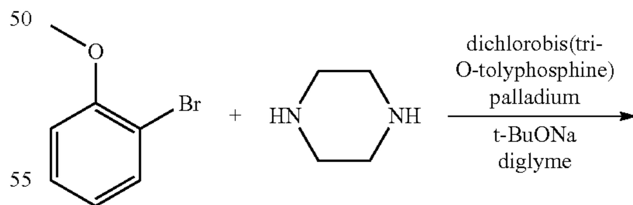
Scheme 77. Synthesis of intermediate 65
