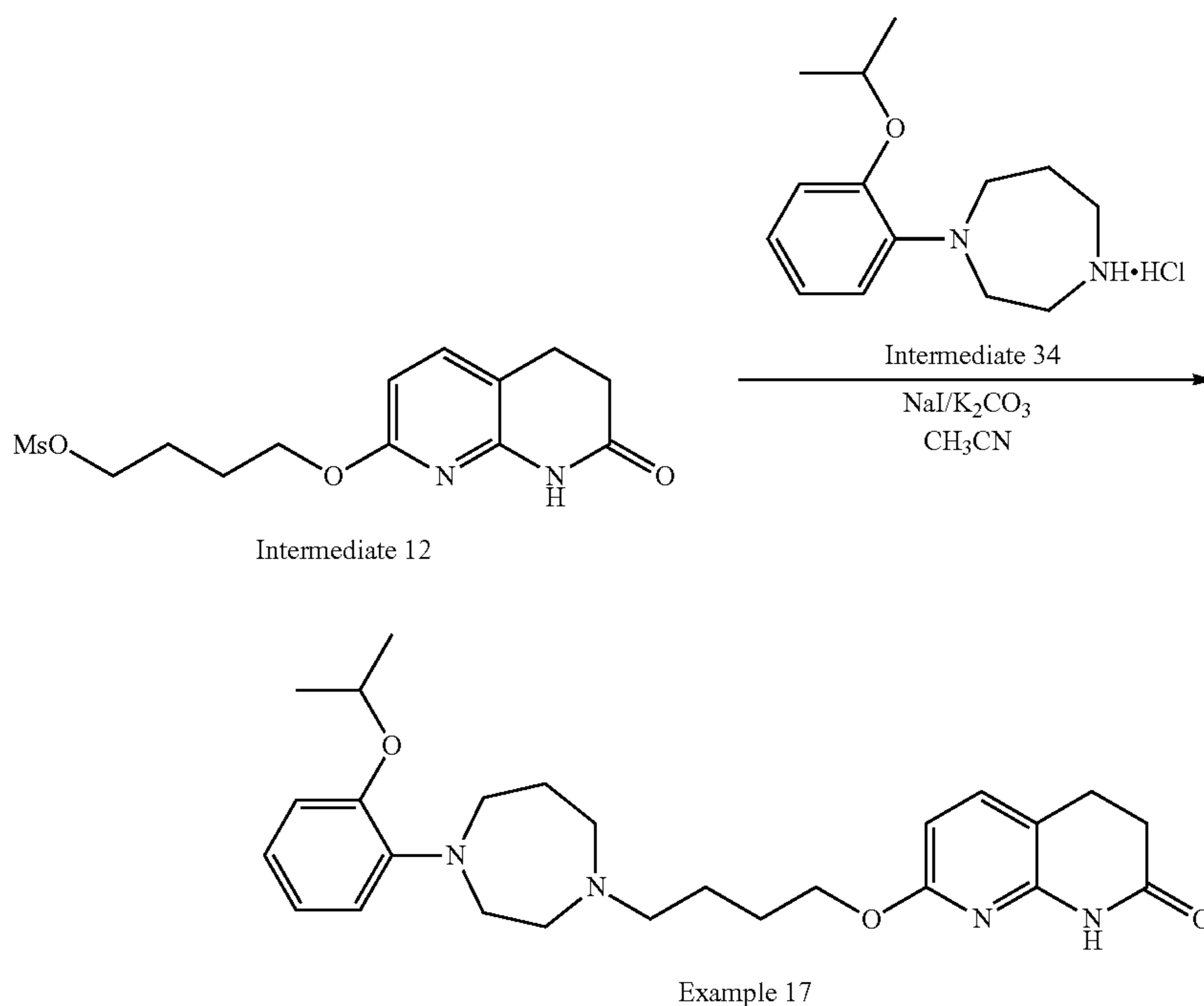
Scheme 30. Synthesis of compound 17
