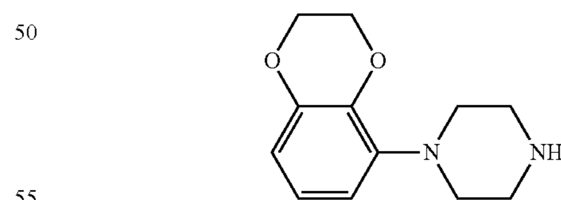
Intermediate 61:
