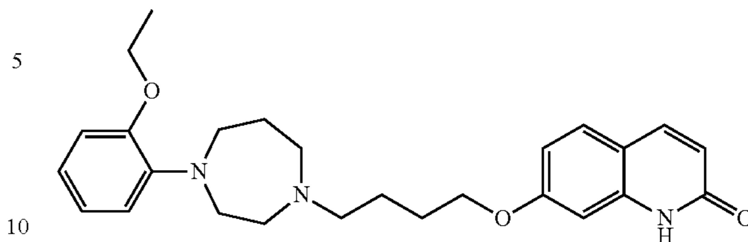
Compound 14:
