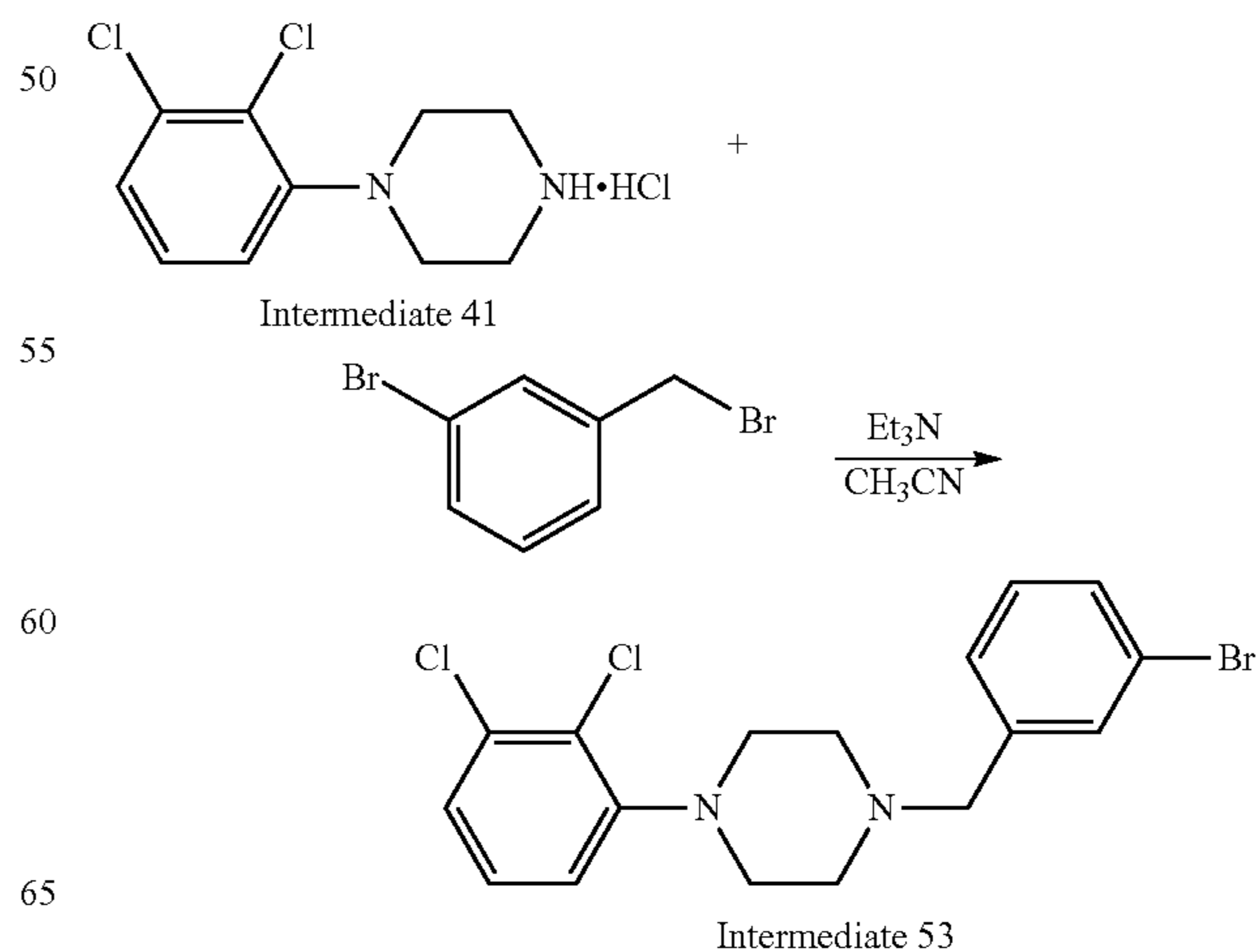
Scheme 52. Synthesis of intermediate 53
