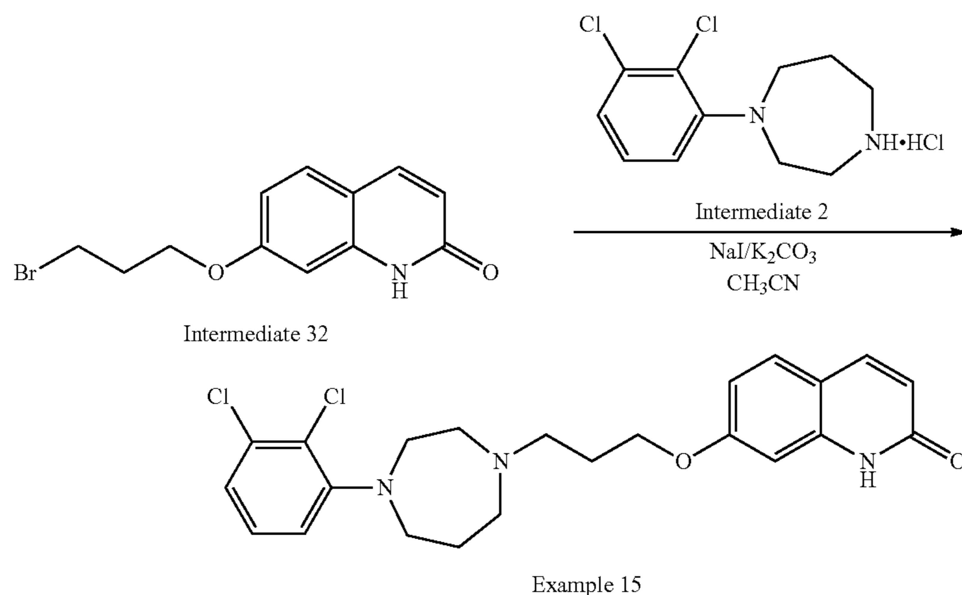
Scheme 27. Synthesis of compound 15
