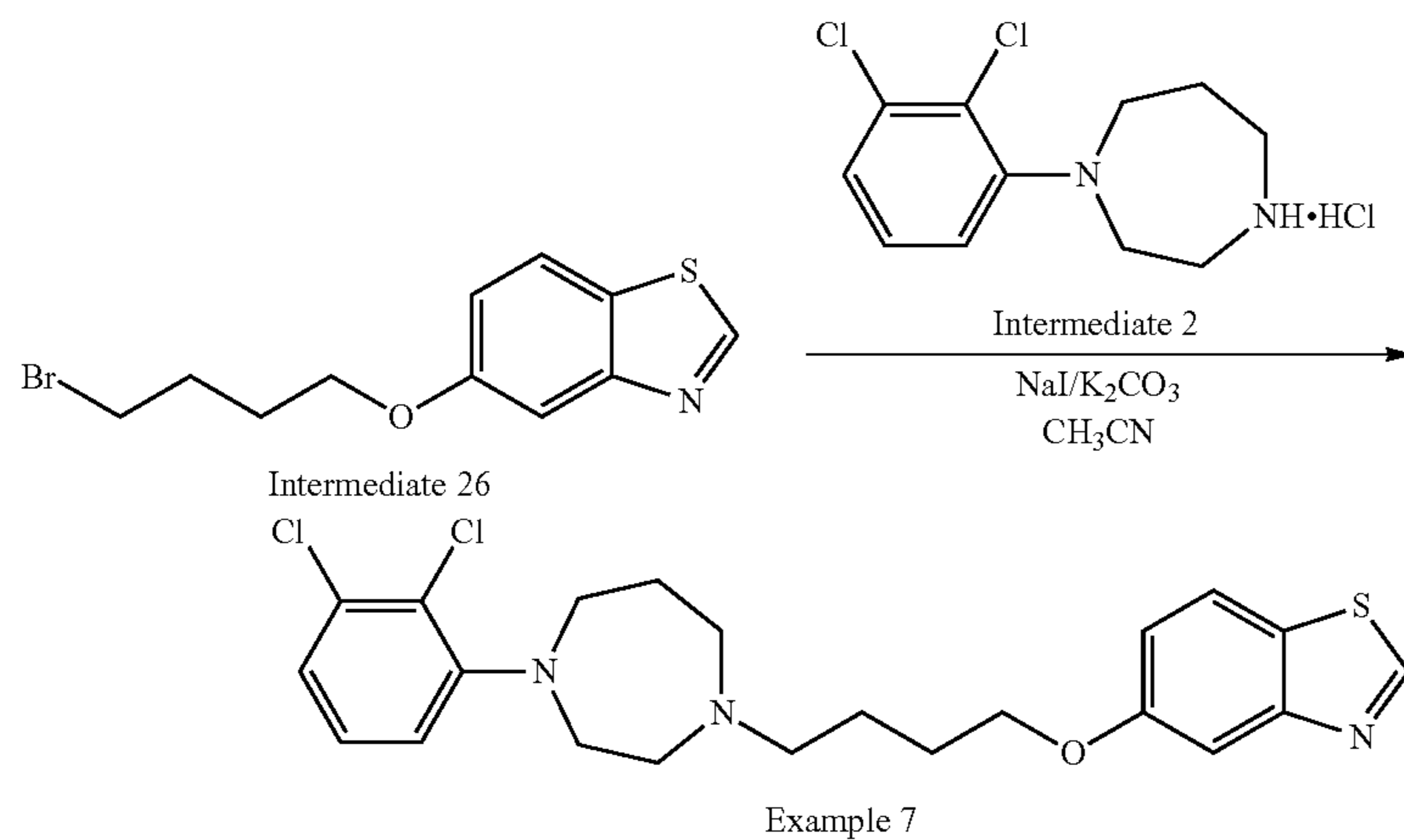
Scheme 15. Synthesis of compound 7
