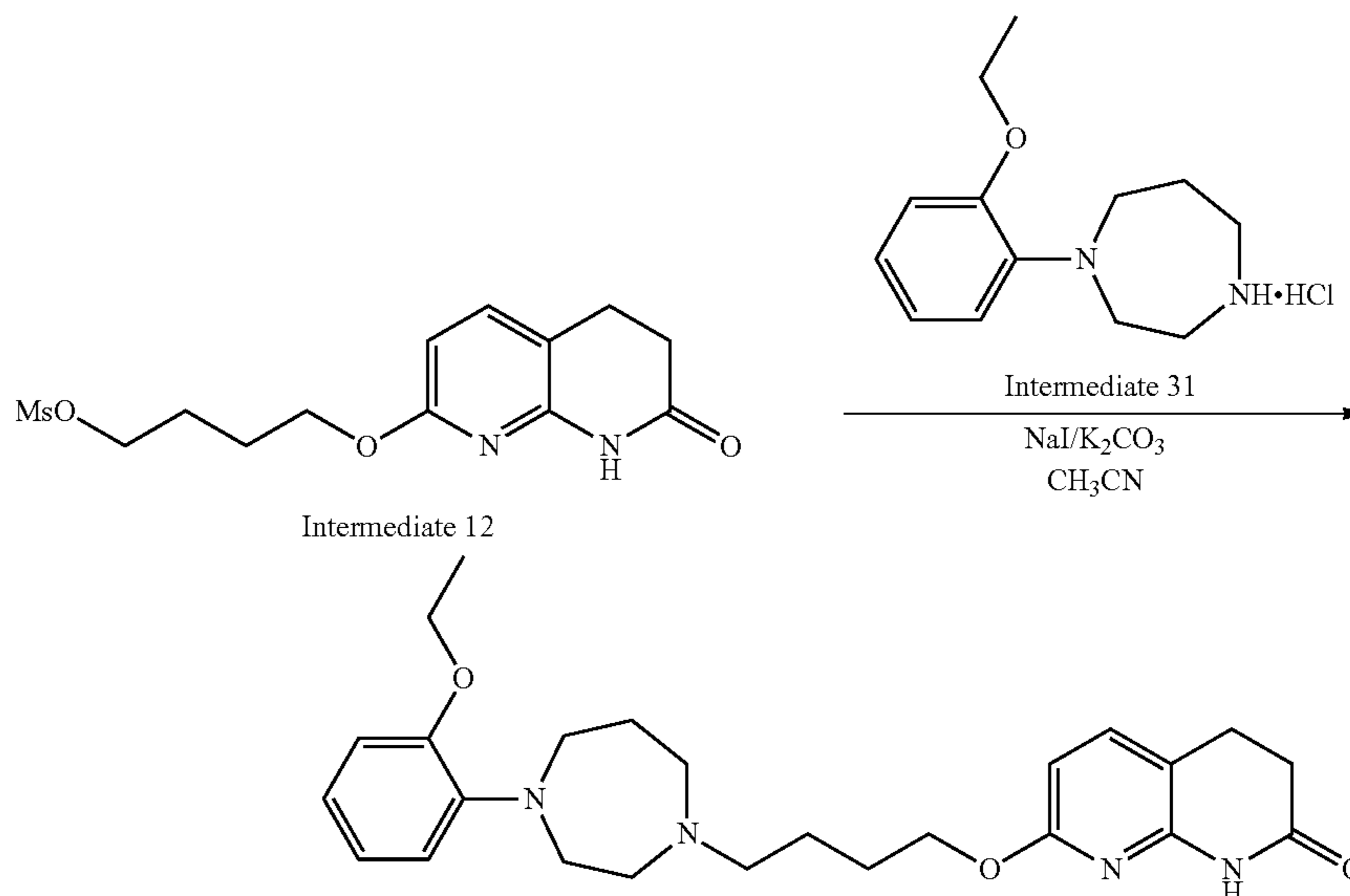
Scheme 24. Synthesis of compound 13
