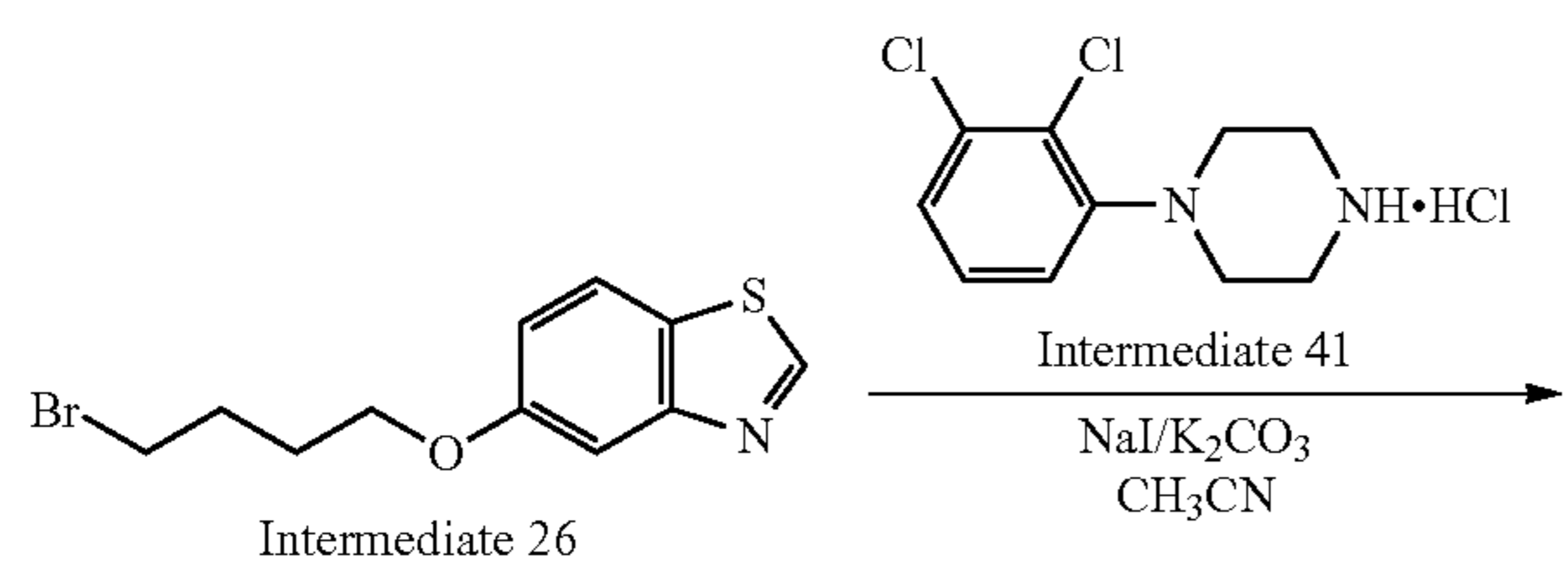
Scheme 60. Synthesis of compound 36
