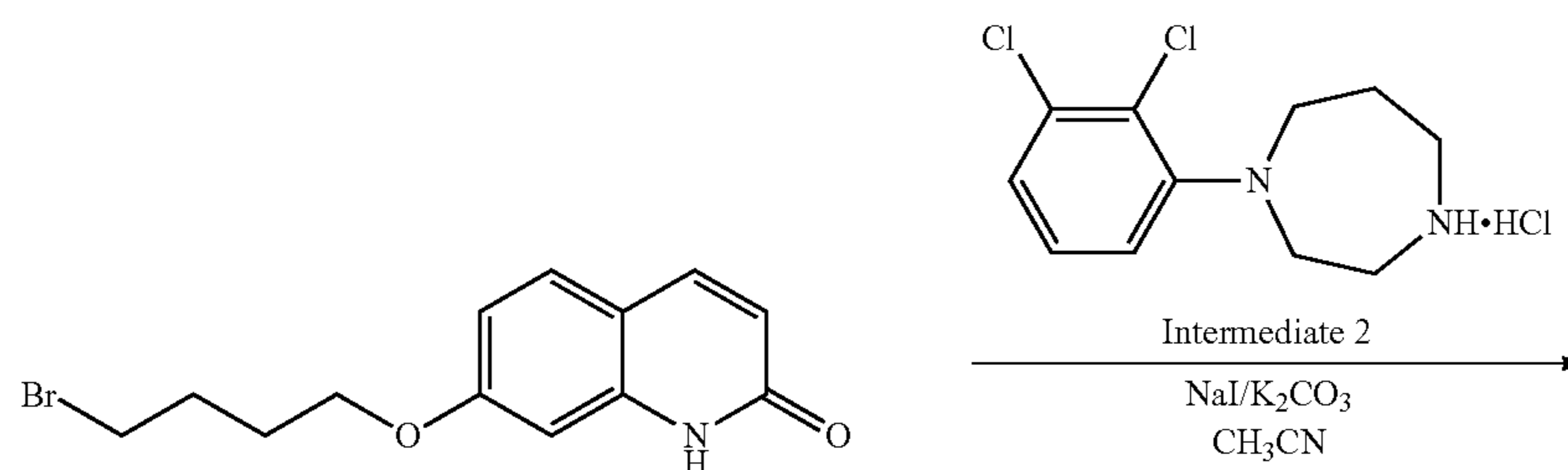
Scheme 9. Synthesis of compound 4
