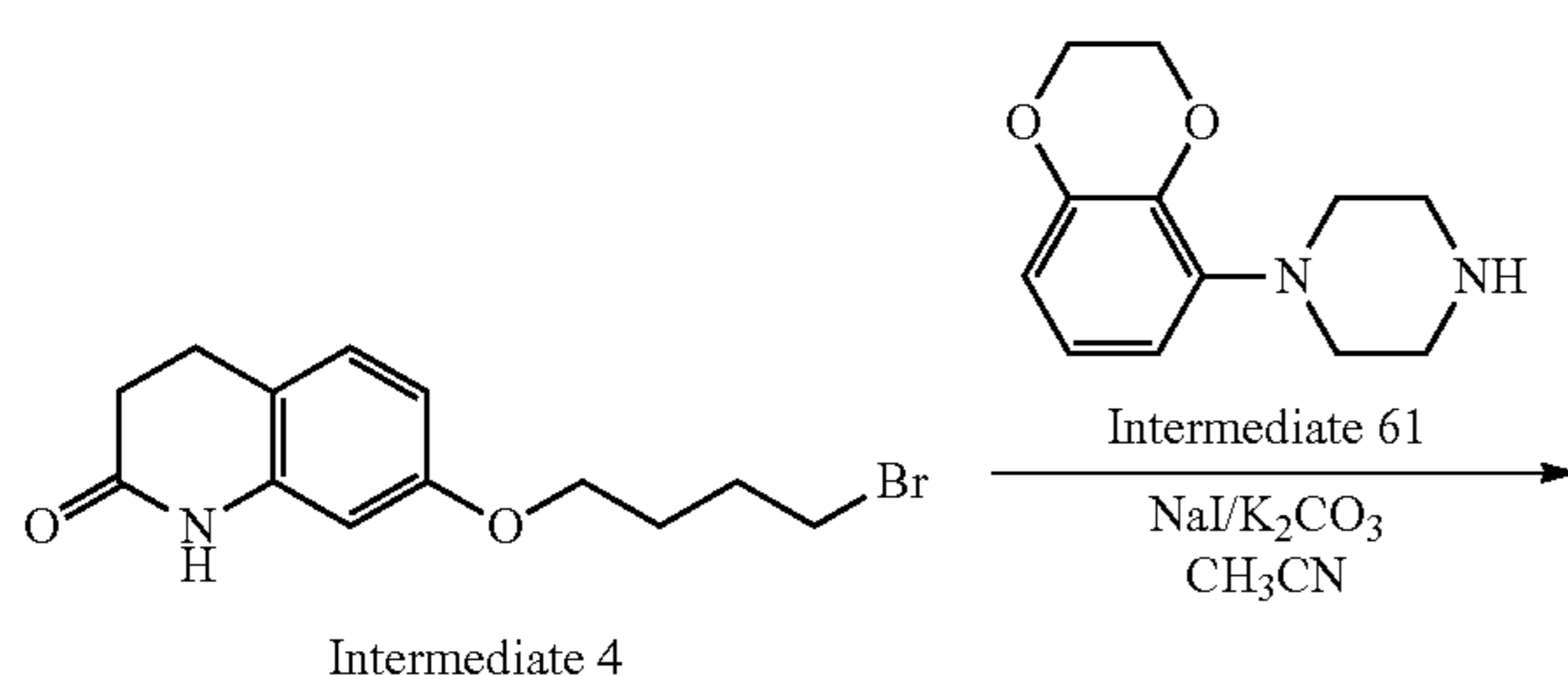
Scheme 67. Synthesis of compound 40
