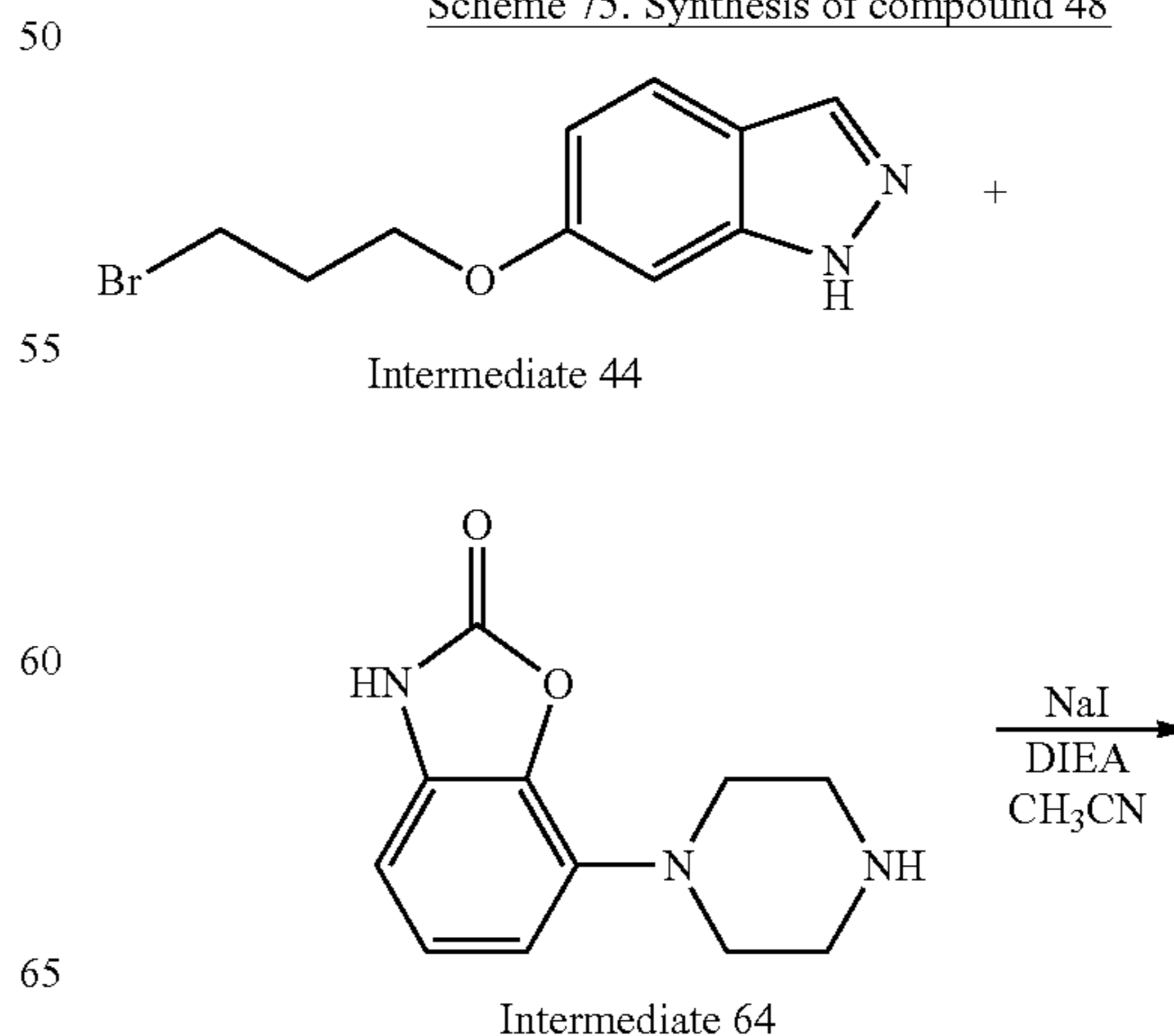
Scheme 75. Synthesis of compound 48
