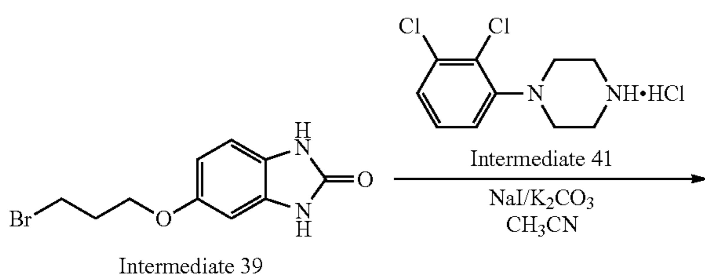
Scheme 58. Synthesis of compound 34
