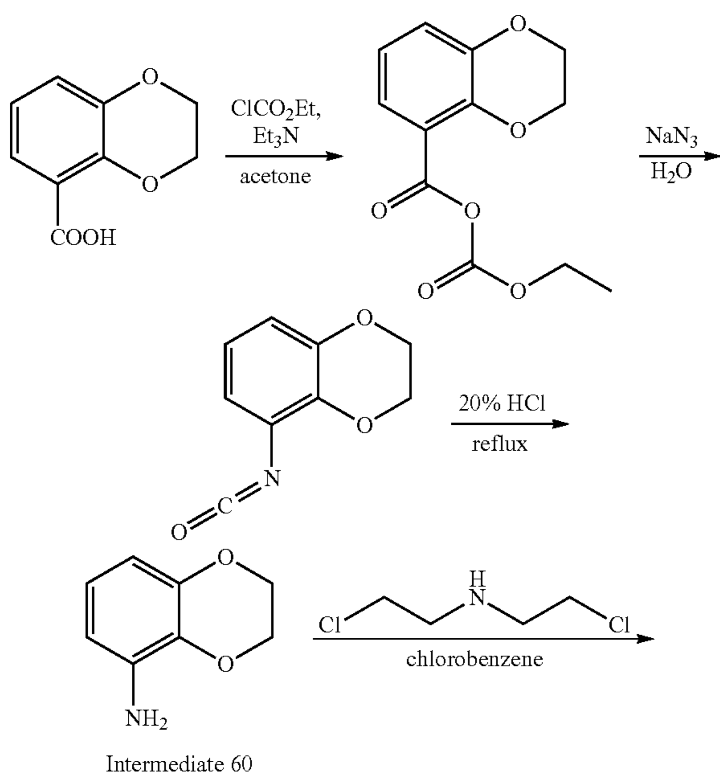
Scheme 66. Synthesis of intermediate 61
