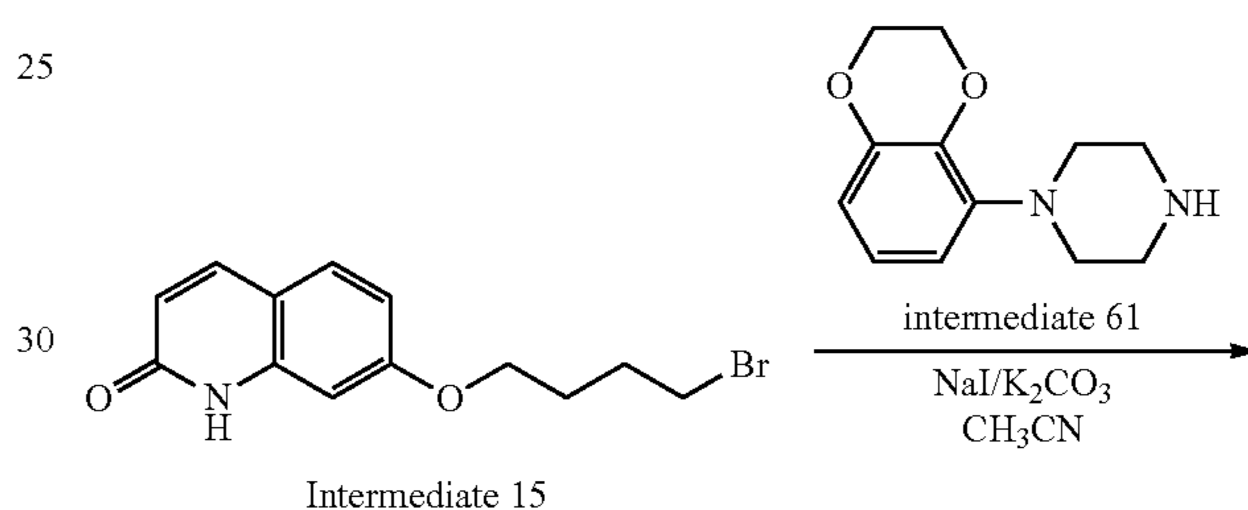
Scheme 69. Synthesis of compound 42
