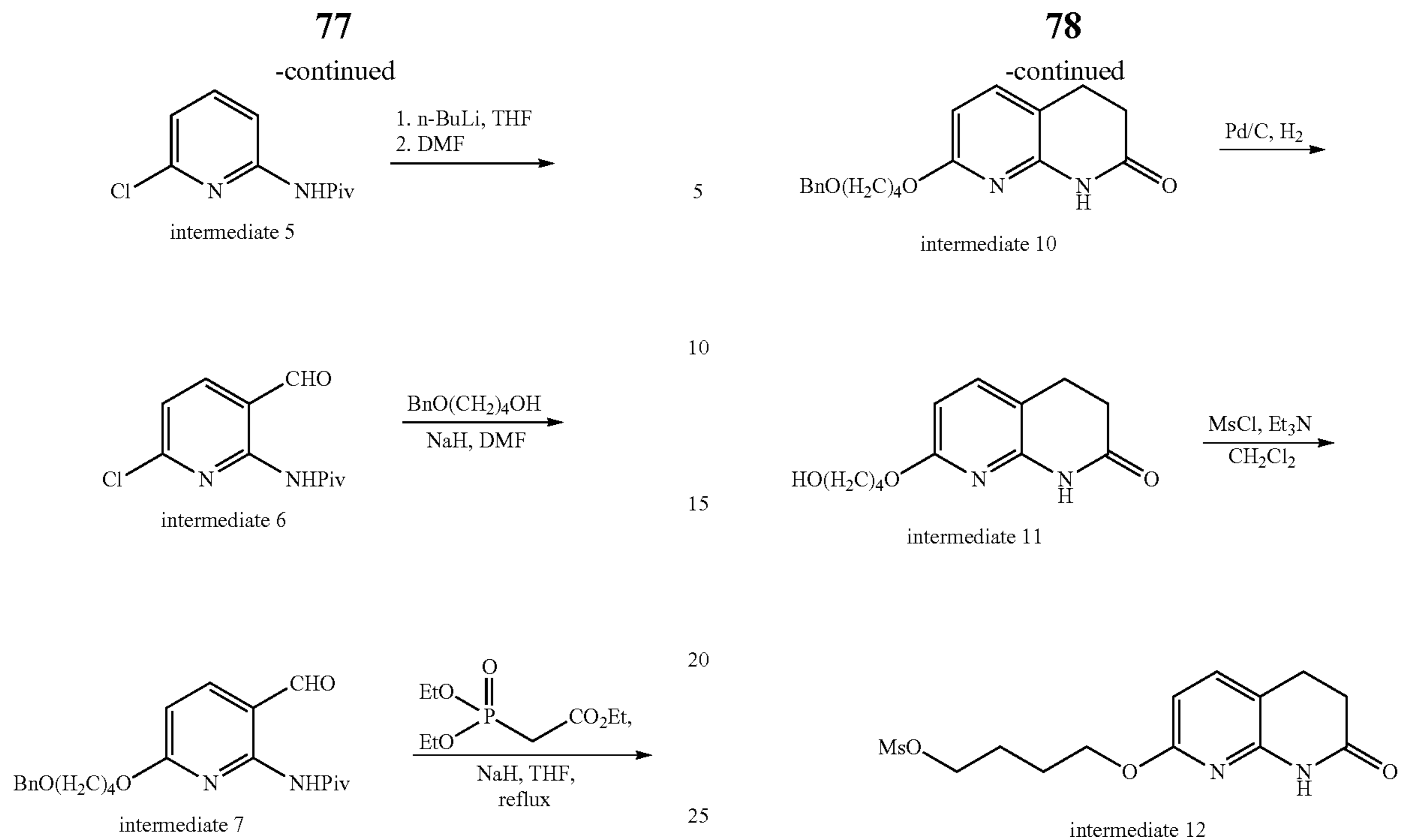
Scheme 7. Synthesis of compound 3
