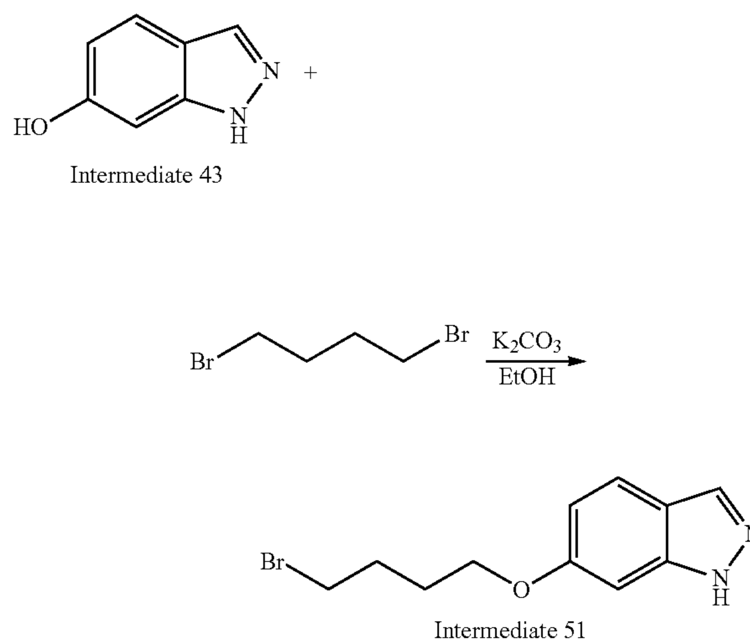
Scheme 48. Synthesis of intermediate 51
