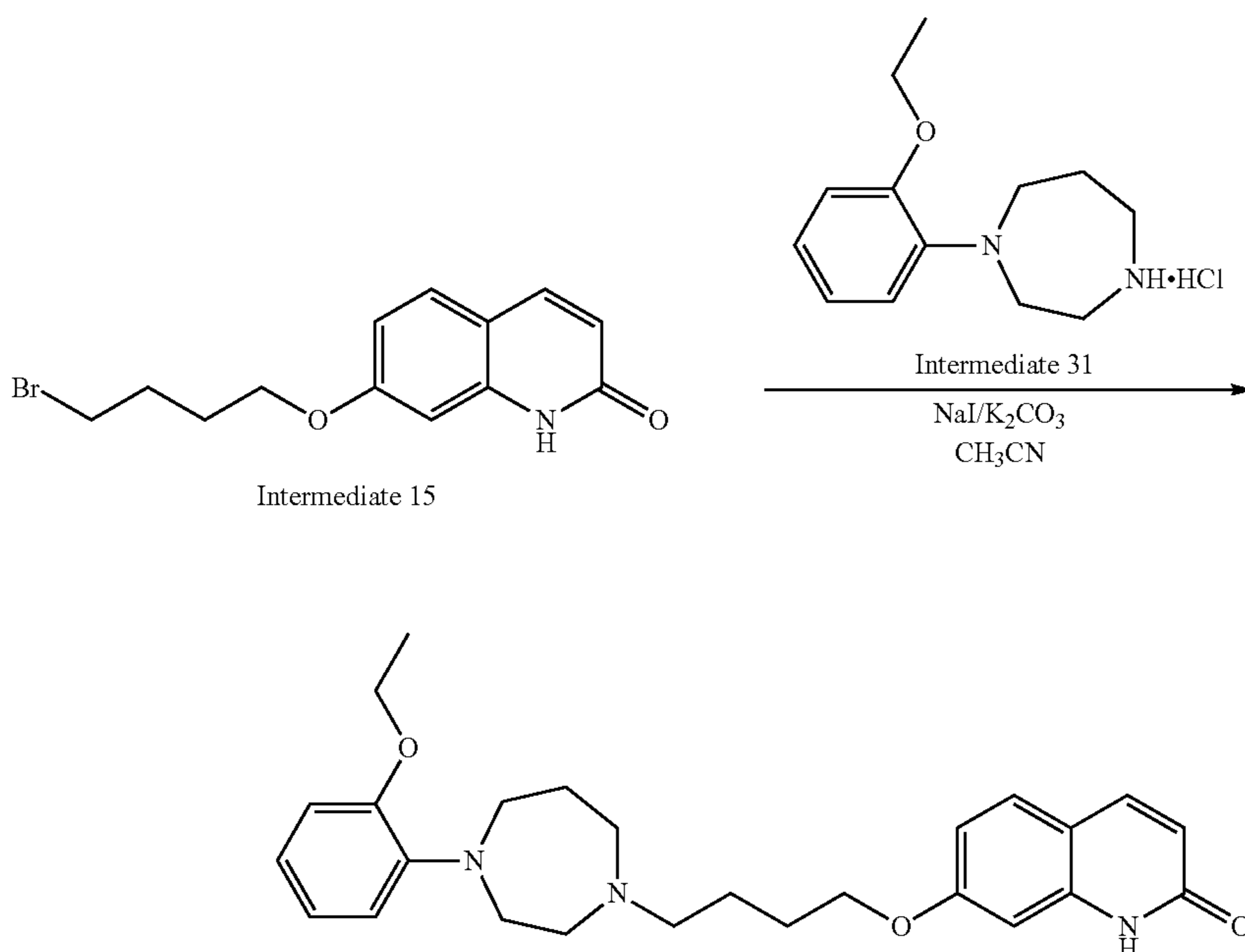
Example 14
