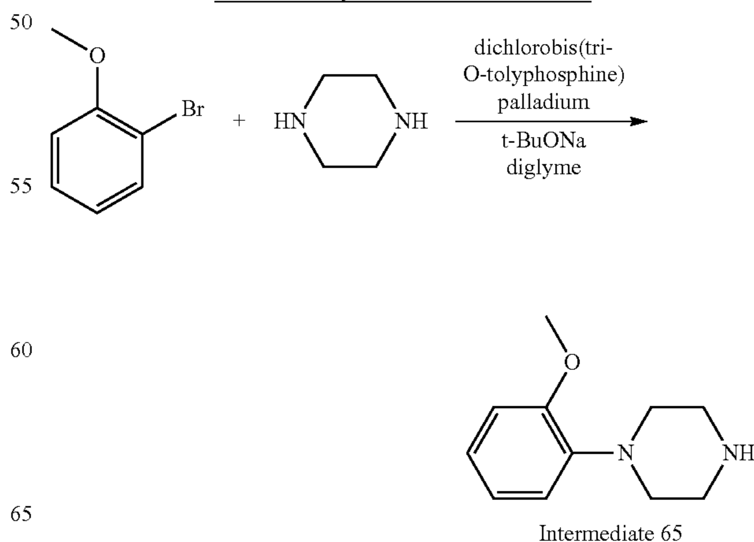
Scheme 77. Synthesis of intermediate 65
