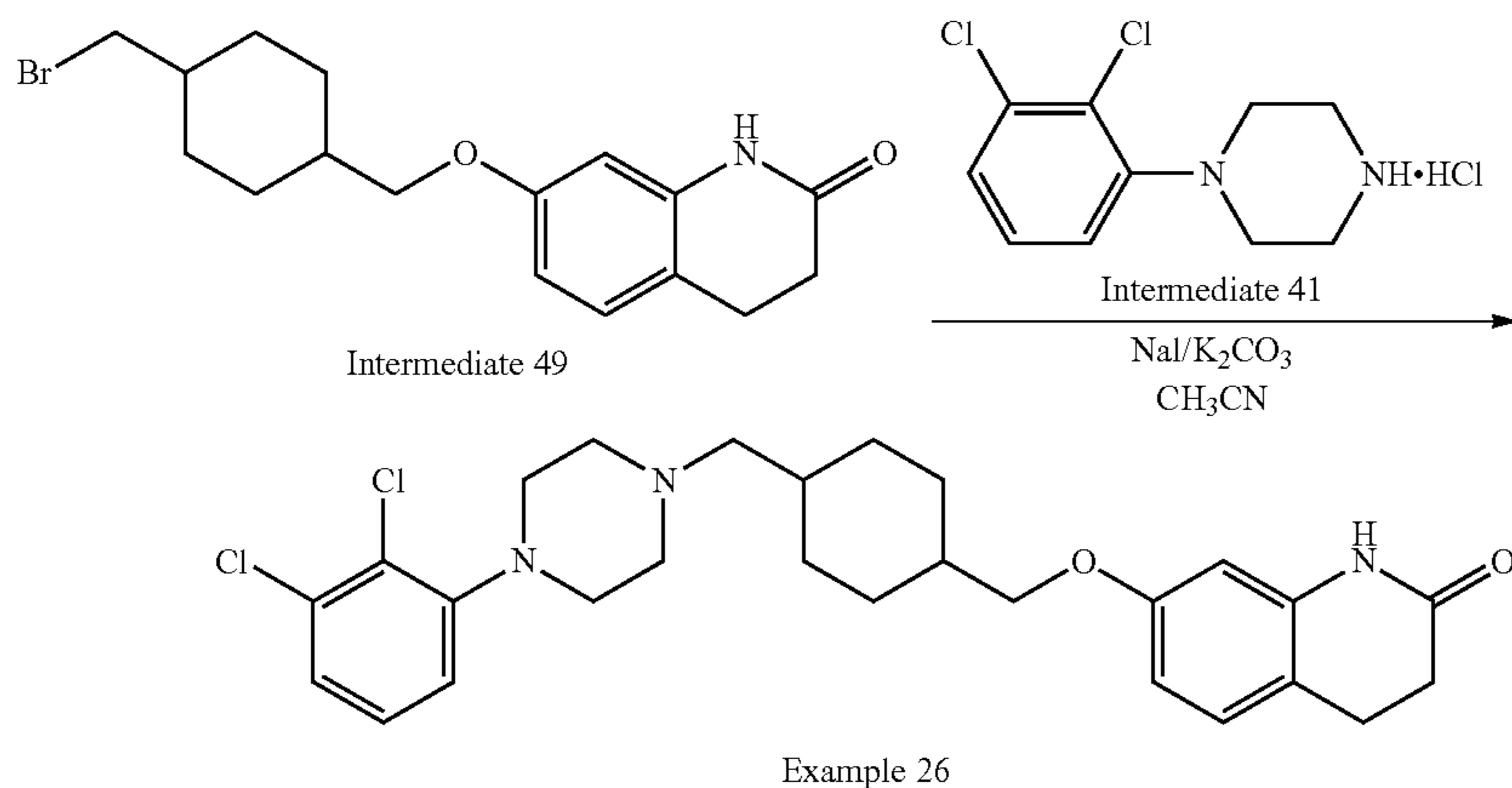
Scheme 45. Synthesis of compound 26
