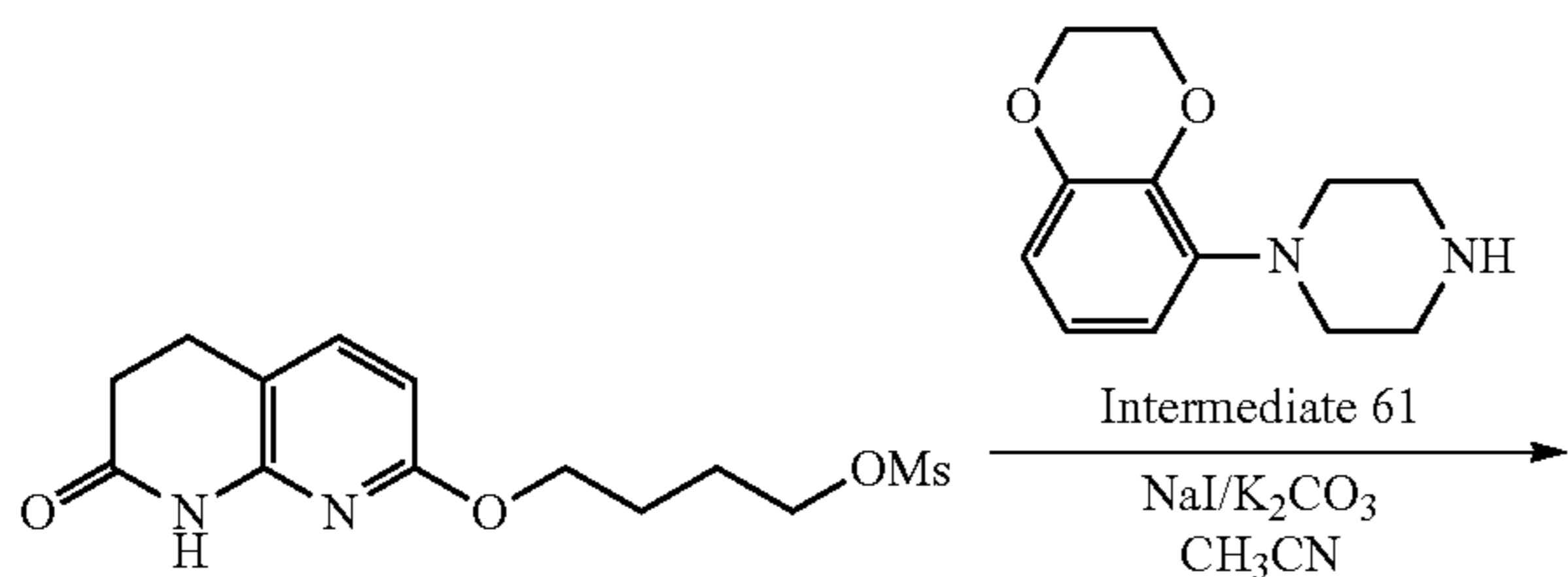
Scheme 68. Synthesis of compound 41
