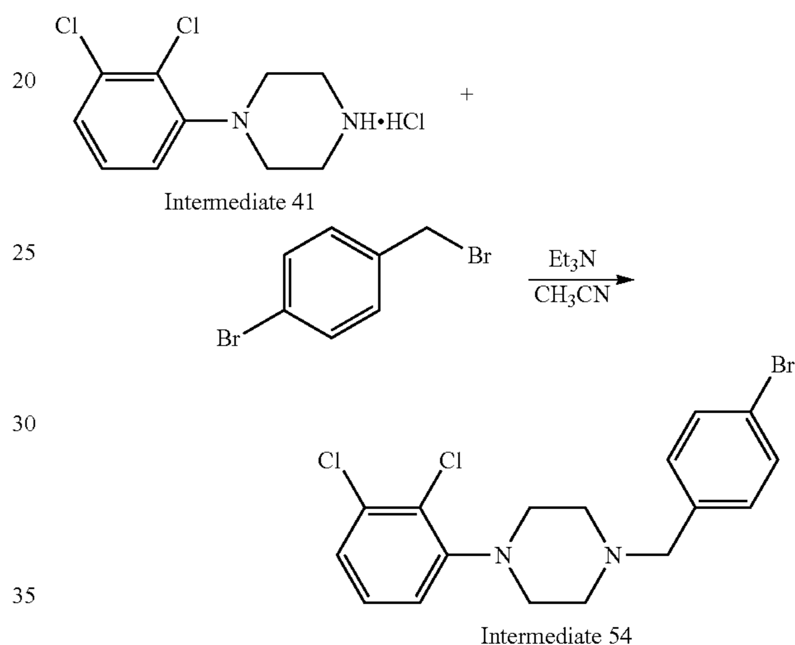
Scheme 54. Synthesis of intermediate 54
