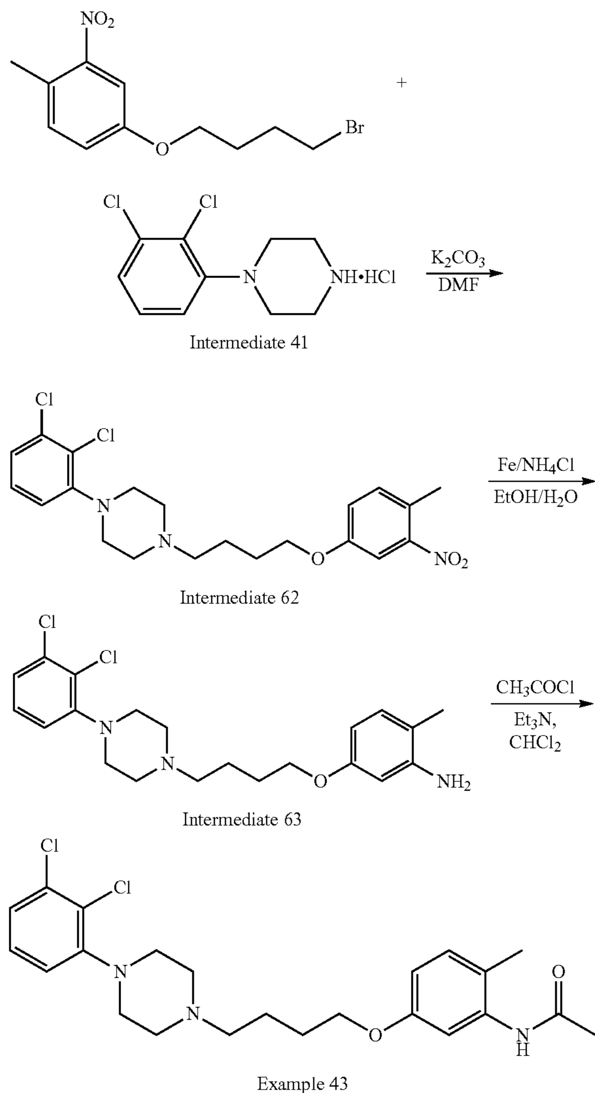
Scheme 70. Synthesis of compound 43
