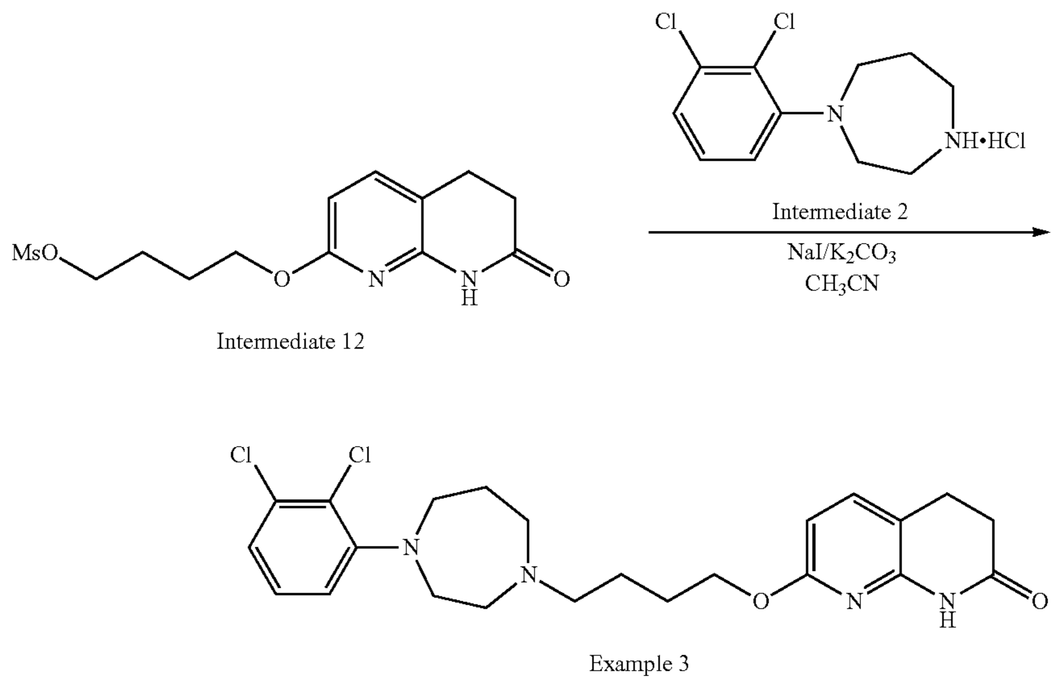
Scheme 7. Synthesis of compound 3
