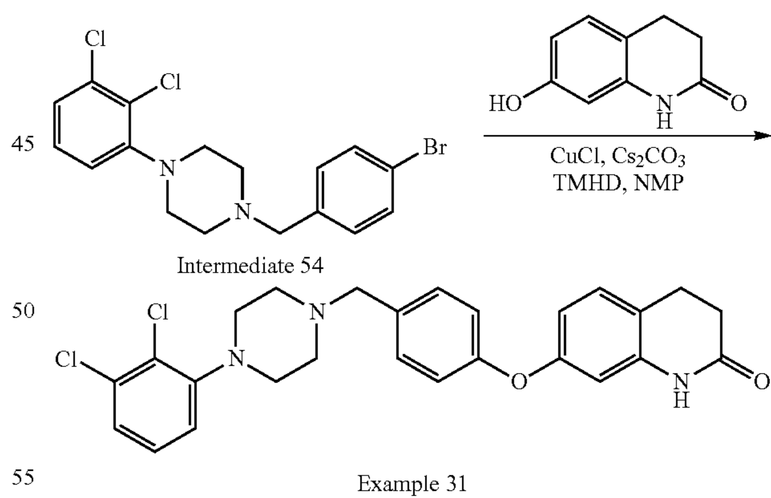
Scheme 55. Synthesis of compound 31
