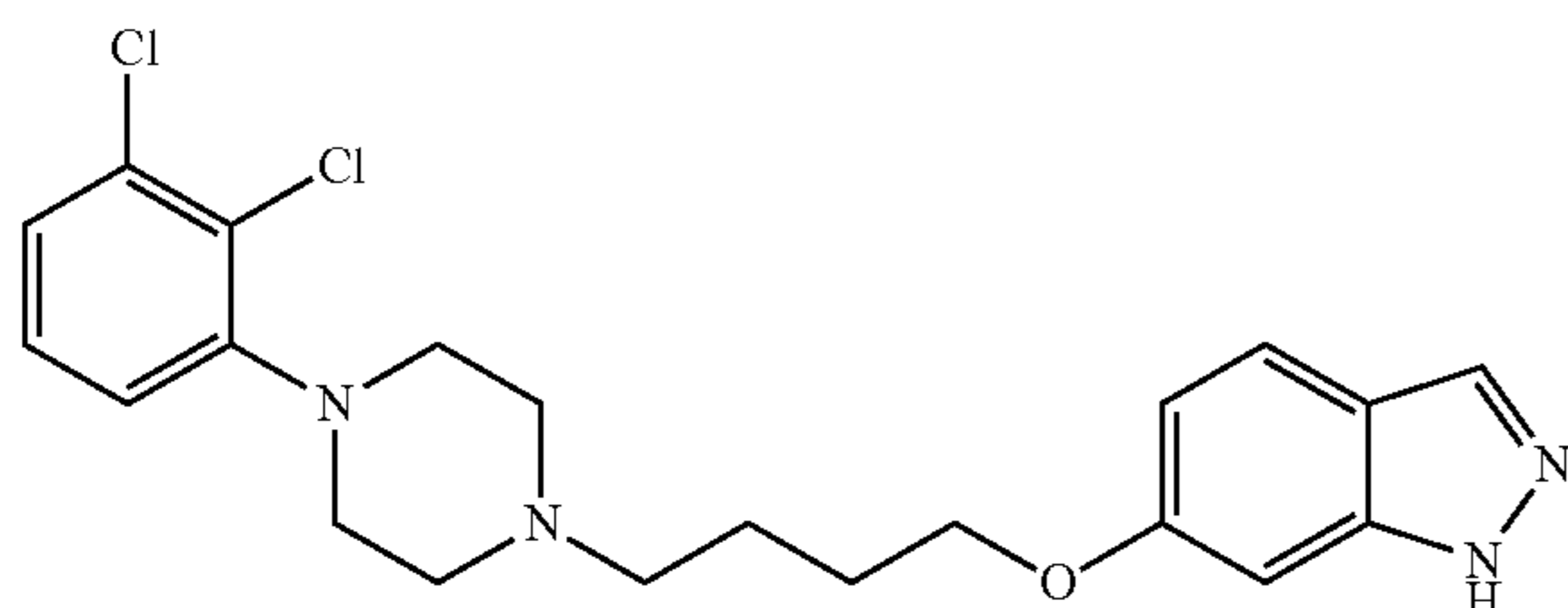
Compound 28:
