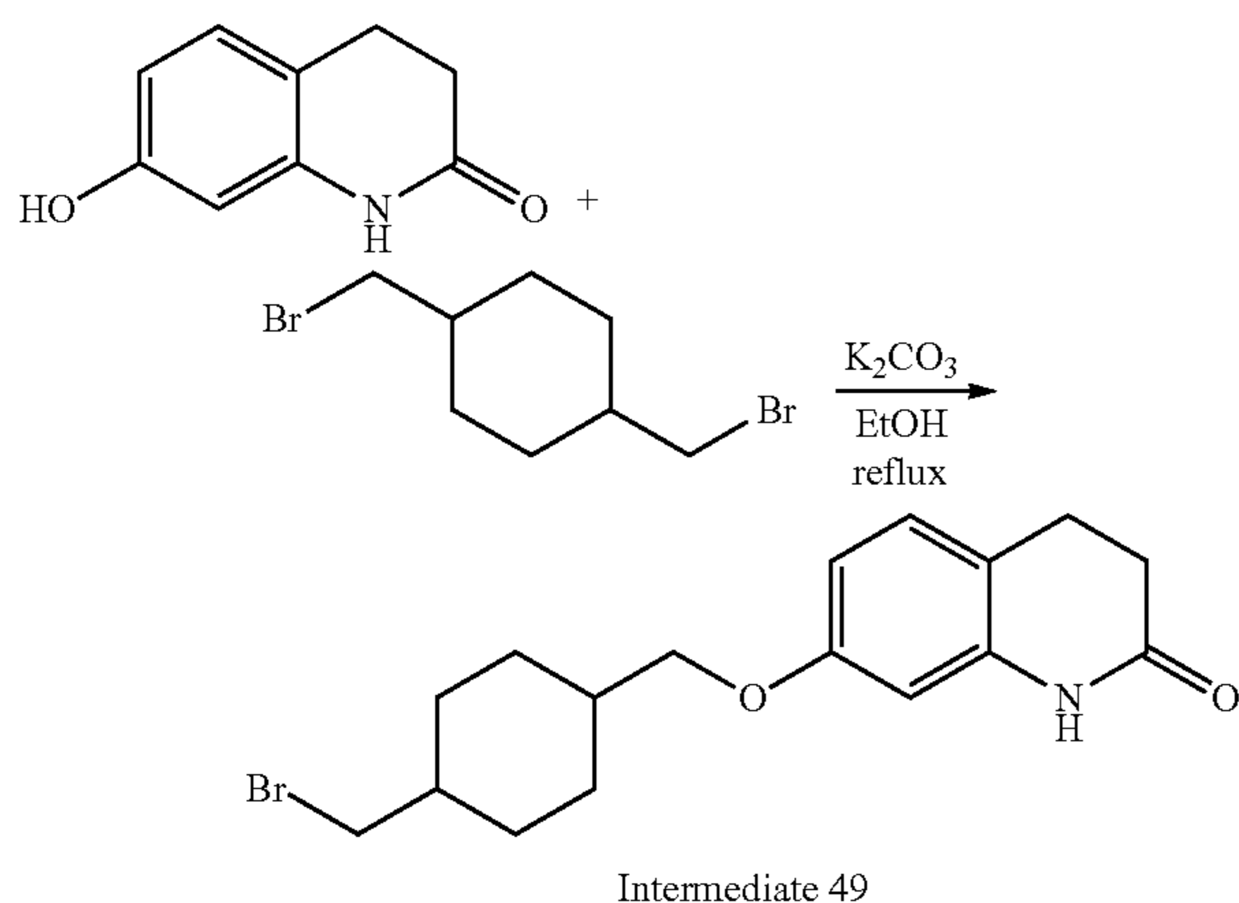
Scheme 44. Synthesis of intermediate 49
