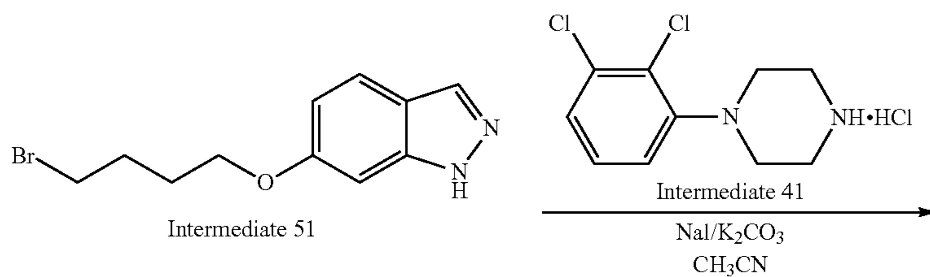
Scheme 49. Synthesis of compound 28
