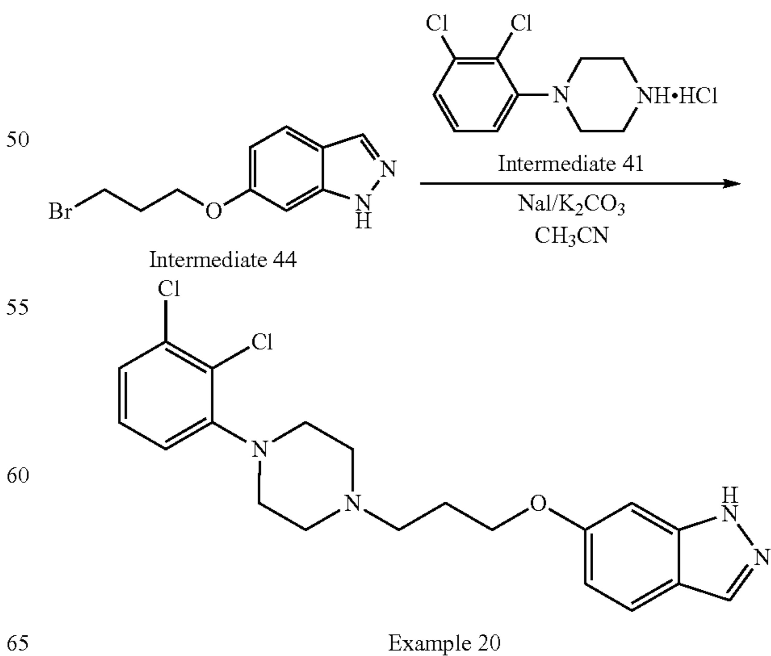
Scheme 36. Synthesis of compound 20
