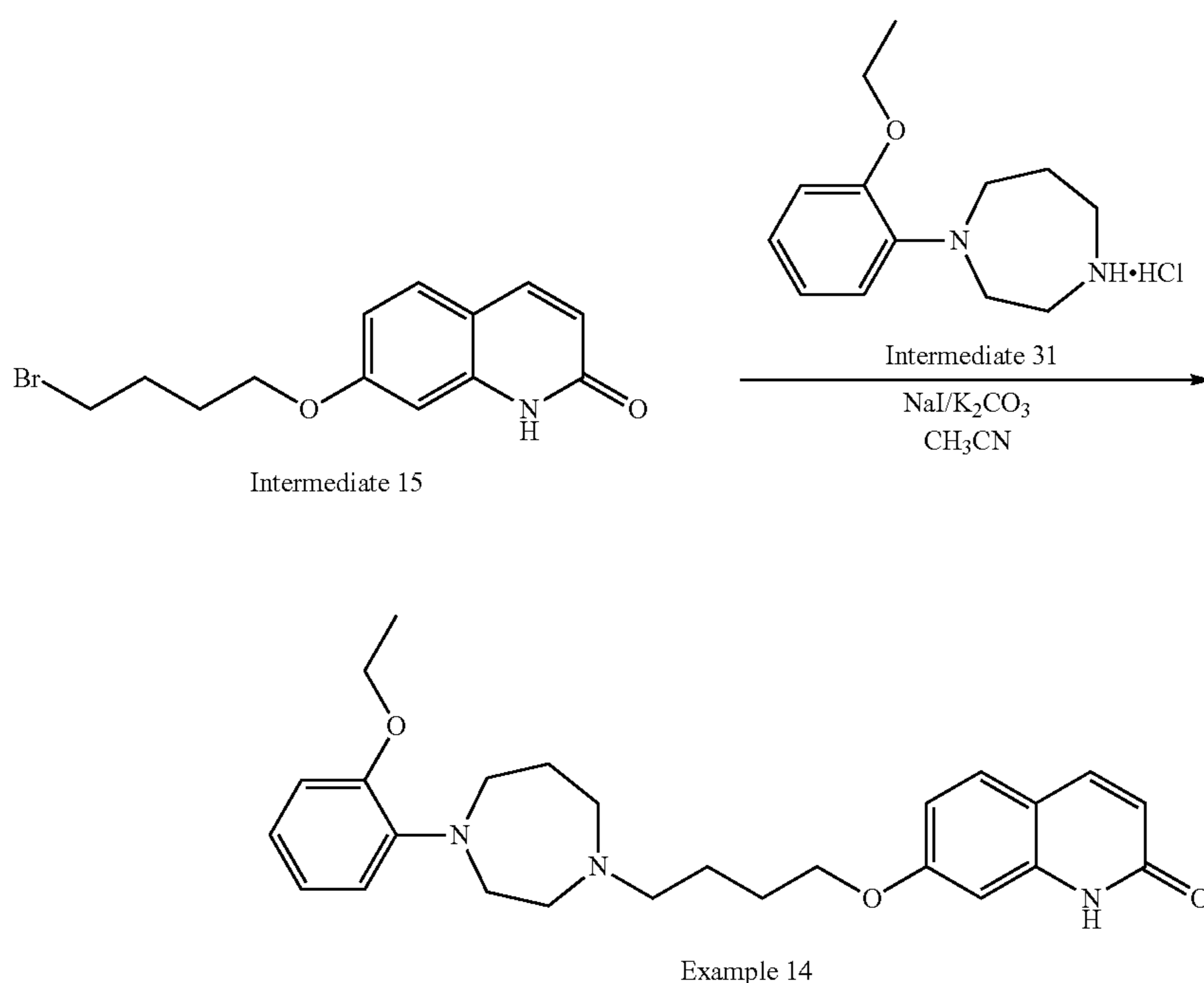
Scheme 25. Synthesis of compound 14
