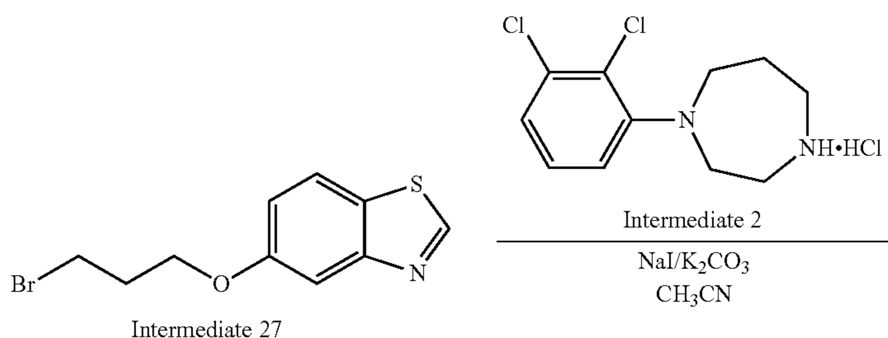
Scheme 17. Synthesis of compound 8
