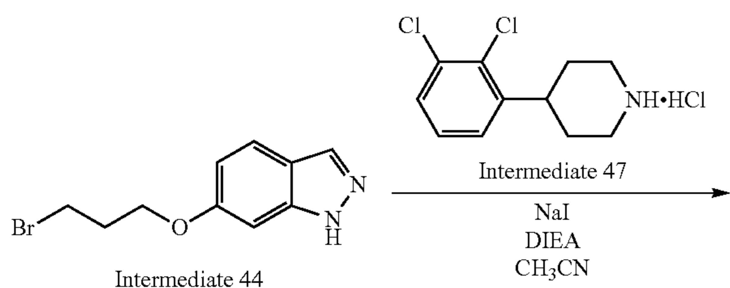
Scheme 71. Synthesis of compound 44
