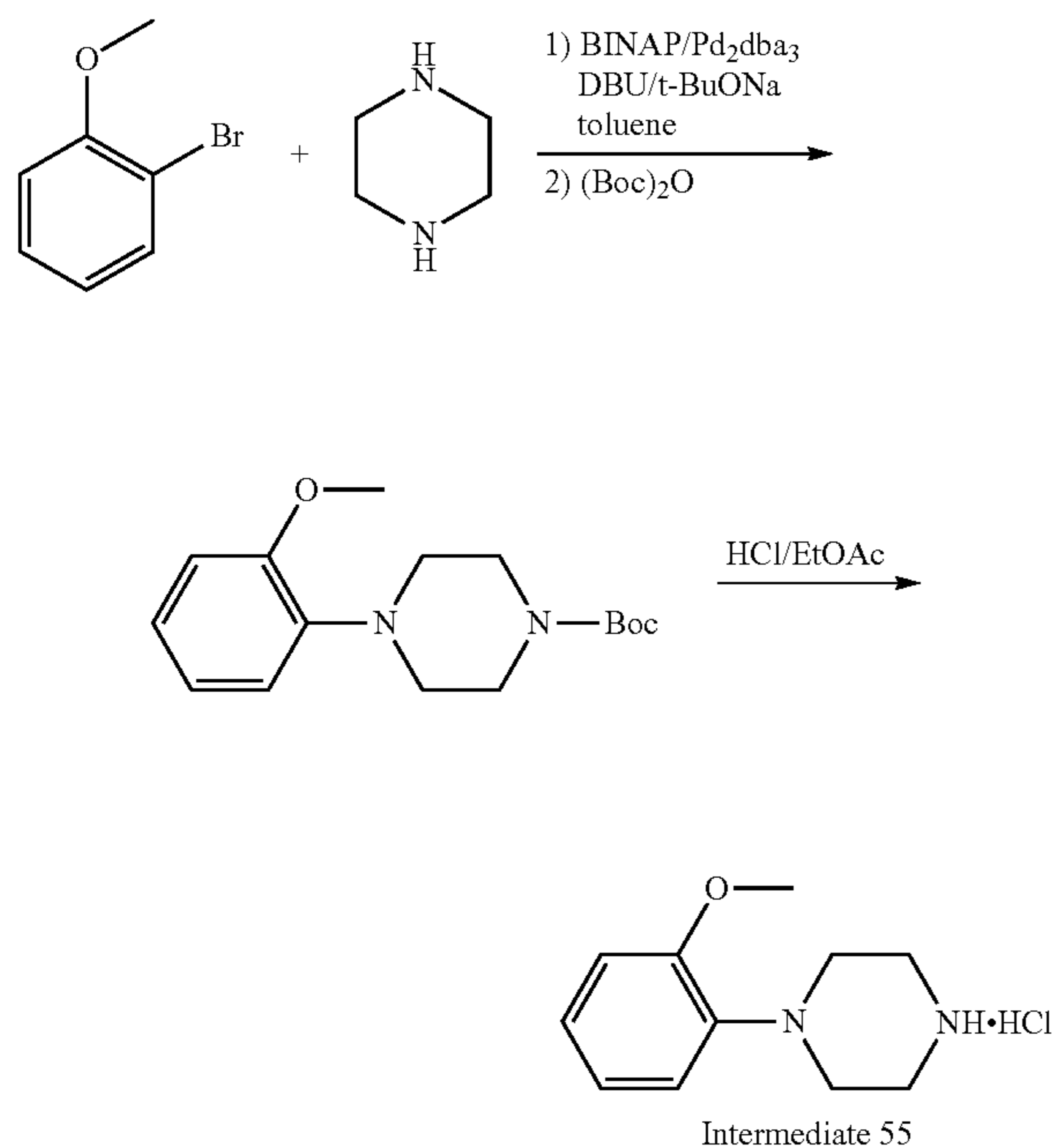
Scheme 61. Synthesis of intermediate 55
