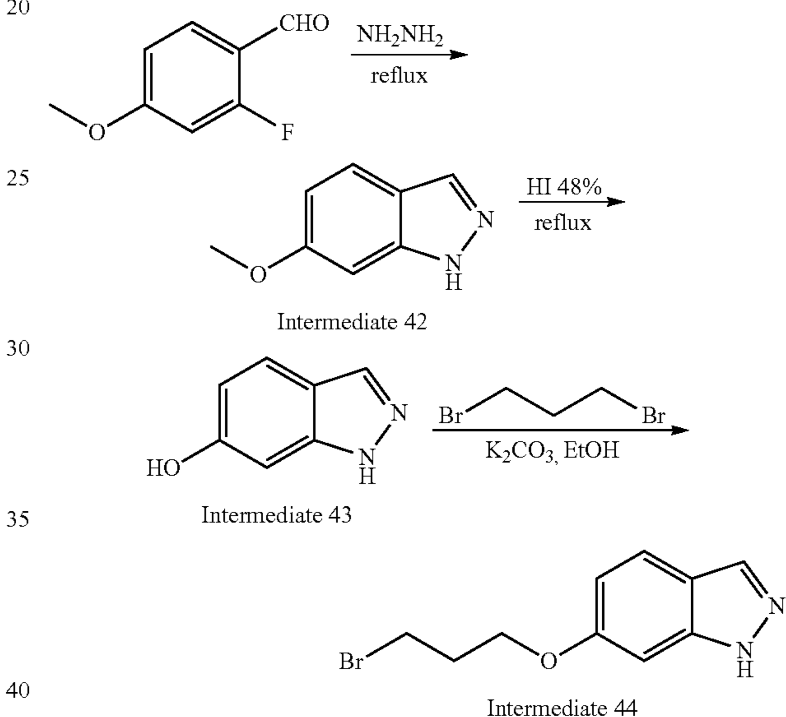
Scheme 35. Synthesis of intermediate 44
