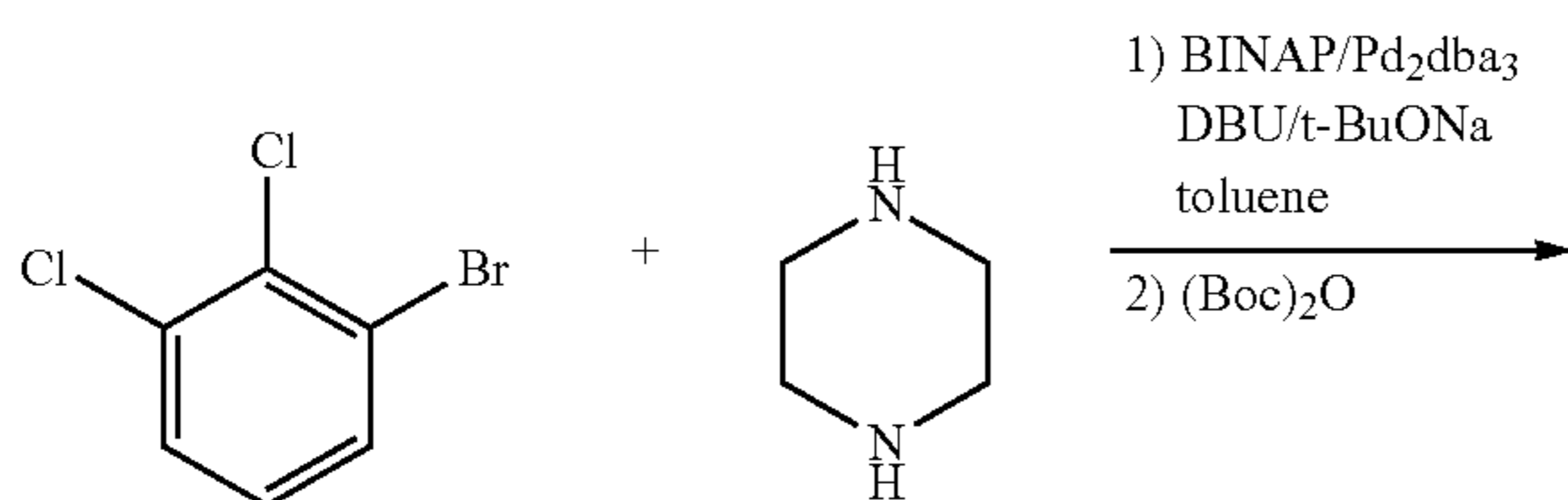
Scheme 34. Synthesis of intermediate 41
