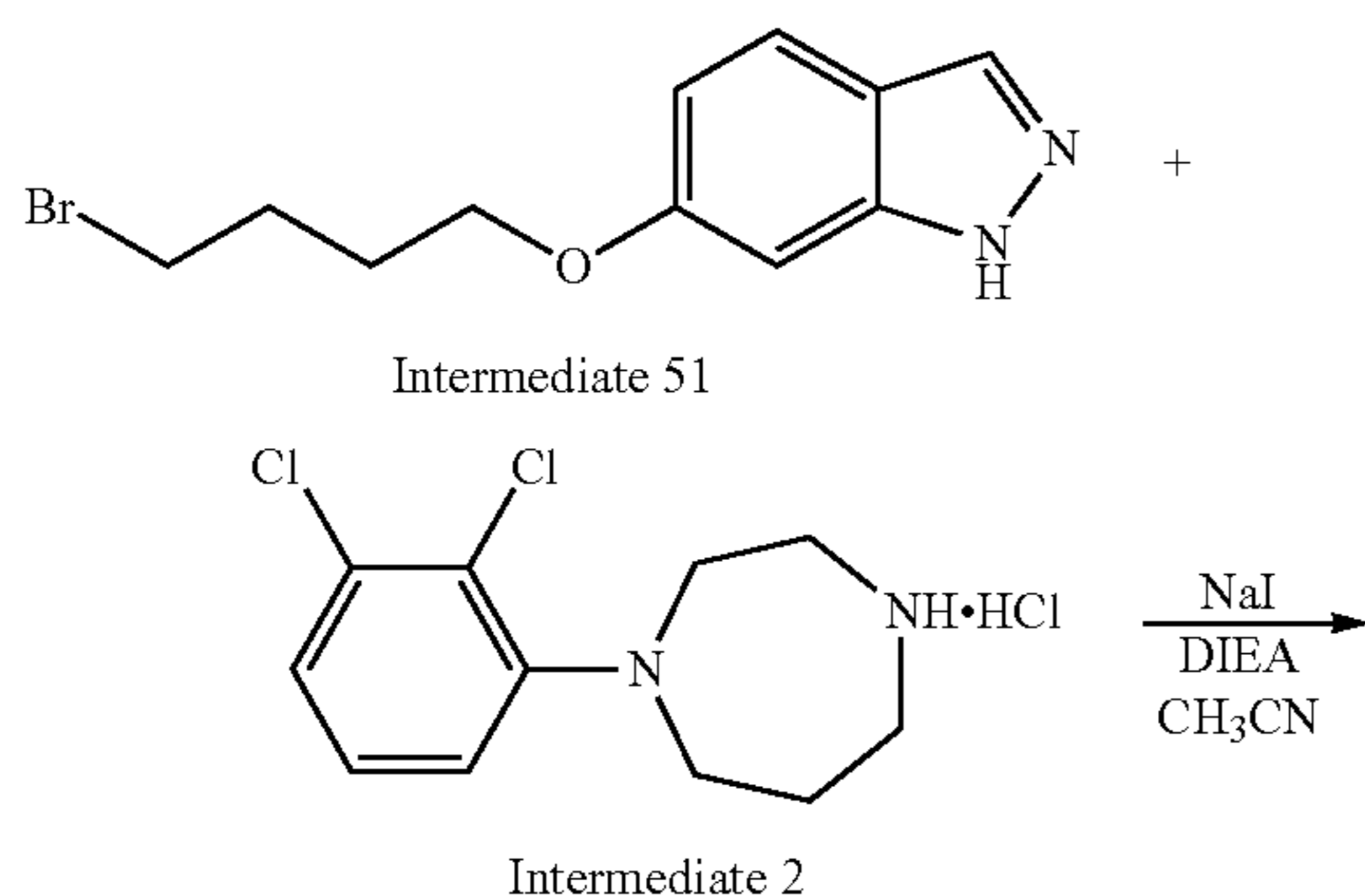
Scheme 74. Synthesis of compound 47
