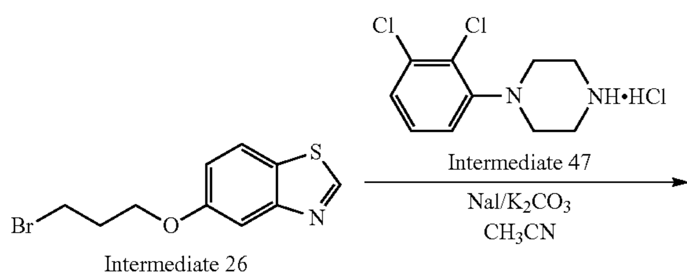
Scheme 39. Synthesis of compound 22
