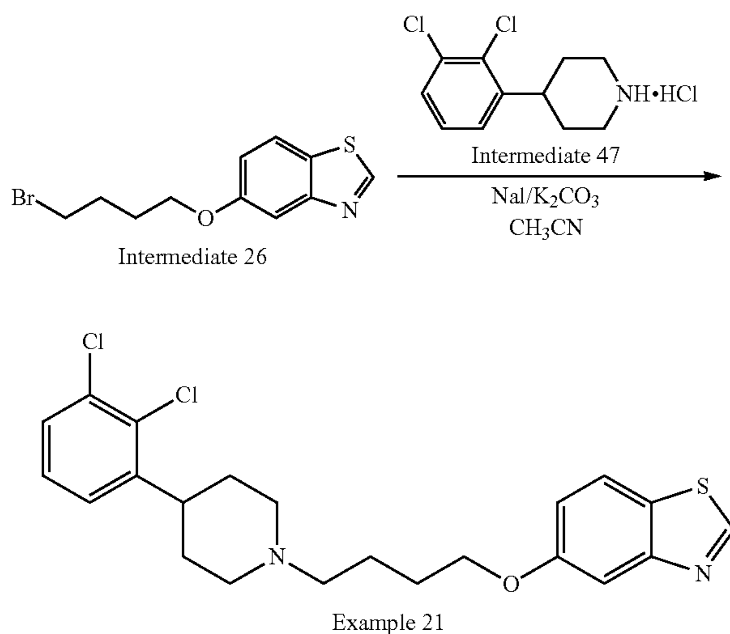
Scheme 38. Synthesis of compound 21
