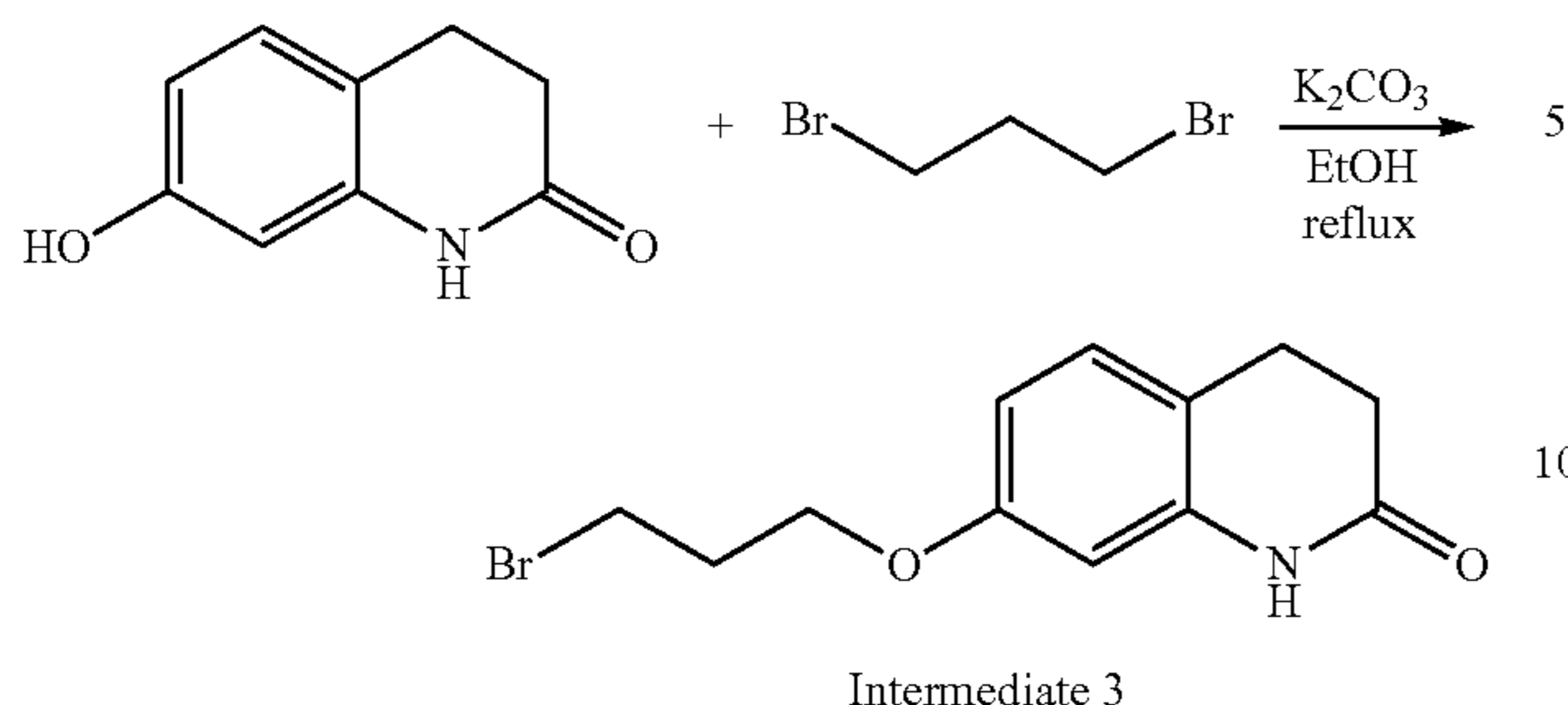
Scheme 2. Synthesis of intermediate 3
