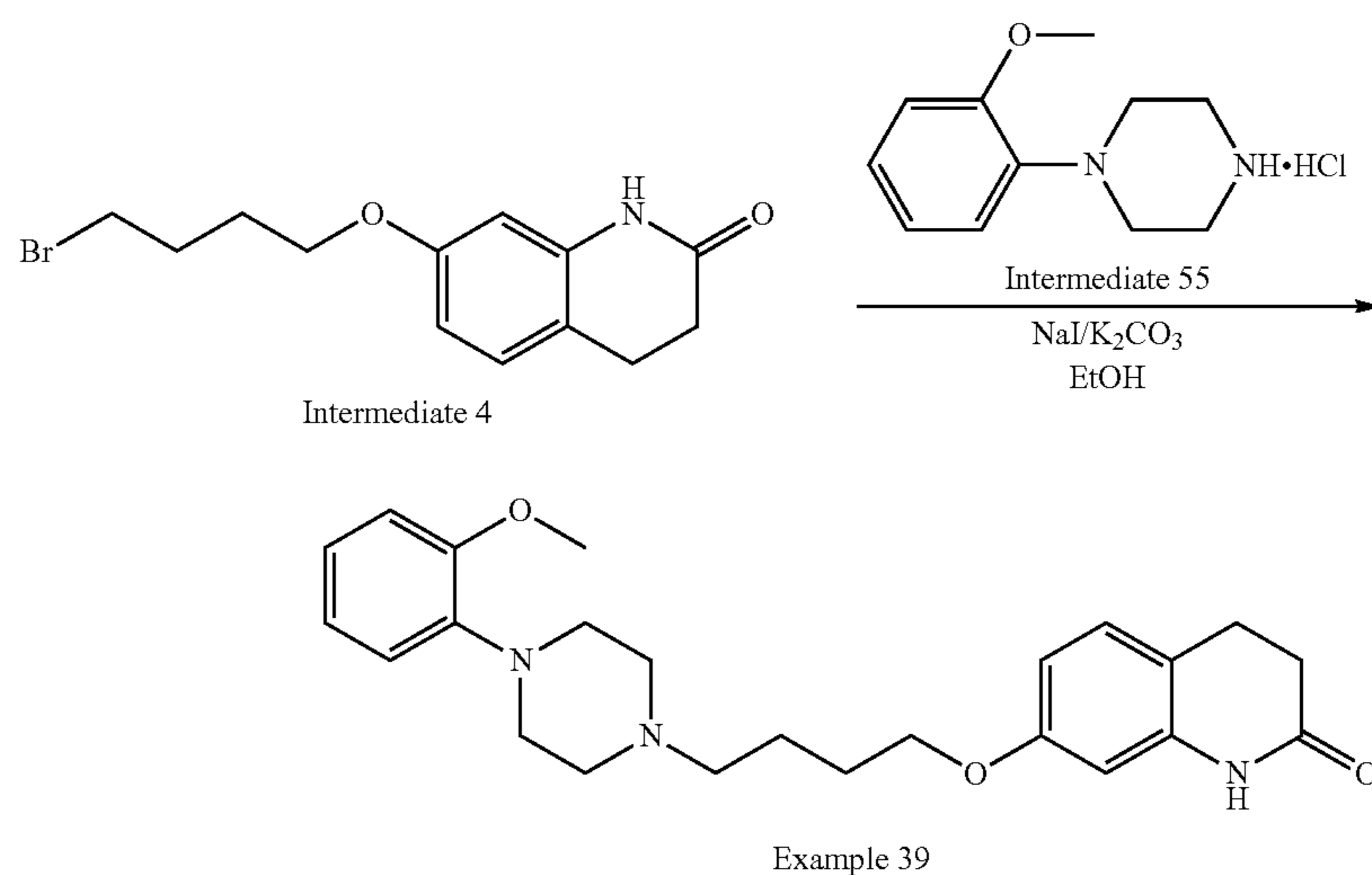
Scheme 65. Synthesis of compound 39
