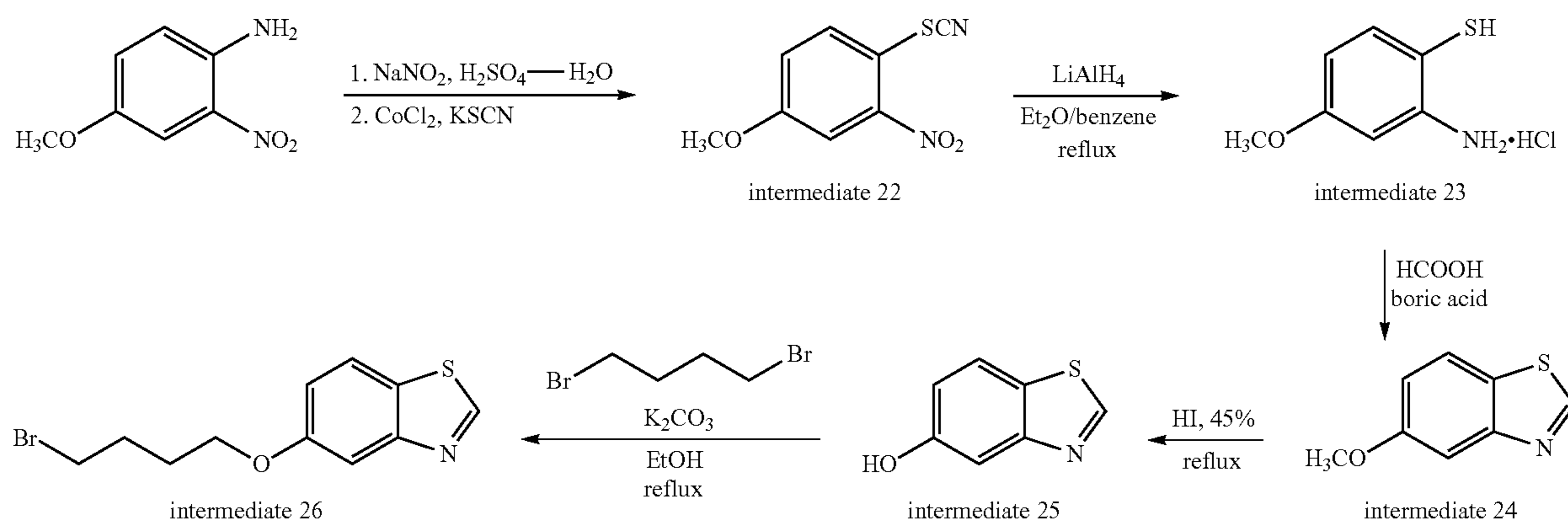
Scheme 14. Synthesis of intermediate 26
