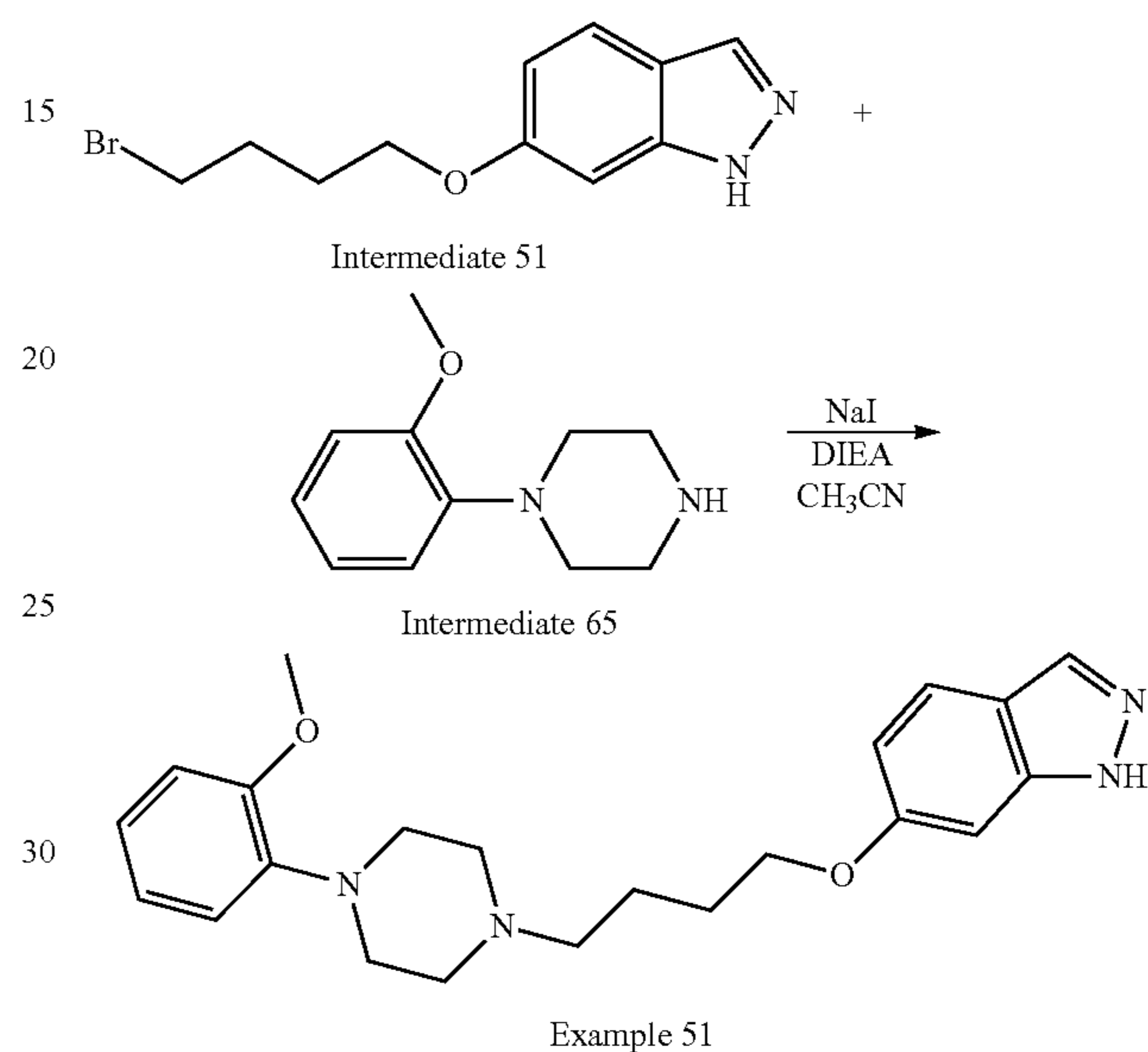
Scheme 79. Synthesis of compound 51
