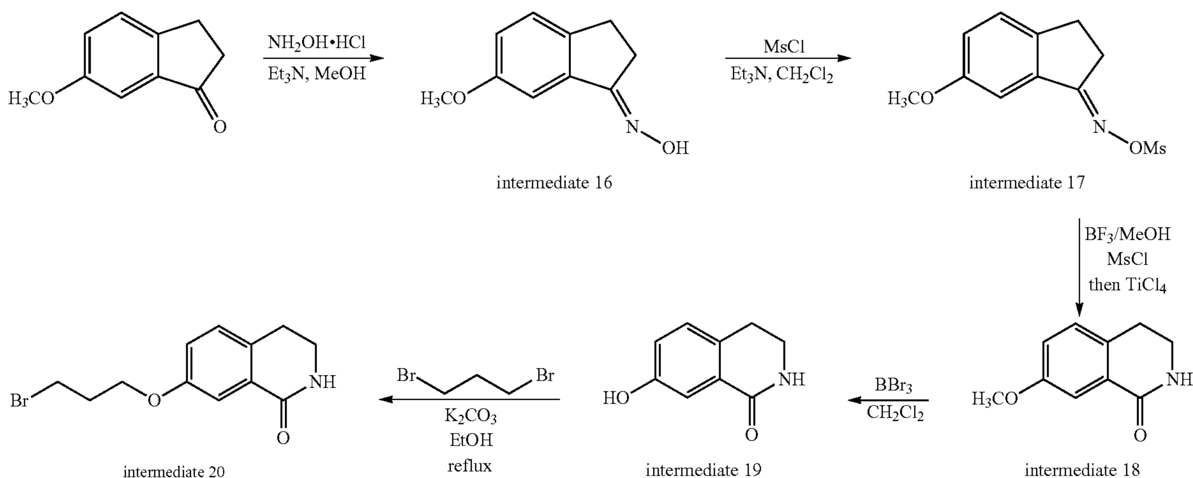
Scheme 10. Synthesis of intermediate 20
