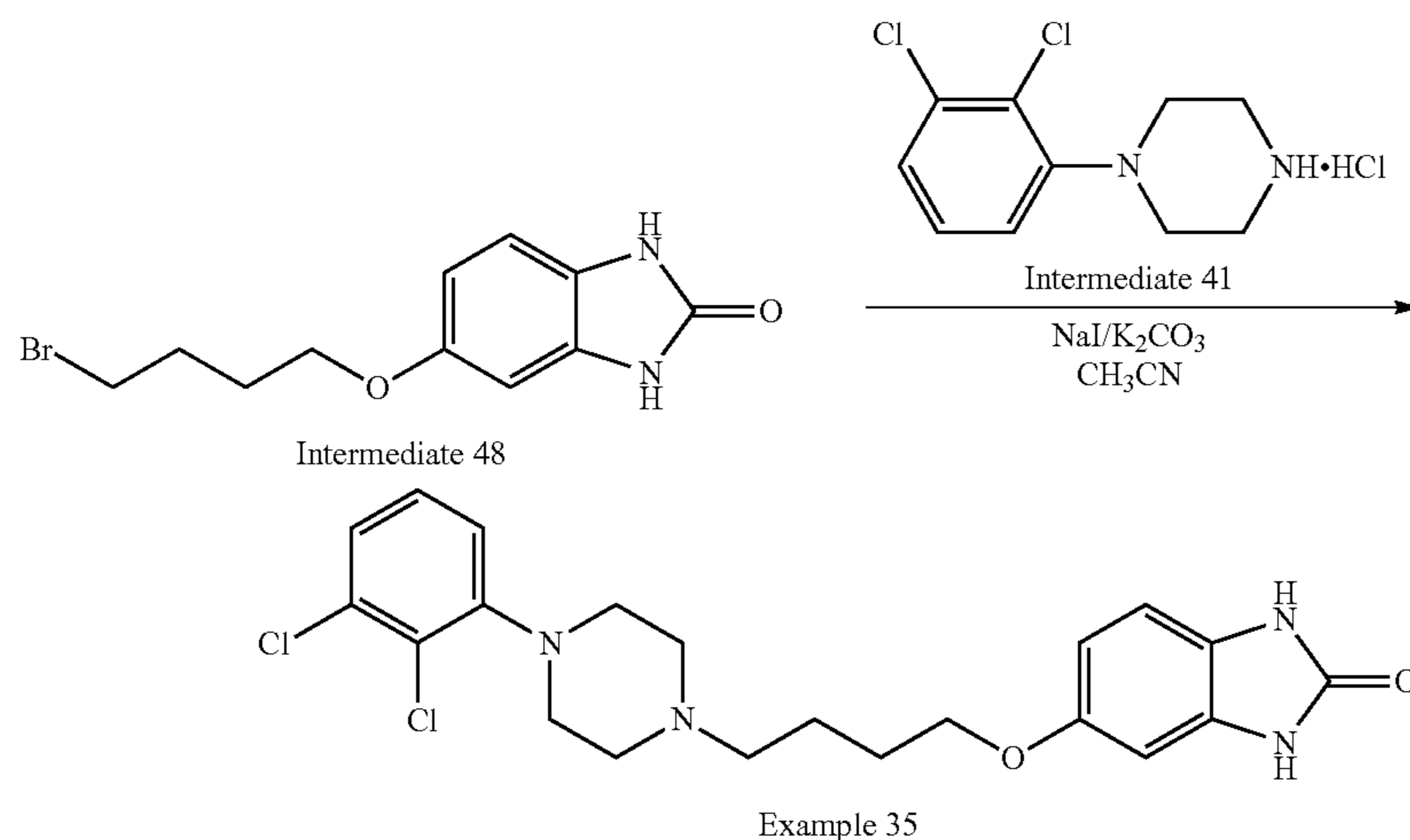
Scheme 59. Synthesis of compound 35
