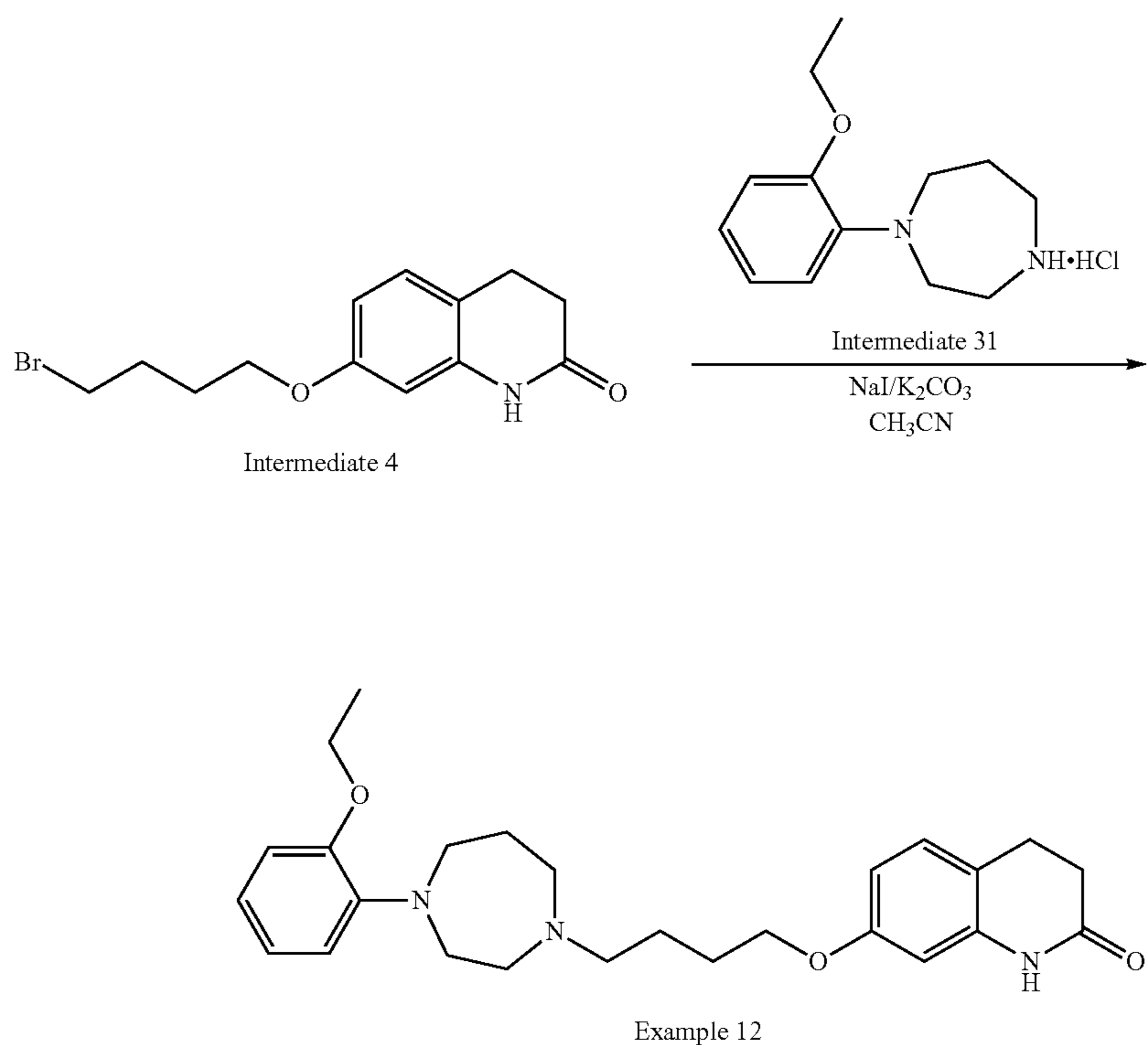
Scheme 23. Synthesis of compound 12
