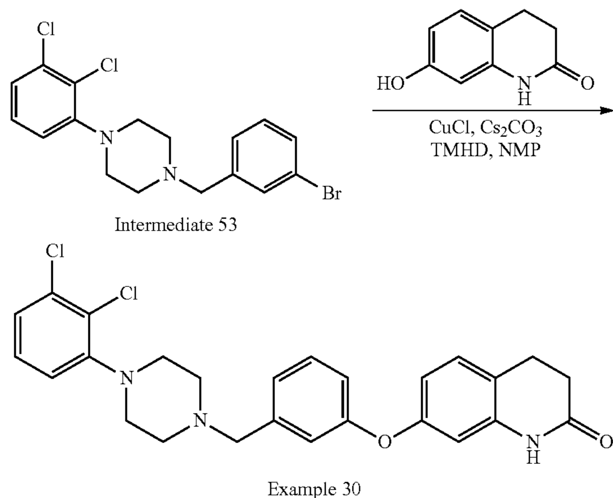
Scheme 53. Synthesis of compound 30
