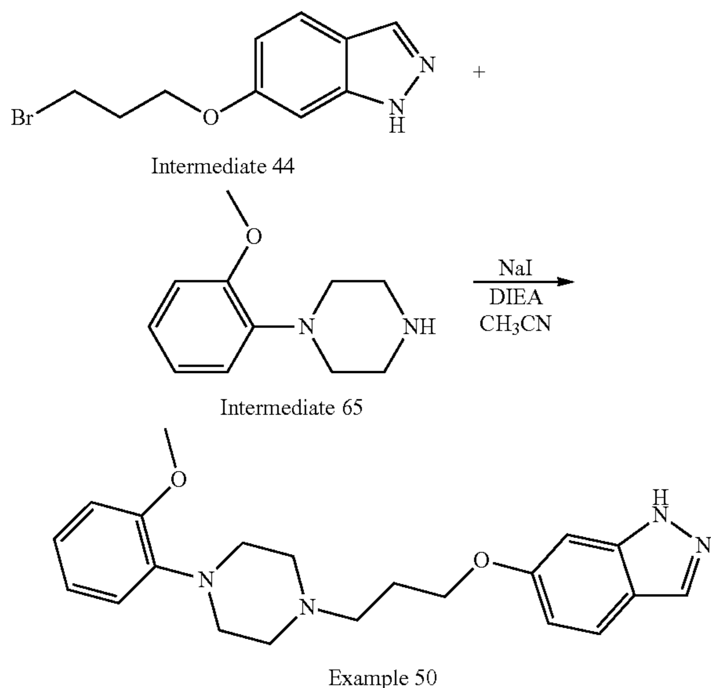
Scheme 78. Synthesis of compound 50
