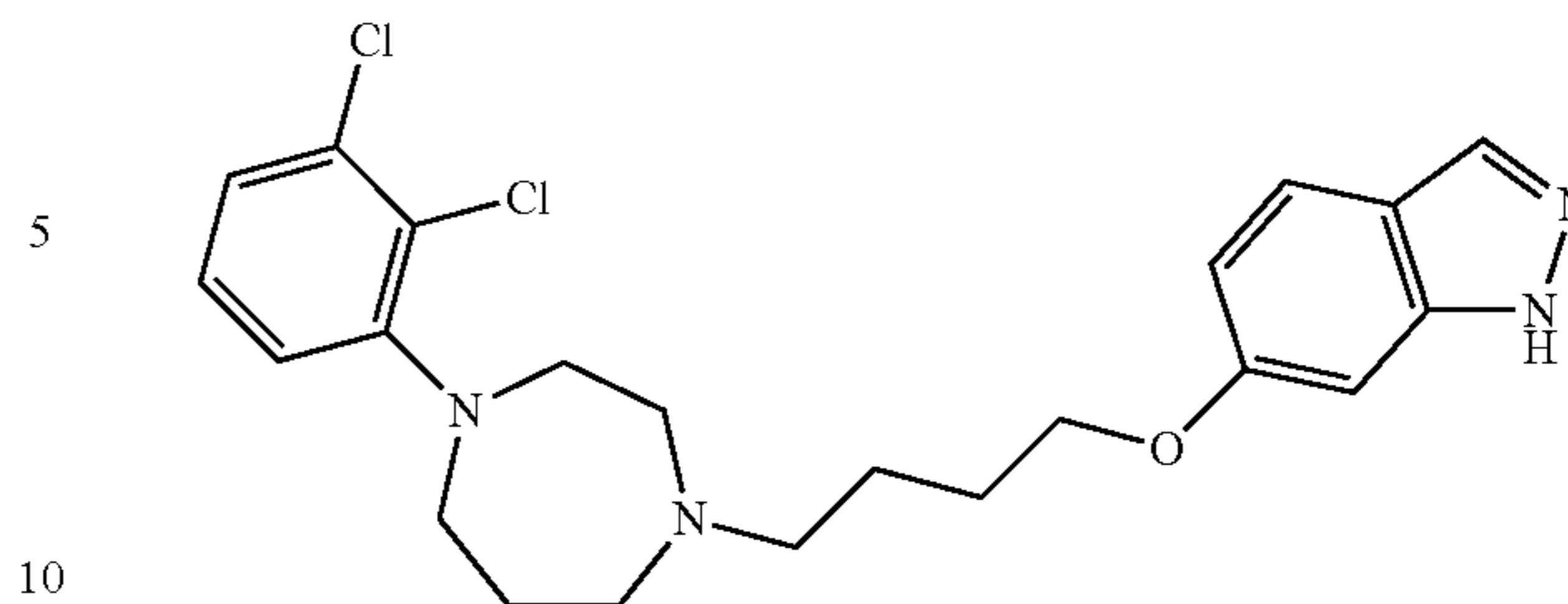
Example 47
