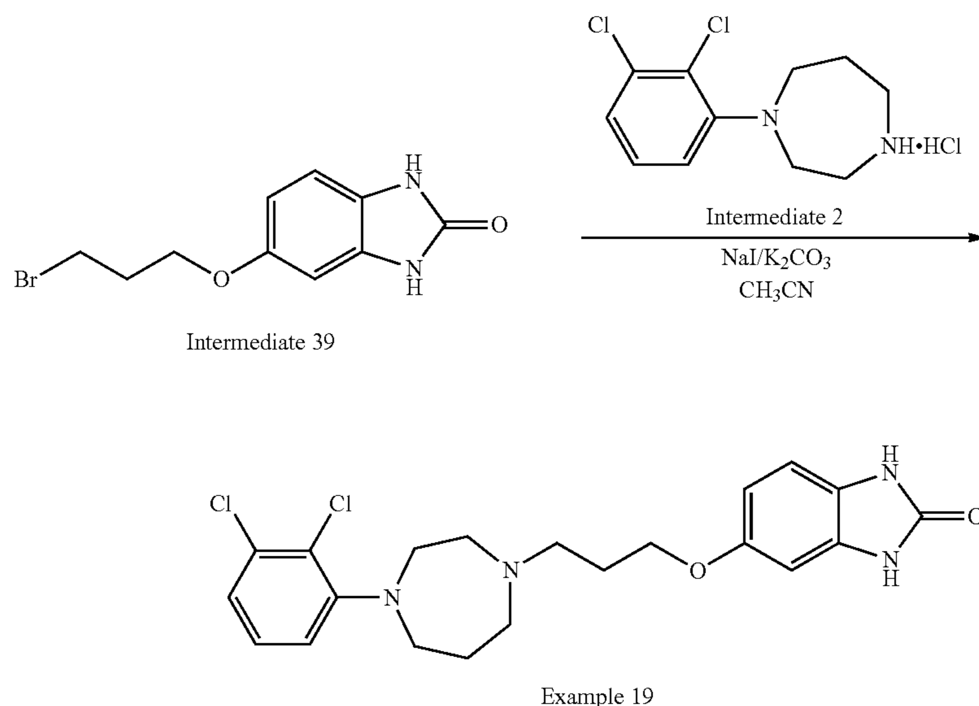
Scheme 33. Synthesis of compound 19
