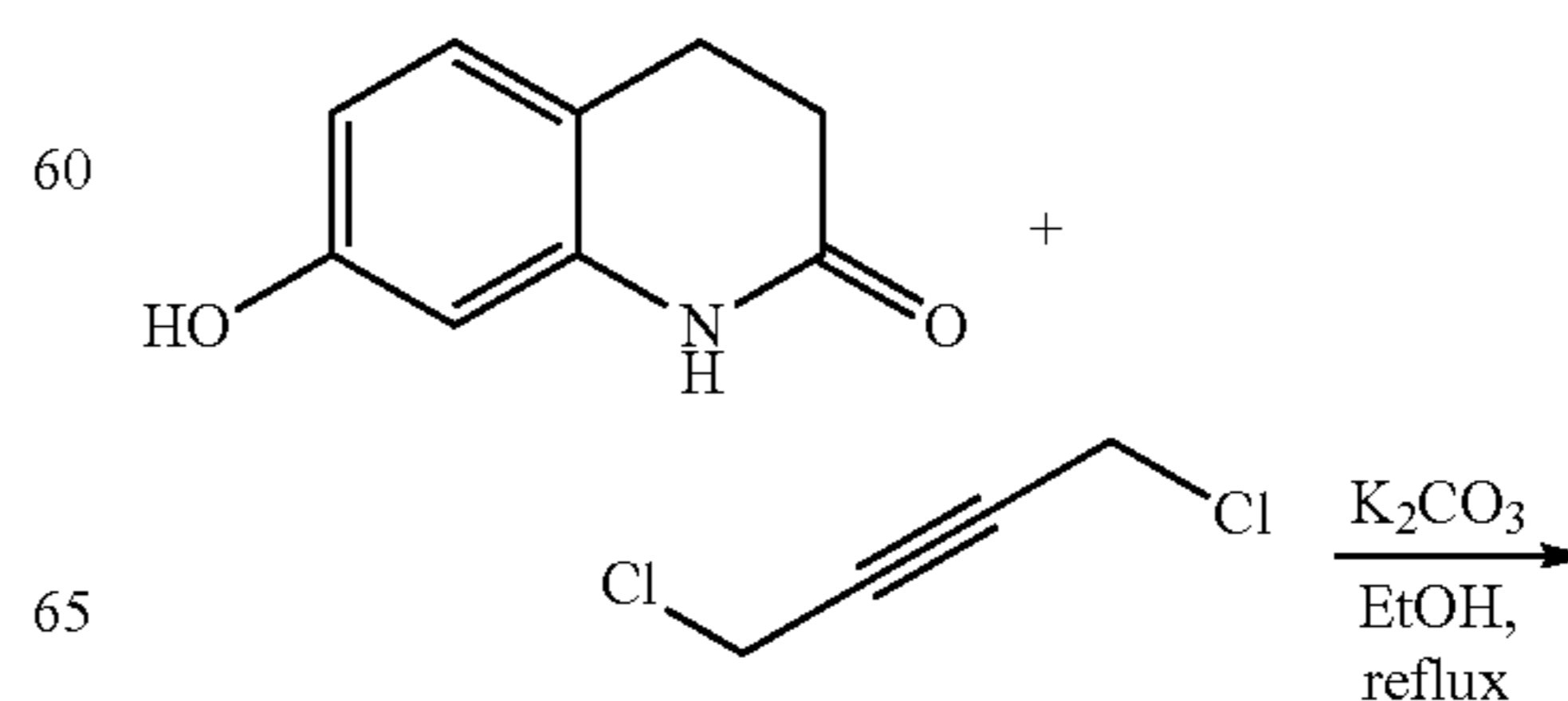
Scheme 46. Synthesis of intermediate 50
