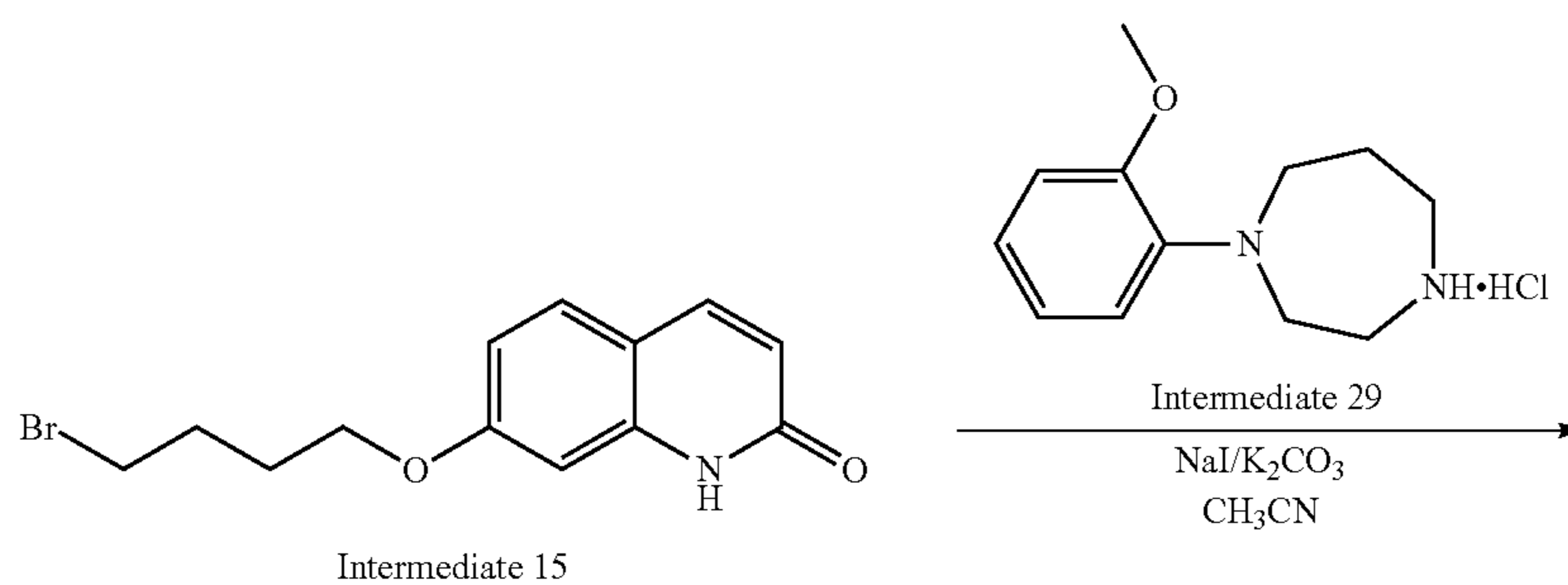
Scheme 20. Synthesis of compound 10
