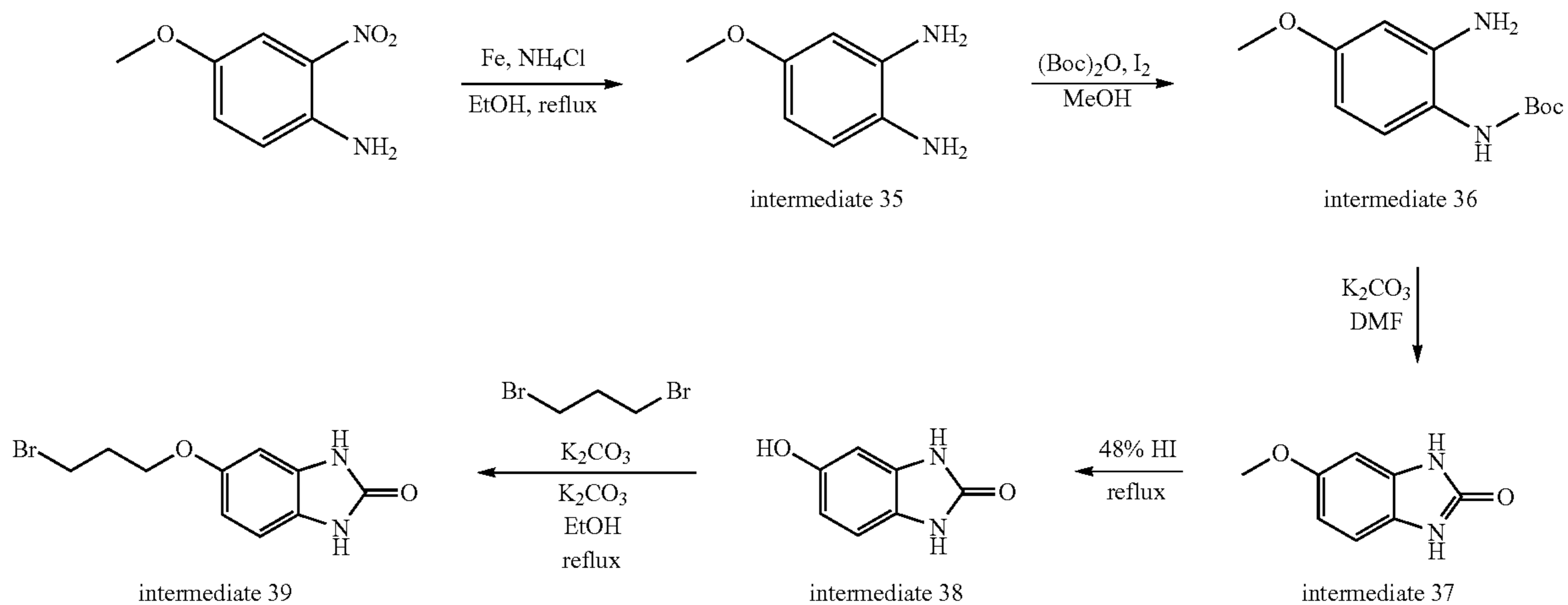
Scheme 32. Synthesis of intermediate 39
