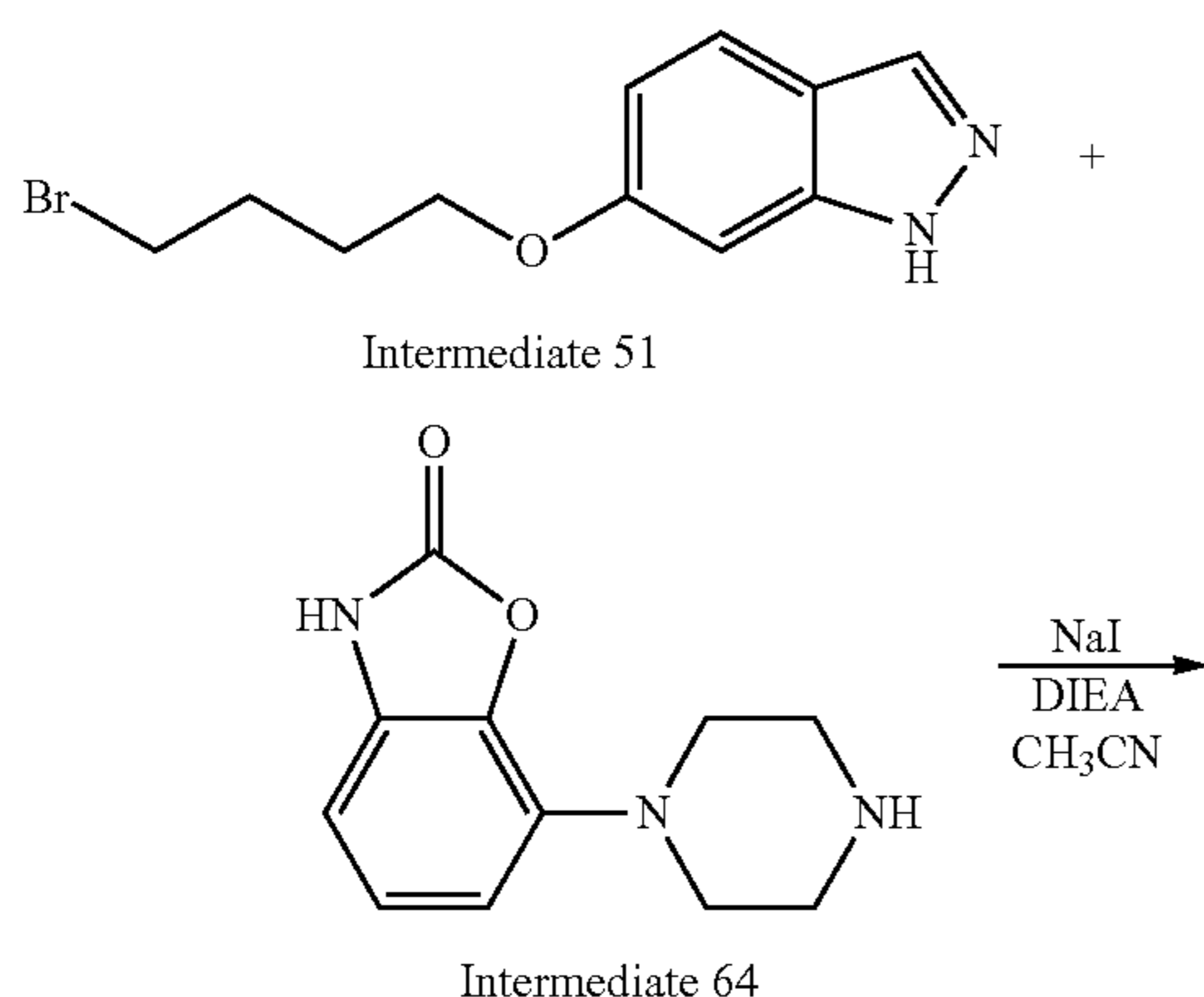
Scheme 76. Synthesis of compound 49
