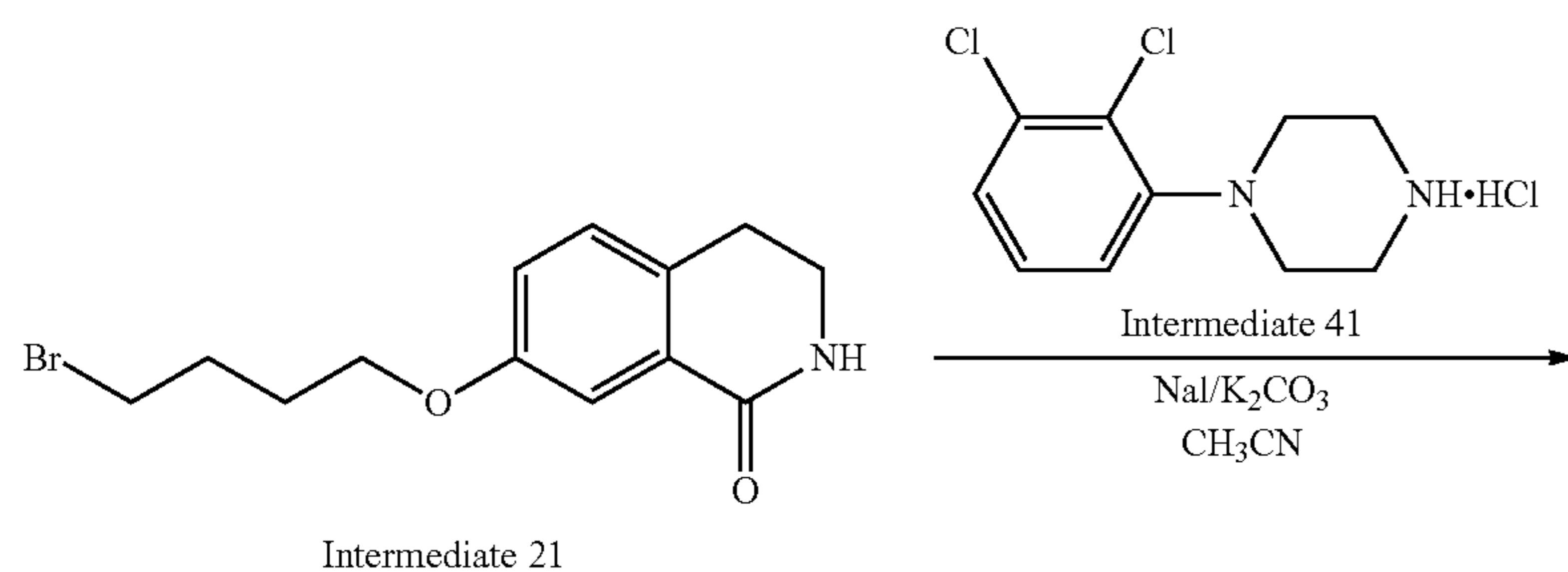
Scheme 43. Synthesis of compound 25
