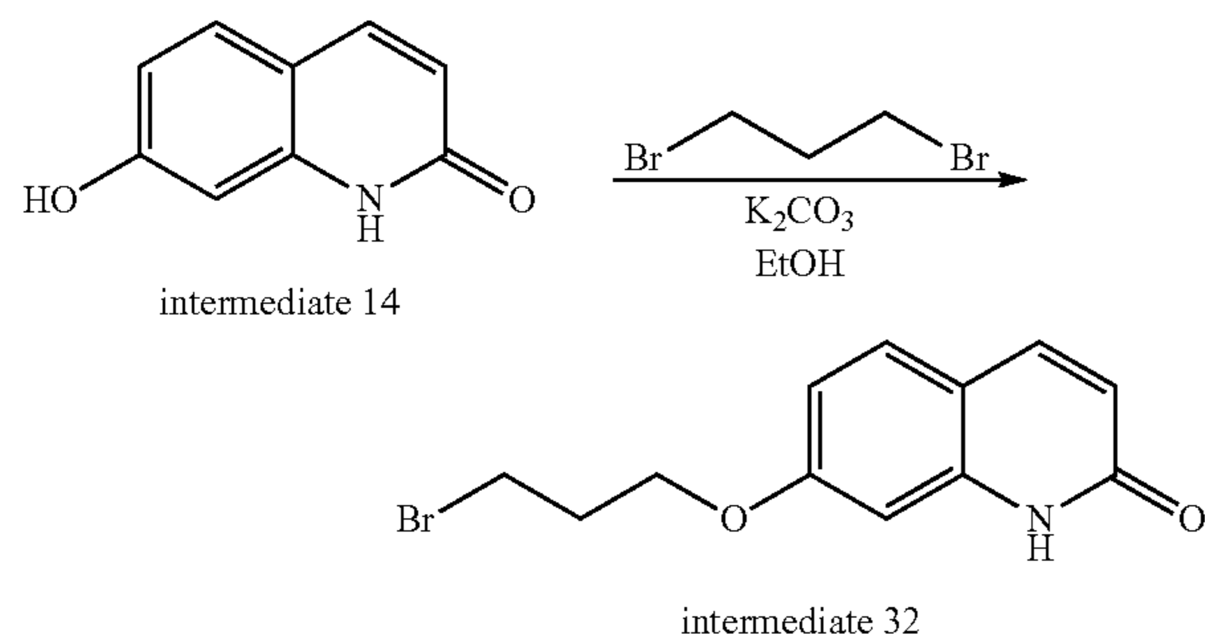
Scheme 26. Synthesis of intermediate 32
