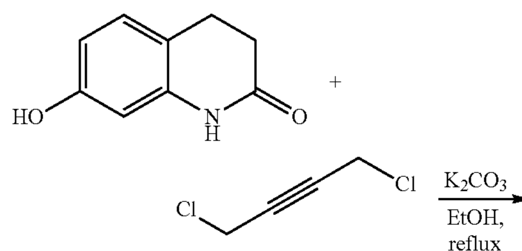
Scheme 46. Synthesis of intermediate 50
