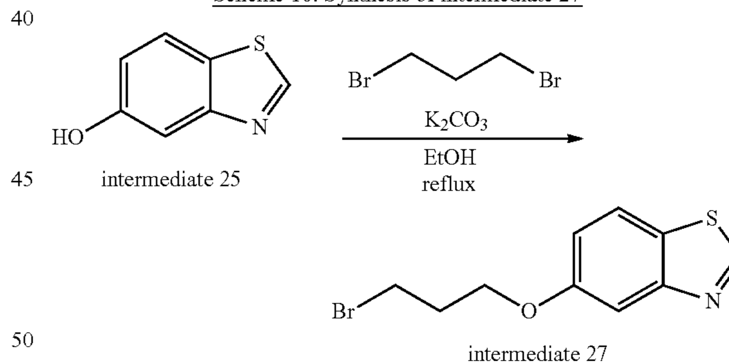
Scheme 16. Synthesis of intermediate 27
