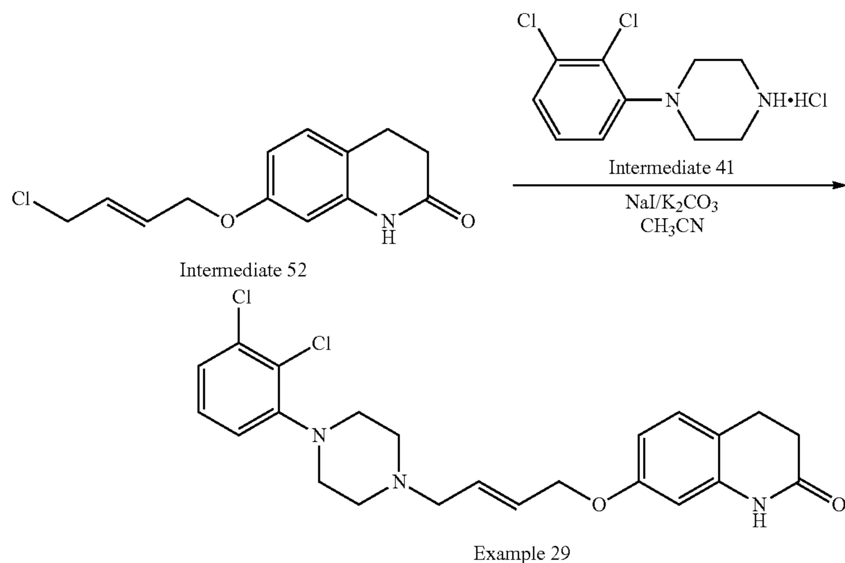
Scheme 51. Synthesis of compound 29
