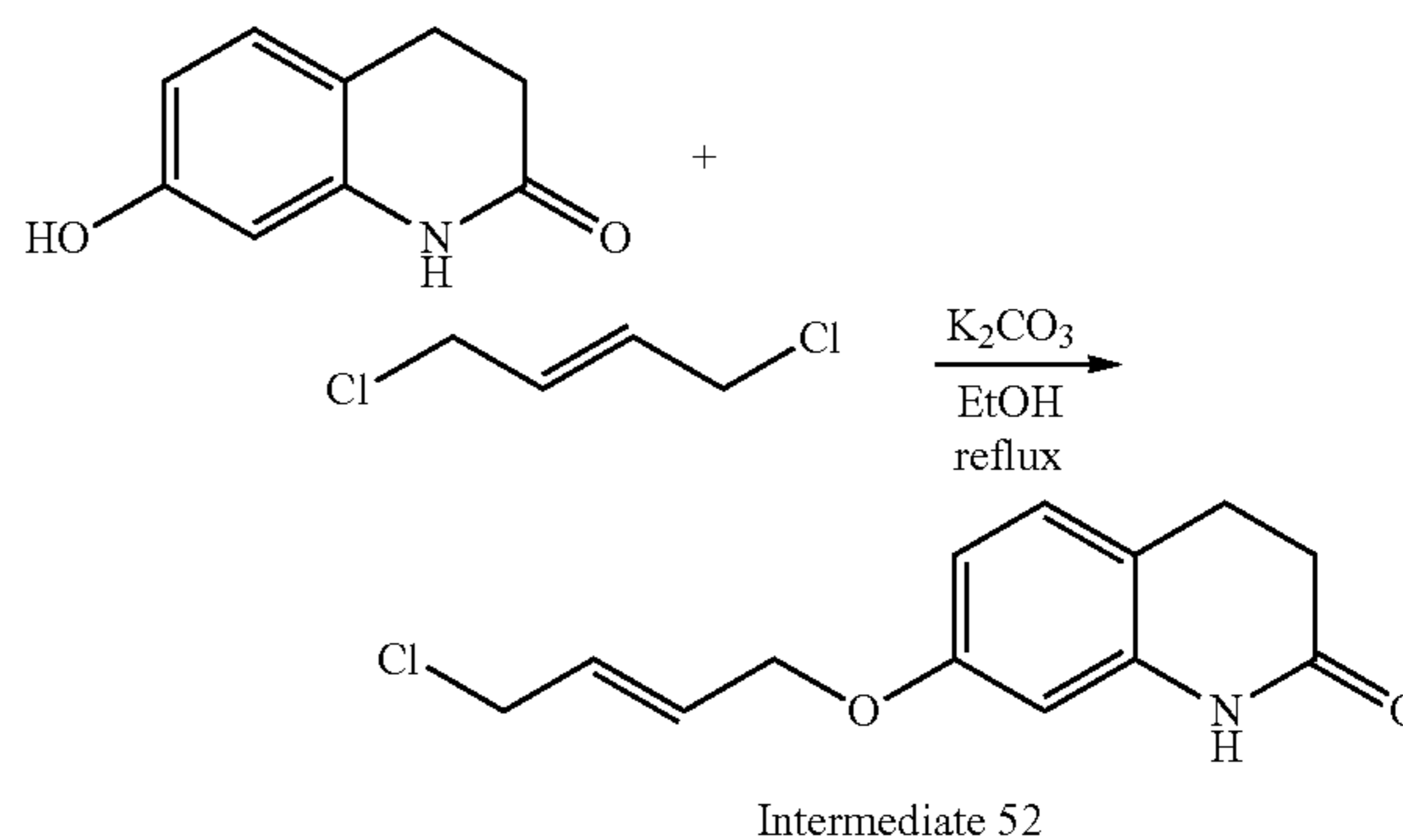
Scheme 50. Synthesis of intermediate 52
