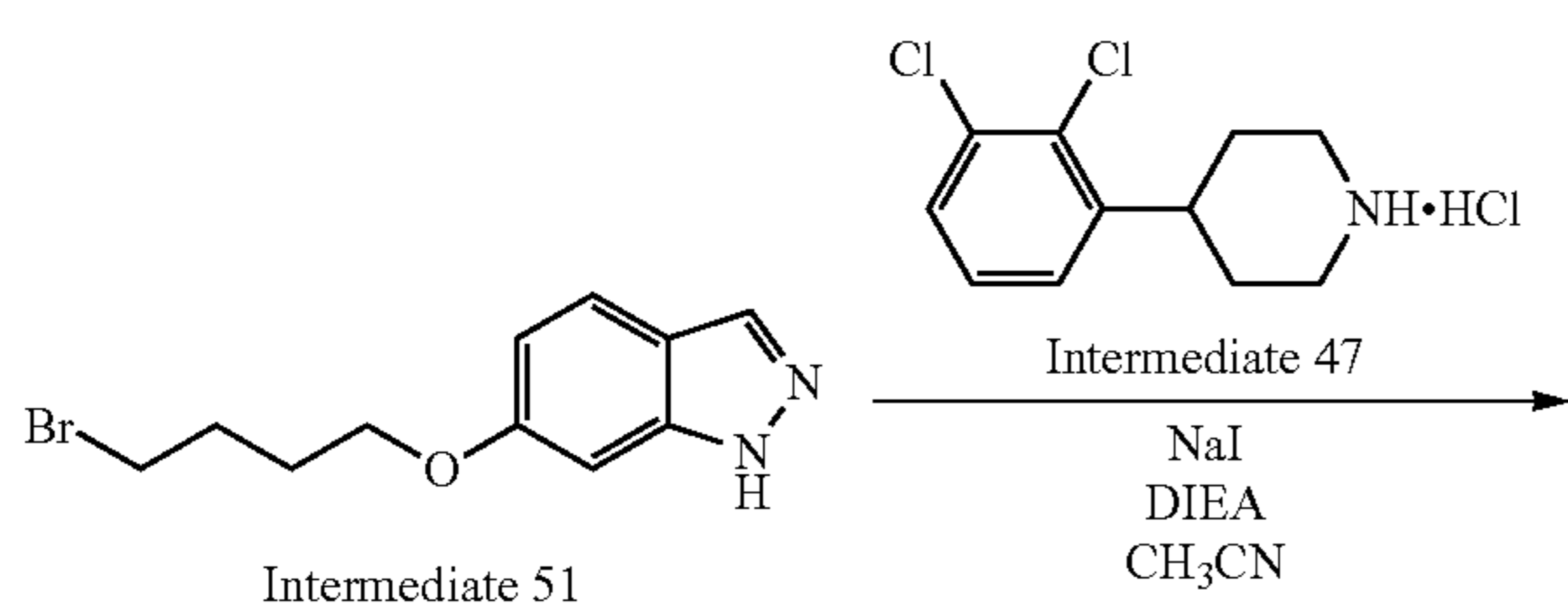
Scheme 72. Synthesis of compound 45
