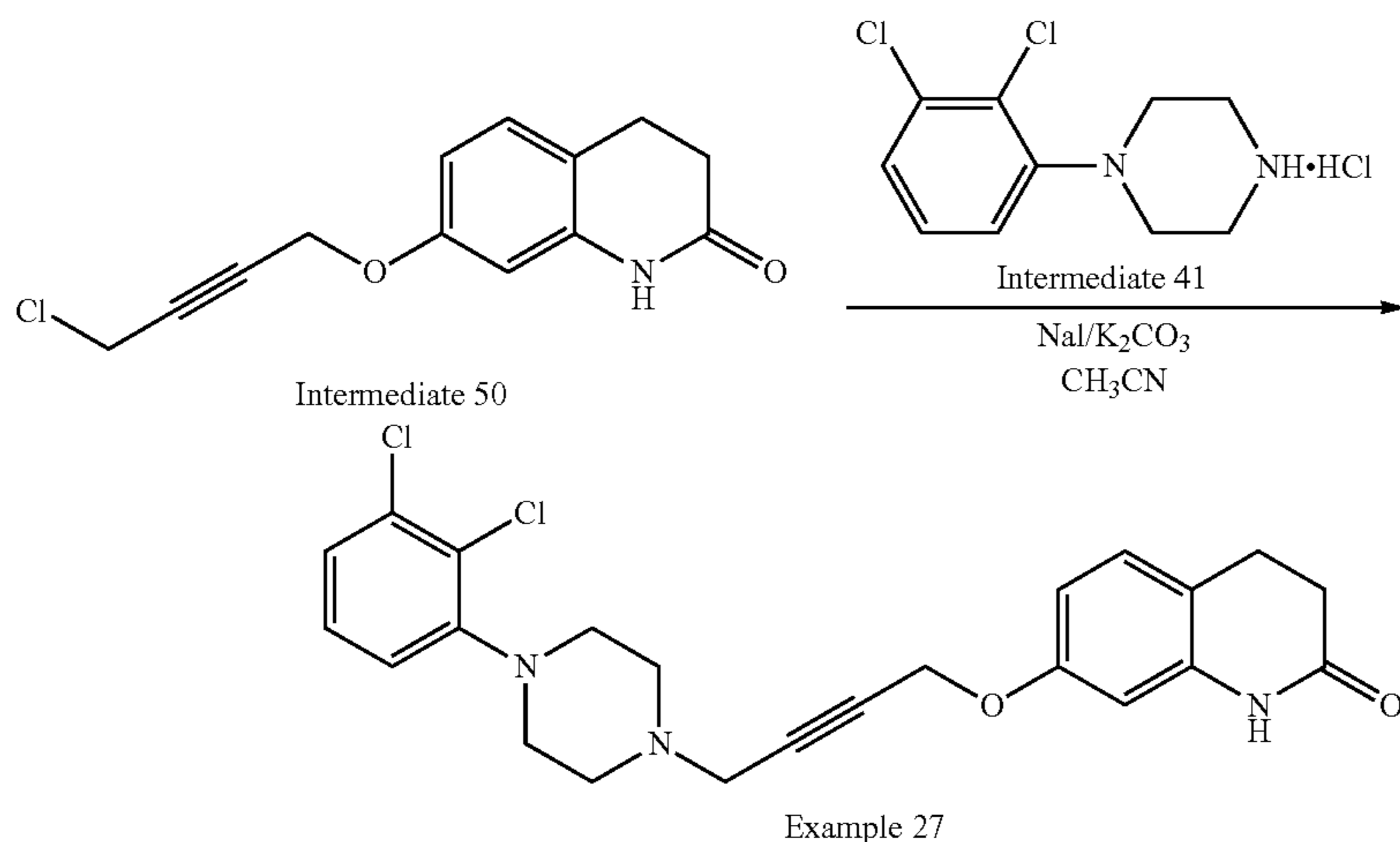
Scheme 47. Synthesis of compound 27
