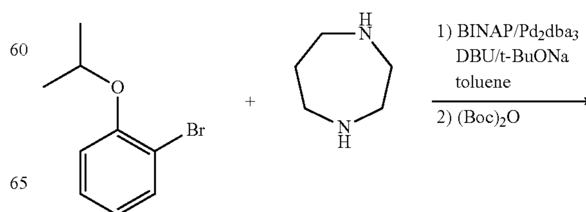
Scheme 28. Synthesis of intermediate 34
