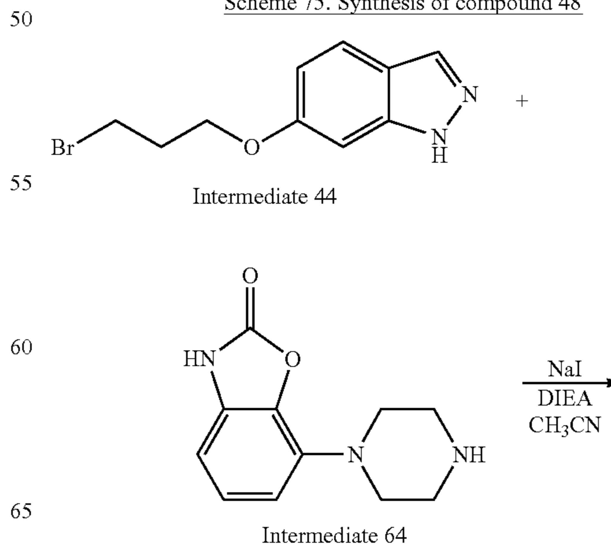
Scheme 75. Synthesis of compound 48
