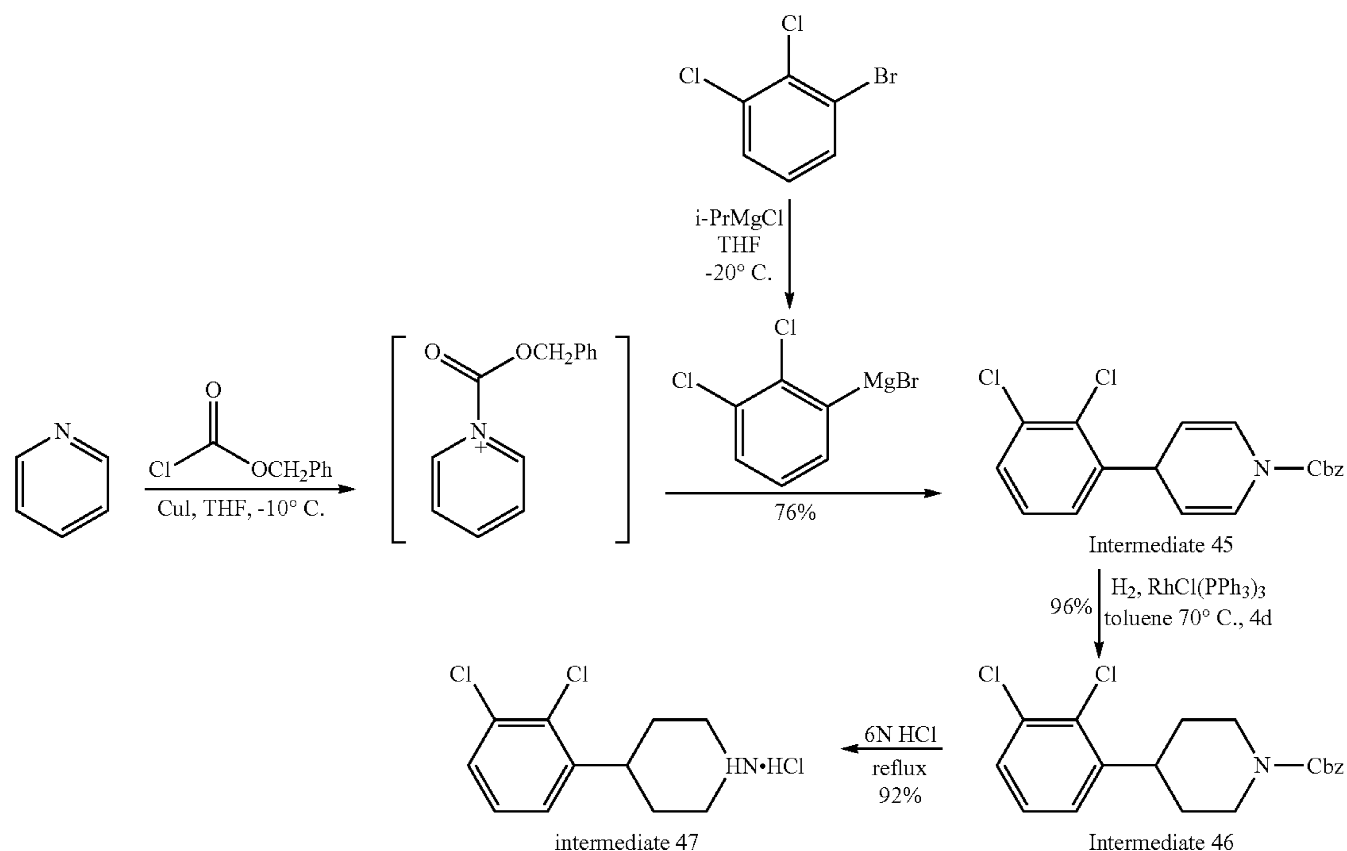
Scheme 37. Synthesis of intermediate 47
