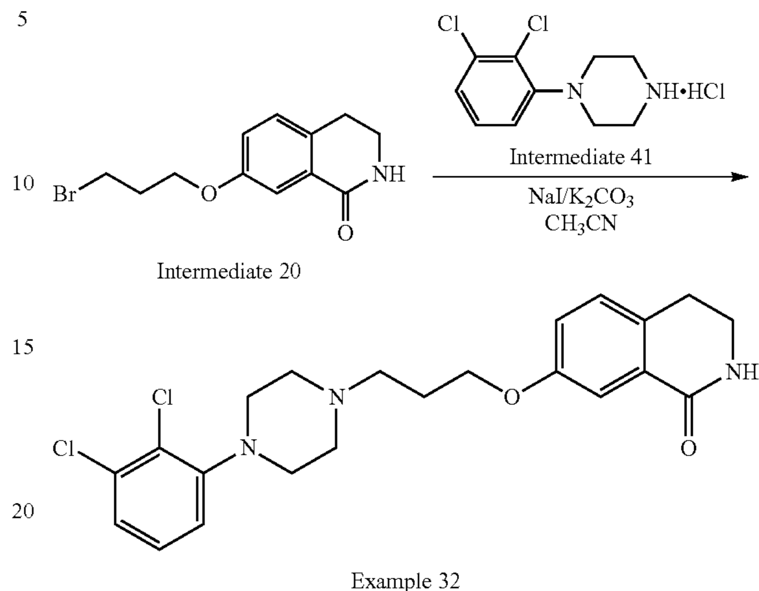
Scheme 56. Synthesis of compound 32
