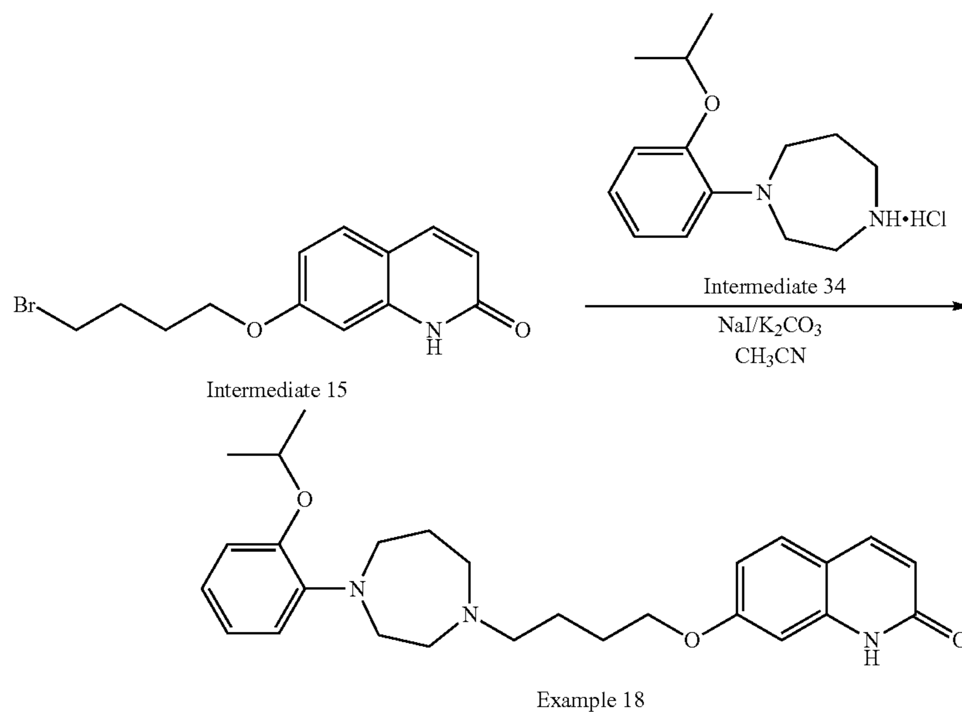
Scheme 31. Synthesis of compound 18
