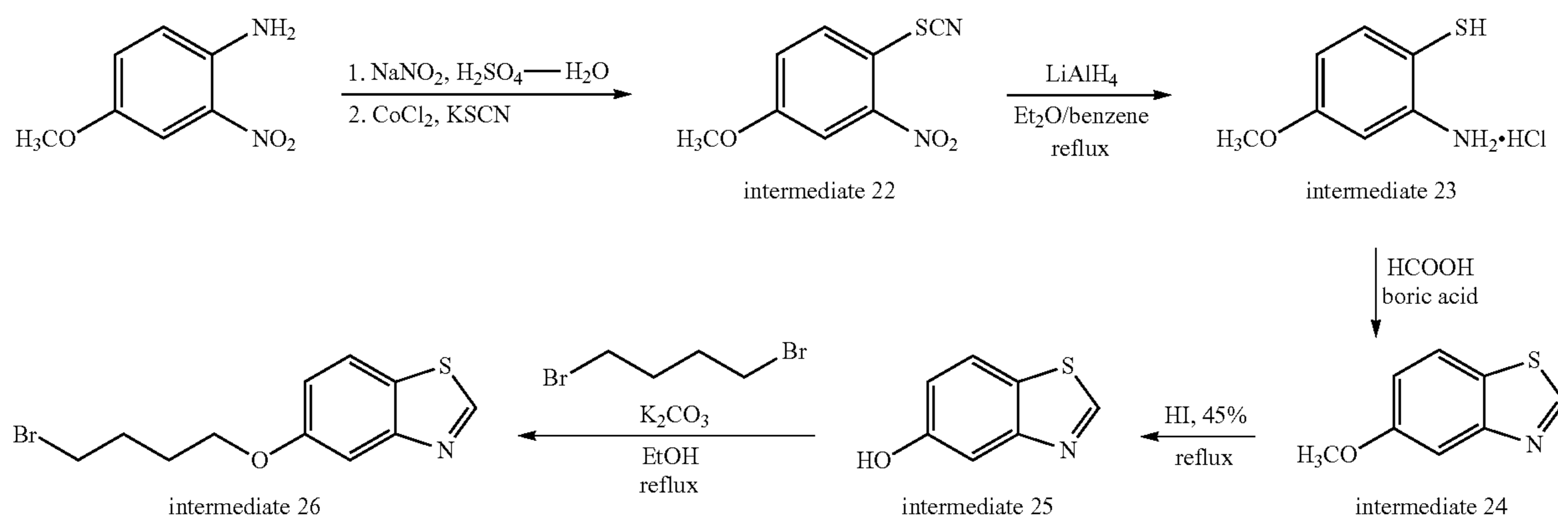
Scheme 14. Synthesis of intermediate 26
