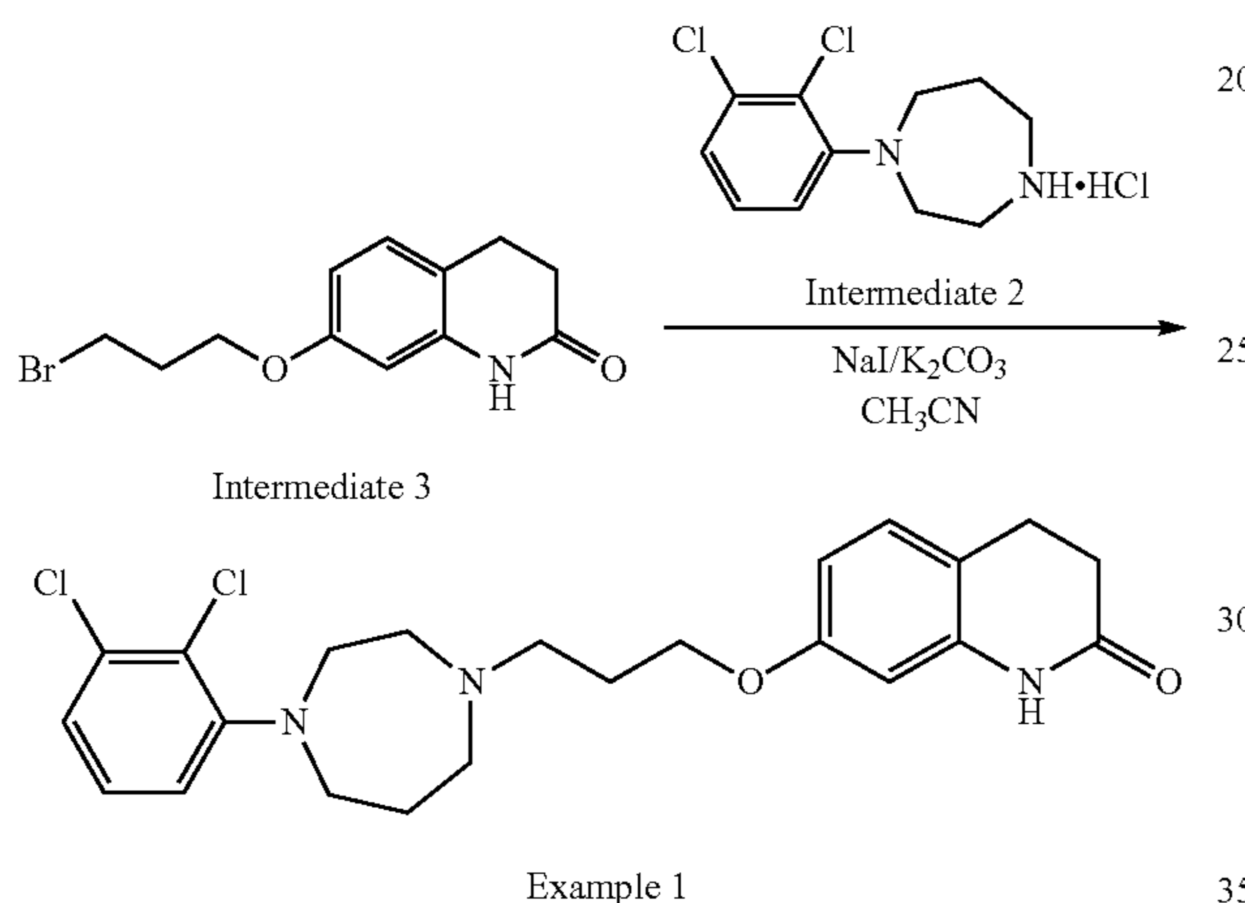
Scheme 3. Synthesis of compound 1
