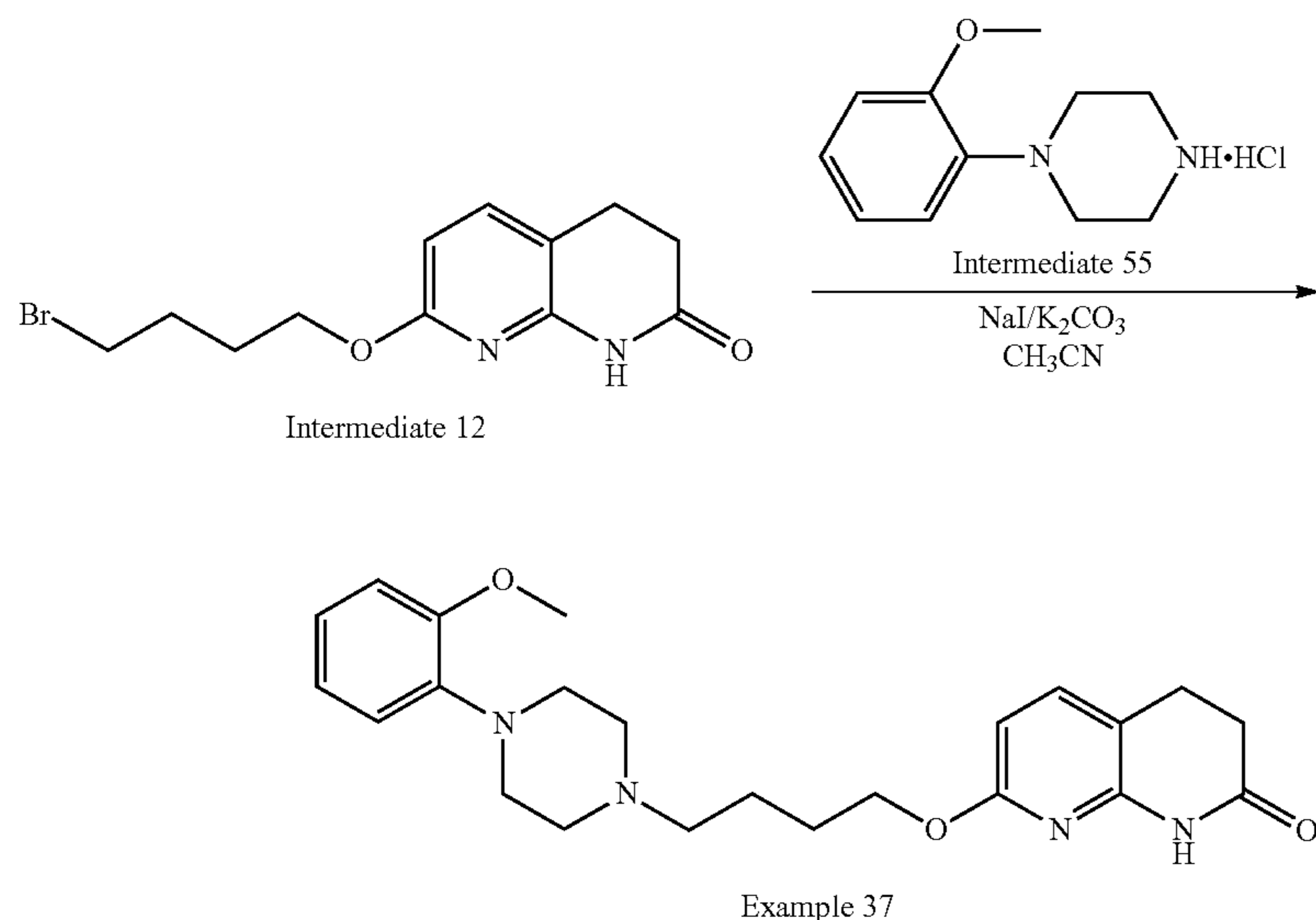
Scheme 62. Synthesis of compound 37
