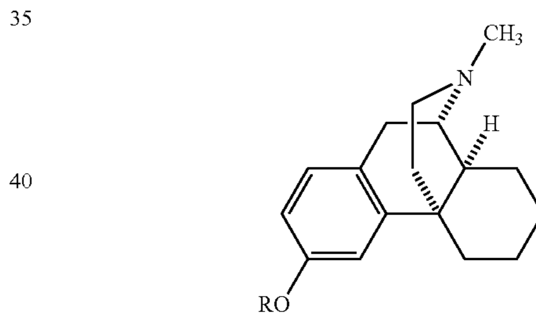
Dextromethorphan; R = CH 3 Dextrorphan; R = H (note "opposite" stereochemistry)
