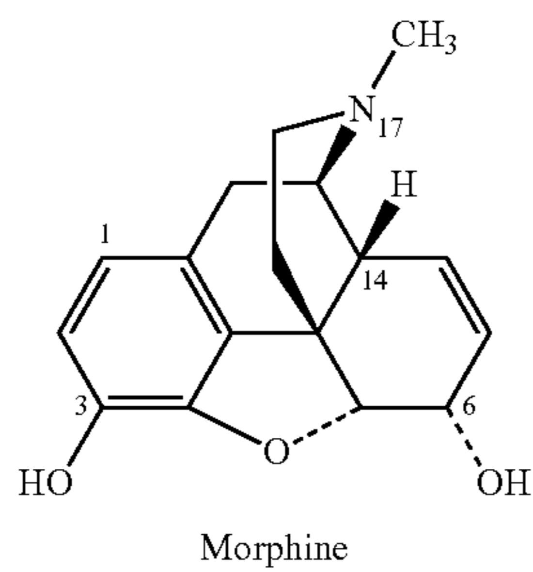
Chart 2. Opioid Receptor Ligands Morphine and Morphinans
