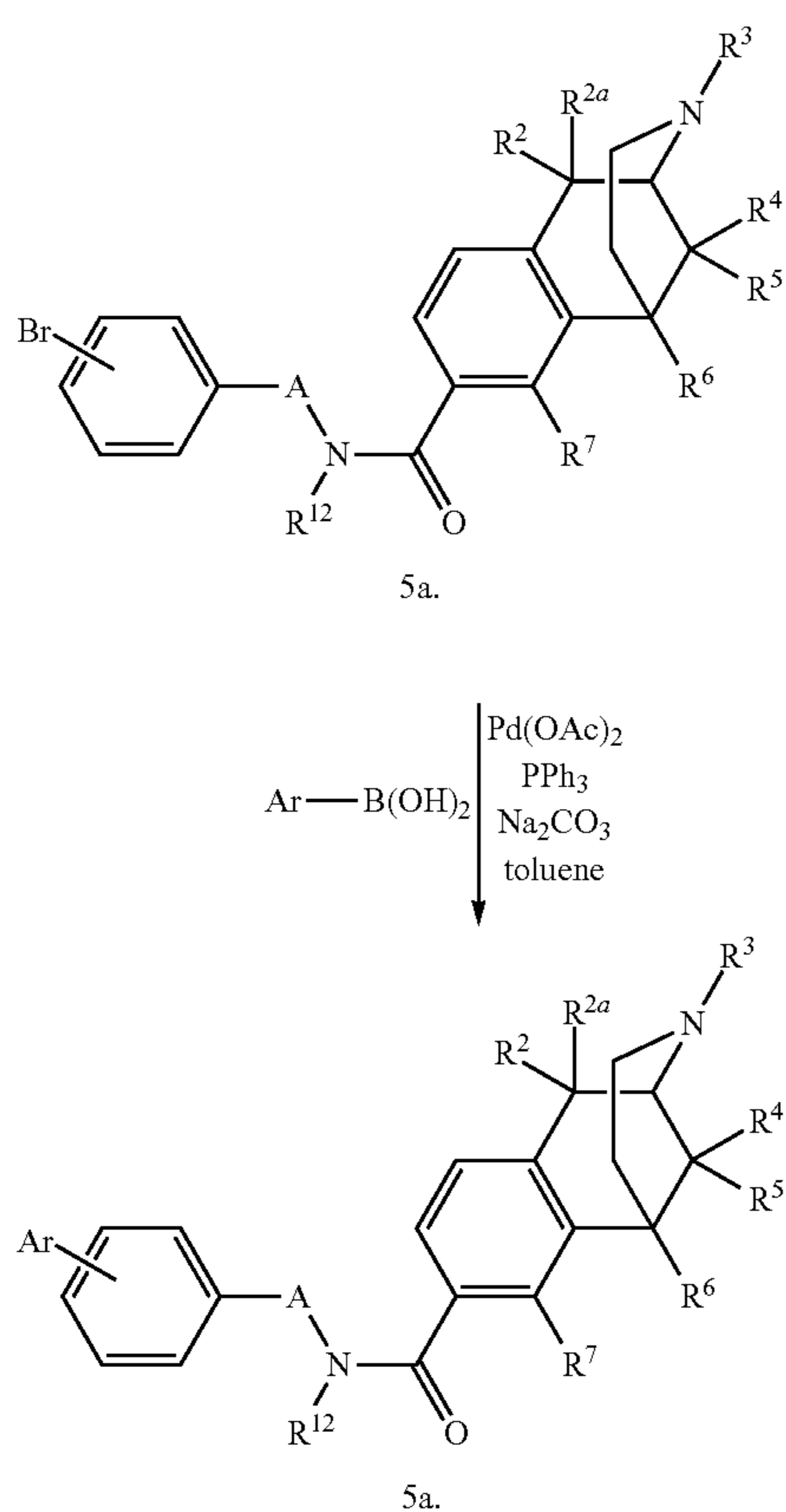
Scheme 3
