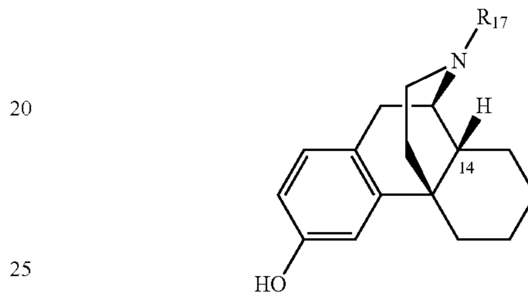
Levorphanol; R 17 = CH 3 Cyclophane; R 17 = CH 2 -c-C 3 H 5 MCL 101; R 17 = CH 2 -c-C 4 H 7 Butorphanol; R 17 = CH 2 -c-C 4 H 7 and 14-OH Merz-morphinane hybrid core; R 17 = CH 2 -(S)-tetrahydrofurfuryl
