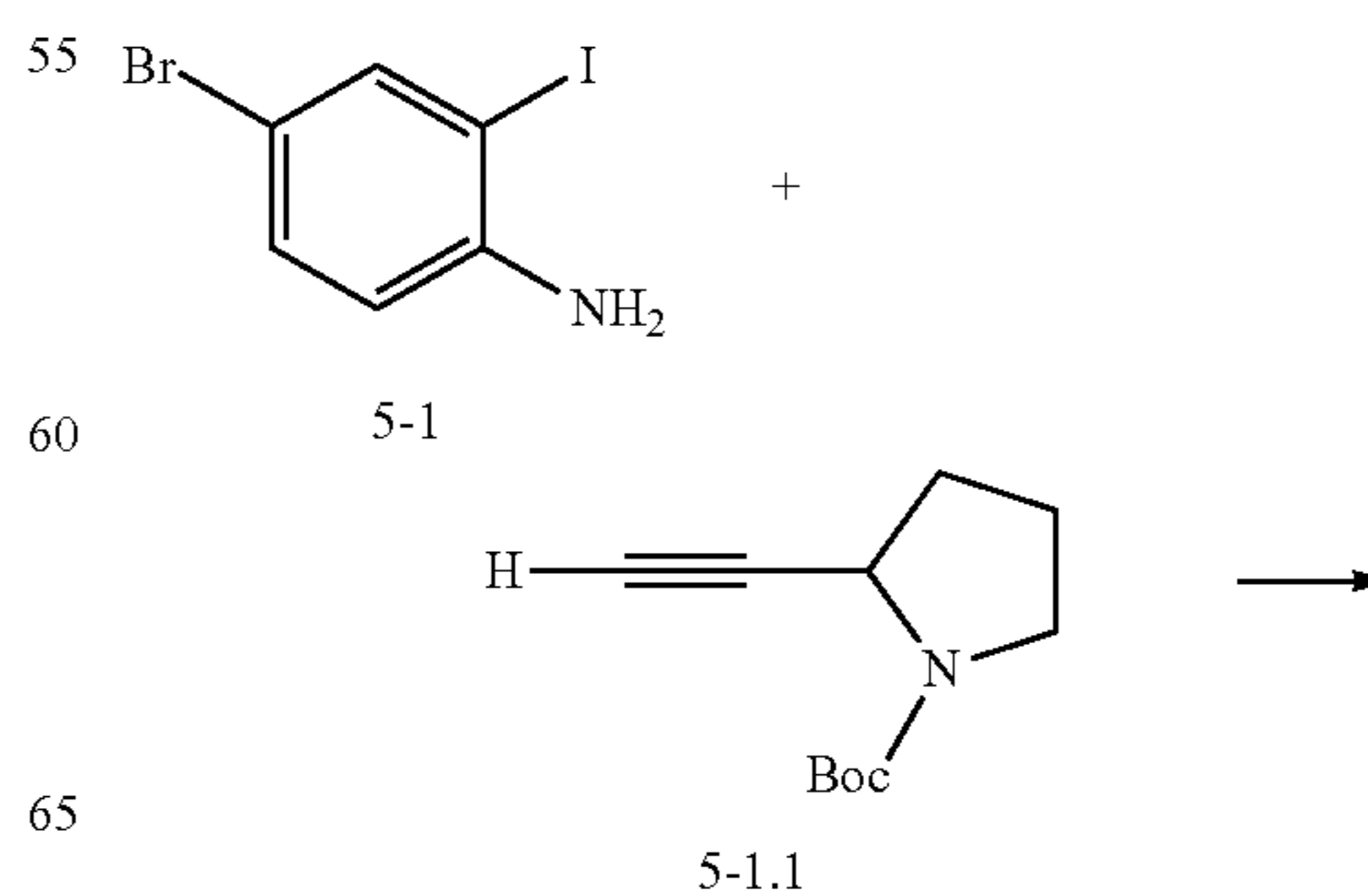
Scheme 5
