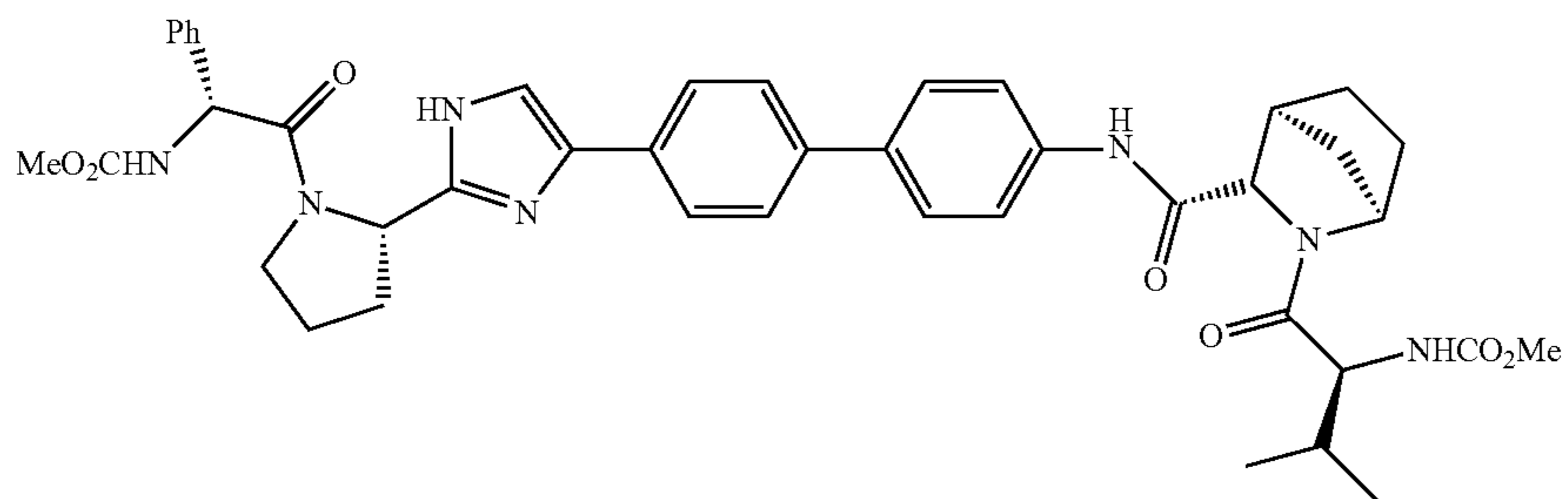
Examples 232-246
