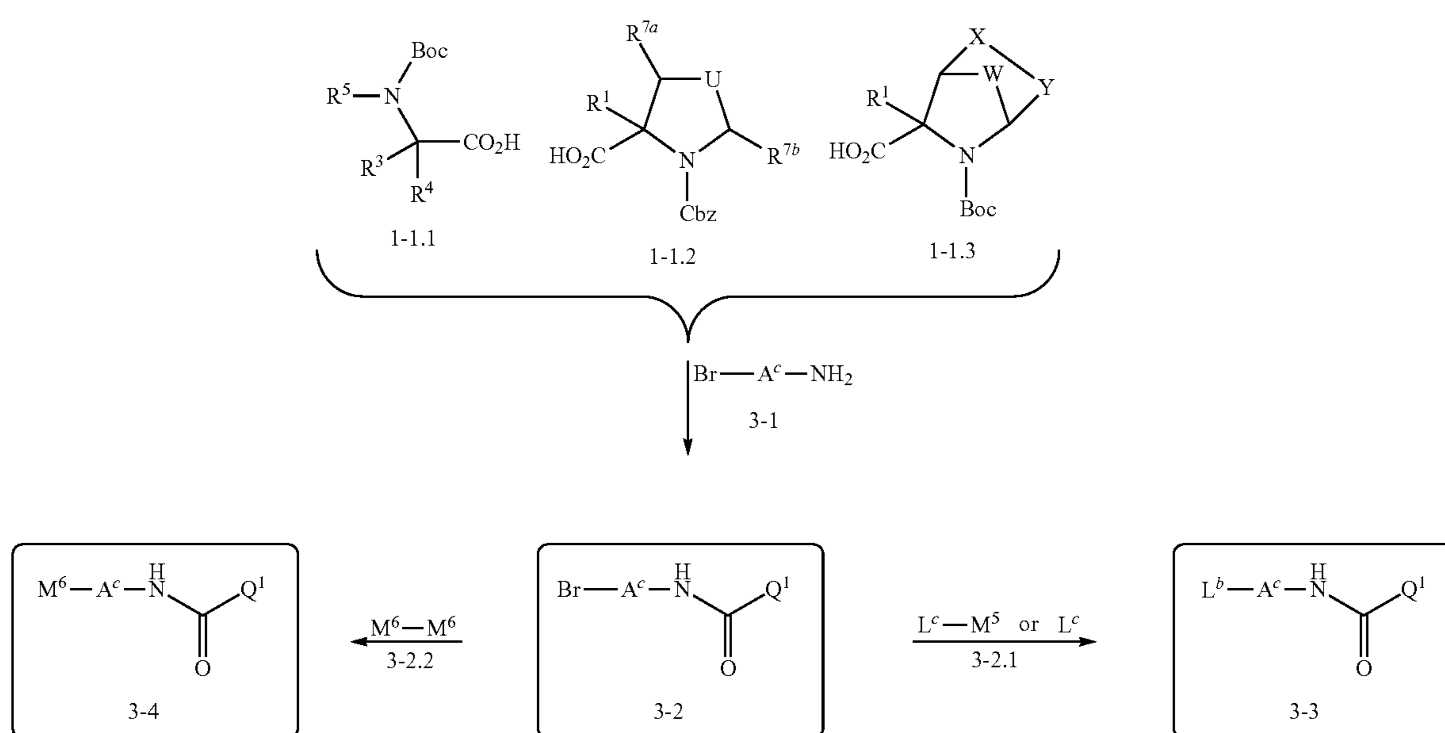
Scheme 3
