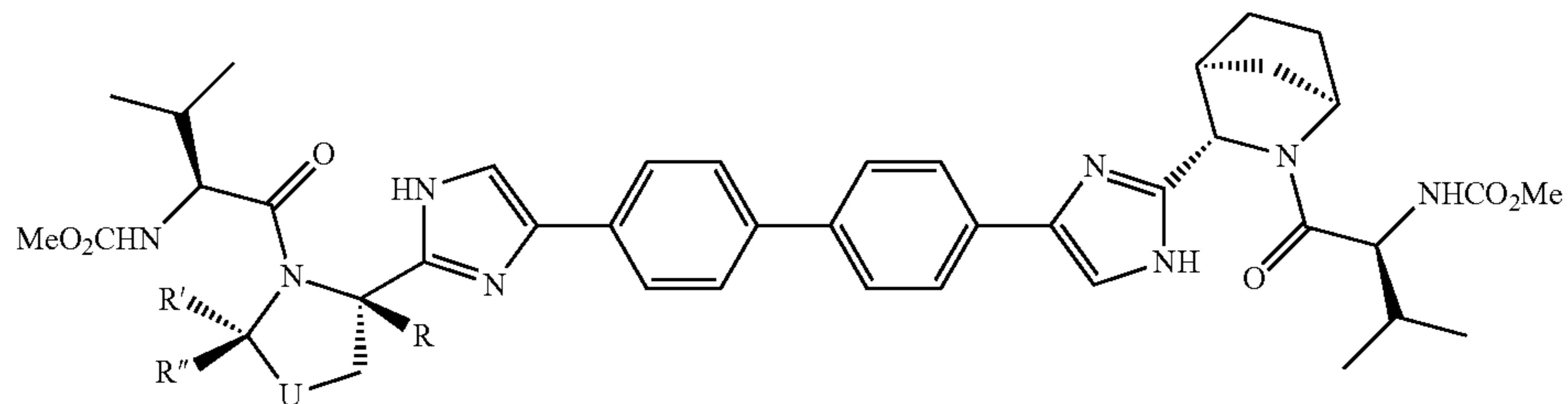
Compounds 220-229.
