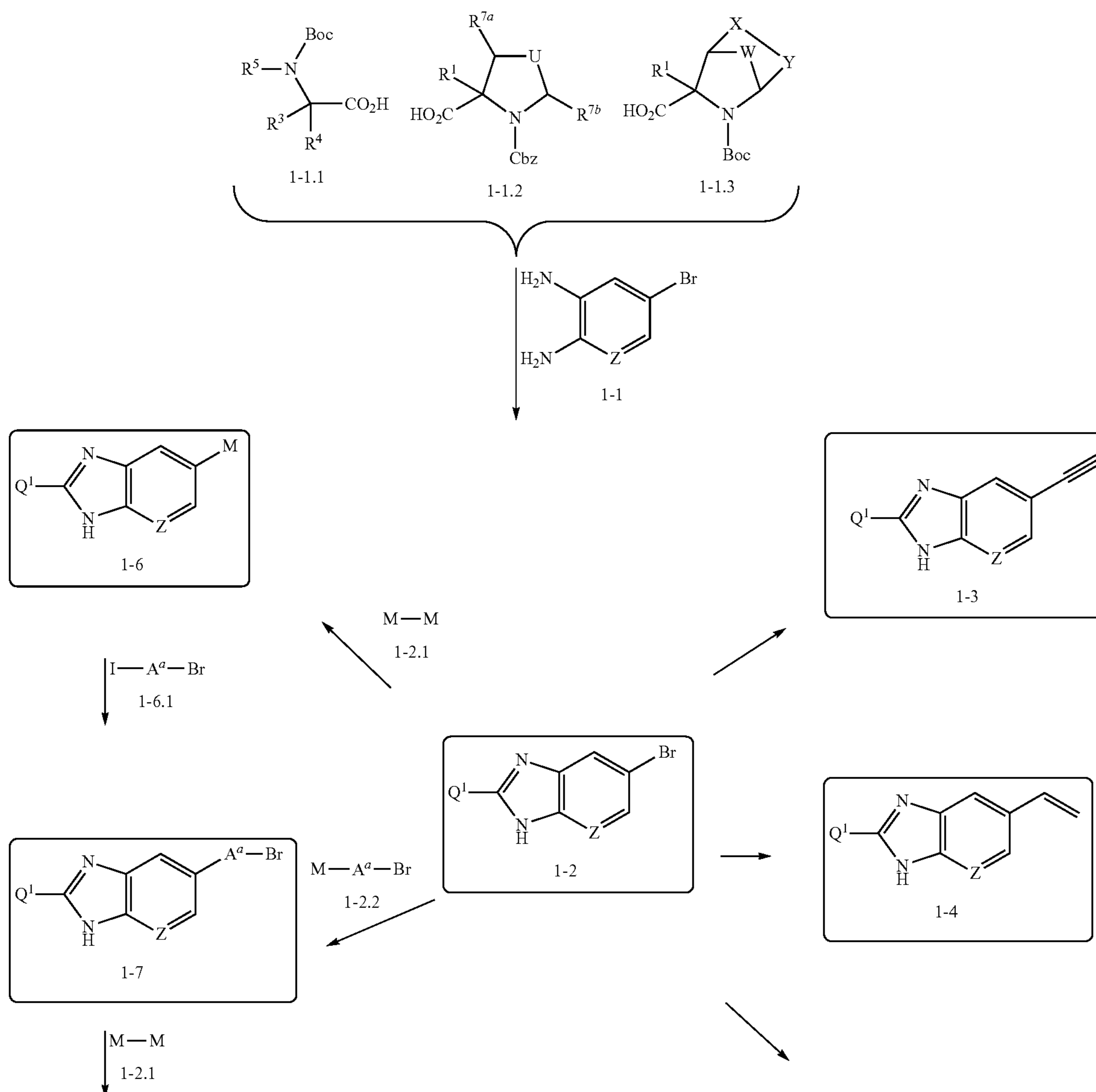
Scheme 1
