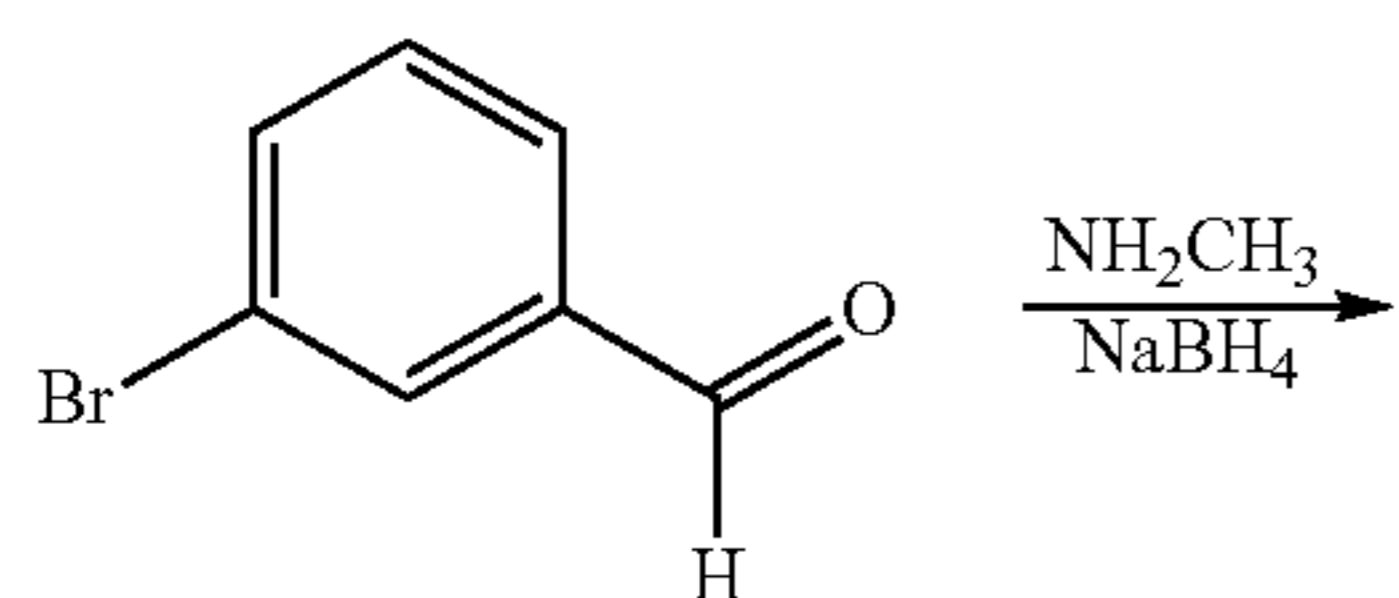
Synthesis Scheme 2
