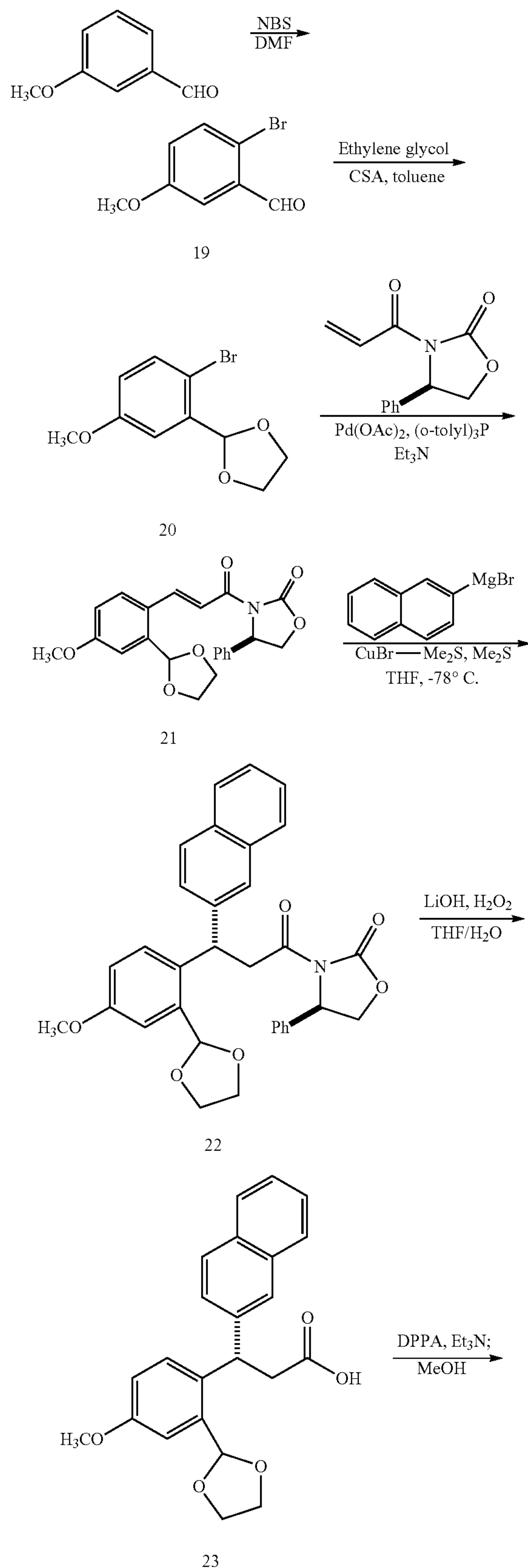
Synthesis Scheme 3
