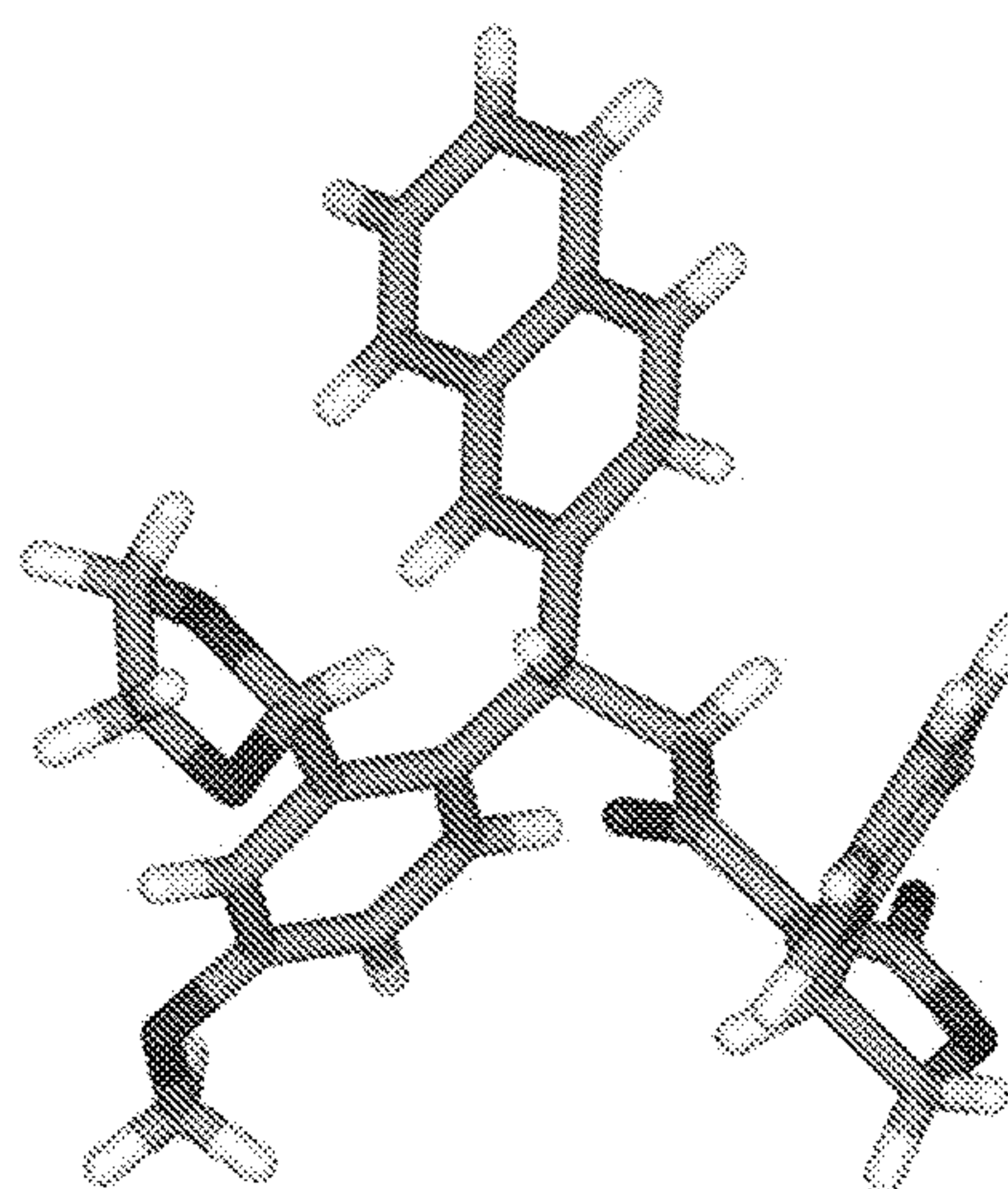
Single Crystal Structure of Compound 22
