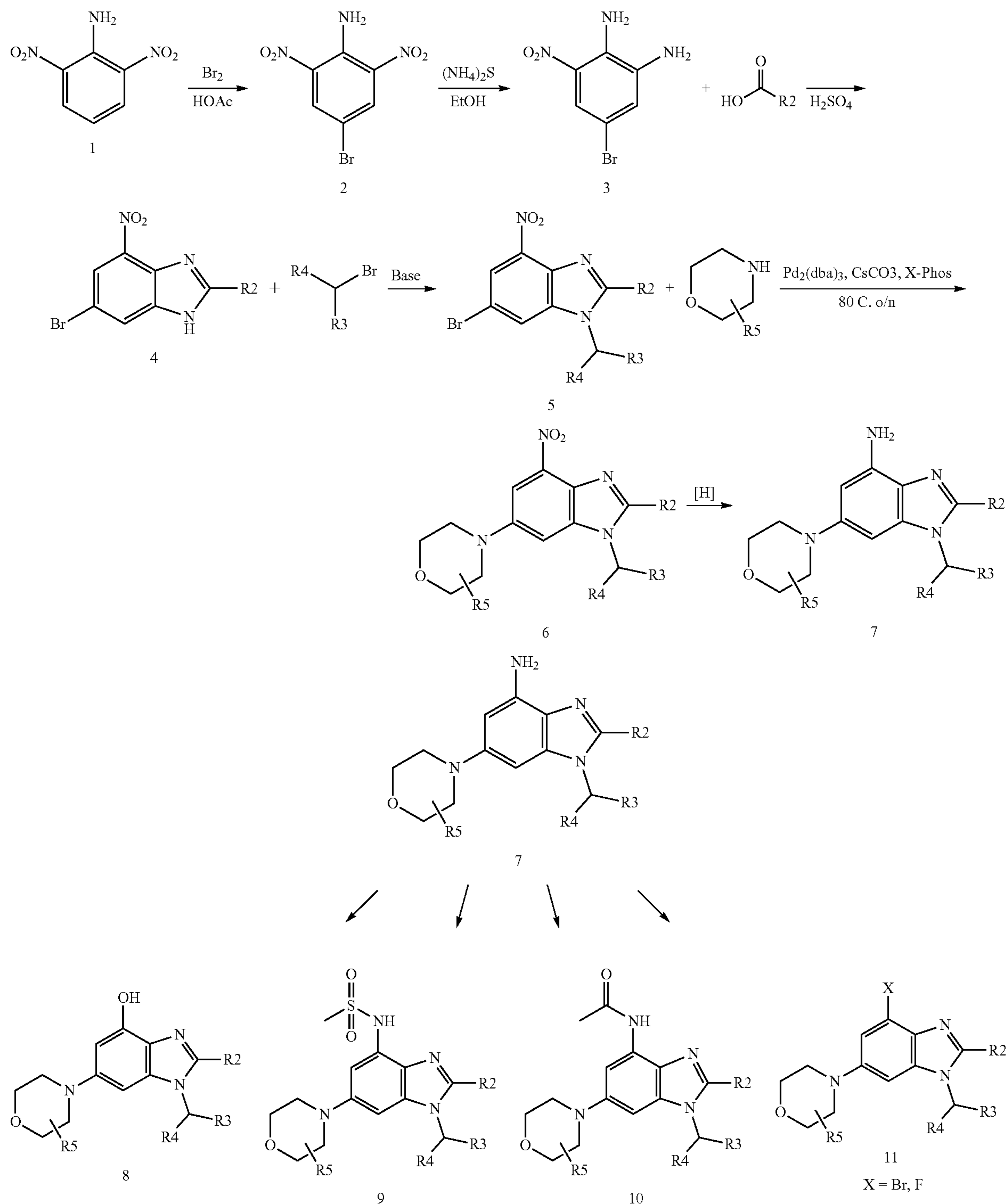
Scheme II
