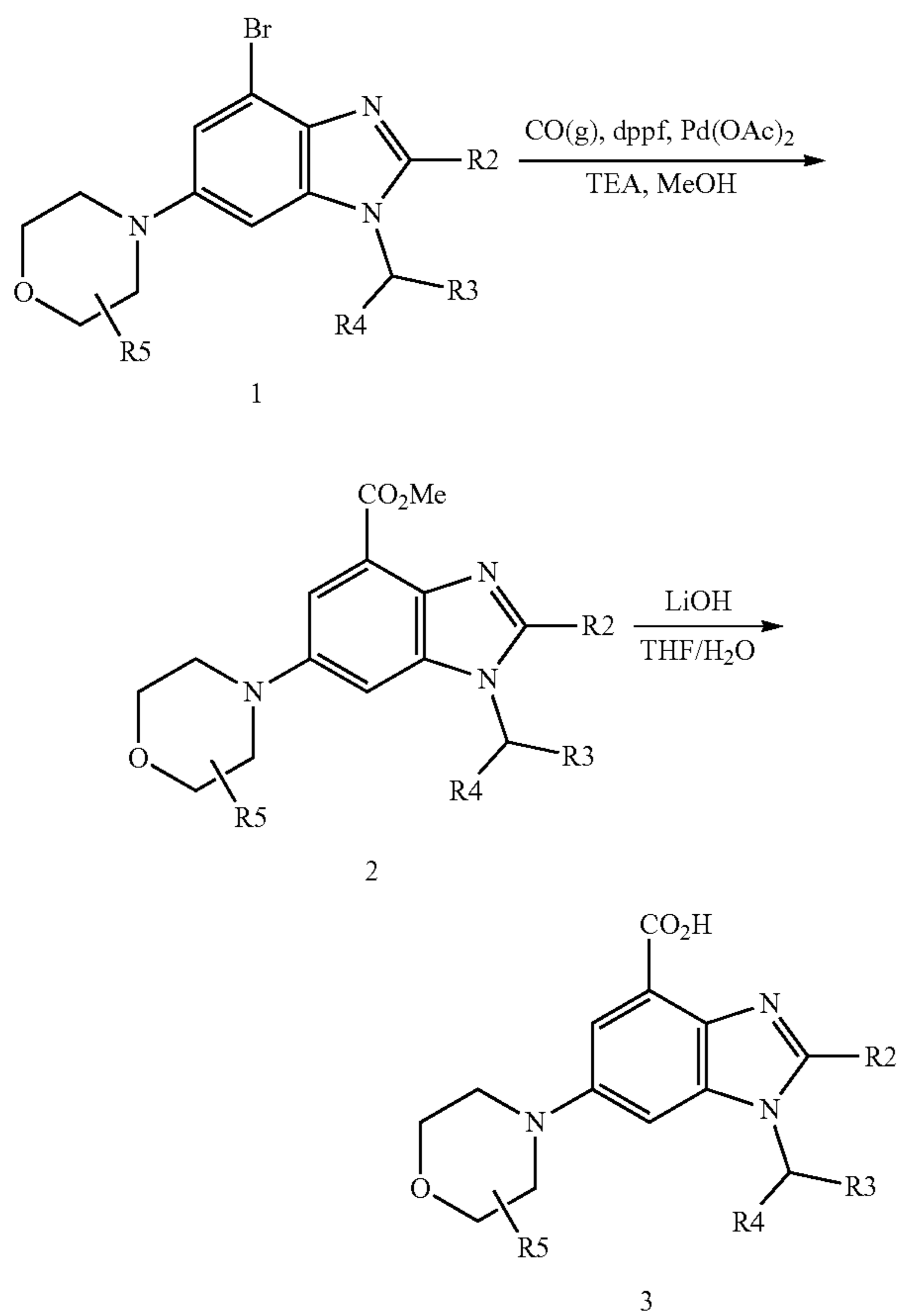
Scheme V
