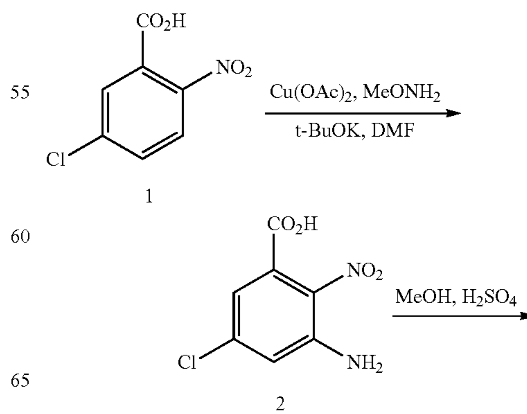
Scheme VII
