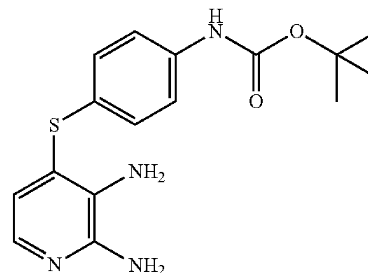
Tert-butyl 4-(2,3-diaminopyridin-4-ylthio)phenylcarbamate
