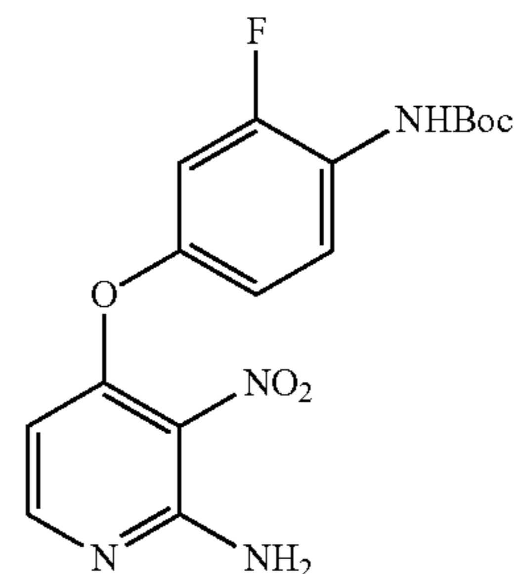
4-(4-N-tert-Butoxycarbonylamino-3-fluorophenoxy)-3-nitro-2-amino-pyridine
