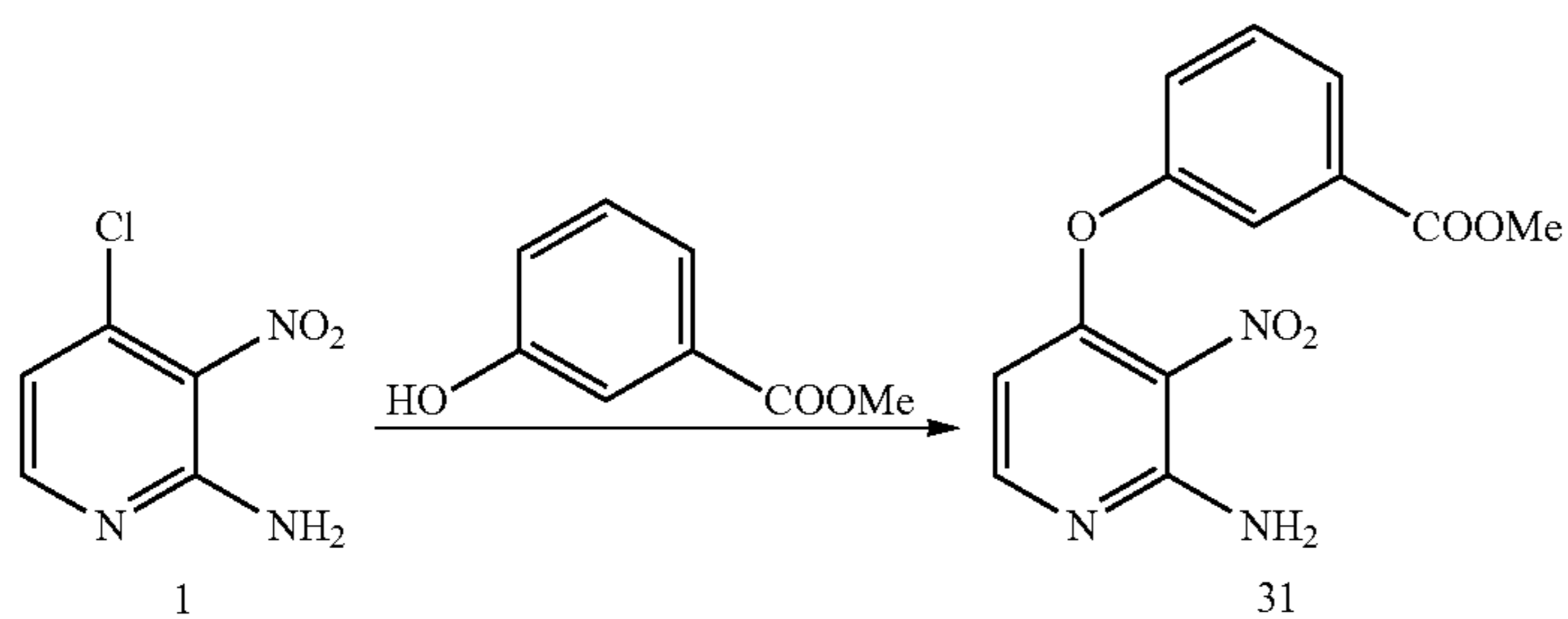
Scheme 10
