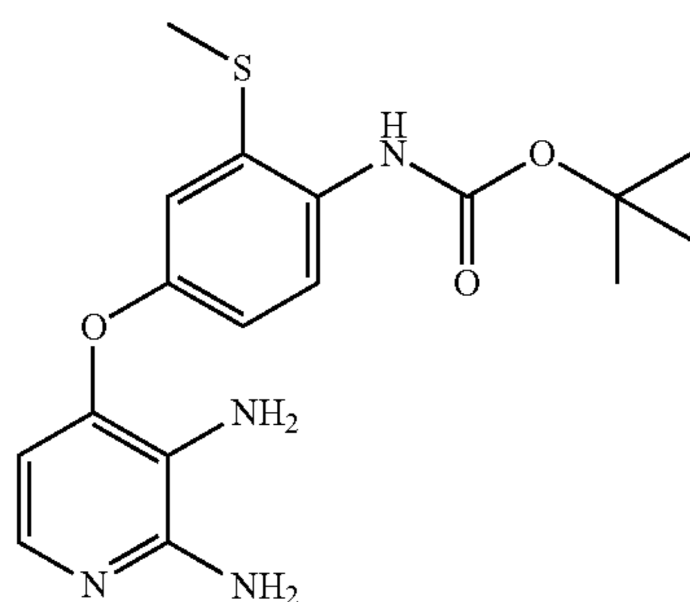
Tert-butyl 4-(2,3-diaminopyridin-4-yloxy)-2-(methylthio)phenylcarbamate
