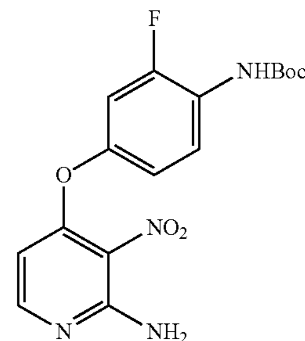
4-(4-N-tert-Butoxycarbonylamino-3-fluorophenoxy)-3-nitro-2-amino-pyridine
