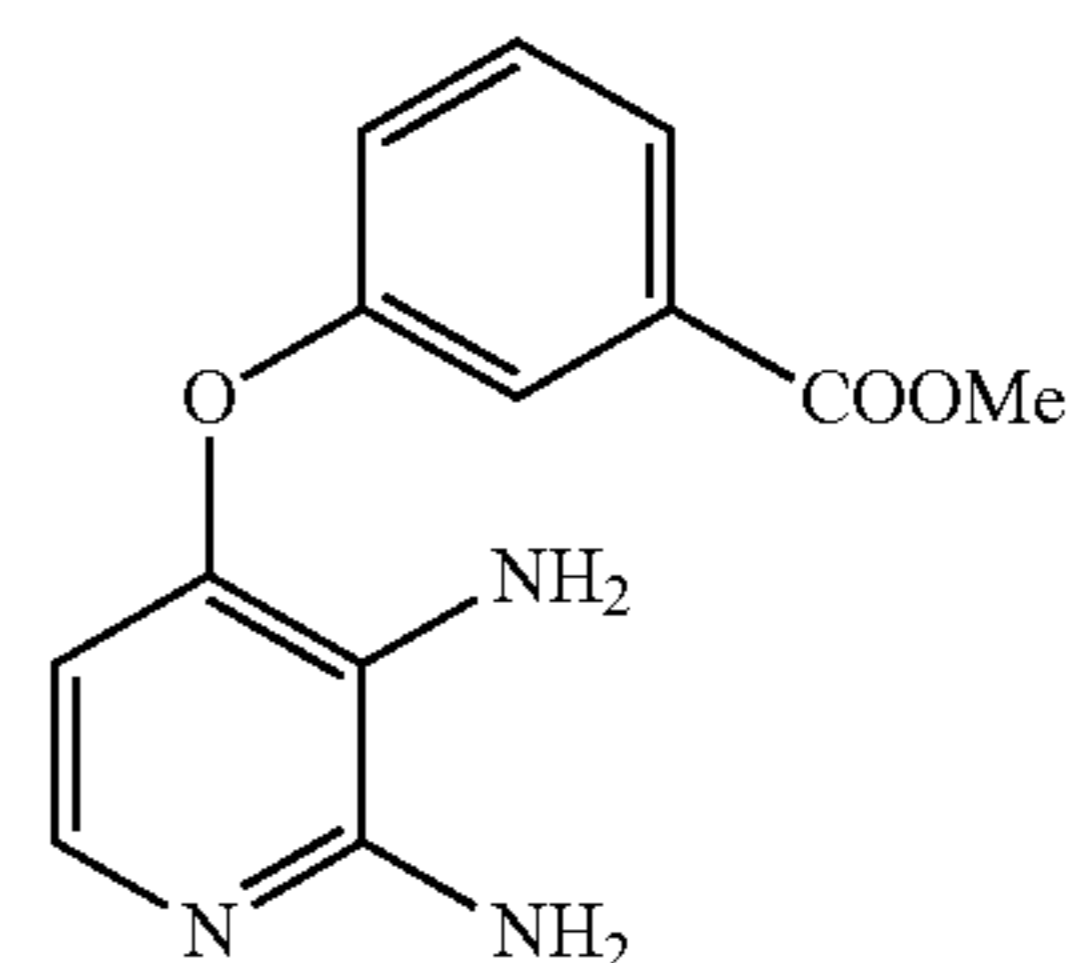
Methyl 3-(2,3-diaminopyridin-4-yloxy)benzoate
