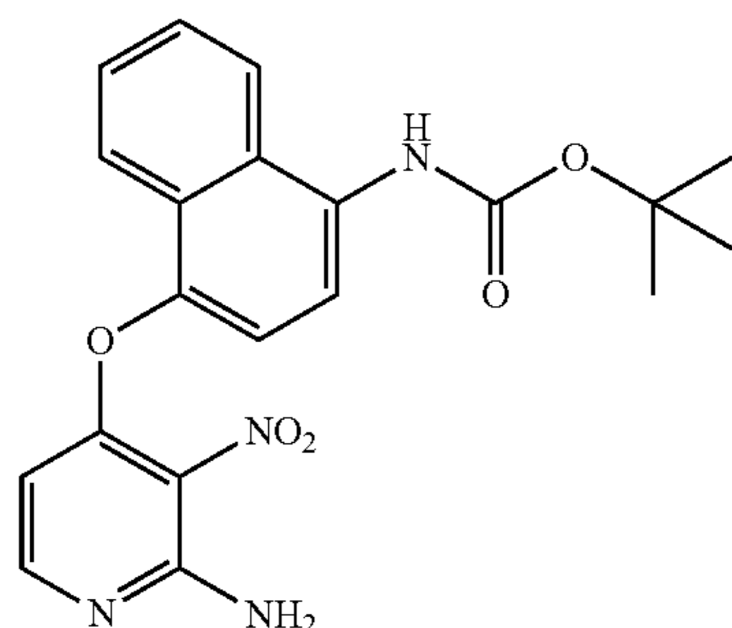
Tert-butyl 4-(2-amino-3-nitropyridin-4-yloxy)naphthalen-1-ylcarbamate
