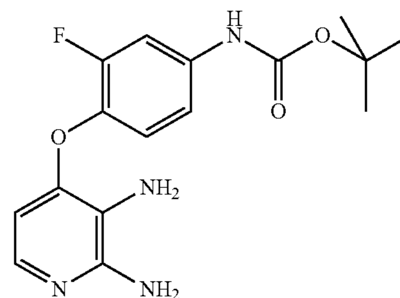
tert-butyl 4-(2,3-diaminopyridin-4-yloxy)-3-fluorophenylcarbamate
