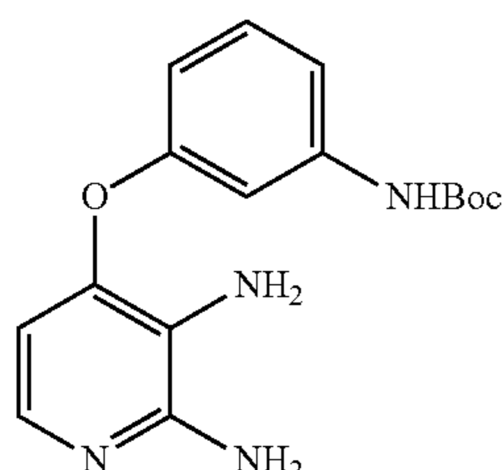
4-(3-N-(tert-Butoxycarbonyl)aminophenoxy)-2,3-diamino-pyridine
