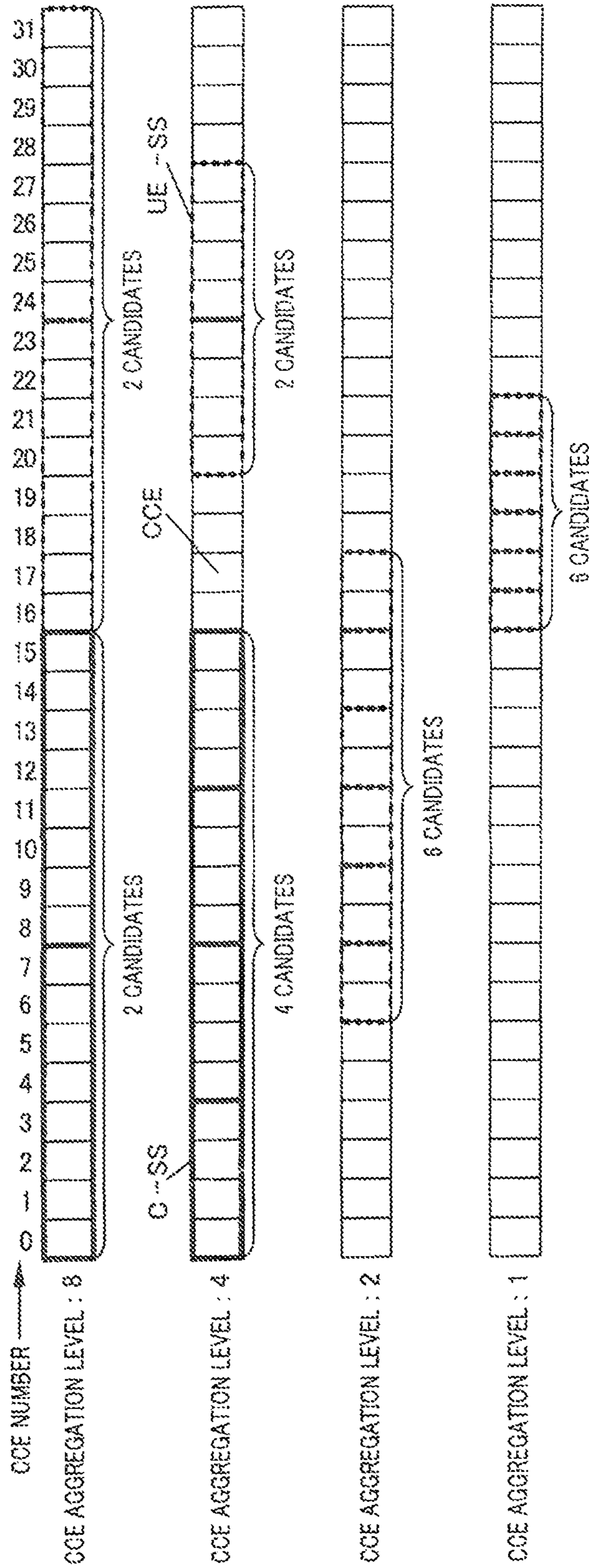
FIG. 2 PRIOR ART
