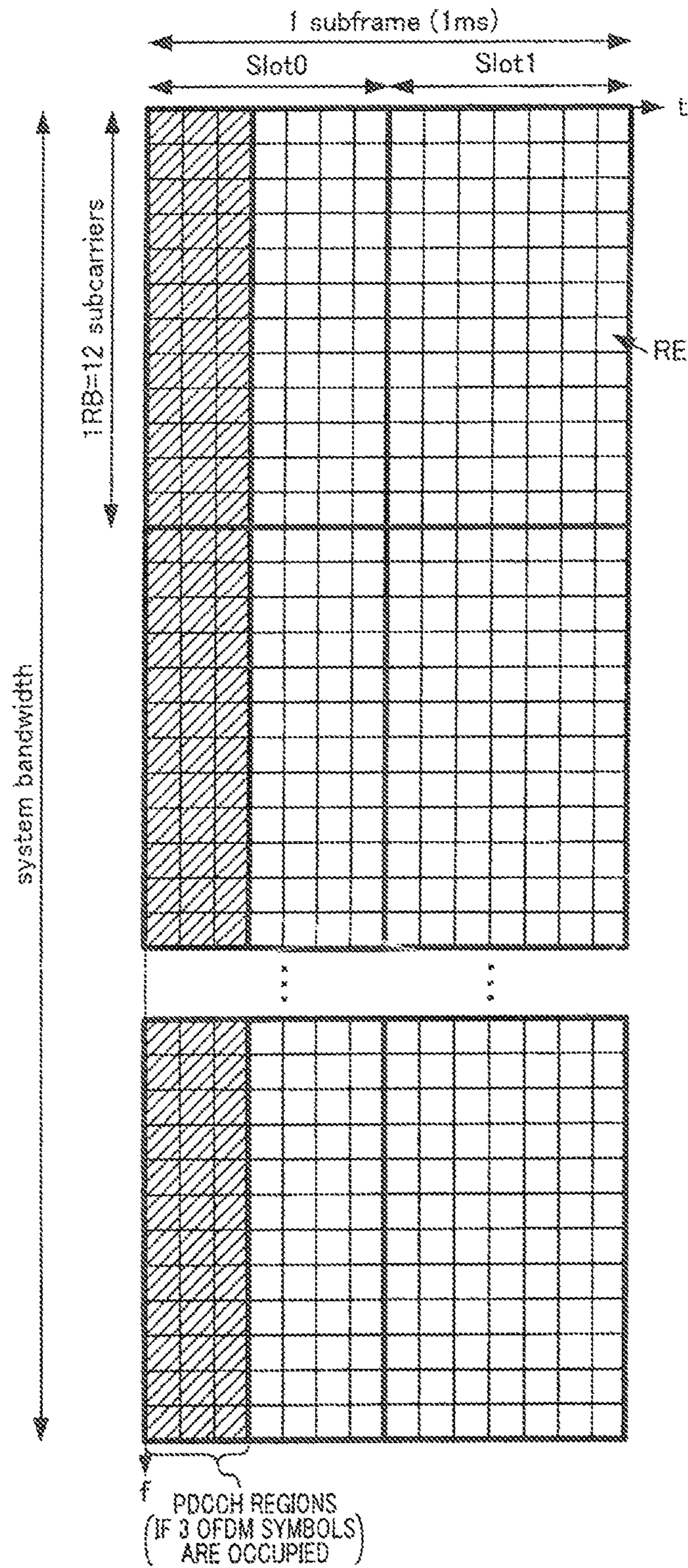
FIG. 1 PRIOR ART
