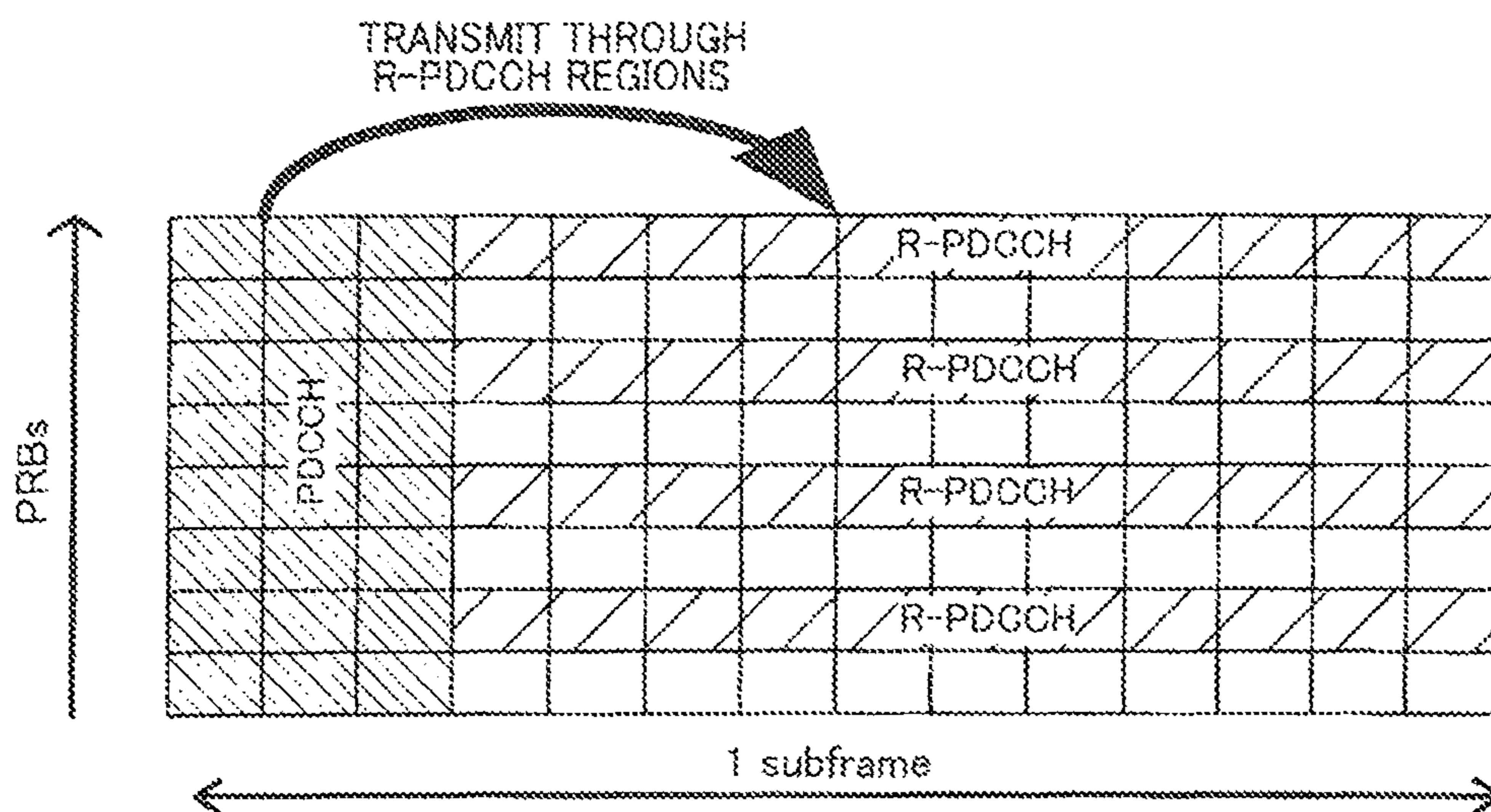
FIG. 6 PRIOR ART
