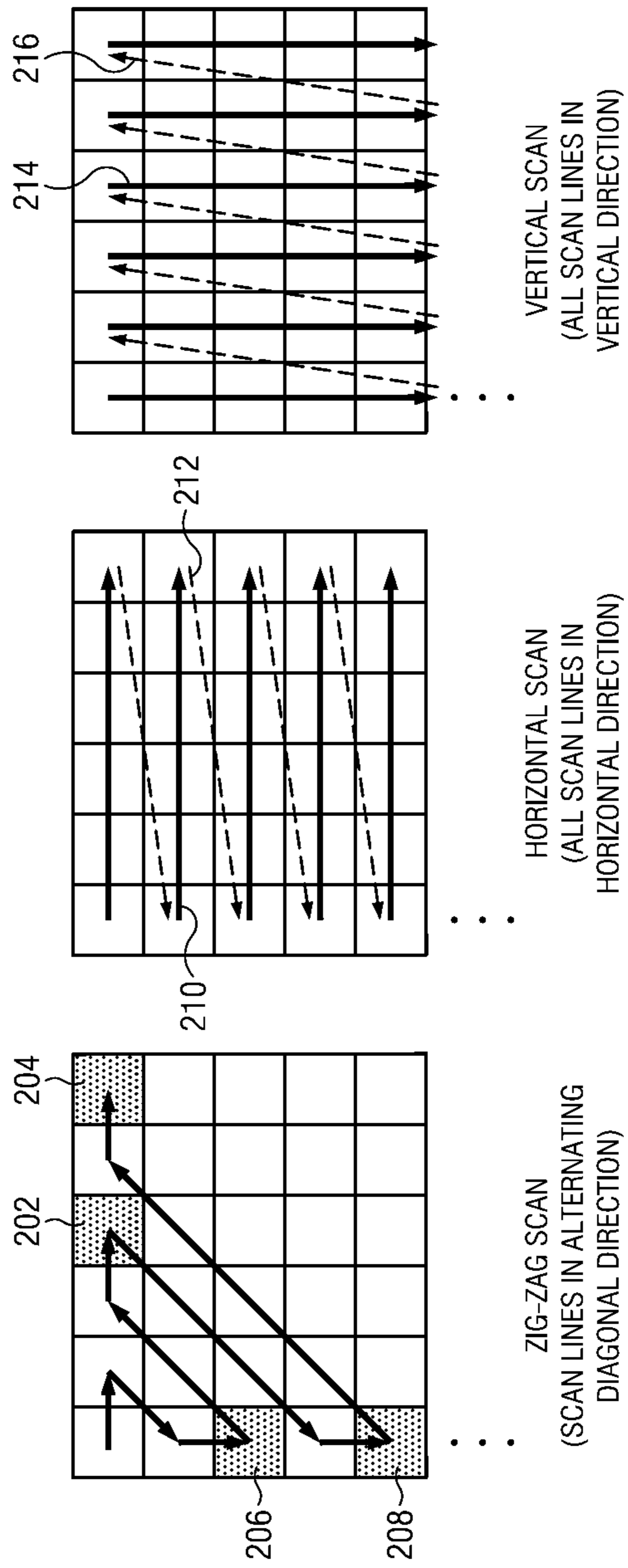
FIG. 2 (PRIOR ART)
