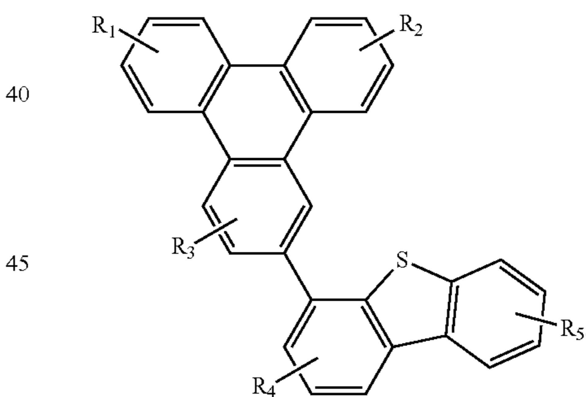
Compound 7'
