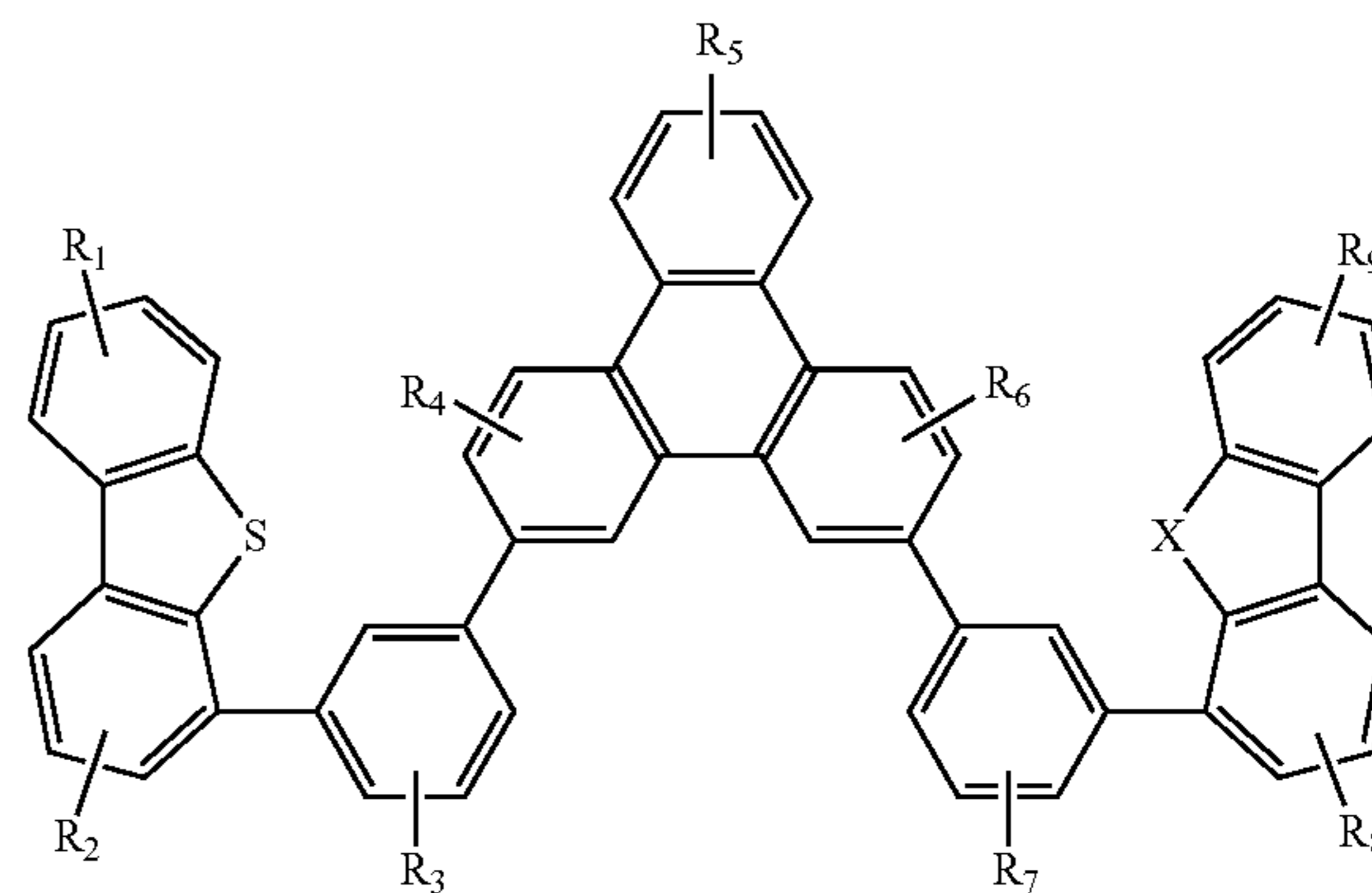
Compound 4G
