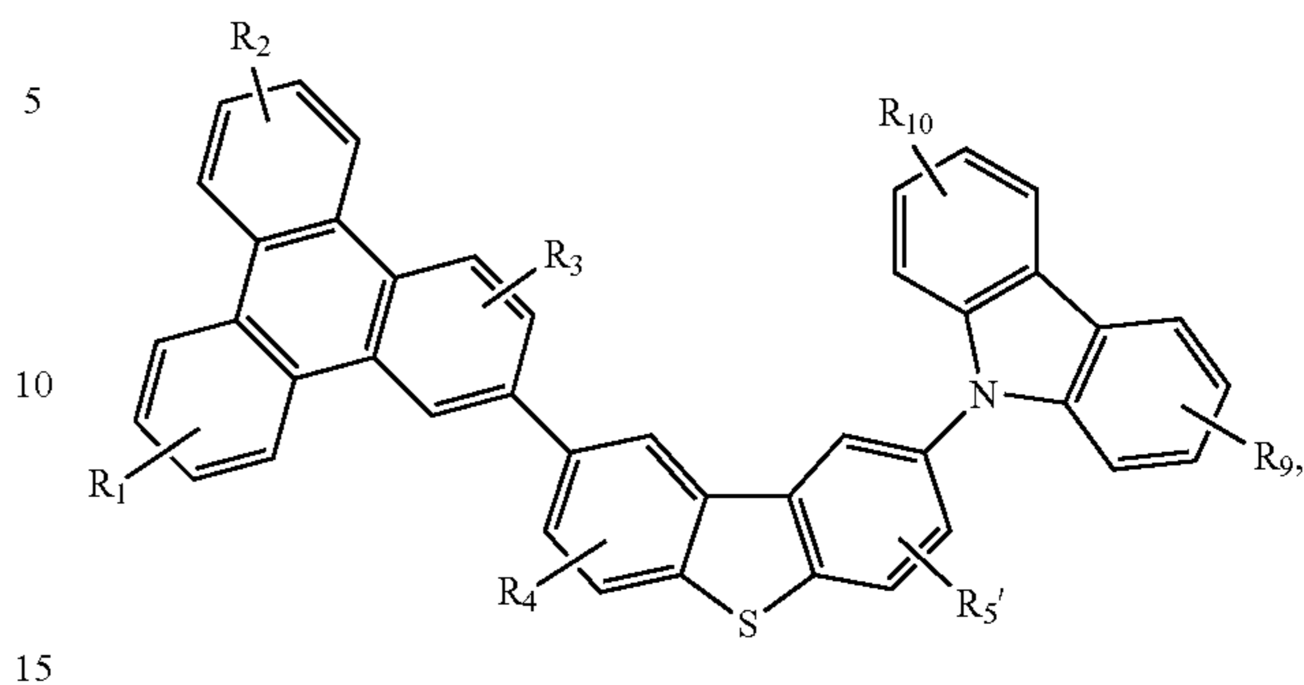
Compound 15'G
