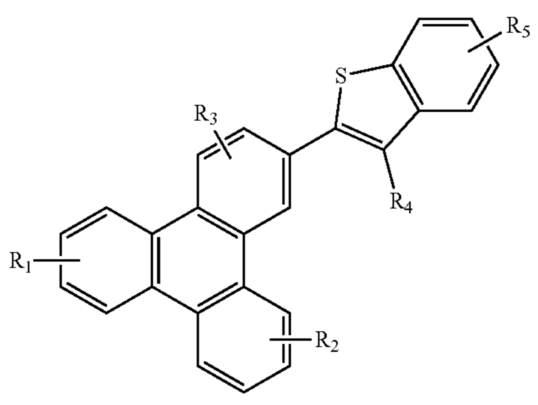
Compound 14'G
