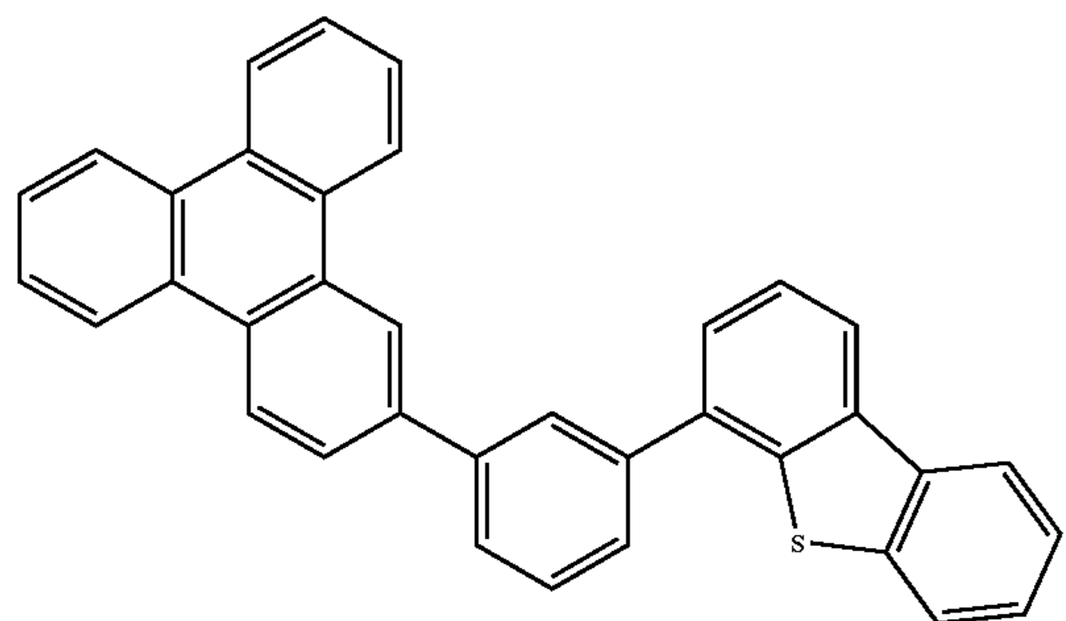
Compound 2S
