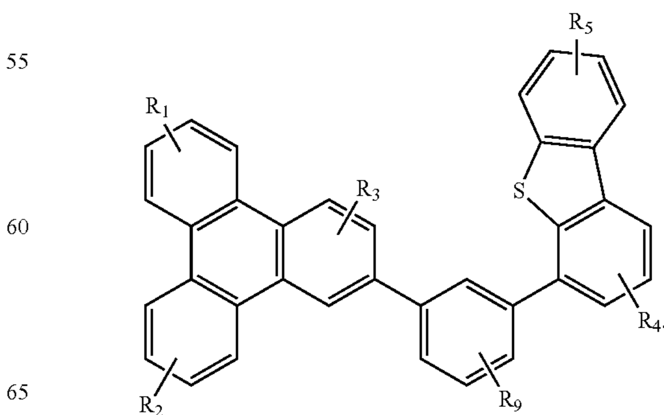
Compound 2'G
