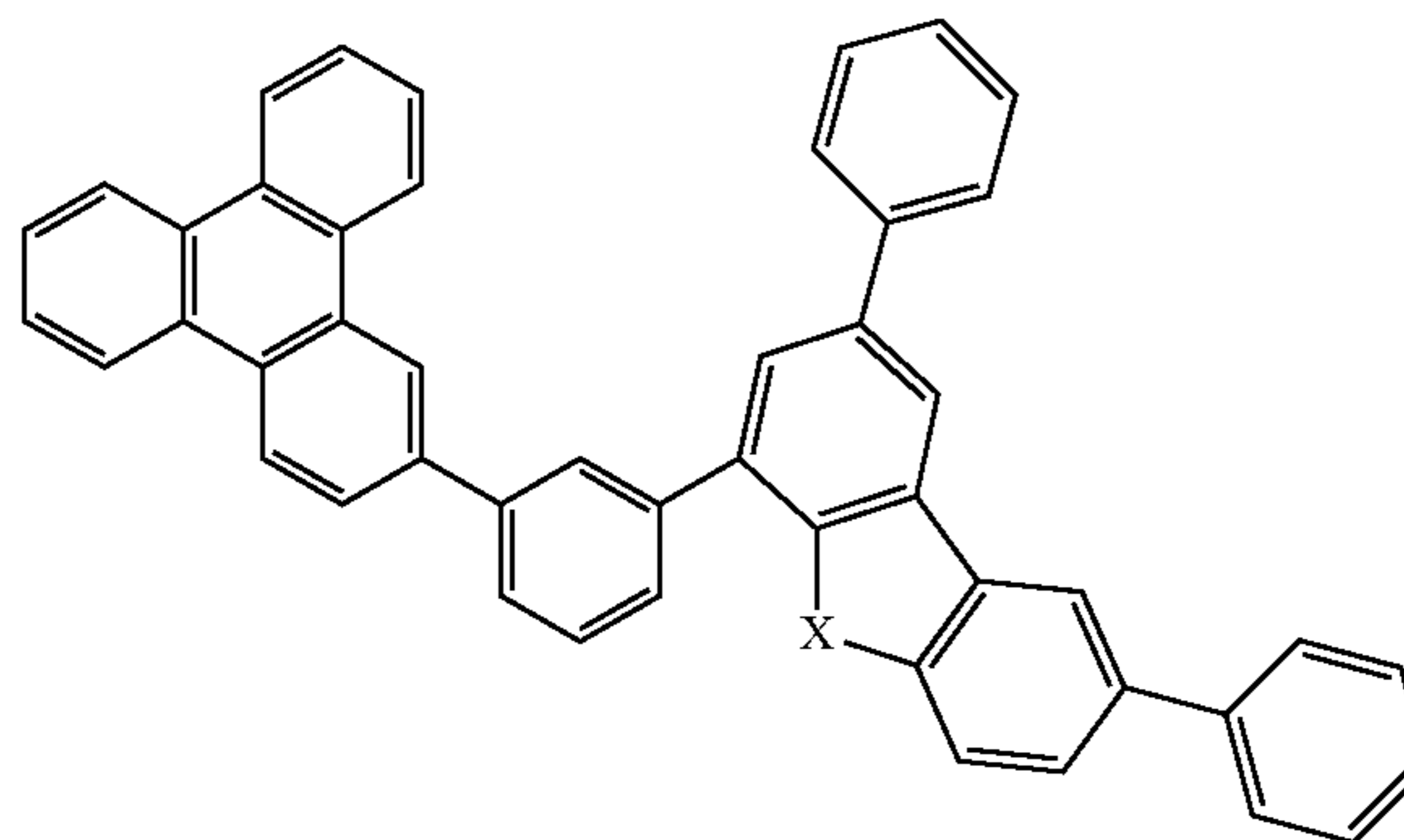
Compound 24
