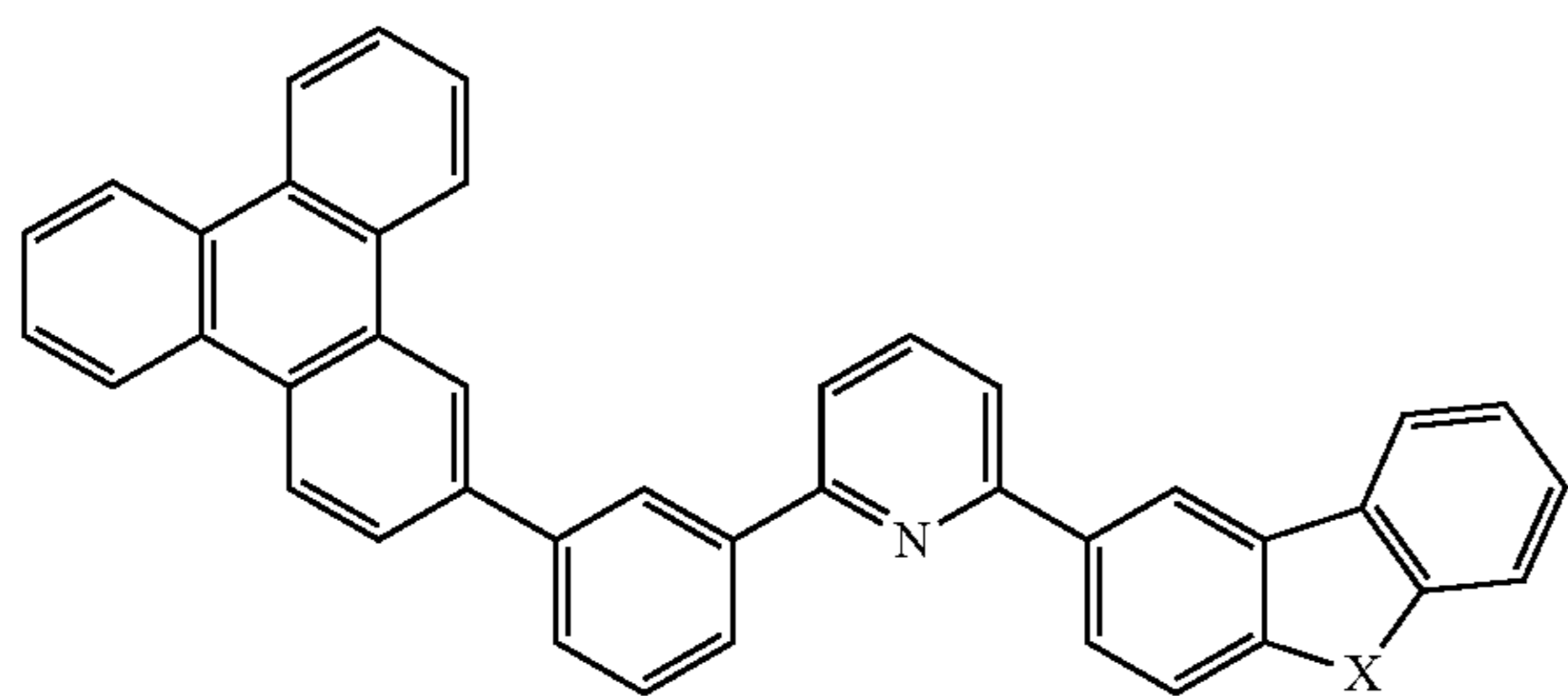
Compound 44
