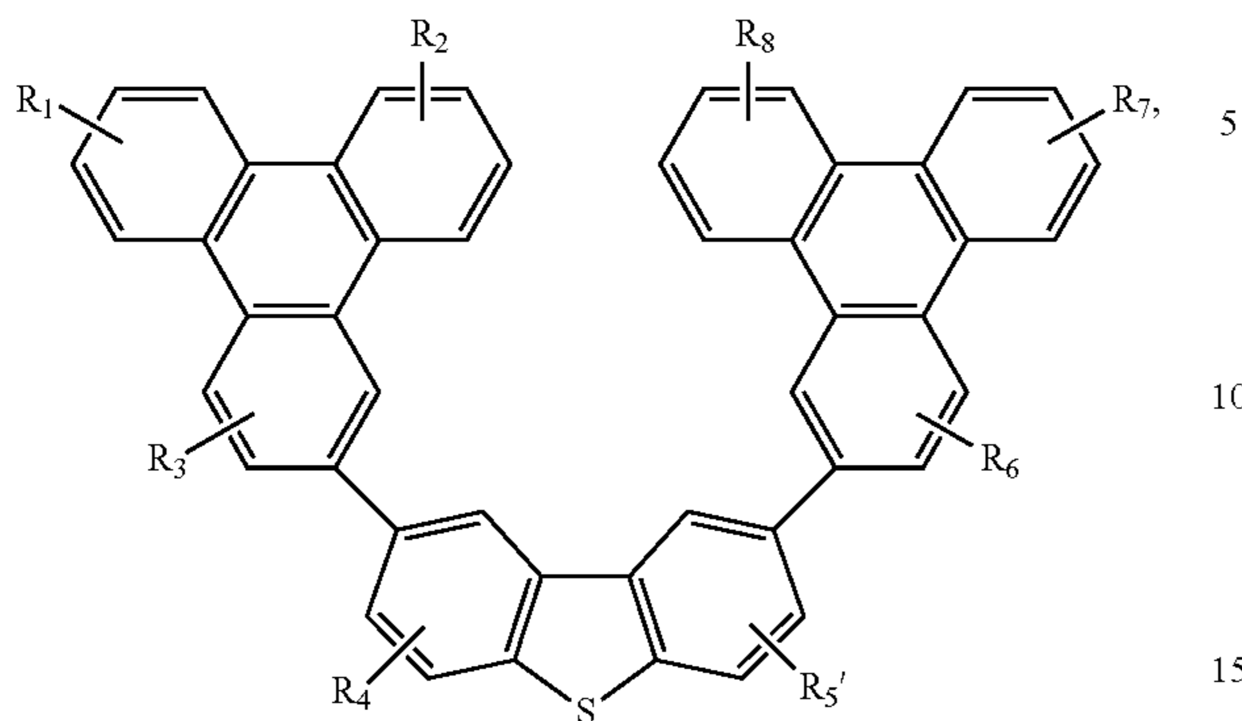
Compound 6'G
