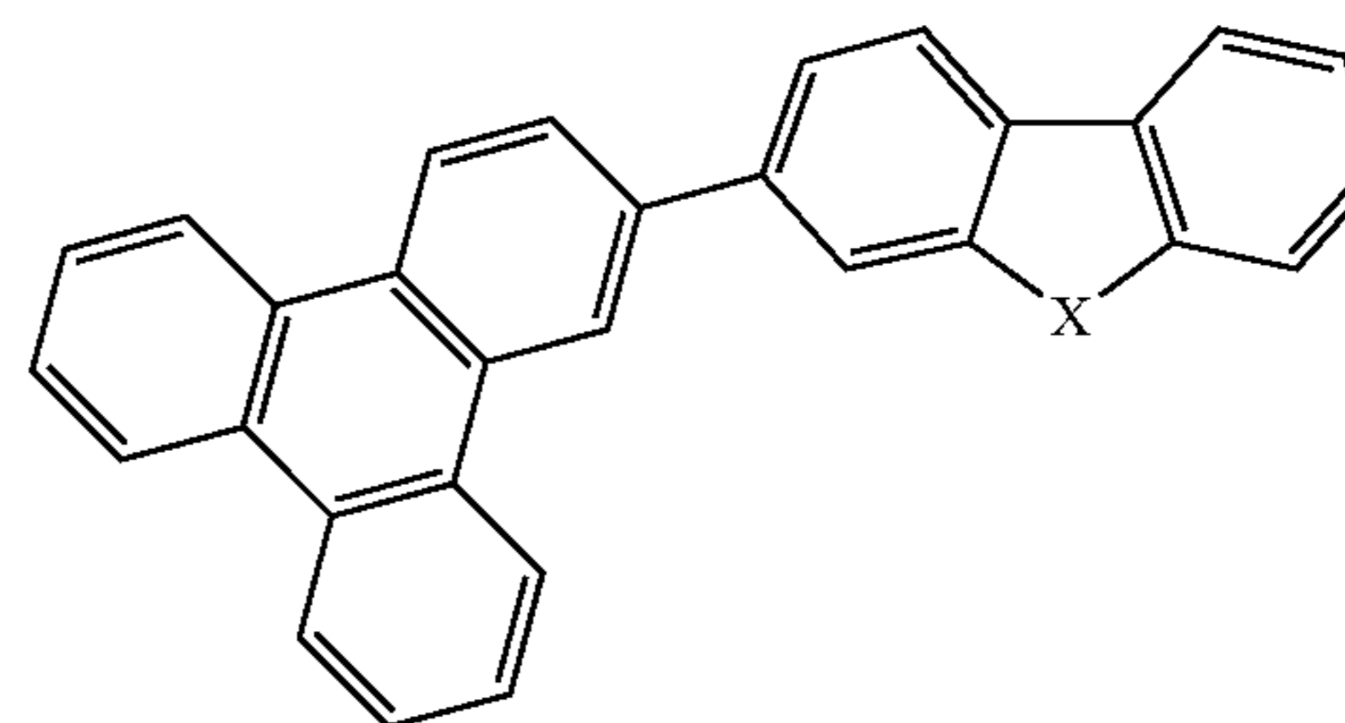
Compound 8
