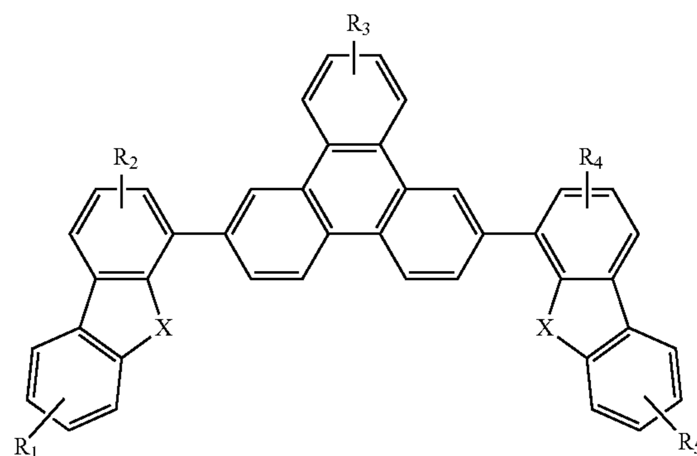
Compound 19 G
