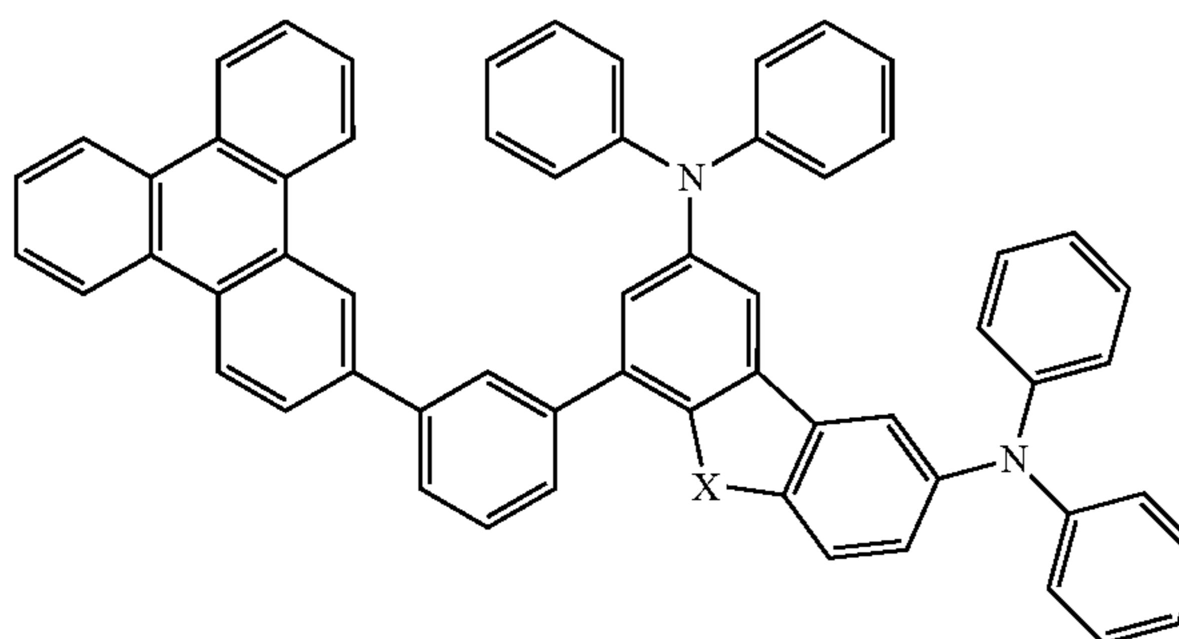
Compound 28
