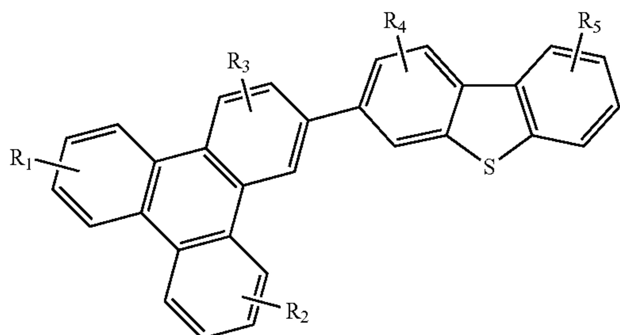
Compound 8'G
