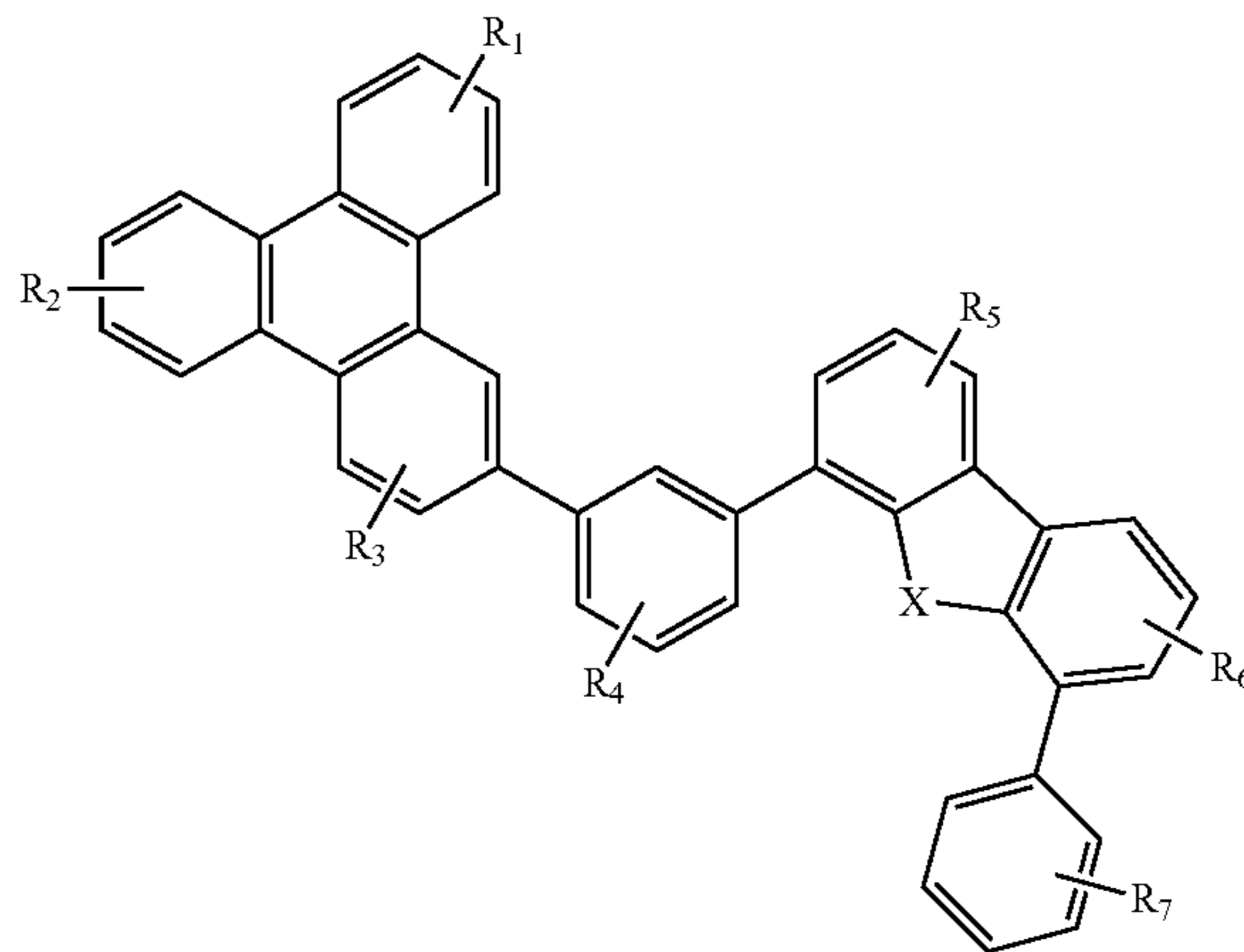
Compound 23 G
