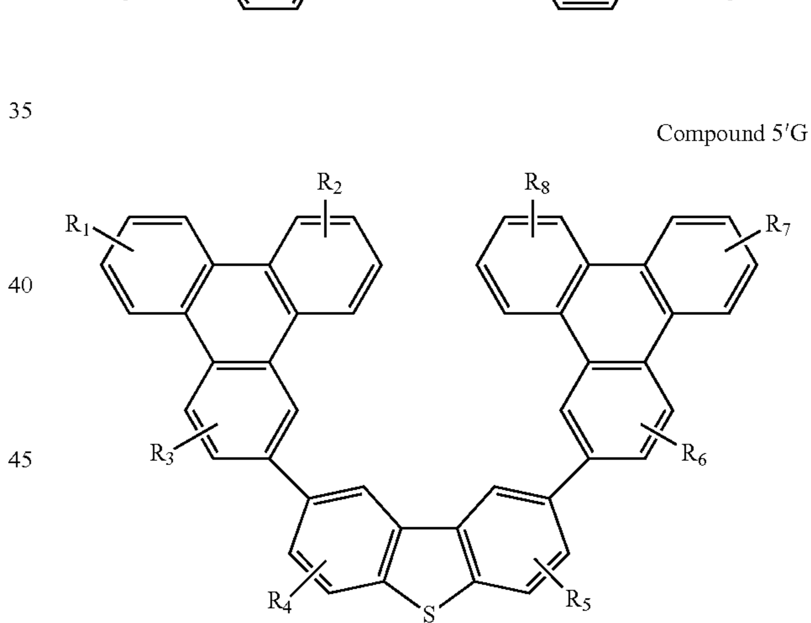
Compound 3'G
