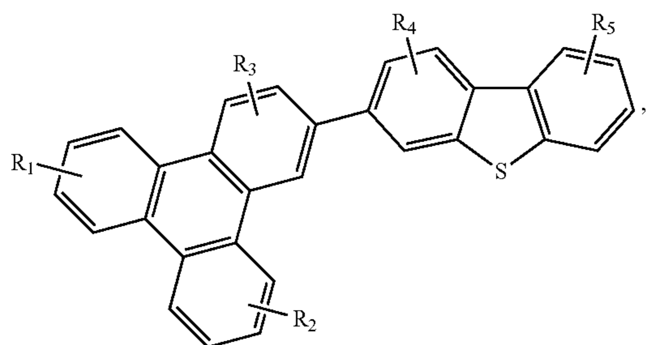
Compound 9'G
