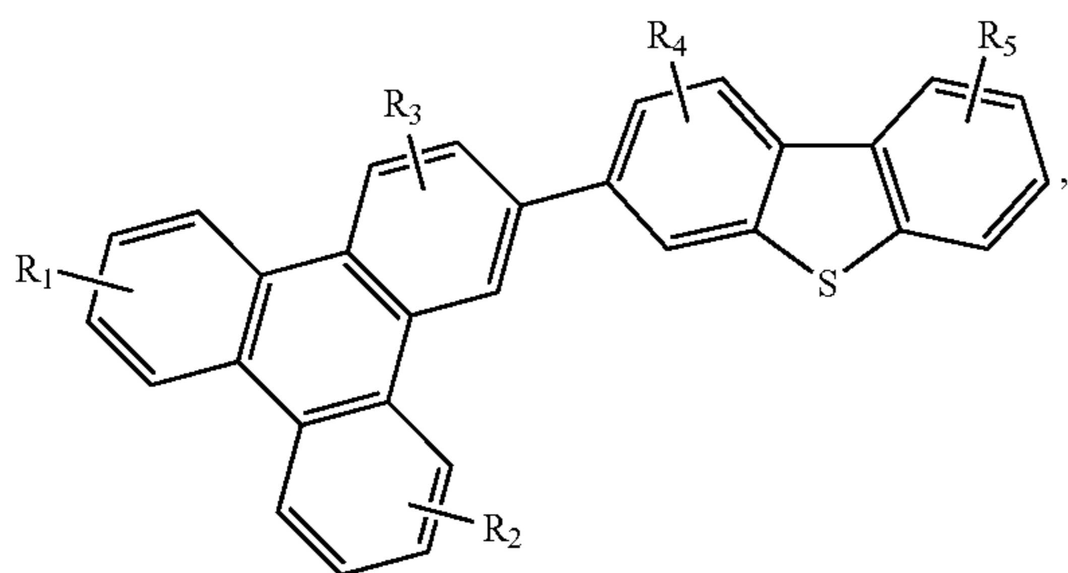
Compound 9'G
