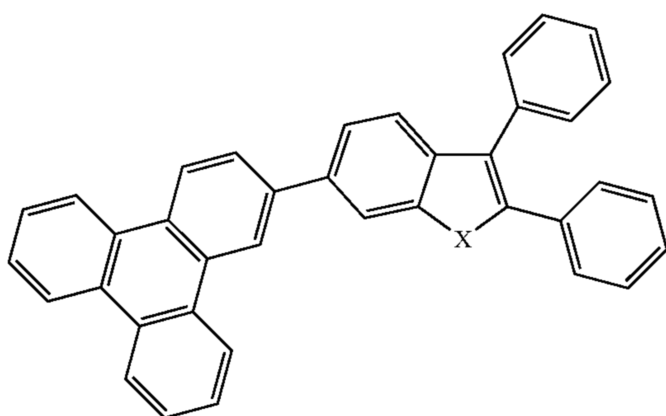
Compound 17
