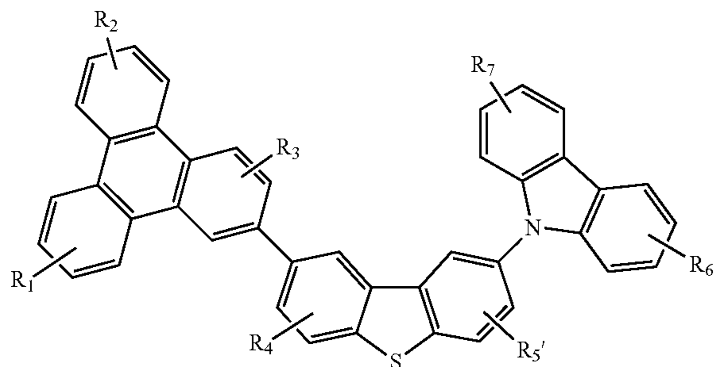
Compound 15'G
