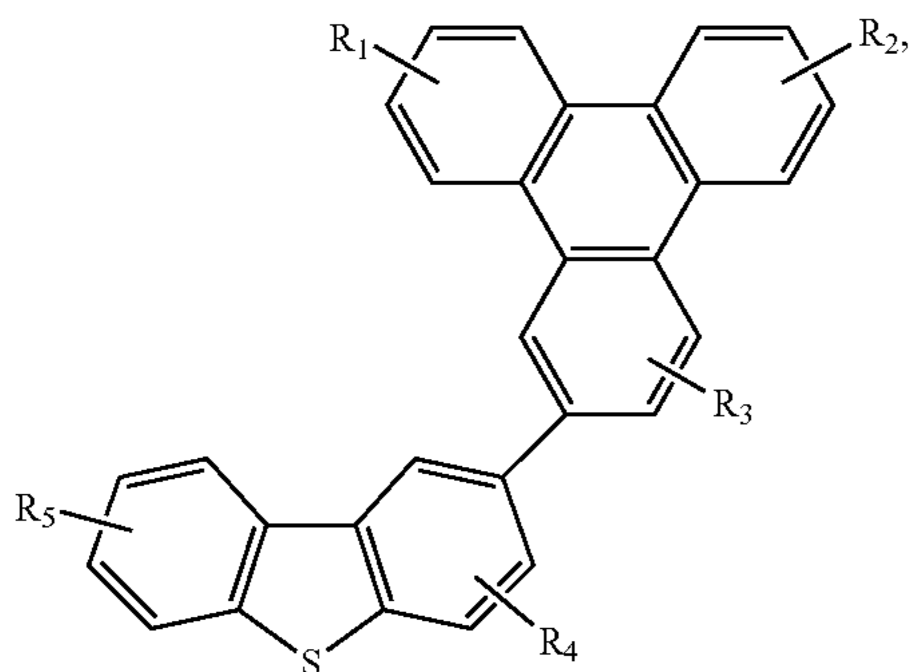
Compound 6'G
