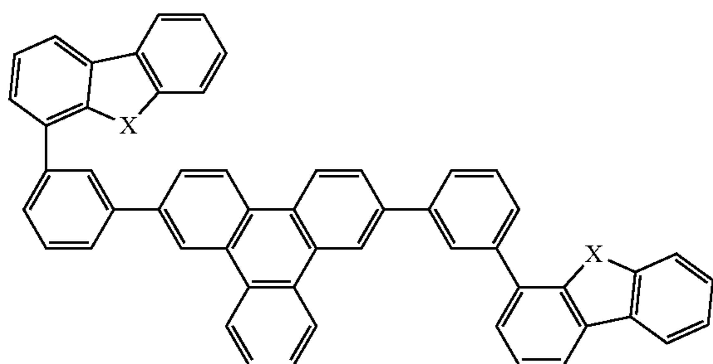
Compound 26
