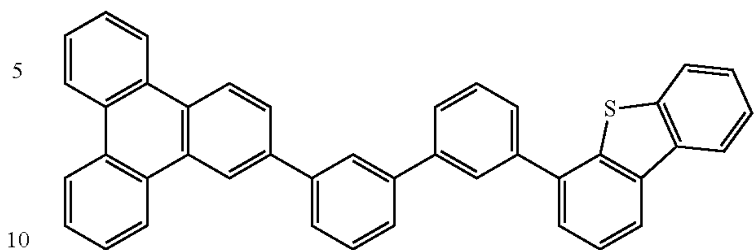
Compound 10'
