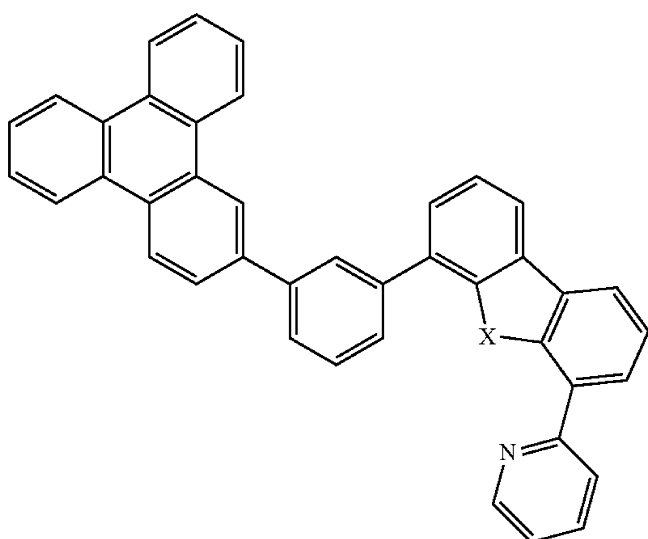
Compound 47
