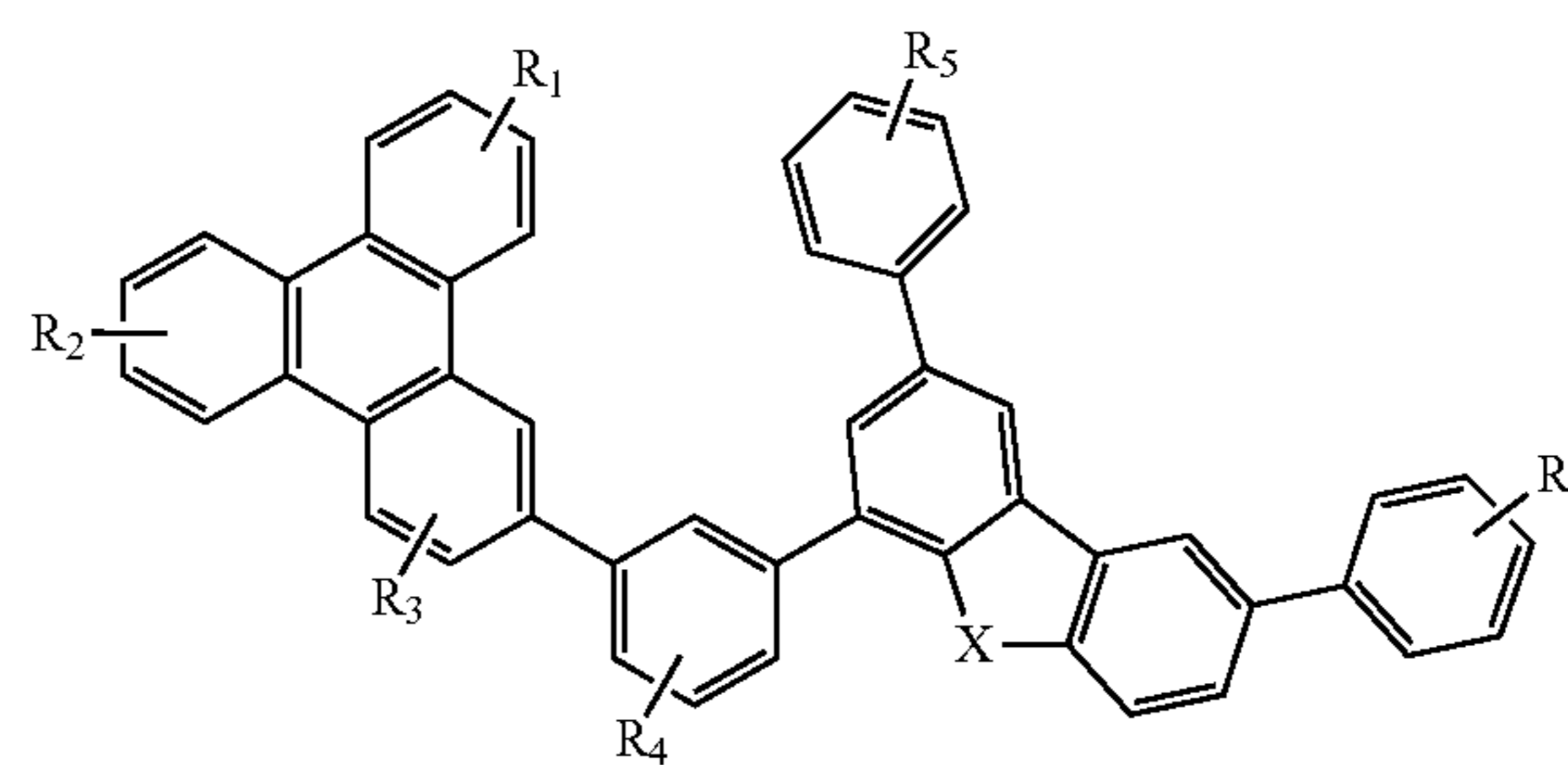
Compound 24
