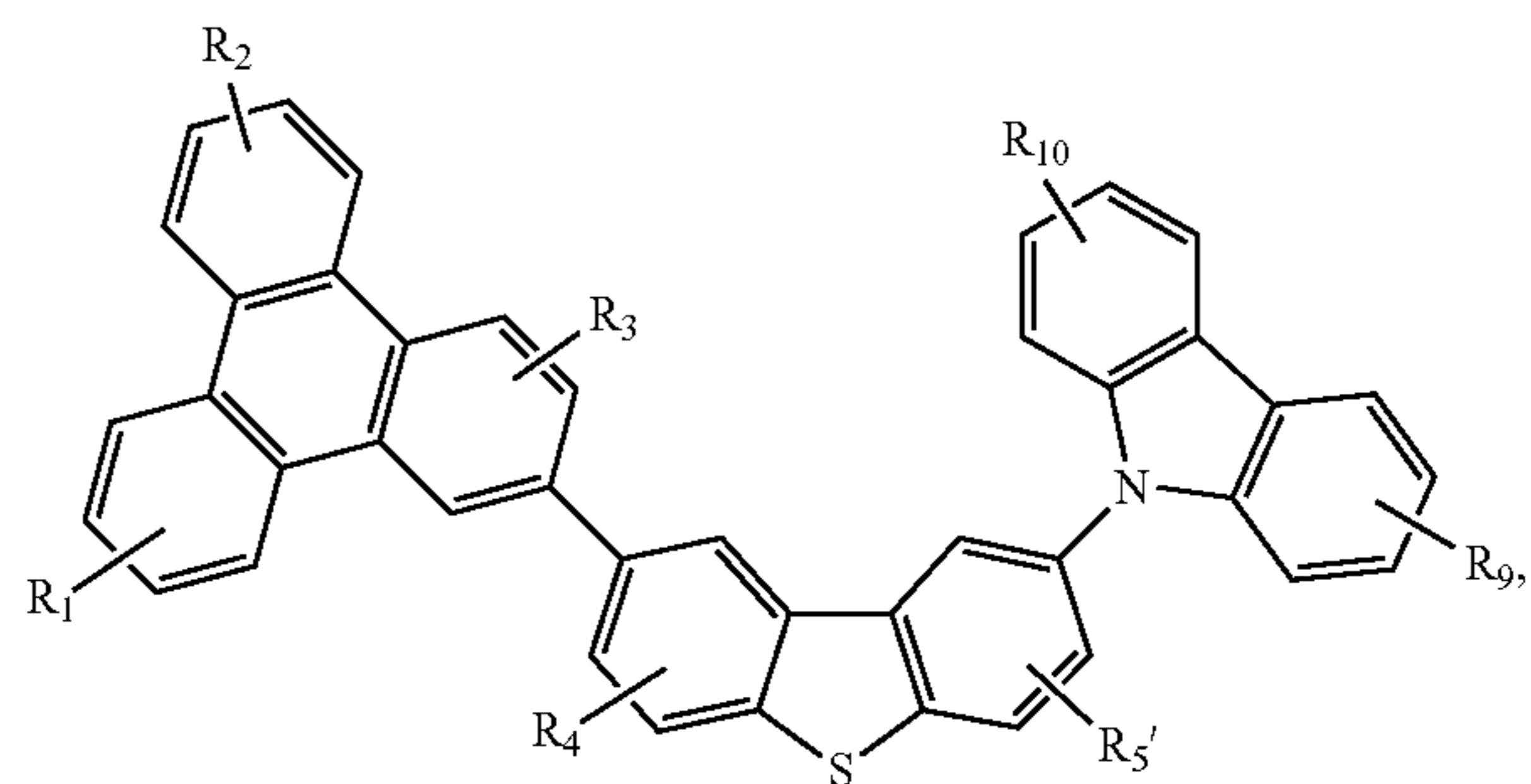
Compound 15'G
