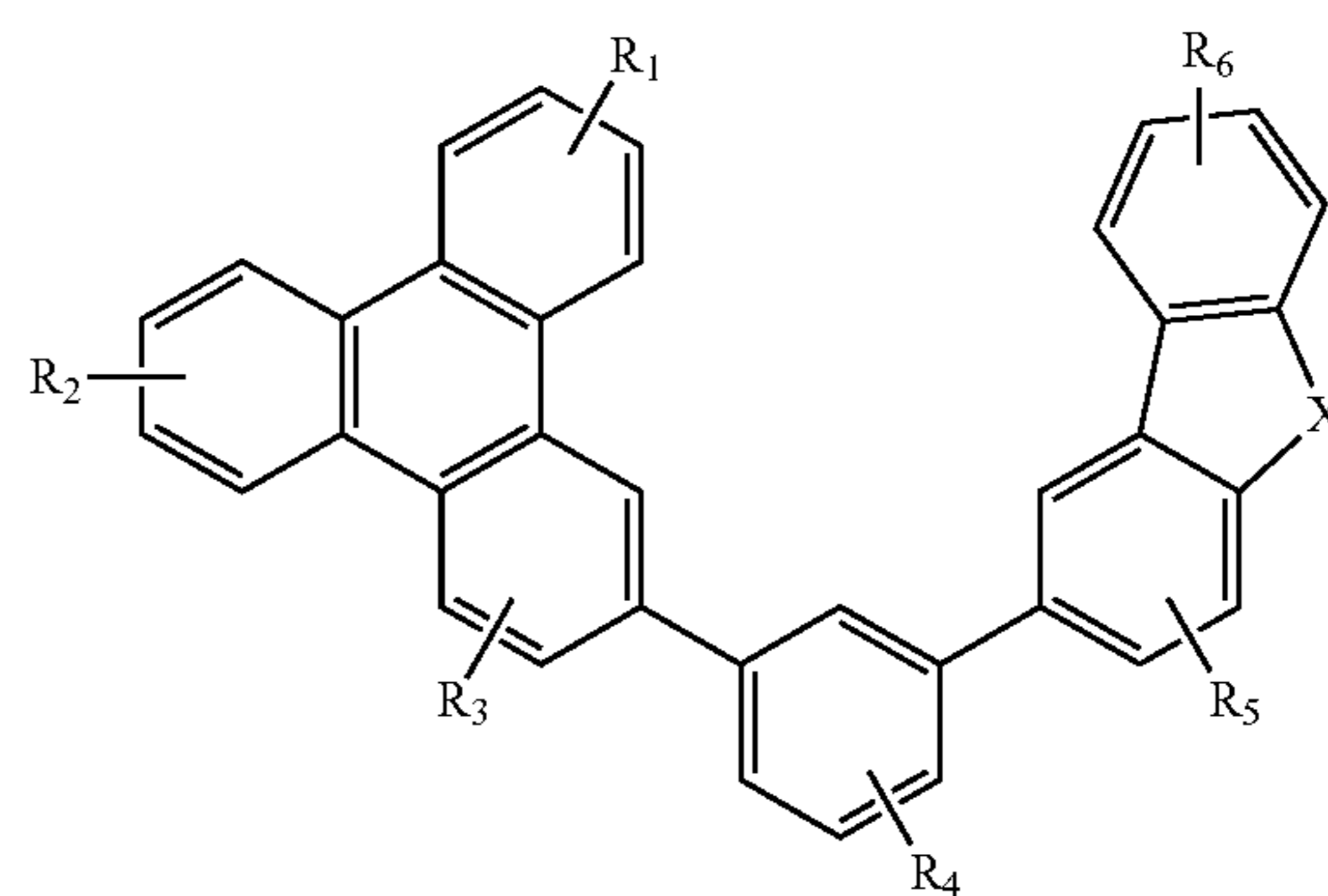
Compound 20 G
