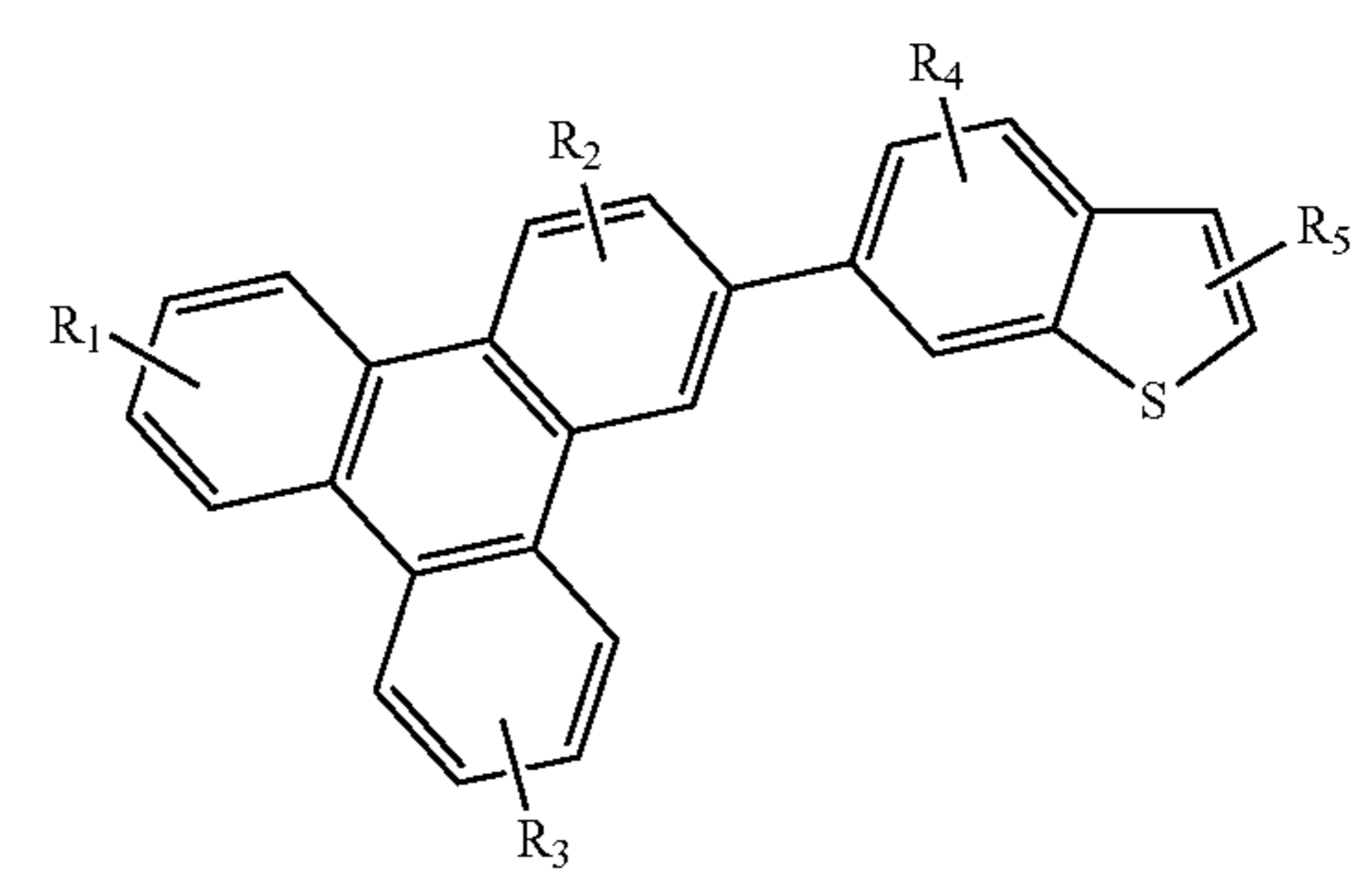
Compound 17'G
