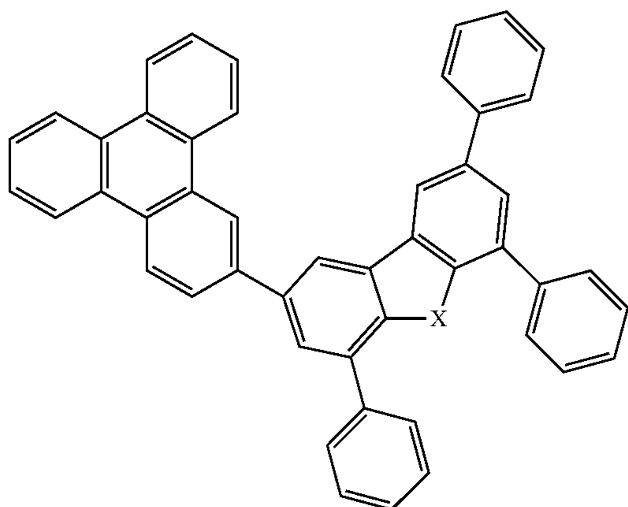
Compound 35
