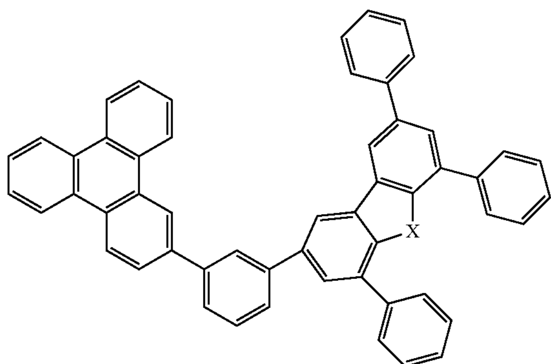
Compound 36
