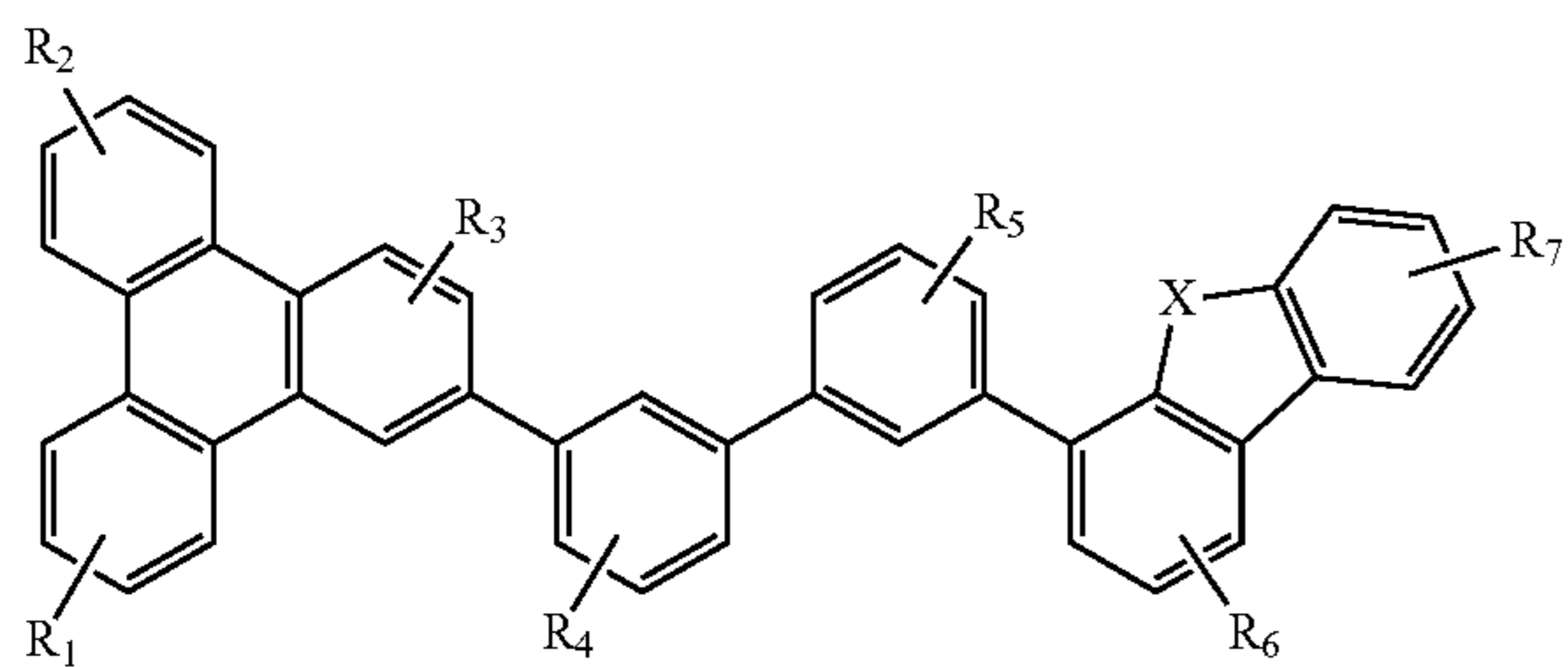
Compound 9G
