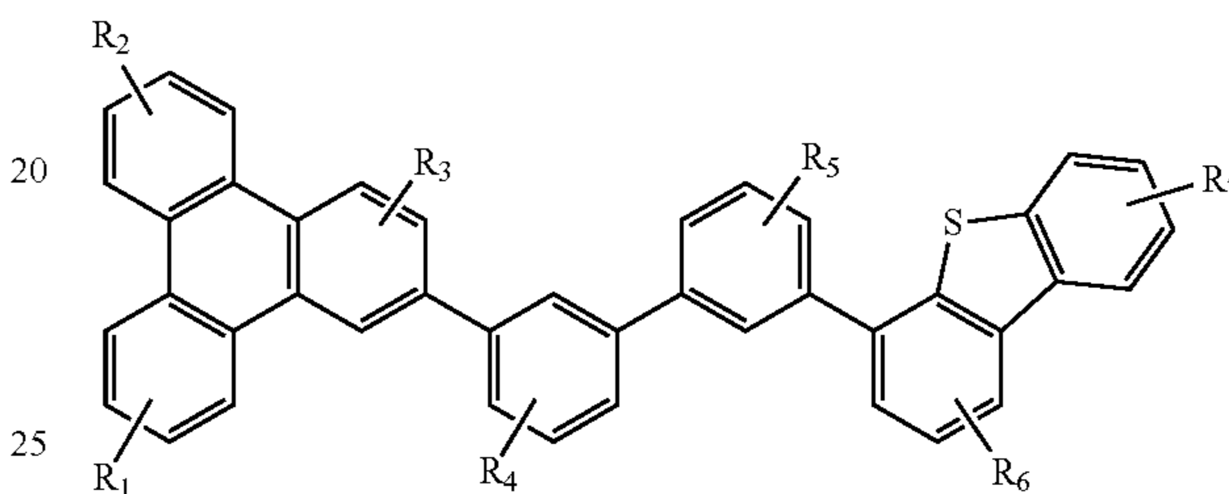
Compound 9'G
