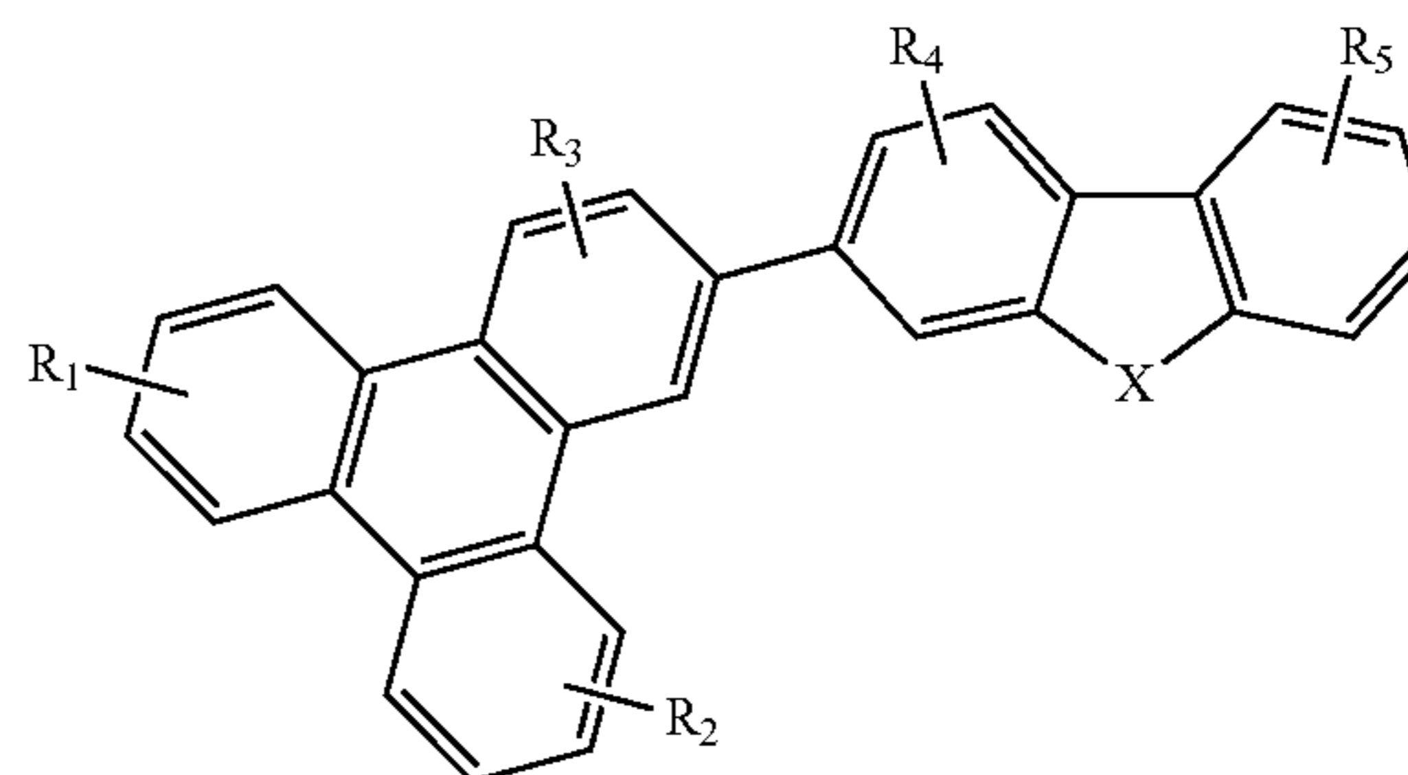
Compound 8
