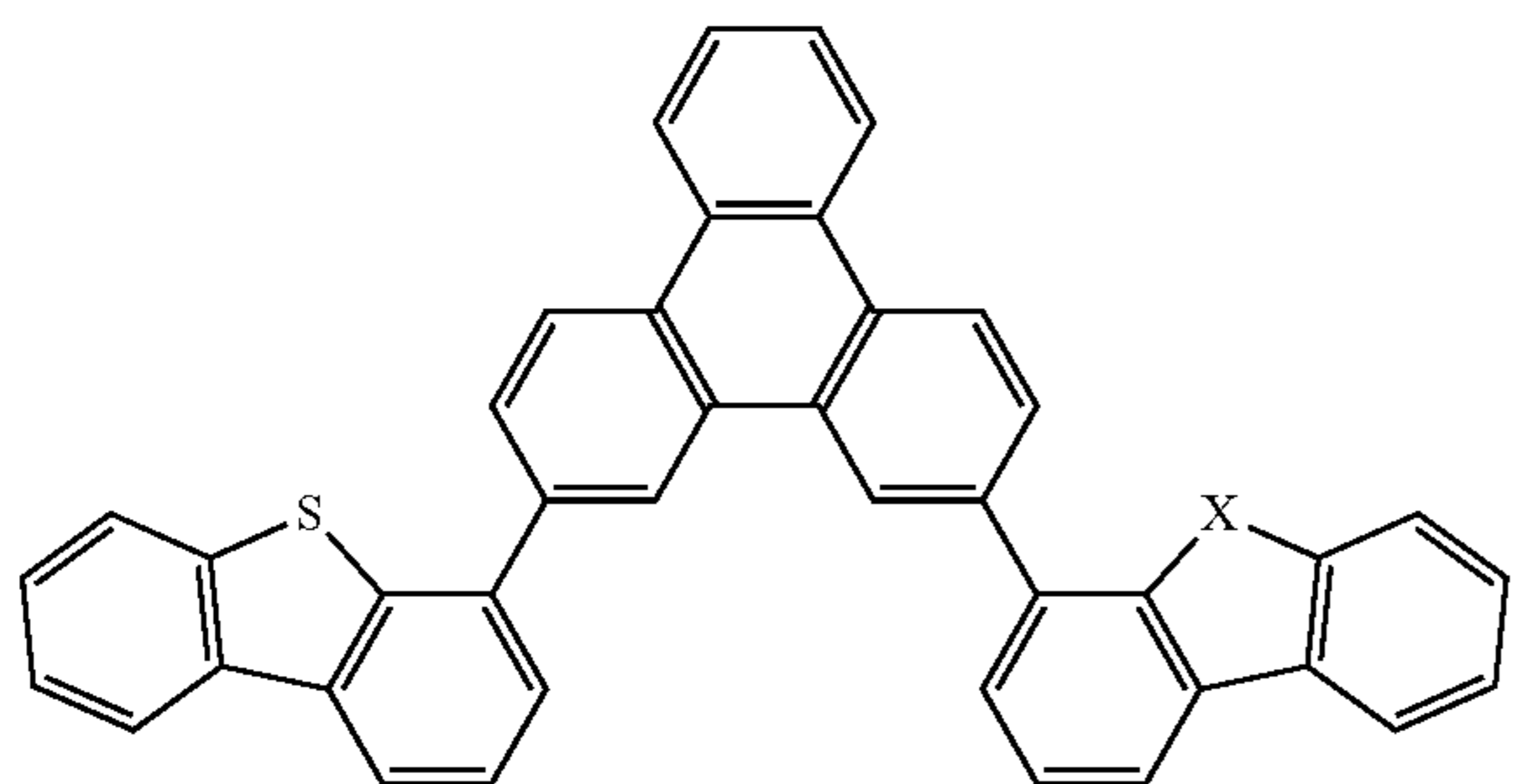
Compound 10
