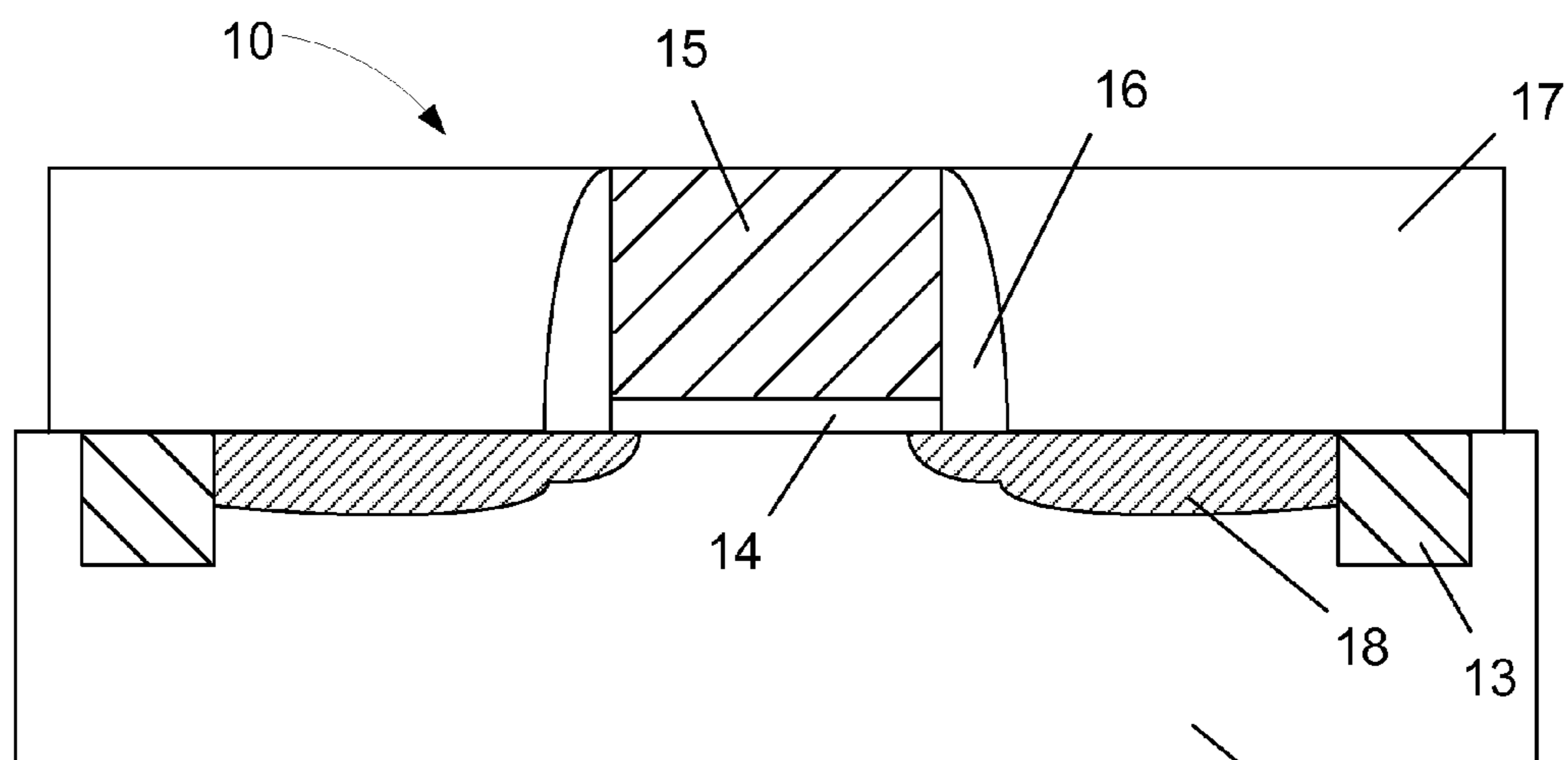
(Prior Art) Figure 1B 12
