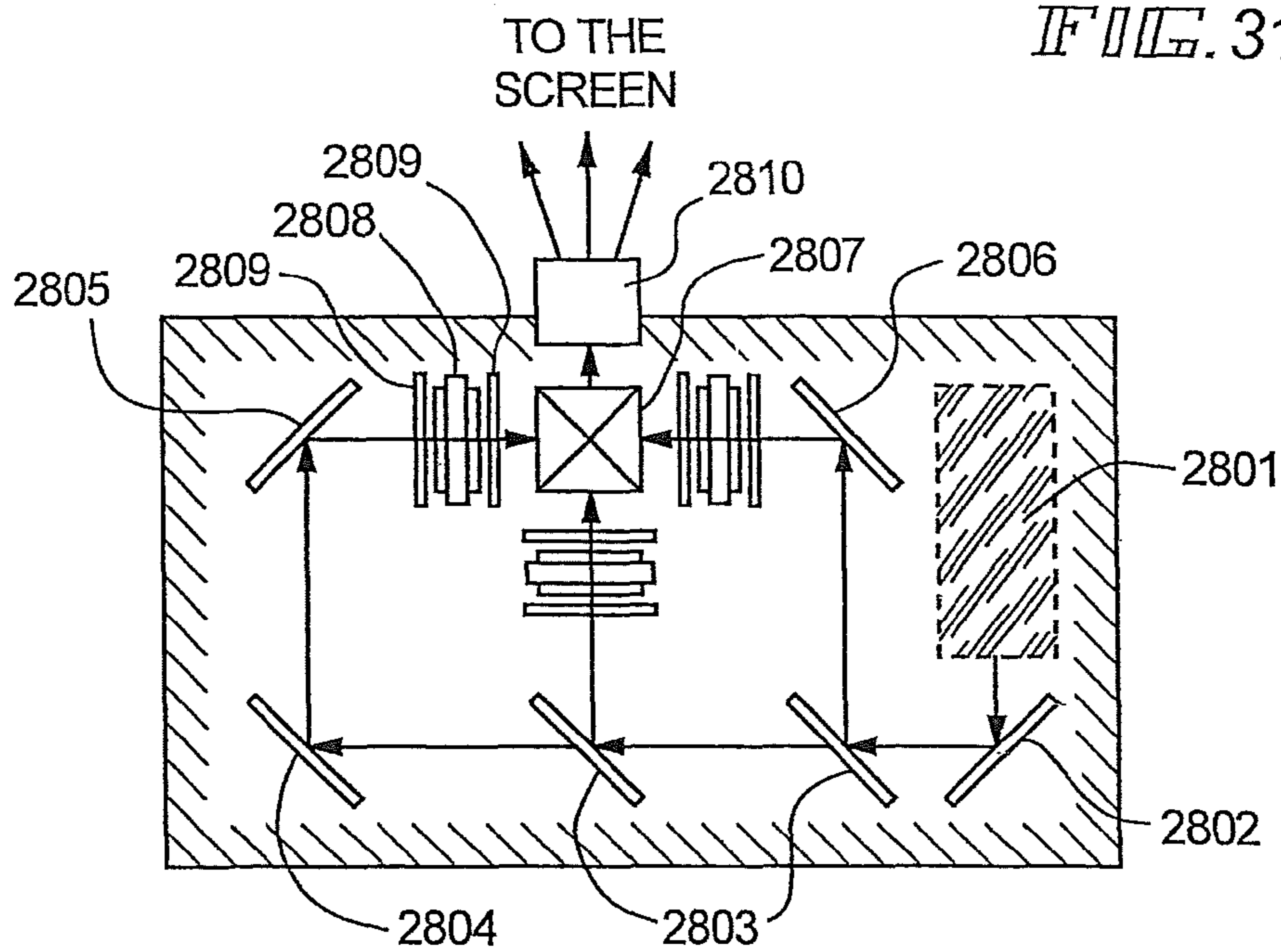
PROJECTION DEVICE (THREE PLATE TYPE)
