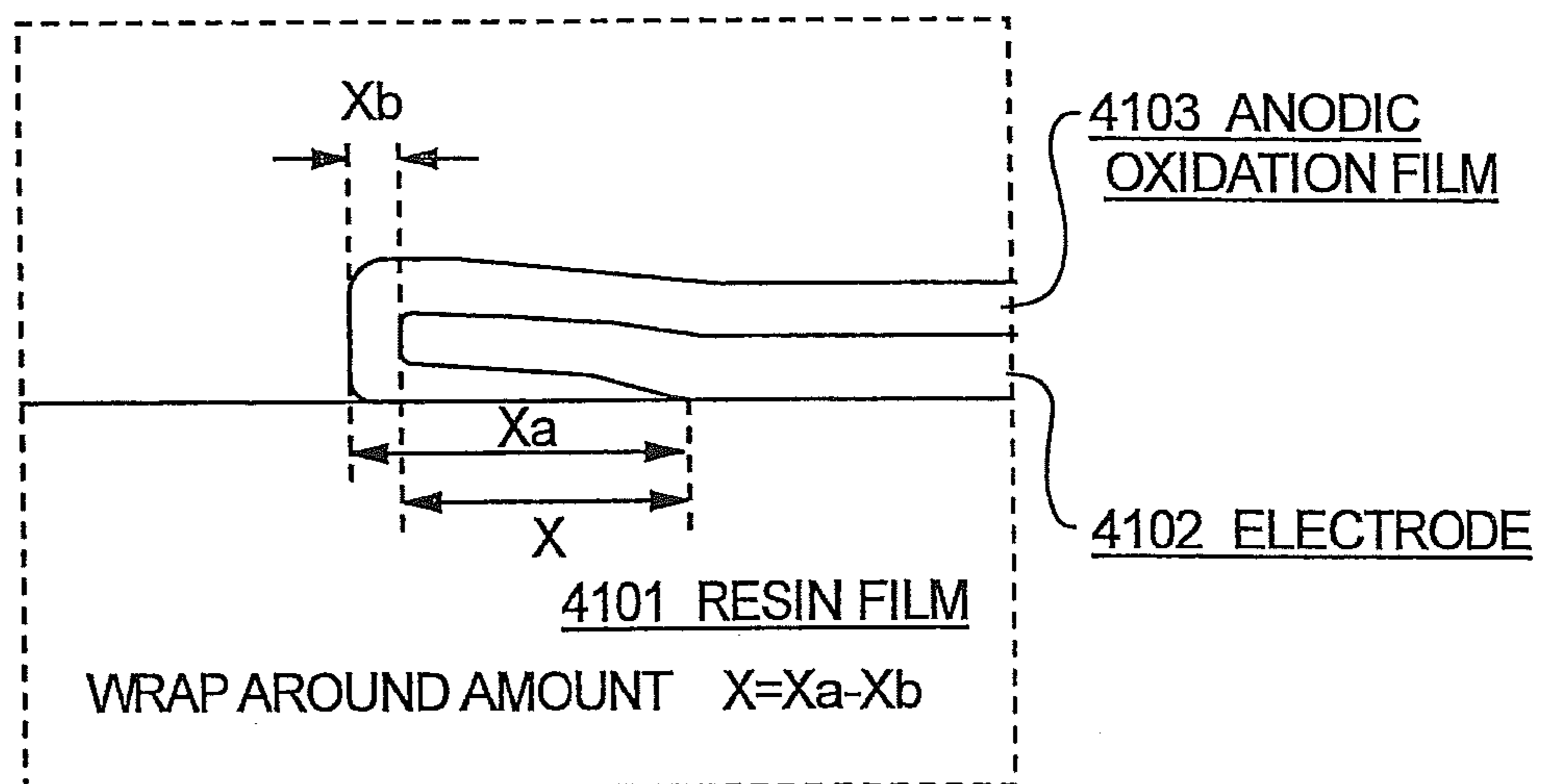
SCHEMATIC DIAGRAM OF ENLARGED ELECTRODE EDGE PORTION
