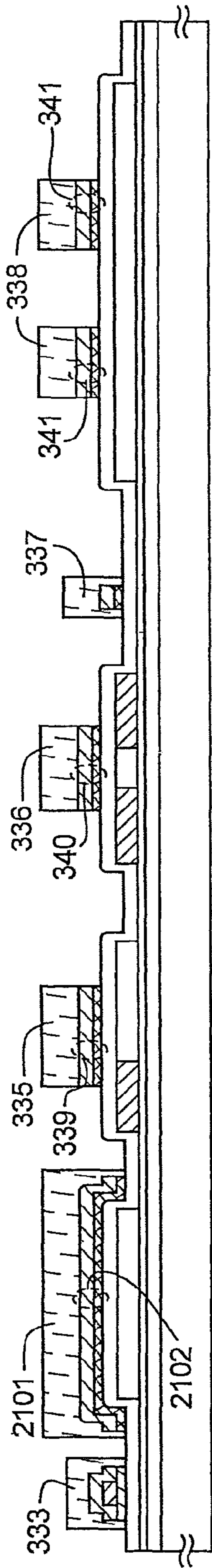
FIG. 21A FORMING n-ch TFT GATE WIRING
