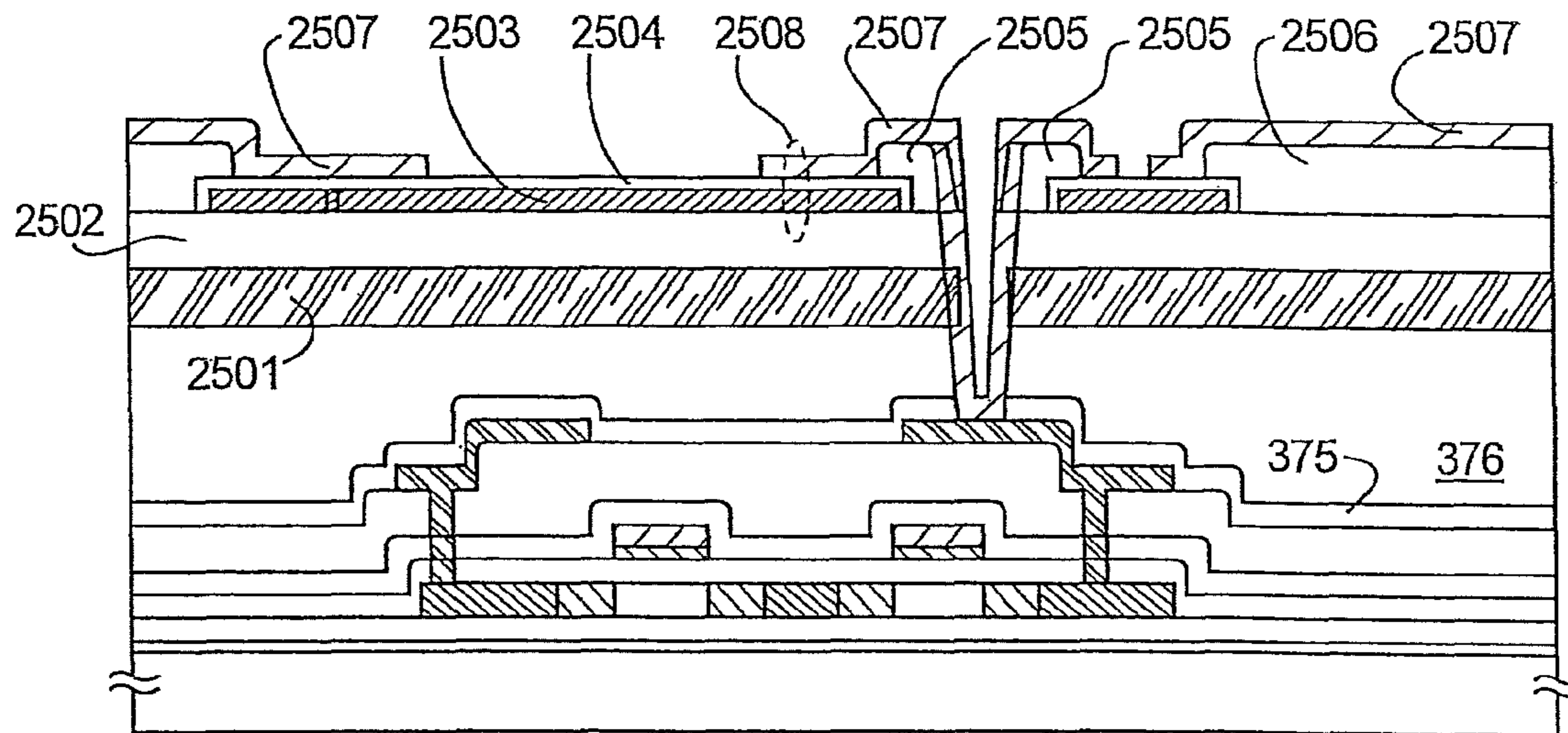
701: n-CHANNEL TFT
