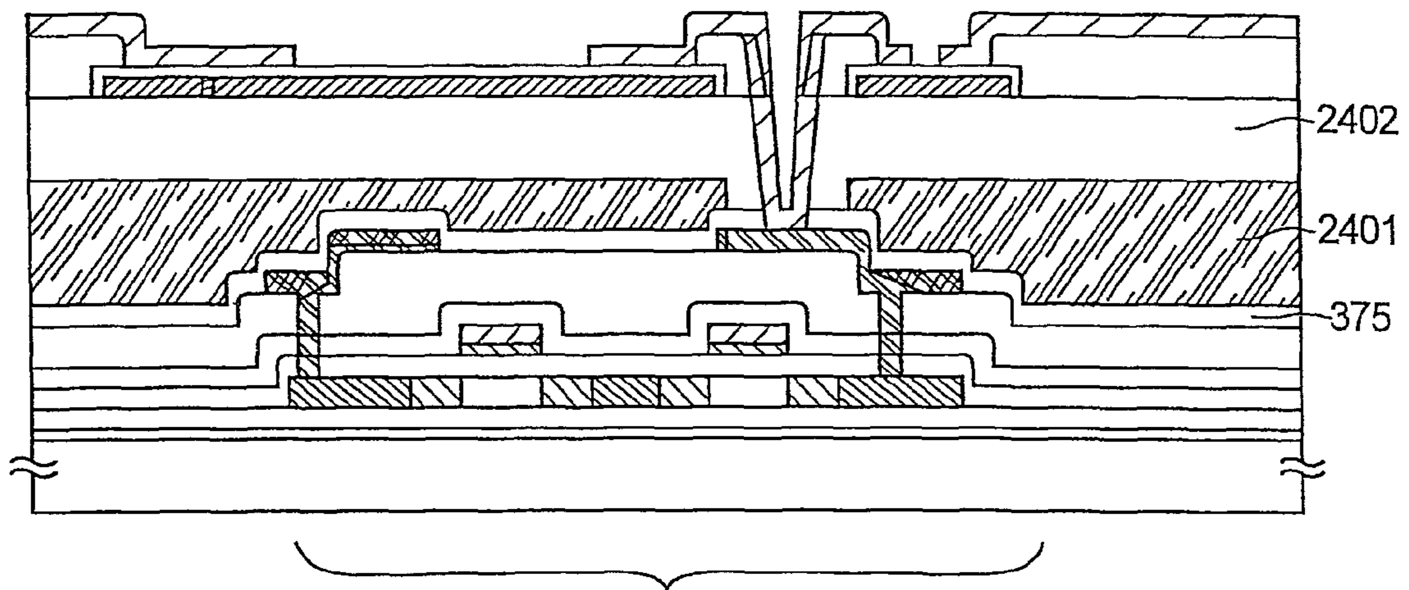
701: n-CHANNEL TFT
