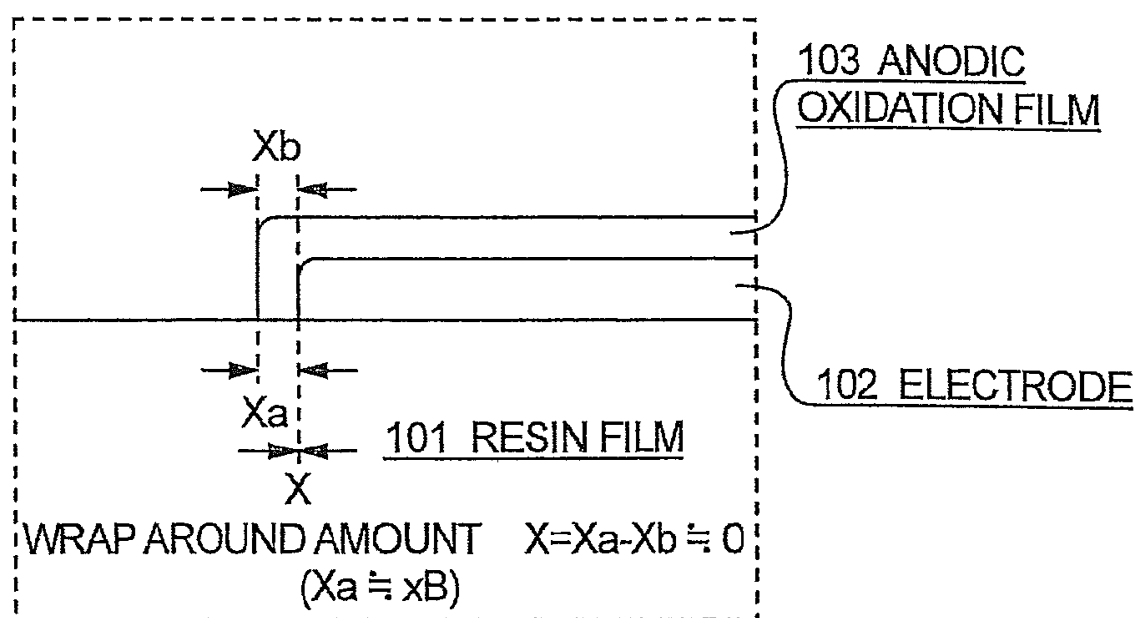
FIG. 1B SCHEMATIC DIAGRAM OF ENLARGED ELECTRODE EDGE PORTION
