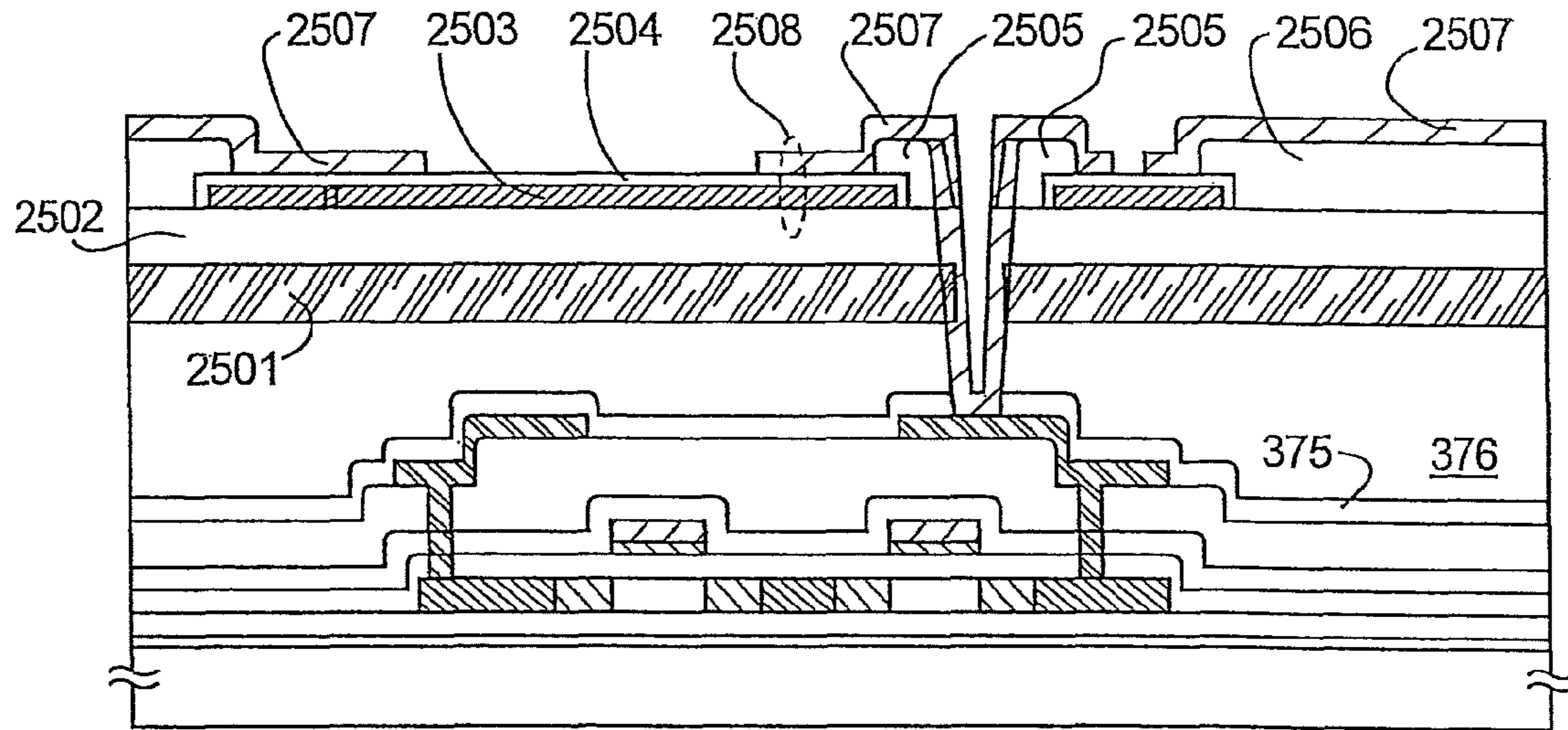
701: n-CHANNEL TFT
