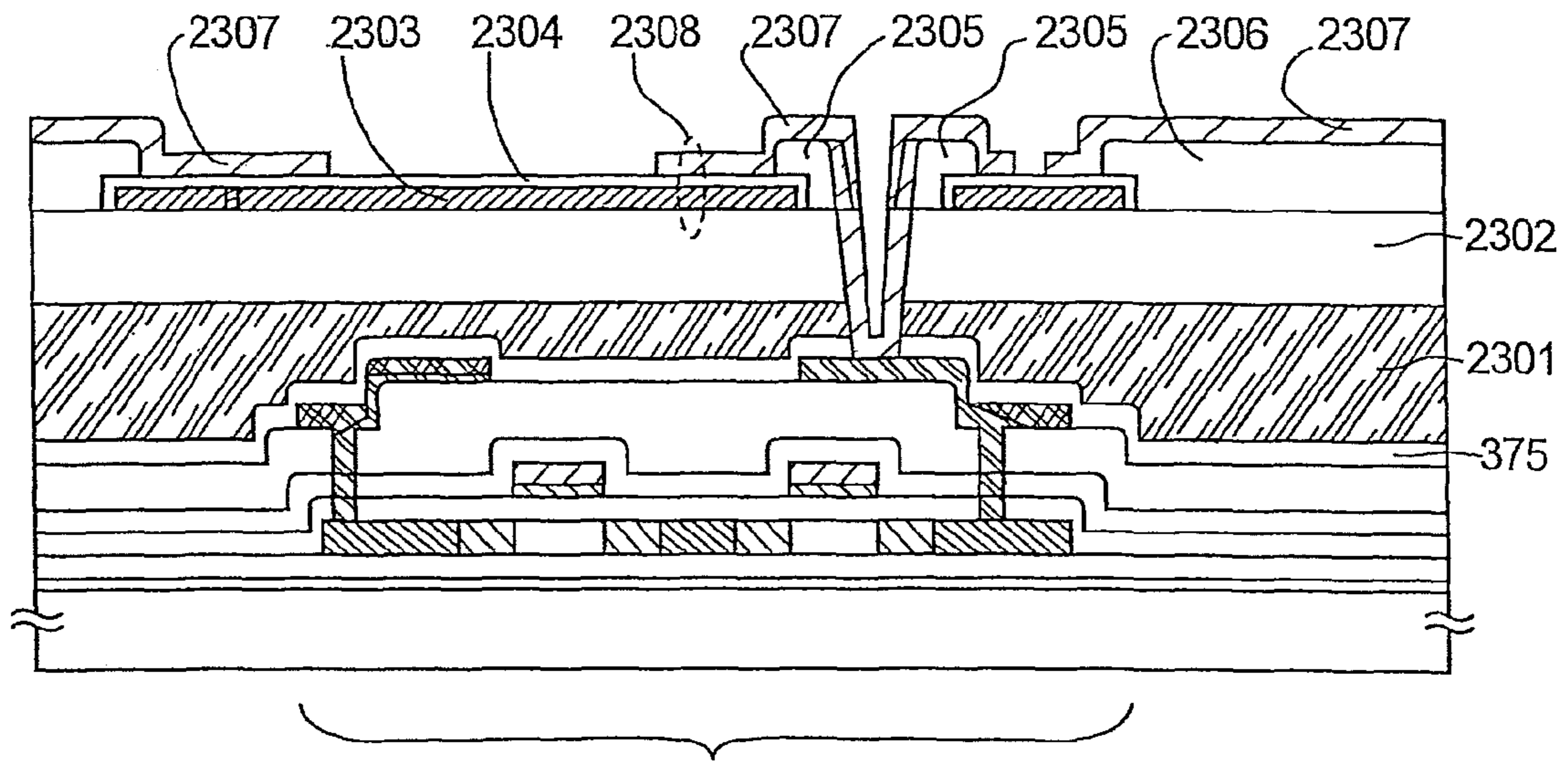
701: n-CHANNEL TFT
