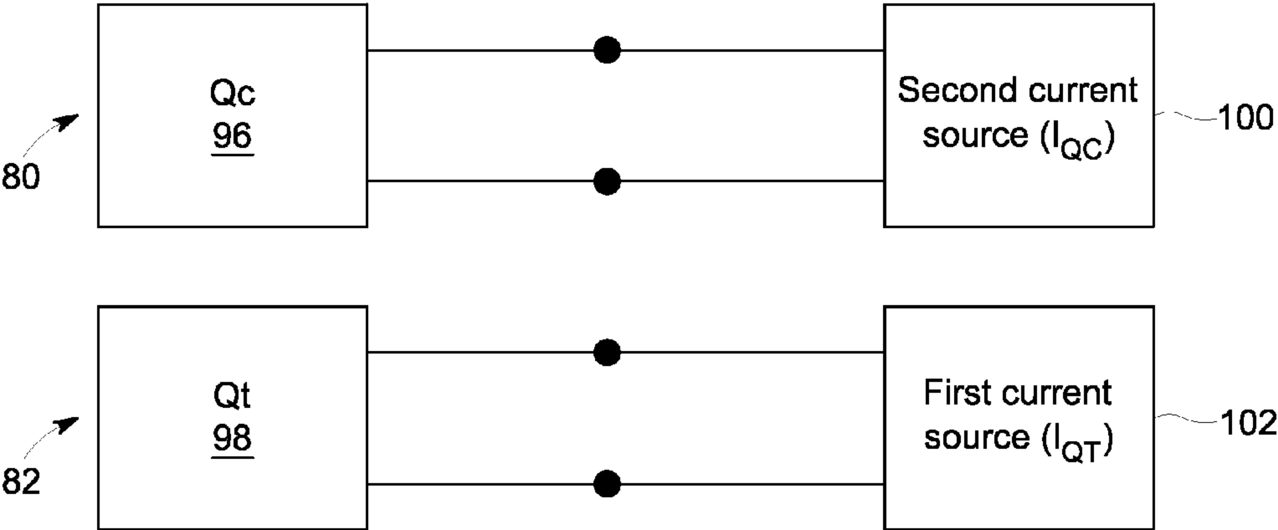
FIG. 5 PRIOR ART
