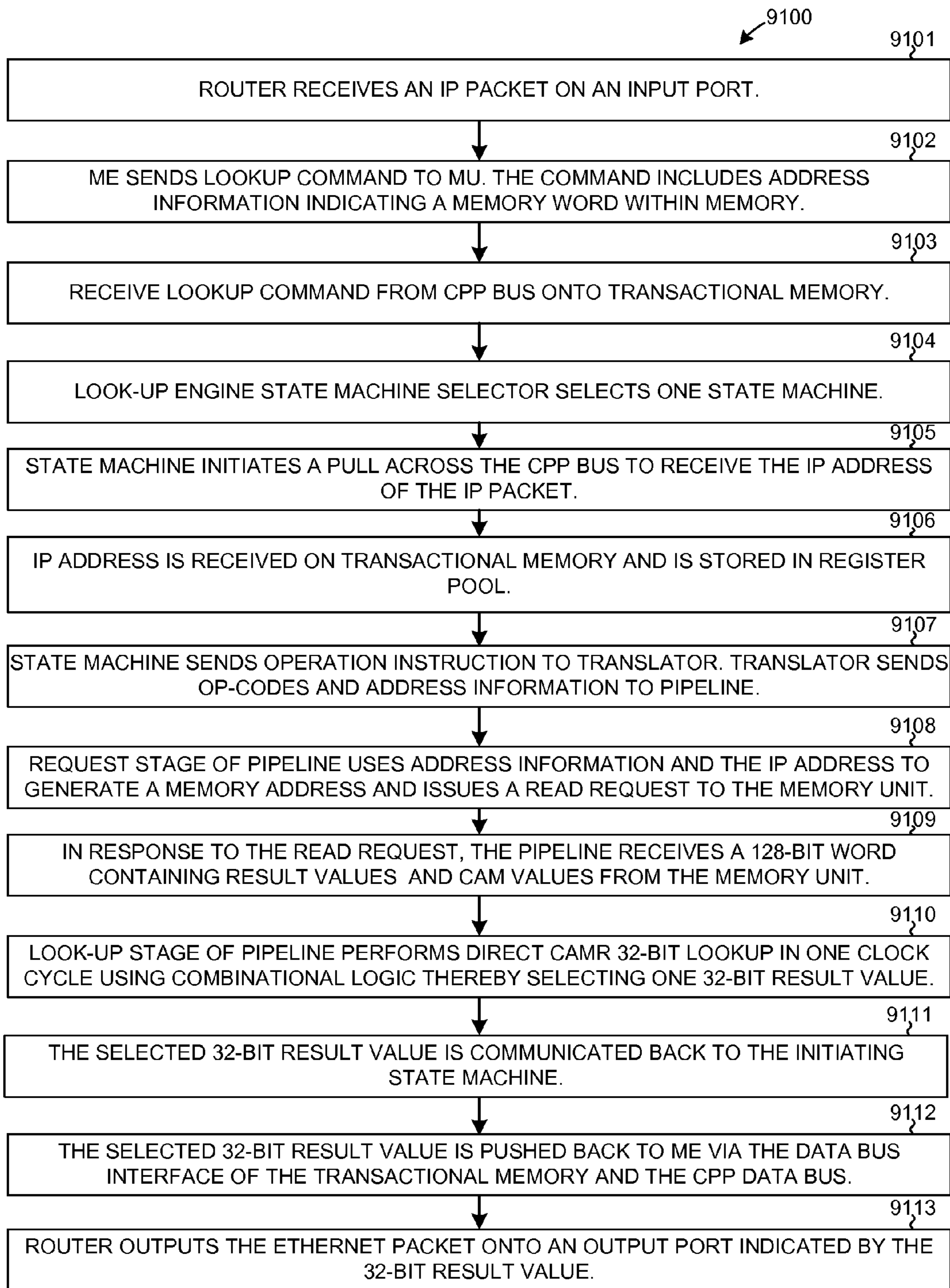
CAMR 32-BIT LOOKUP FLOWCHART FIG. 55
