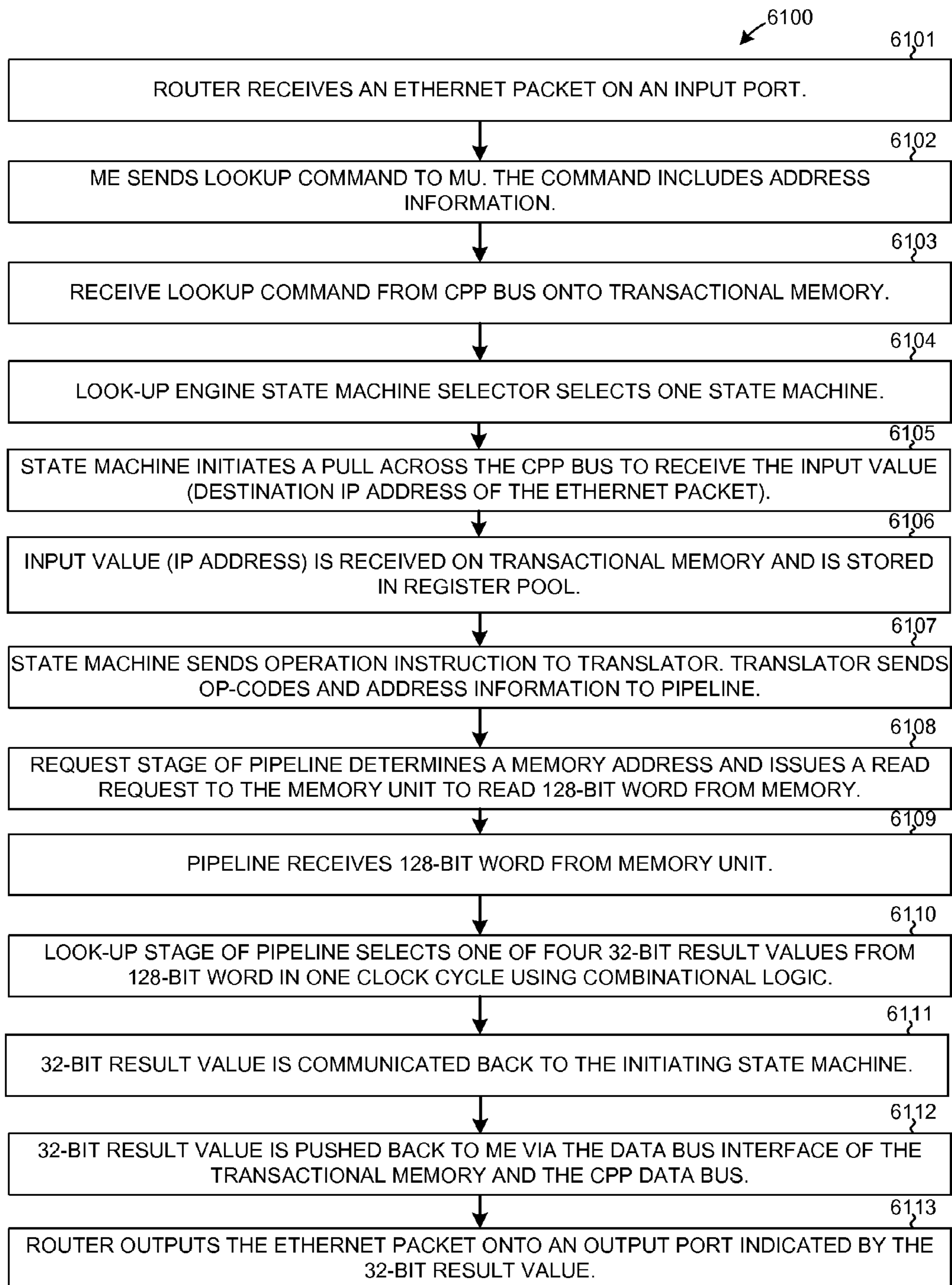
DIRECT 32-BIT LOOKUP FLOWCHART FIG. 44
