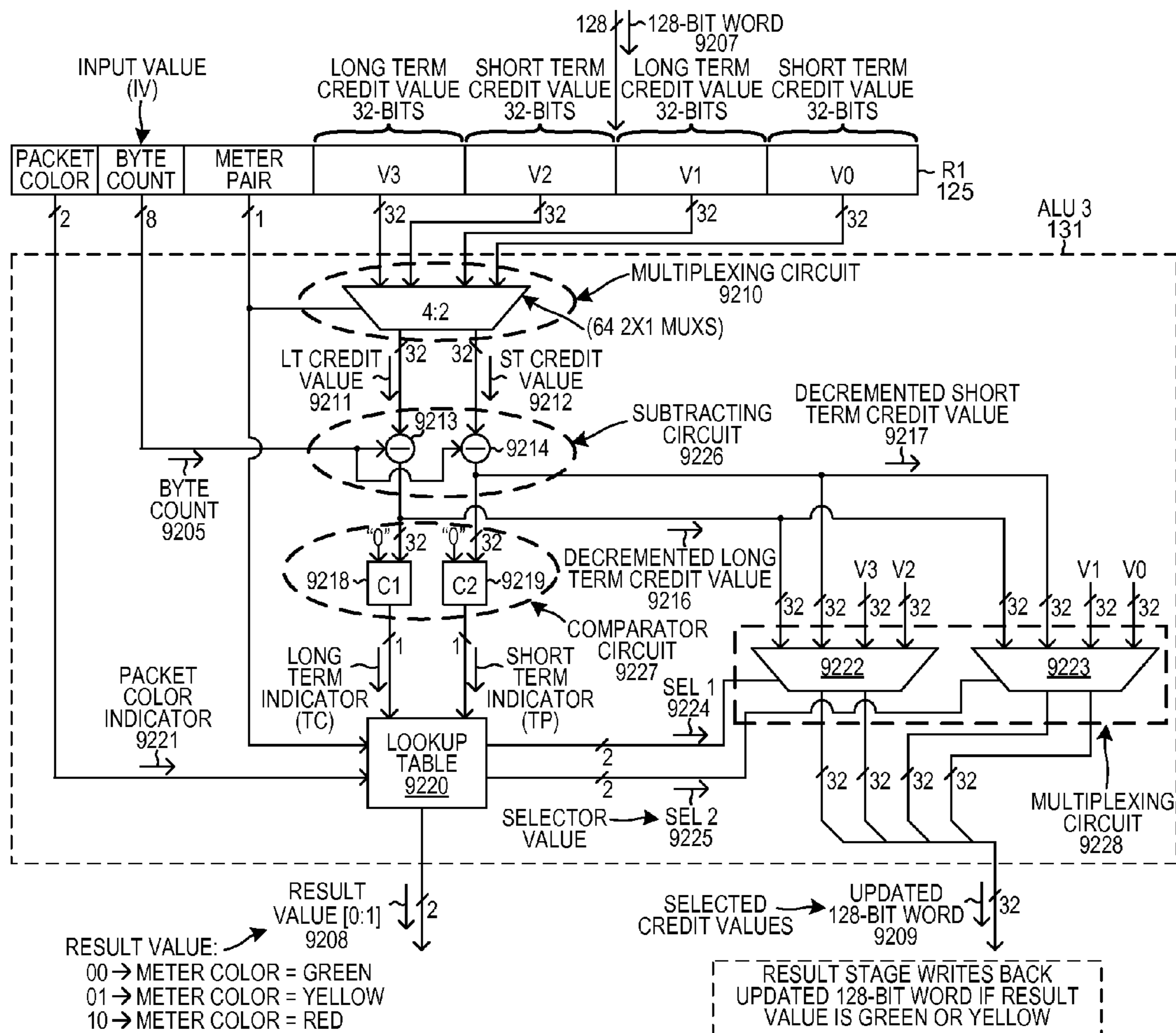
ATOMIC METERING COMMAND LOOKUP STAGE FIG. 59
