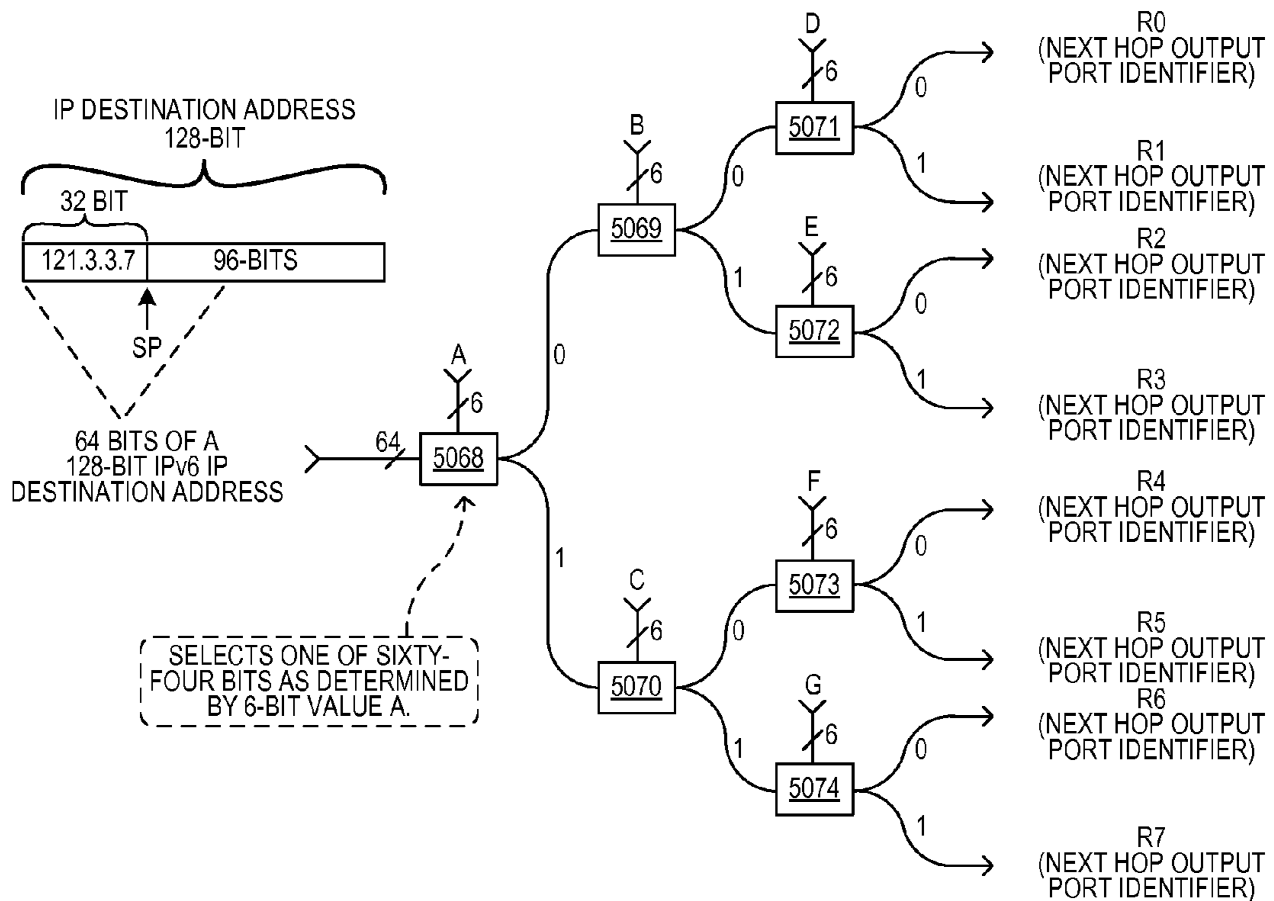
CONCEPTUAL DIAGRAM OF TRIE MULTI-BIT LOOKUP OPERATION FIG. 37
