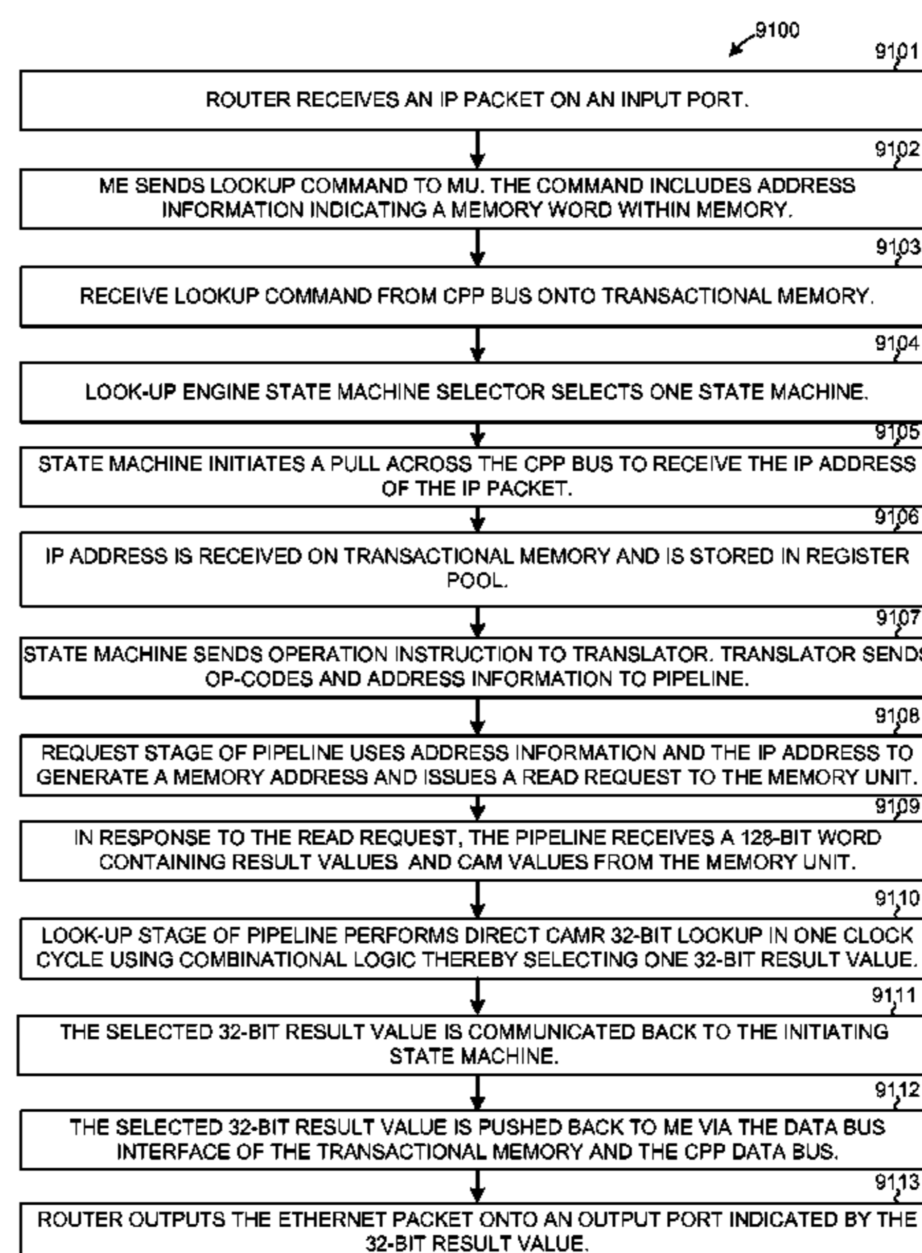
CAMR 32-BIT LOOKUP FLOWCHART
