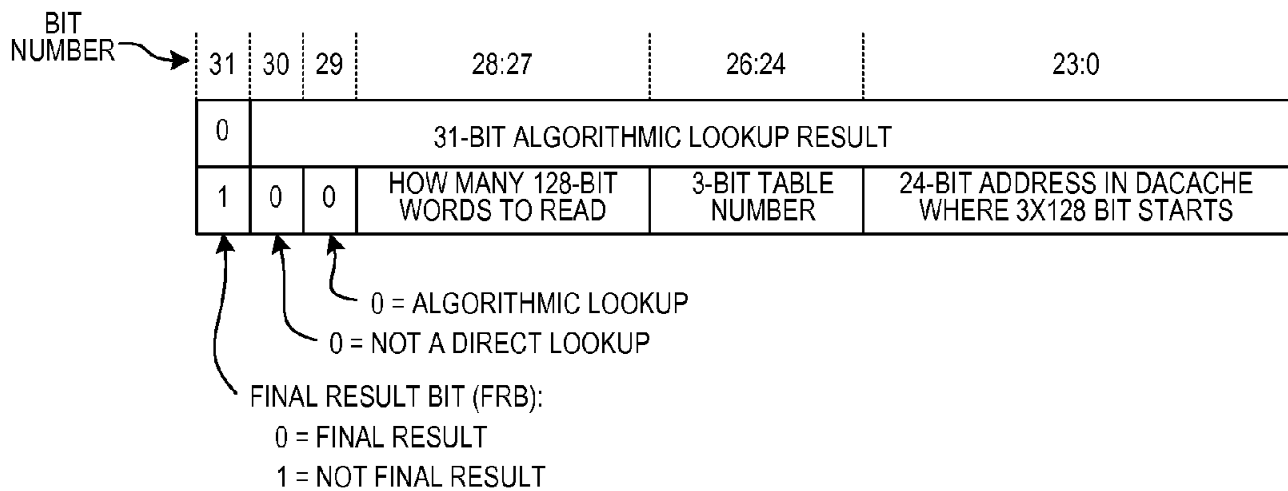
RESULT VALUE (IF THE ALGORITHMIC LOOKUP BIT IS ZERO) FIG. 38
