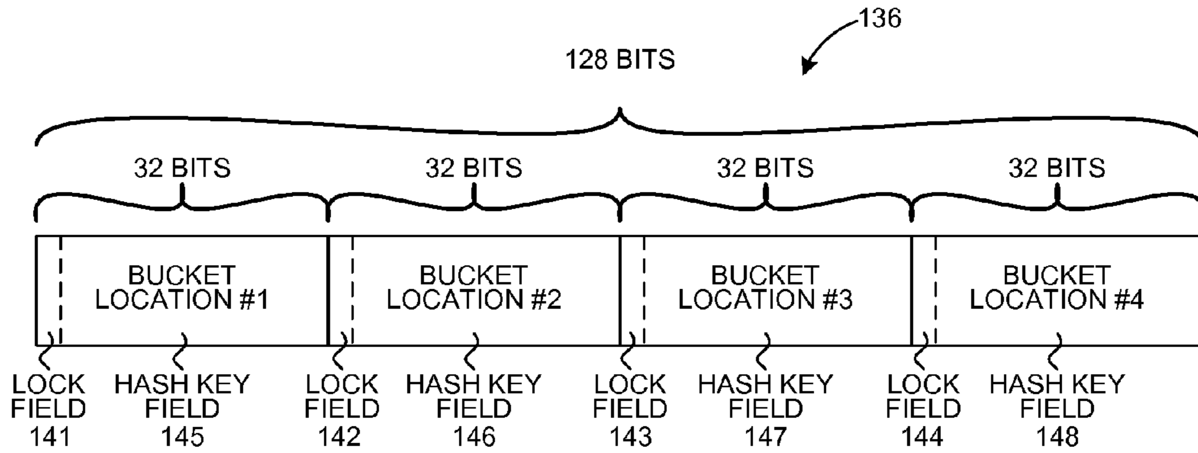
HASH BUCKET FIG. 19
