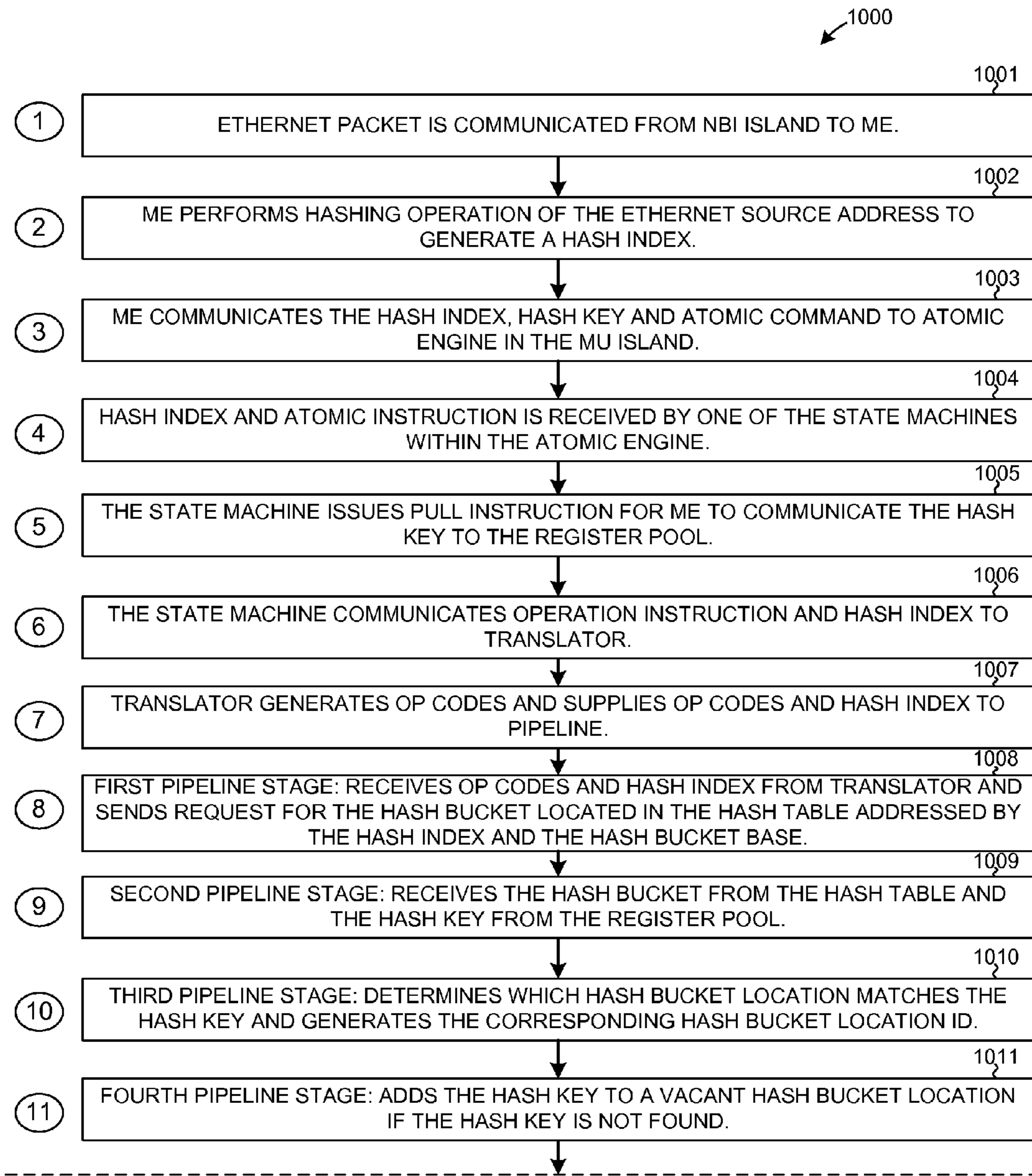
TRANSACTIONAL MEMORY FLOWCHART
