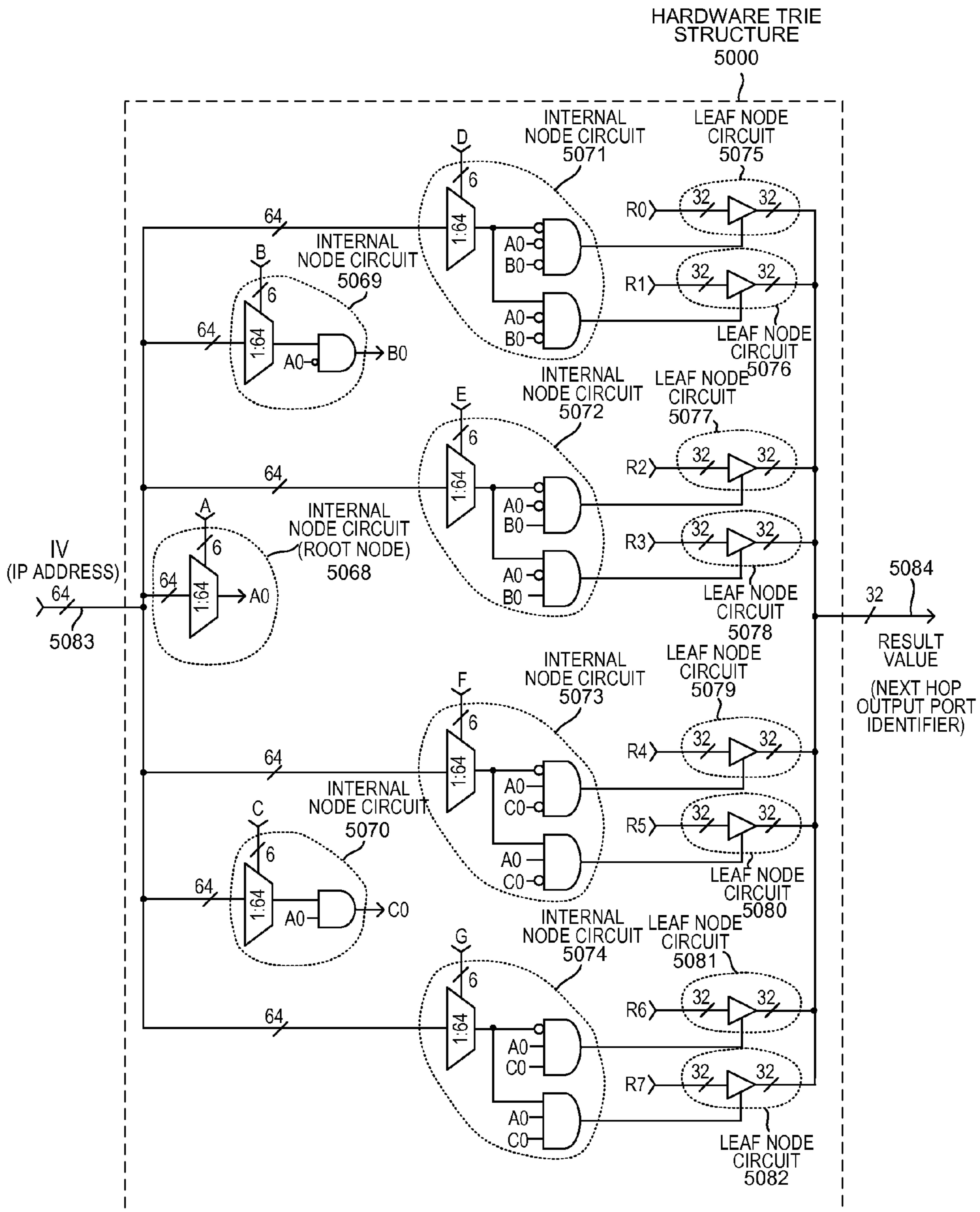
HARDWARE TRIE STRUCTURE FIG. 36
