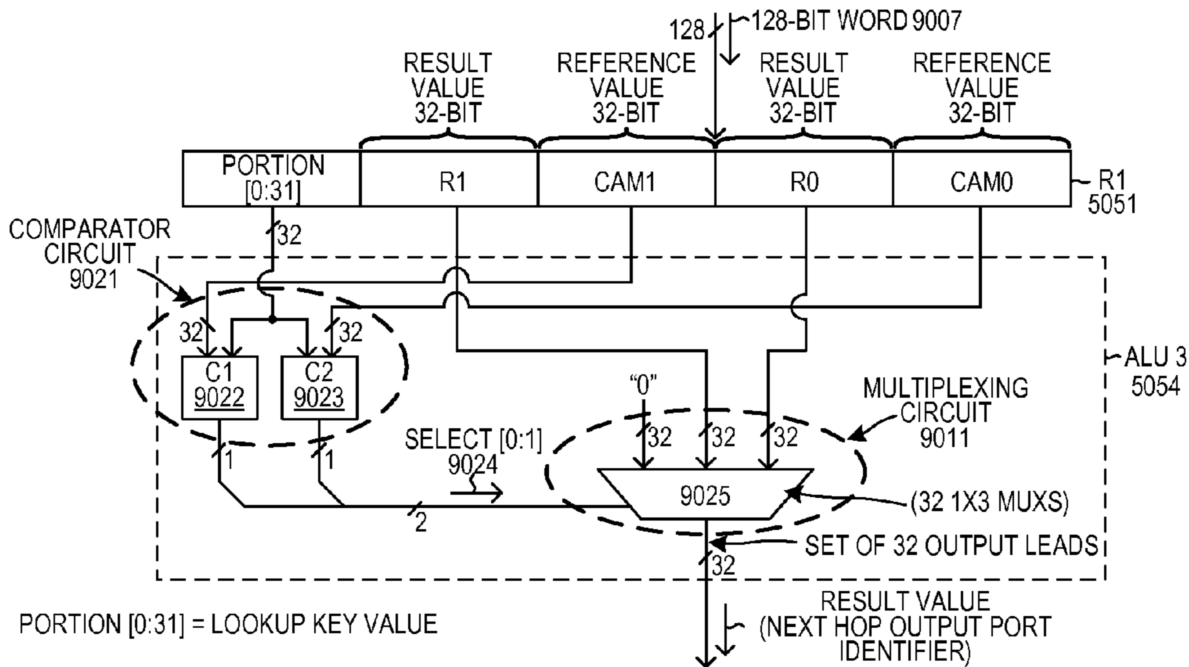
DIRECT CAMR 32-BIT LOOKUP STAGE FIG. 54
