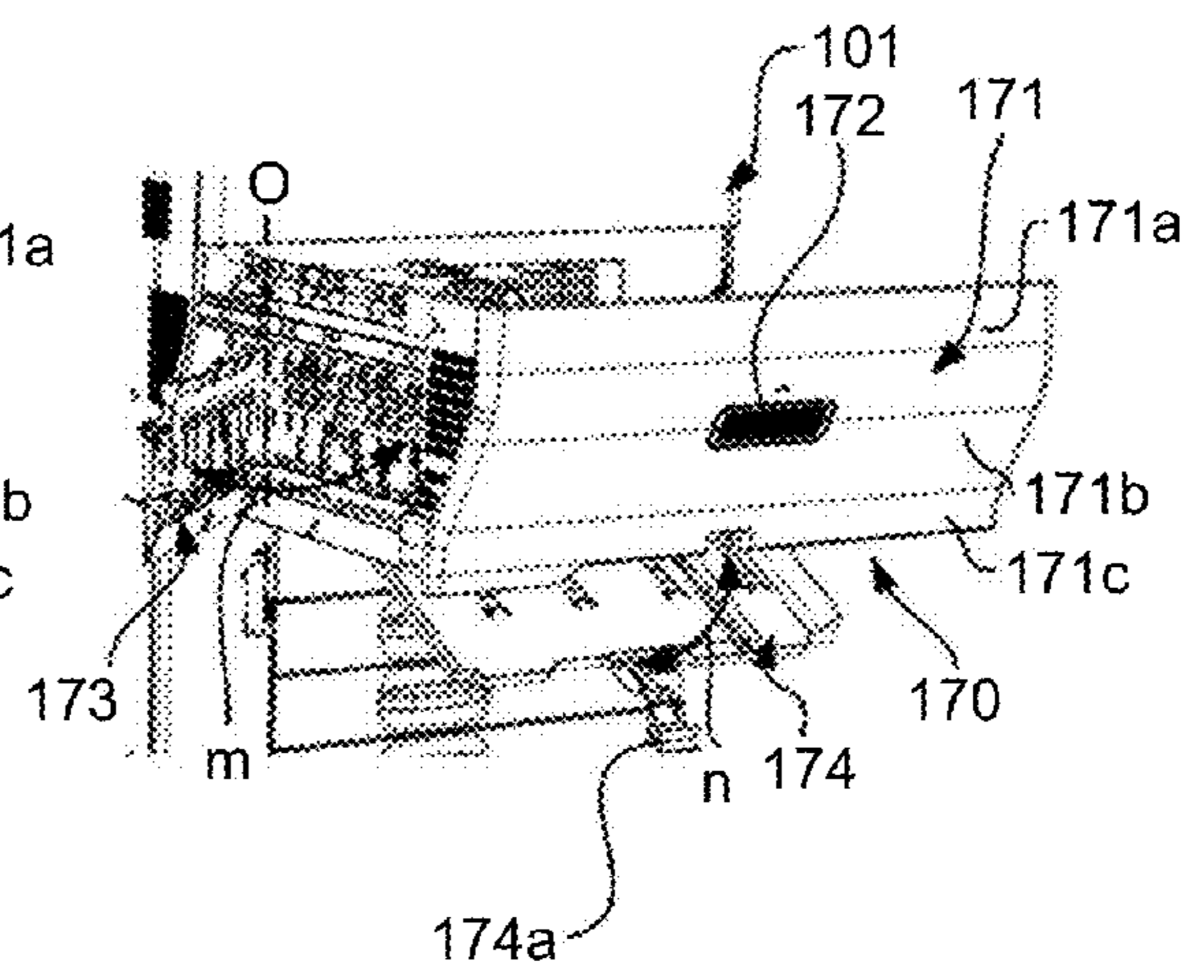
FIG.5C
